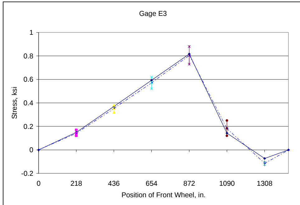
Fig. D.39: Field Test No. 1 - Member L4U5 of upstream truss
