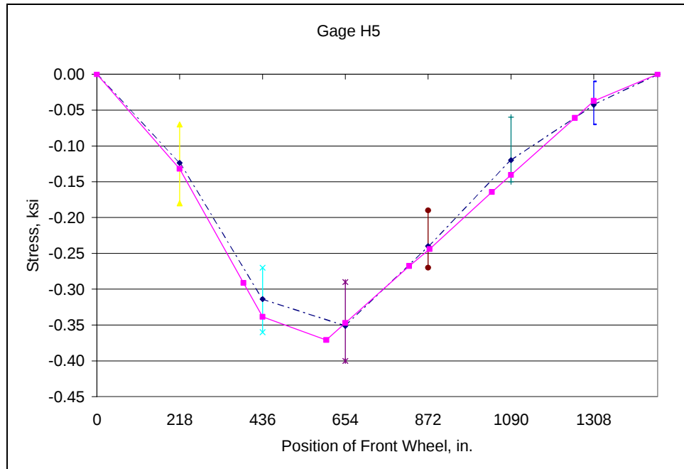
Fig. D.63: Field Test No. 2 - Top chord U2U3
