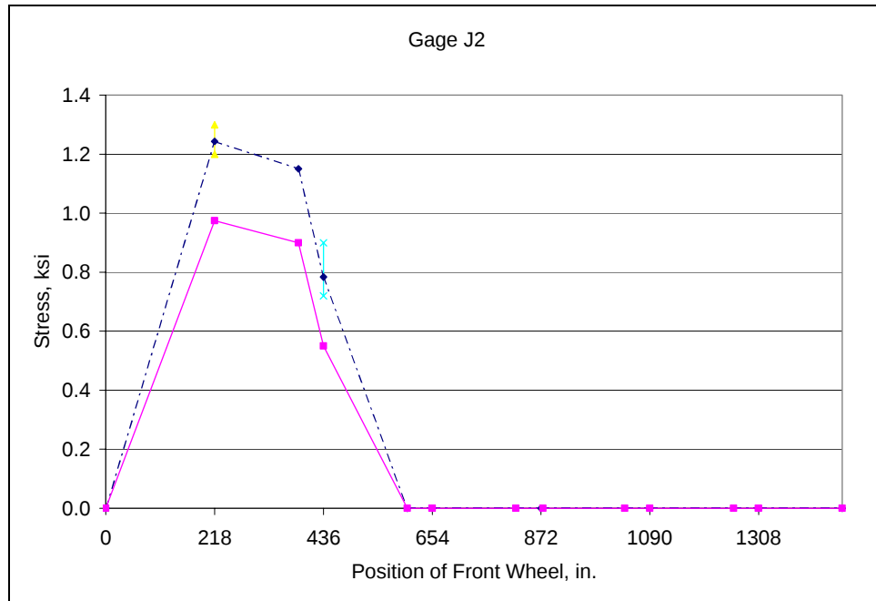
Fig. D.71: Field Test No. 2 - Vertical hanger L1U1
