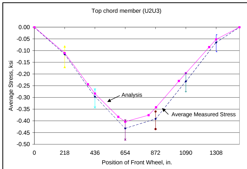
Figure 5.12: Average stress in top chord member U2U3
