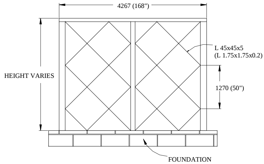
Figure 2.6: Details of typical metal bent
