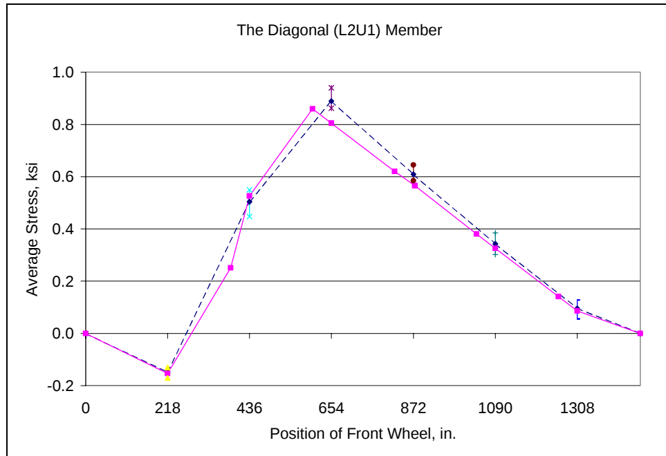
Fig. D.93: Field Test No. 2 - Average stress: Diagonal member (L2U1)
