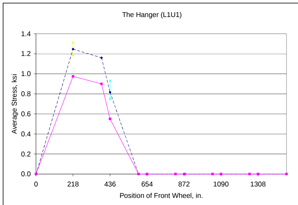
Fig. D.92: Field Test No. 2 - Average stress: Vertical hanger (L1U1)
