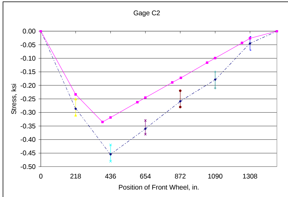
Fig. D.51: Field Test No. 2 - Top chord L0U1
