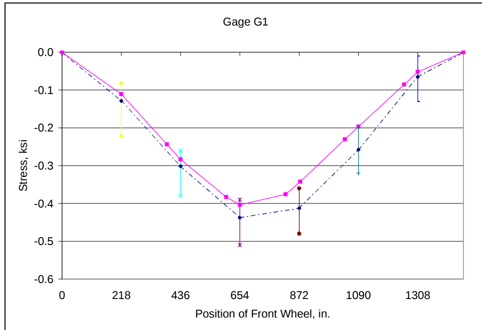
Fig. D.55: Field Test No. 2 - Top chord U1U2
