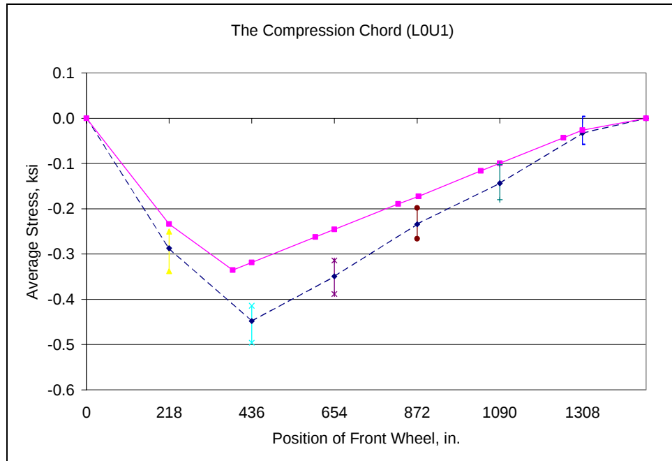
Fig. D.89: Field Test No. 2 - Average stress: Top chord (L0U1)
