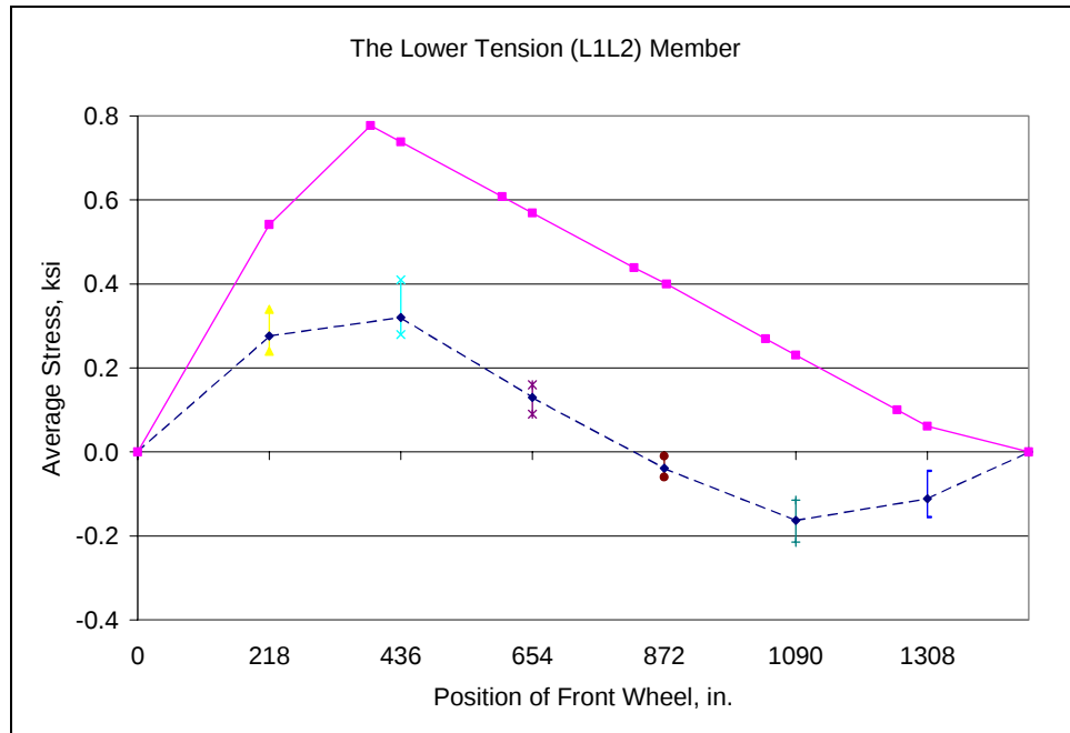
Fig. D.87: Field Test No. 2 - Average stress: Bottom chord (L1L2)
