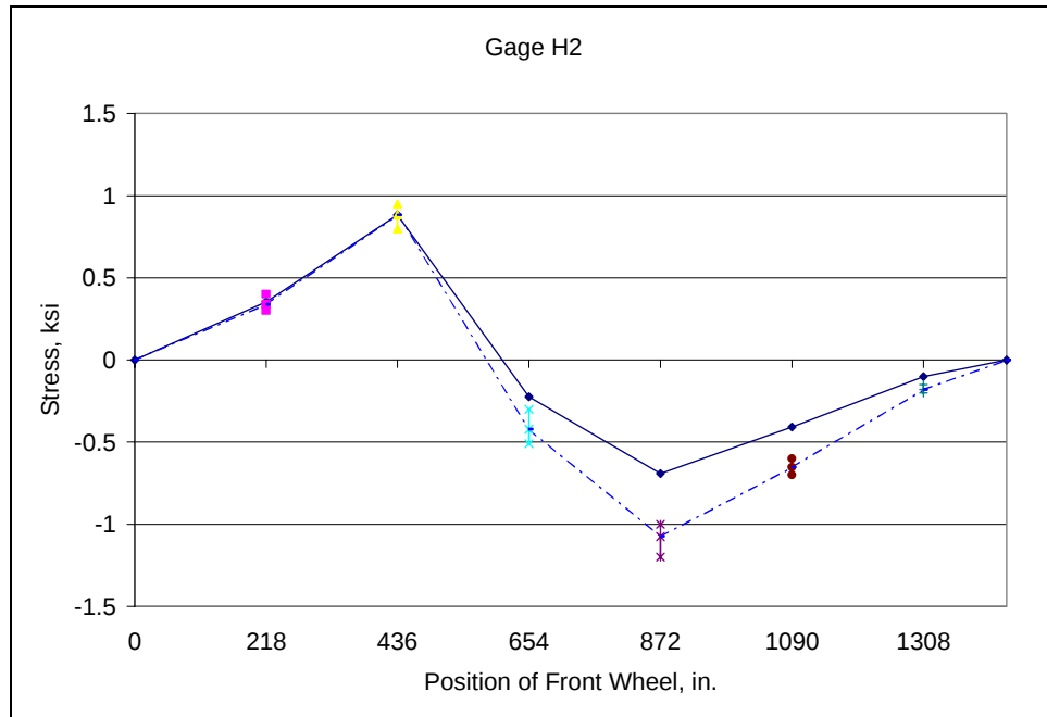
Fig. D.37: Field Test No. 1 - Member L2U3 of downstream truss
