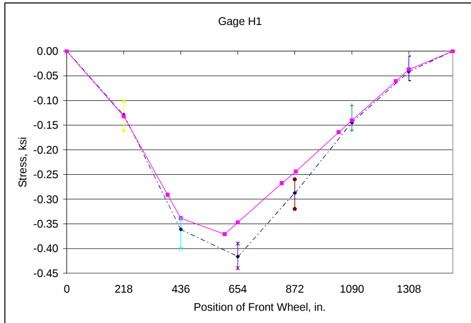
Fig. D.59: Field Test No. 2 - Top chord U2U3
