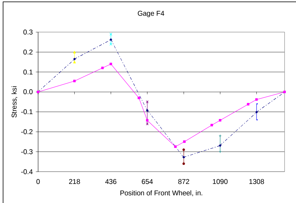
Fig. D.85: Field Test No. 2 - Vertical member L2U2
