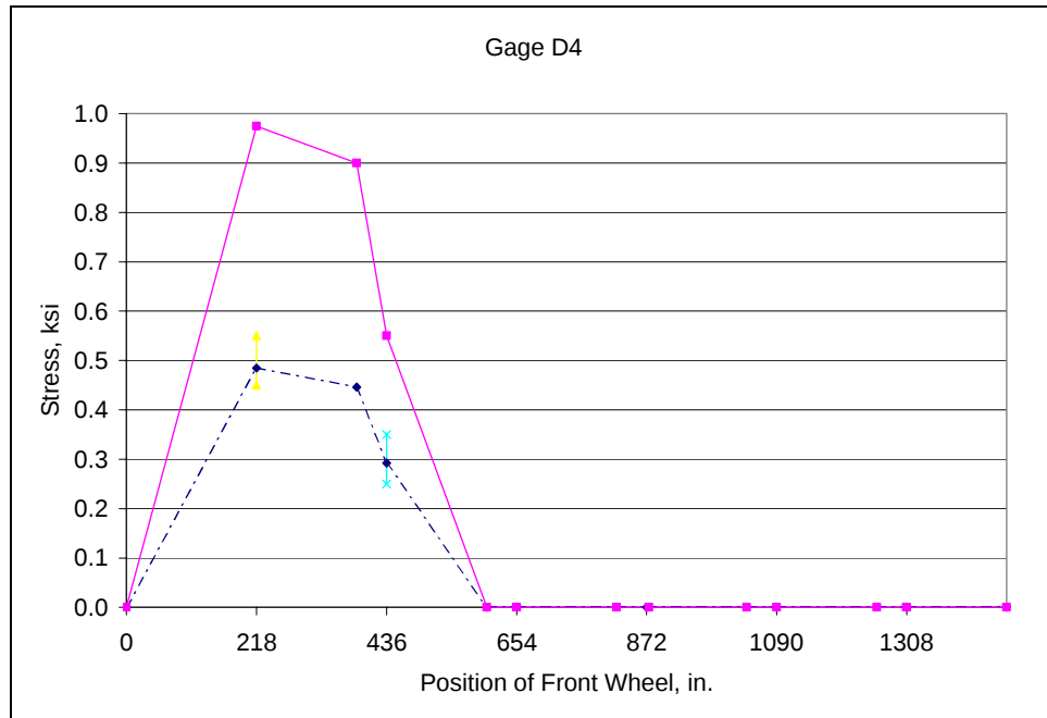
Fig. D.67: Field Test No. 2 - Vertical hanger L1U1
