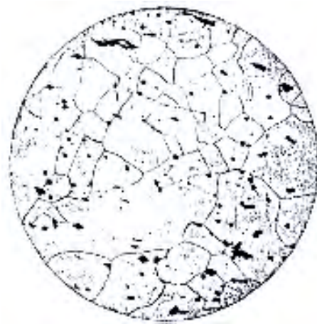
Figure C.2: Transverse section of wrought iron
