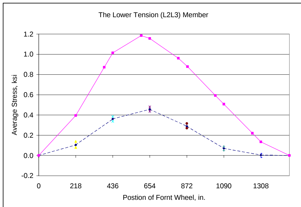
Fig. D.88: Field Test No. 2 - Average stress: Bottom chord (L2L3)
