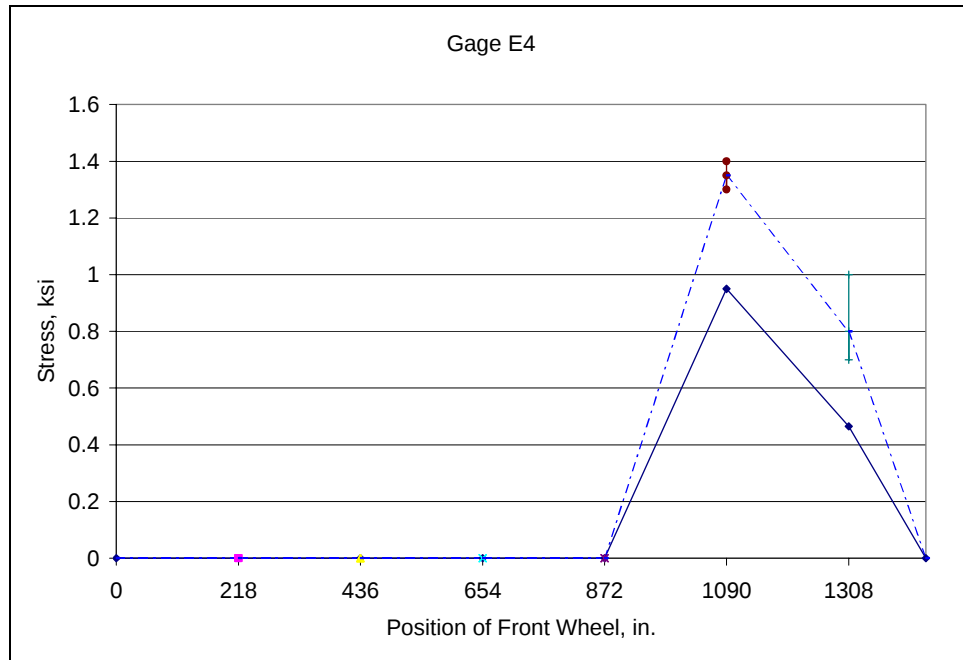
Fig. D.33: Field Test No. 1 - Member L5U5 of upstream truss
