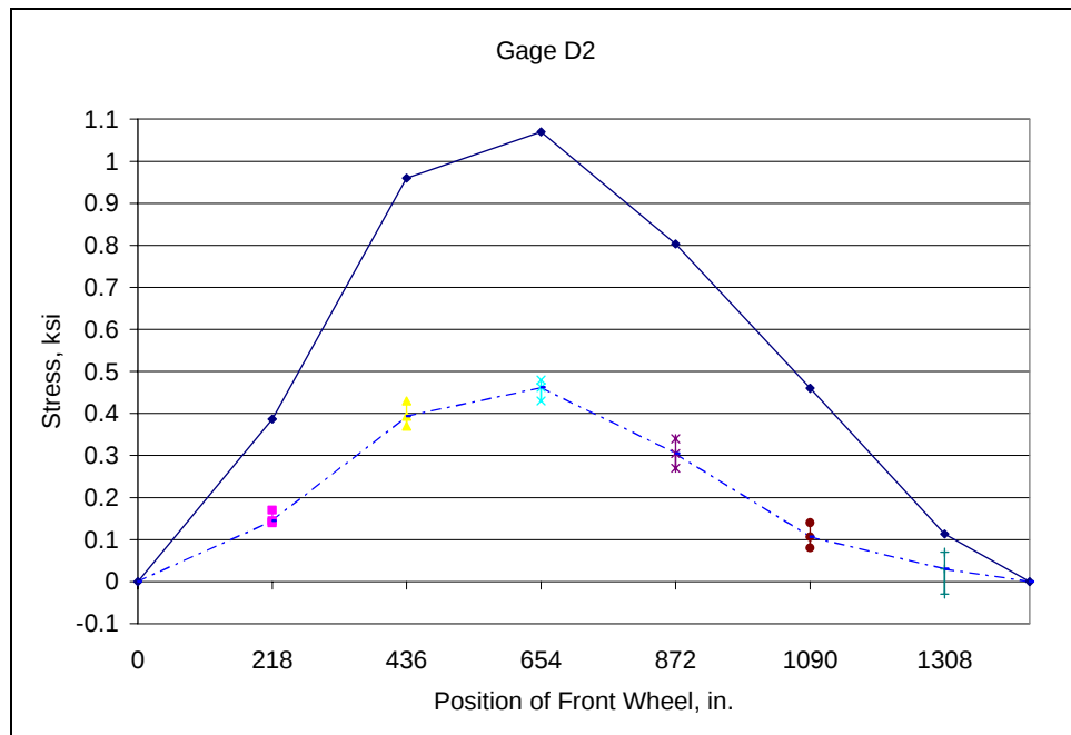
Fig. D.8: Field Test No. 1 - Member L2L3 (Inside) of upstream truss
