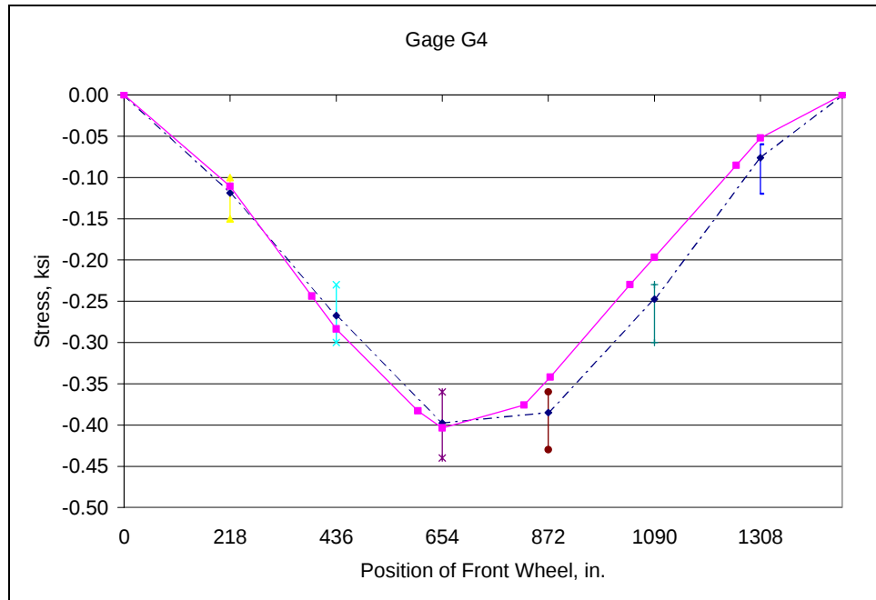
Fig. D.57: Field Test No. 2 - Top chord U1U2
