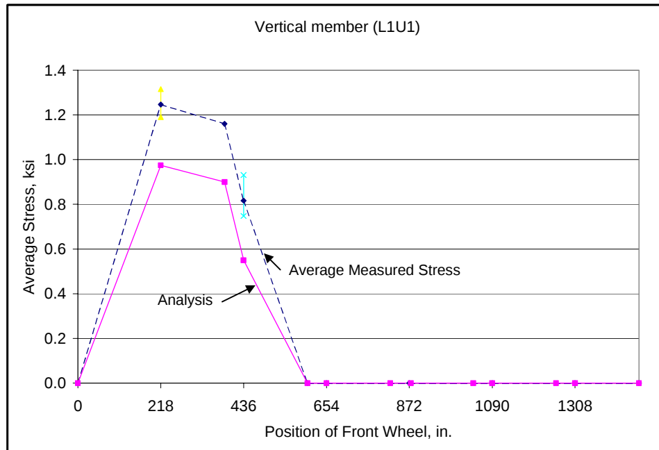
Figure 5.14: Average stress in vertical member L1U1
