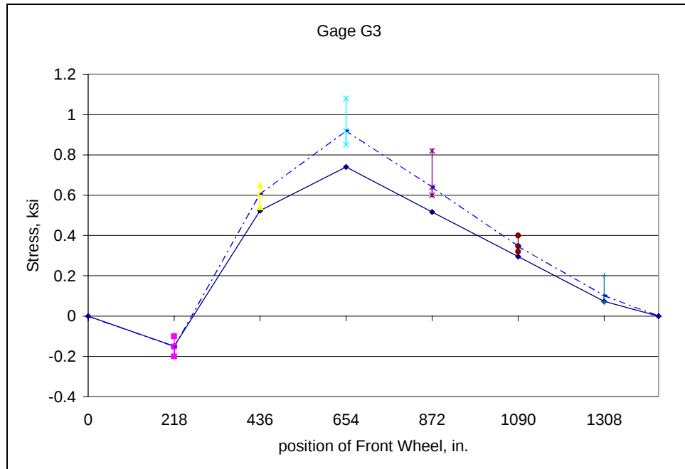
Fig. D.35: Field Test No. 1 - Member L2U1 of downstream truss
