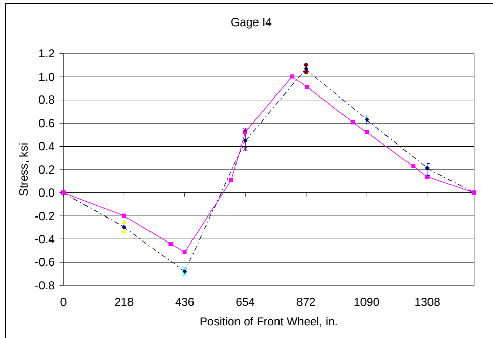
Fig. D.79: Field Test No. 2 - Diagonal member L3U2
