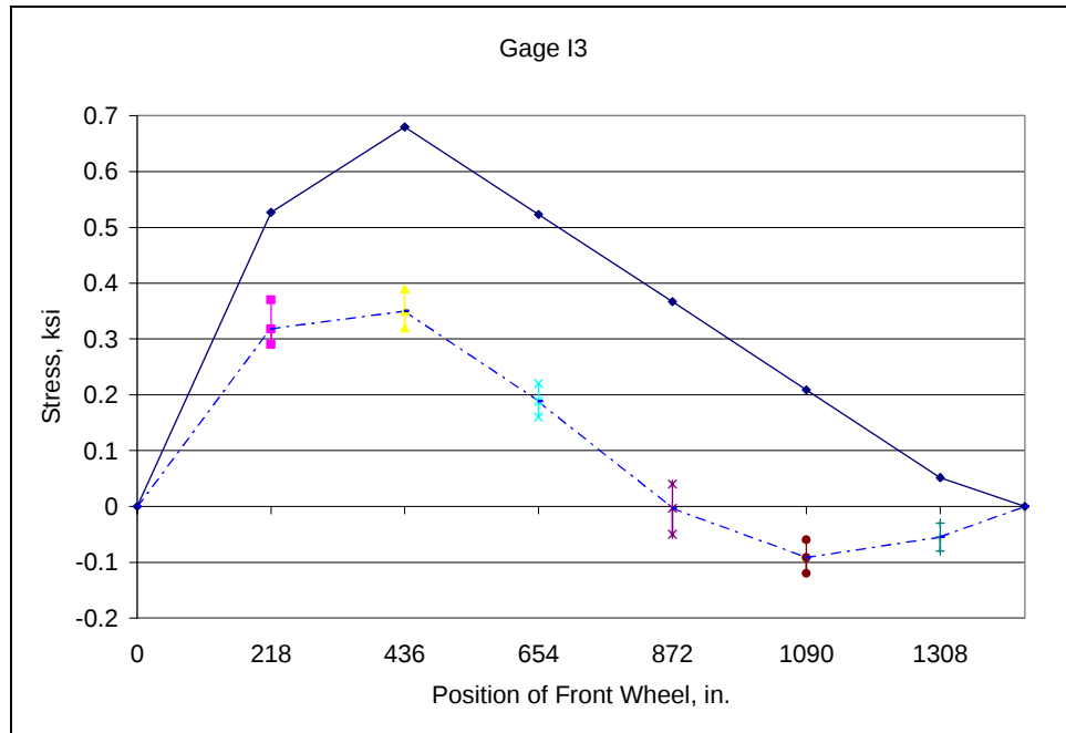
Fig. D.5: Field Test No. 1 - Member L1L2 (Inside) of upstream truss
