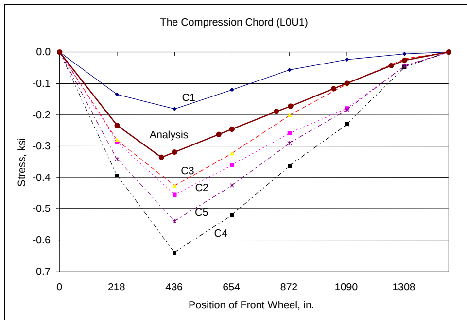
Fig. D.98: Field Test No. 2 - Stress variation: Top chord (L0U1)
