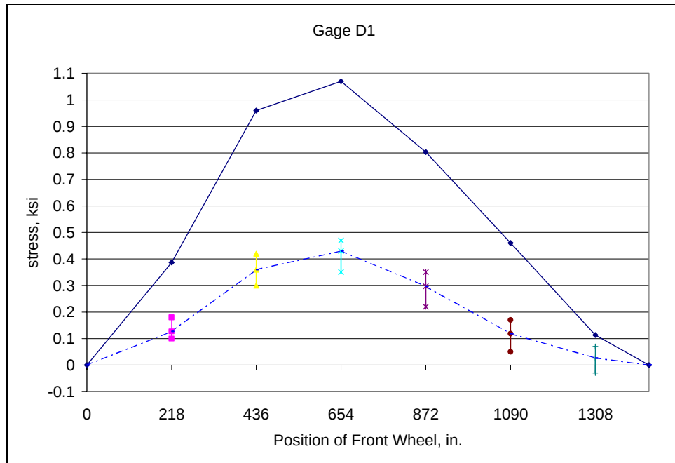
Fig. D.7: Field Test No. 1 - Member L2L3 (Outside) of upstream truss
