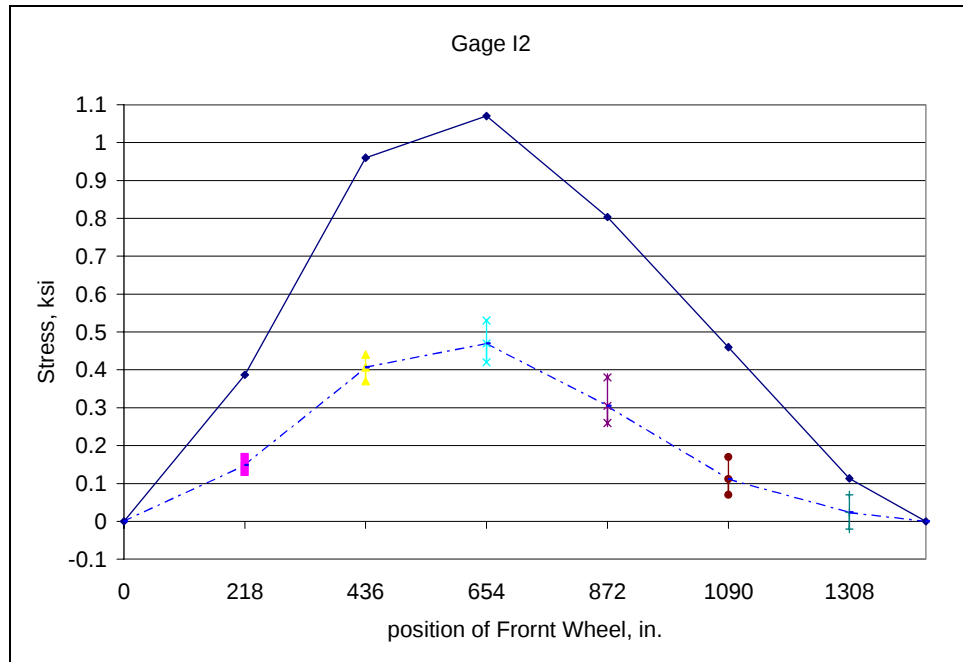
Fig. D.9: Field Test No. 1 - Member L2L3 (Outside) of downstream truss
