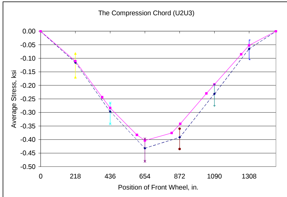
Fig. D.91: Field Test No. 2 - Average stress: Top chord (U2U3)
