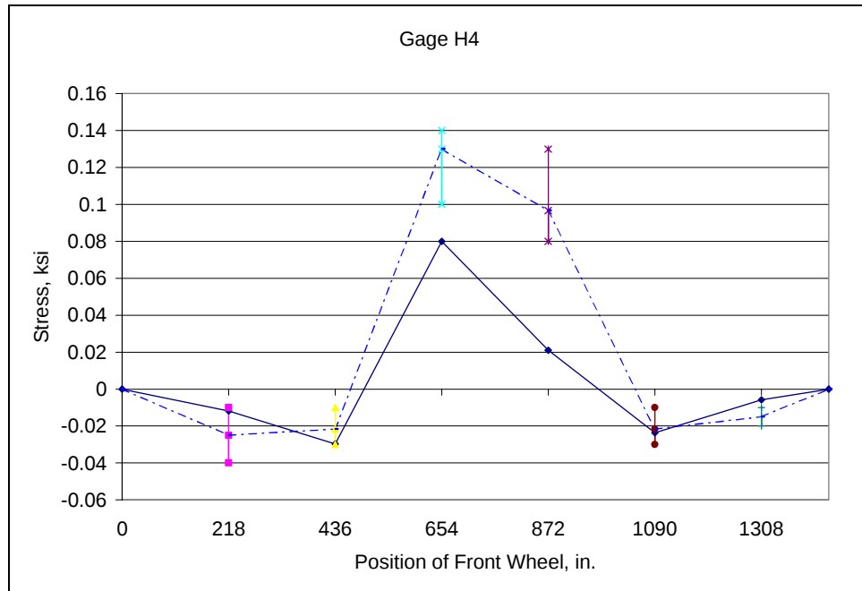
Fig. D.31: Field Test No. 1 - Member L3U3 of downstream truss
