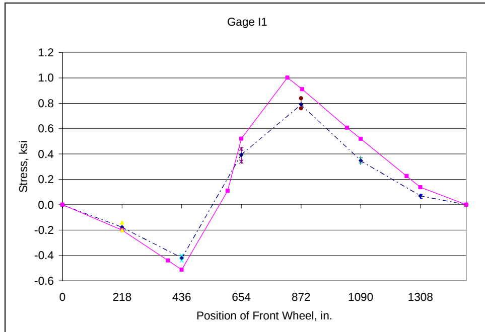
Fig. D.77: Field Test No. 2 - Diagonal member L3U2
