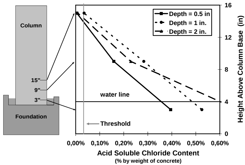
Figure B.6 Concrete Chloride Penetration for Column DJ-TC-S in Dripper Side at End of Testing 1
