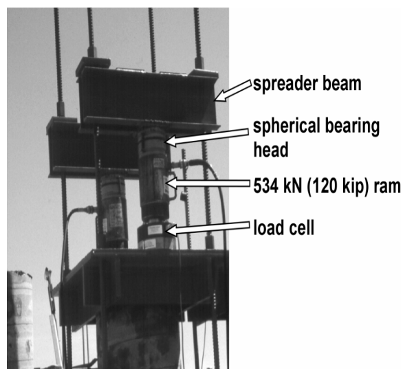
Figure 2.17 Loading System 2
