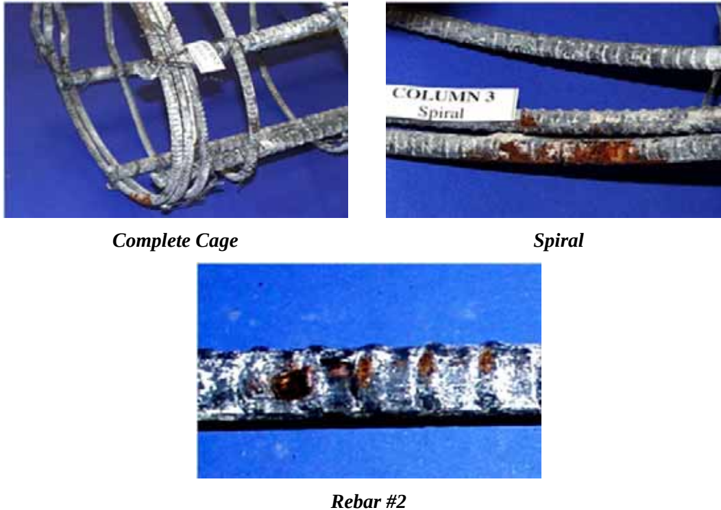
Figure 4.8 Reinforcement Condition for Specimen NJ-TC-N 1
