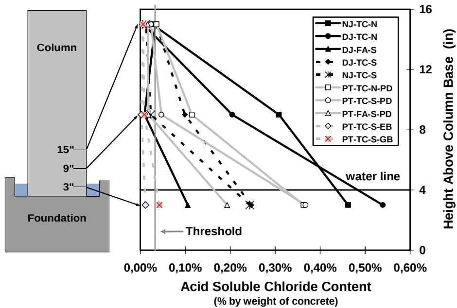
Figure 3.21 Concrete Chloride Penetration at 2.0 inches for All Columns in Non-Dripper Side at End of Testing 1
