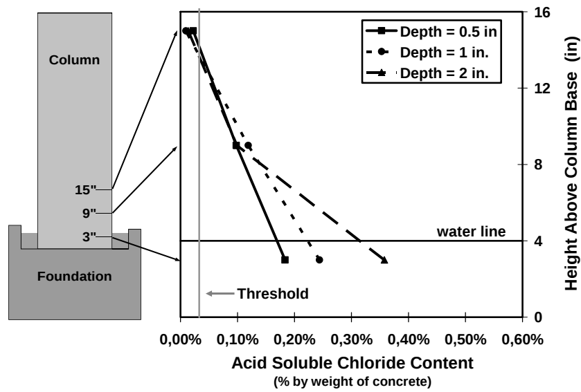
Figure B.14 Concrete Chloride Penetration for Column PT-TC-S-EB in Dripper Side at End of Testing 1
