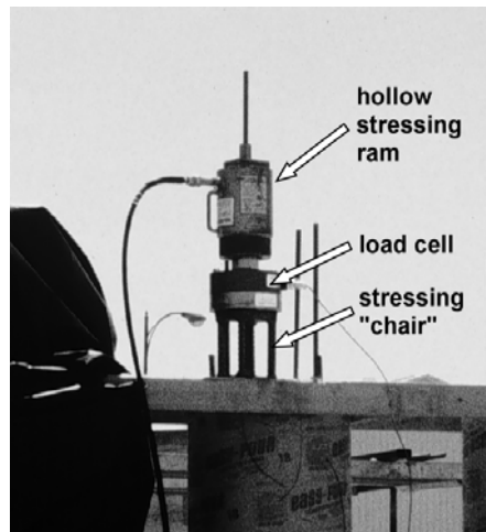
Figure 2.15 Column Post-Tensioning 2
