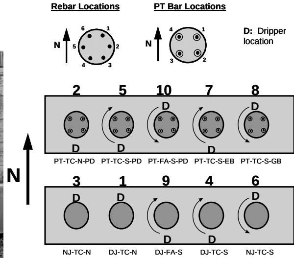
Figure 2.11 Specimen Location and Specimen Details 2
