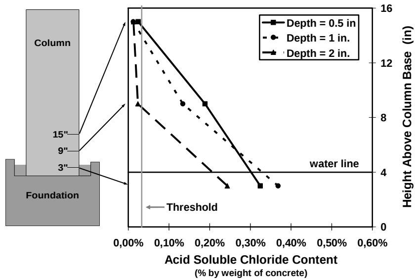
Figure B.7 Concrete Chloride Penetration for Column NJ-TC-S in Non-Dripper Side at End of Testing 1
