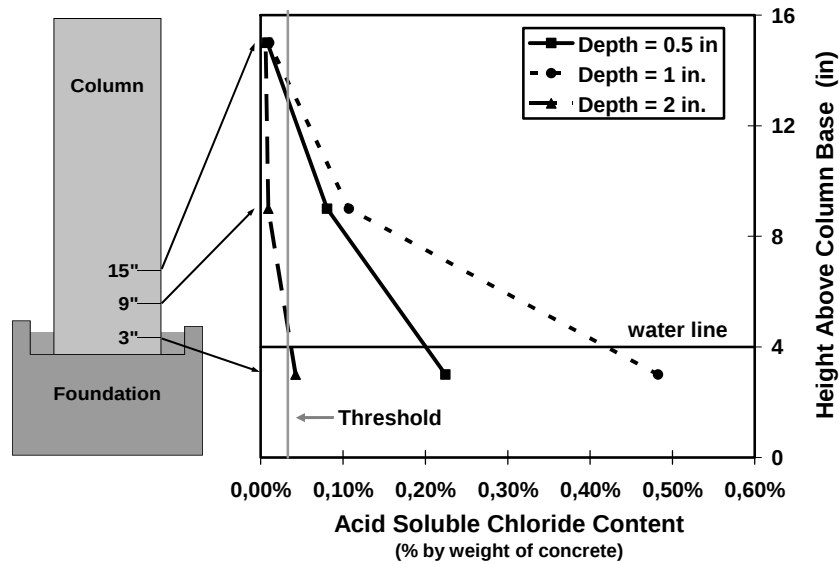
Figure B.15 Concrete Chloride Penetration for Column PT-TC-S-GB in Non-Dripper Side at End of Testing 1
