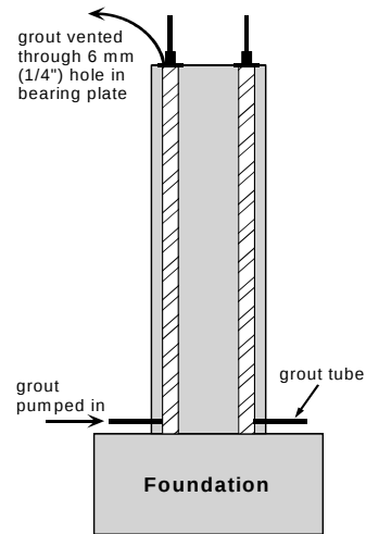
Figure 2.16 Inlet and Vent for Grouting 2
