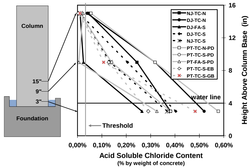
Figure 3.20 Concrete Chloride Penetration at 1.0 inch for All Columns in Non-Dripper Side at End of Testing 1
