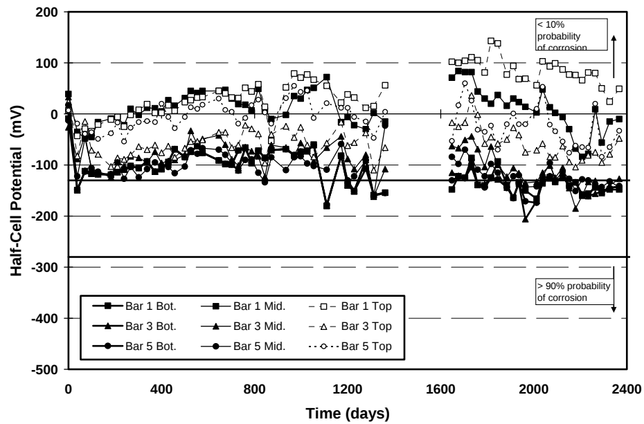
Figure A.2 All Half-Cell Potential Readings for Column DJ-TC-S¹
