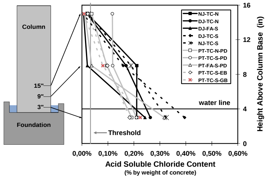
Figure 3.19 Concrete Chloride Penetration at 0.5 inches for All Columns in Non-Drifter Side at End of Testing 1
