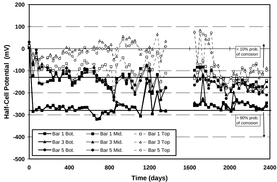
Figure 3.2 All Half-Cell Potential Readings: Column DJ-TC-N 1
