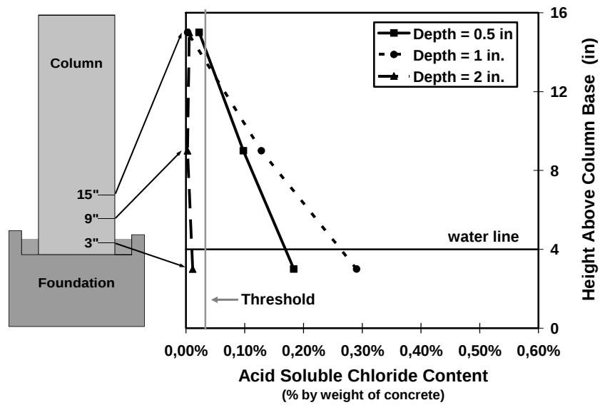
Figure B.13 Concrete Chloride Penetration for Column PT-TC-S-EB in Non-Dripper Side at End of Testing 1
