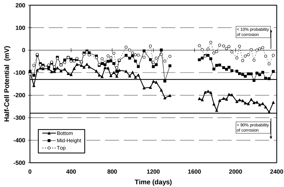
Figure A.3 All Half-Cell Potential Readings for Column PT-TC-S-PD – Rebar¹
