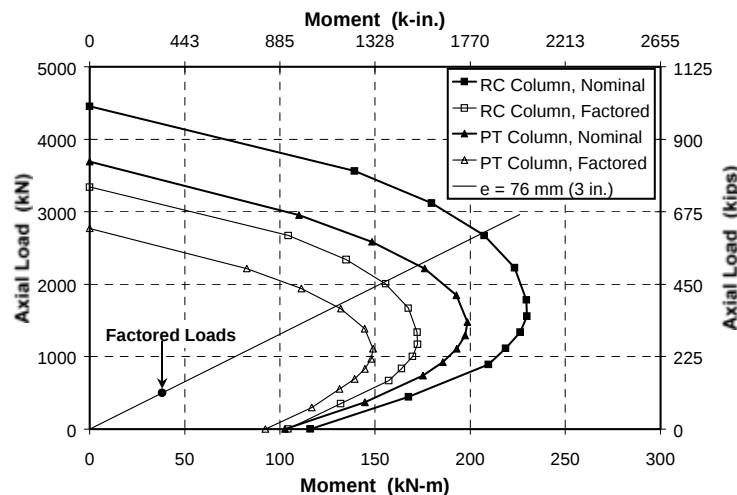
Figure 2.3 Column Interaction Diagrams 2
