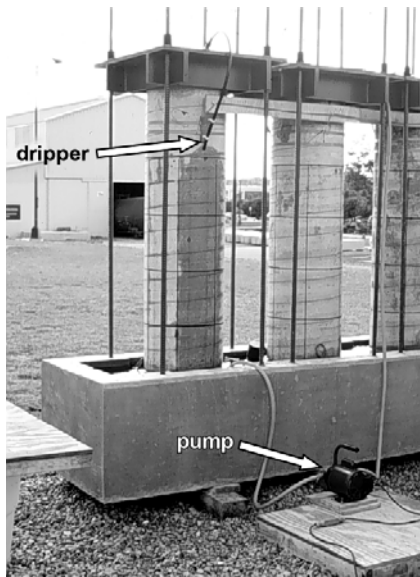
Figure 2.10 Column Drinker System 2
