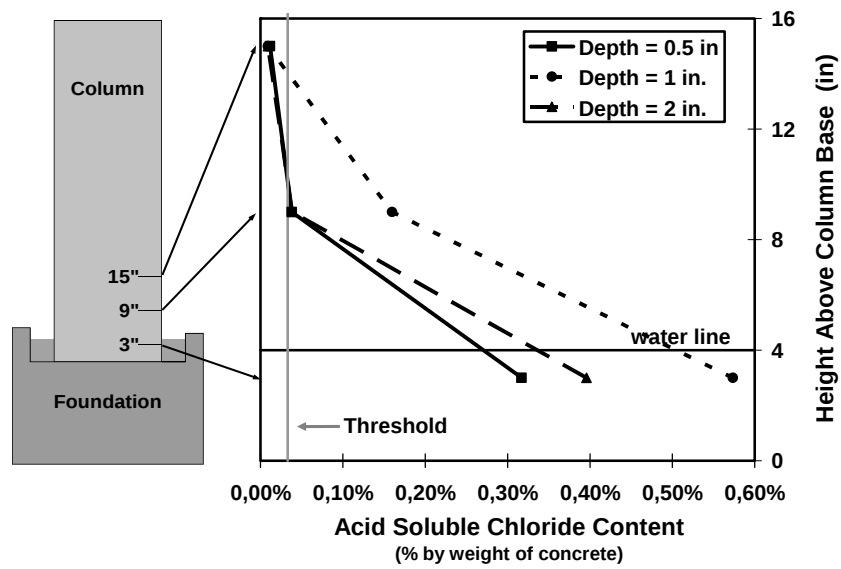
Figure B.12 Concrete Chloride Penetration for Column PT-FA-S-PD in Dripper Side at End of Testing 1
