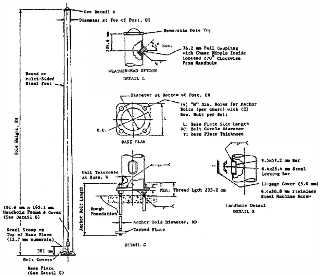
Figure 1.1 Typical signal pole supplied to NYSDOT
