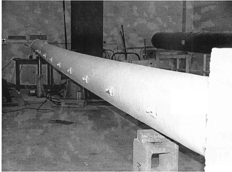
Figure 2.11 FRP pole deformed at 1 kips (4450 N)
