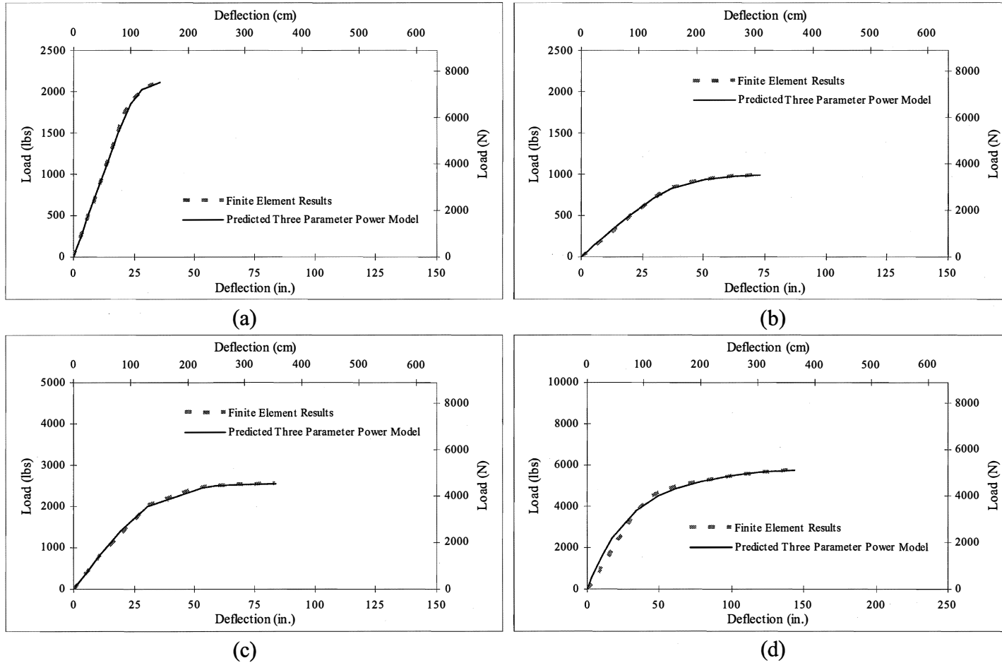
Figure B-4 Comparison of FEM model and predicted equation model for steel poles: (a) S30-1-0.15-0.15-1.25-11-6-3.25-40-15.5-15-50; (b) S30-1.25-0.15-0.15-1-7-4-2.75-45-10.5-10-40; (c) S35-1-0.2-0.2-1.25-11-7-3-40-15.5-17-70; (d) S35-1-0.3-0.3-1.75-12-6-3.75-50-18-17-100
