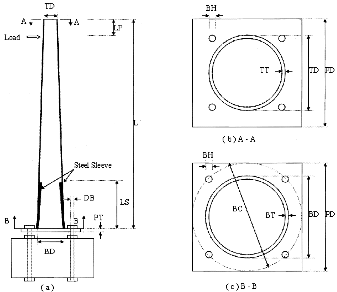
Figure 2.2 Typical dimensions of FRP poles tested:
