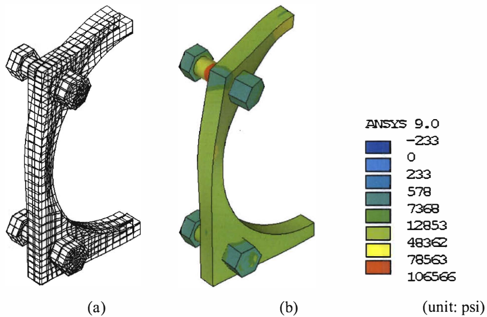
Figure 3.14 FEM results of FRP poles:
