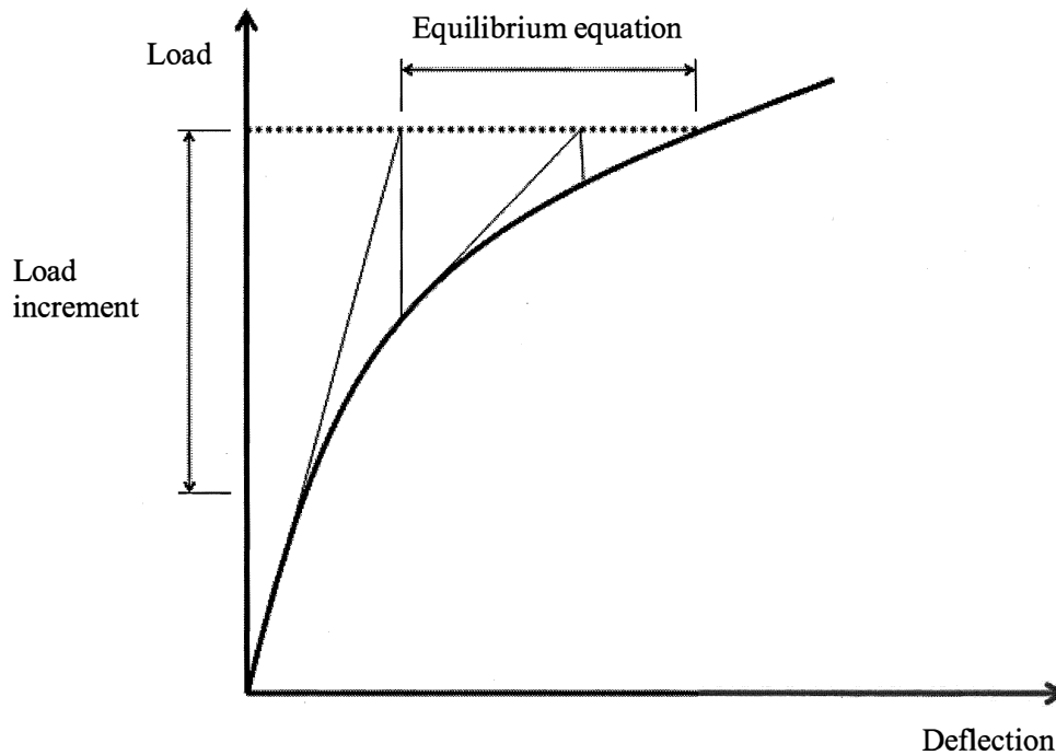
Figure 3.7 Newton-Raphson scheme
