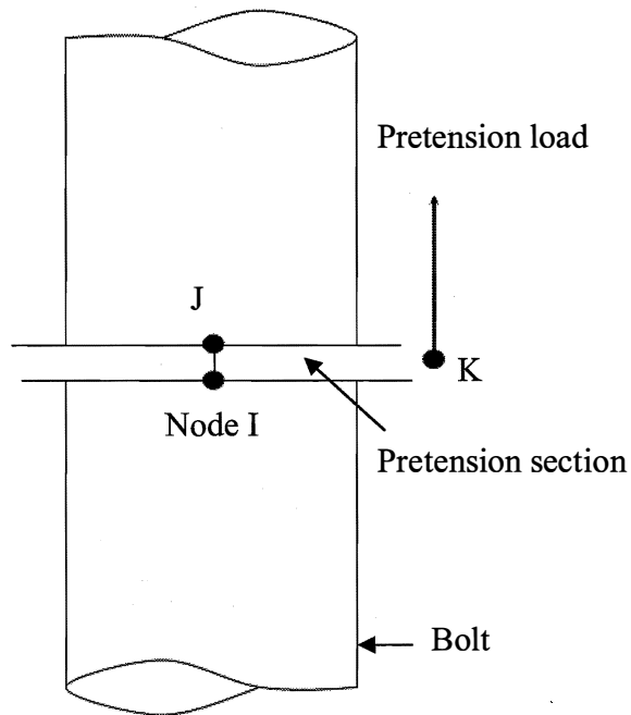
Figure 3.4 Pre-tensioning section
