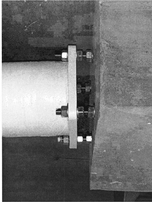
Figure 2.13 Bolt deformation at ultimate state
