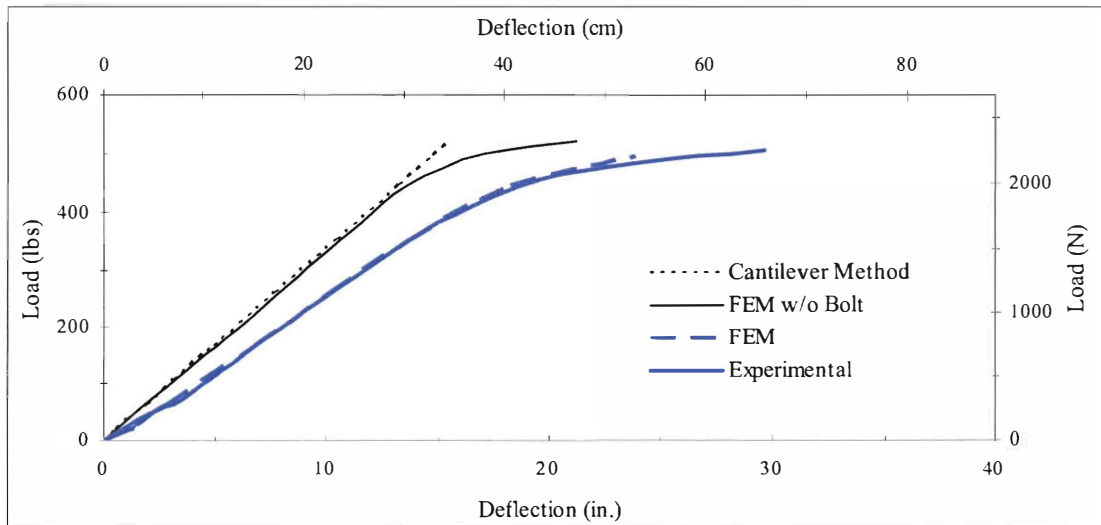
Figure 3.11 Deflection vs. load for steel poles
