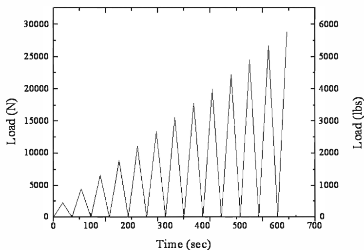
Figure 2.7 Loading history
