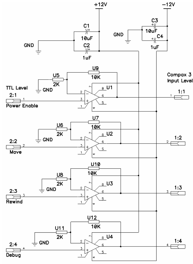
Figure 6-4. Interface Circuit.
