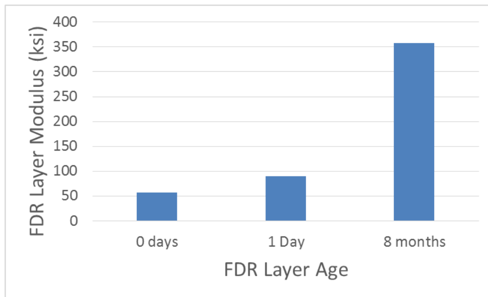
Figure 27. Growth of FDR Layer Modulus on SH 202.
