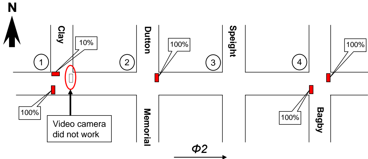
Figure 16. System Detectors and Detector Weights at the Waco Site.
