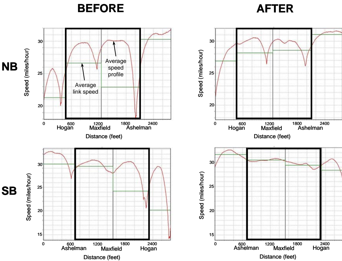
Figure 23. Average PM-Peak Delay and Speed Along the Spur 299 Route at the Bellmead Site Before and After Implementation of TRPS Mode.
