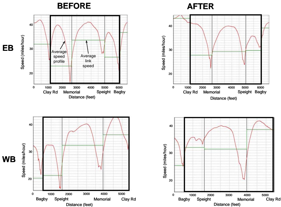
Figure 25. Average PM-Peak Delay and Speed at the Waco Site Before and After Implementation of TRPS Mode.
