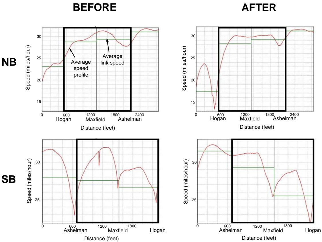
Figure 24. Average PM-Peak Delay and Speed Along the US 84 Route at the Bellmead Site Before and After Implementation of TRPS Mode.
