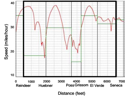
Figure 26. Average PM-Peak Delay and Speed at the San Antonio Site Before and After Implementation of TRPS Mode.
