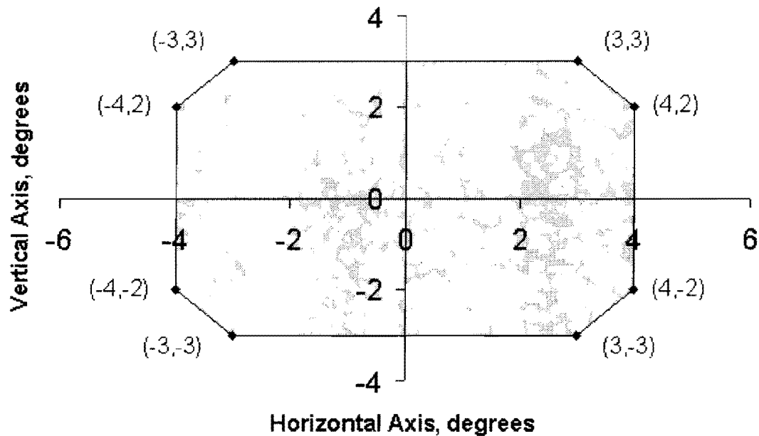
Figure 21. Angularity Requirements.
