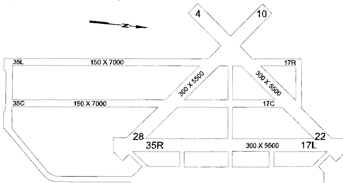
Figure 4. Runway Layout at Texas A&M University Riverside Campus.
