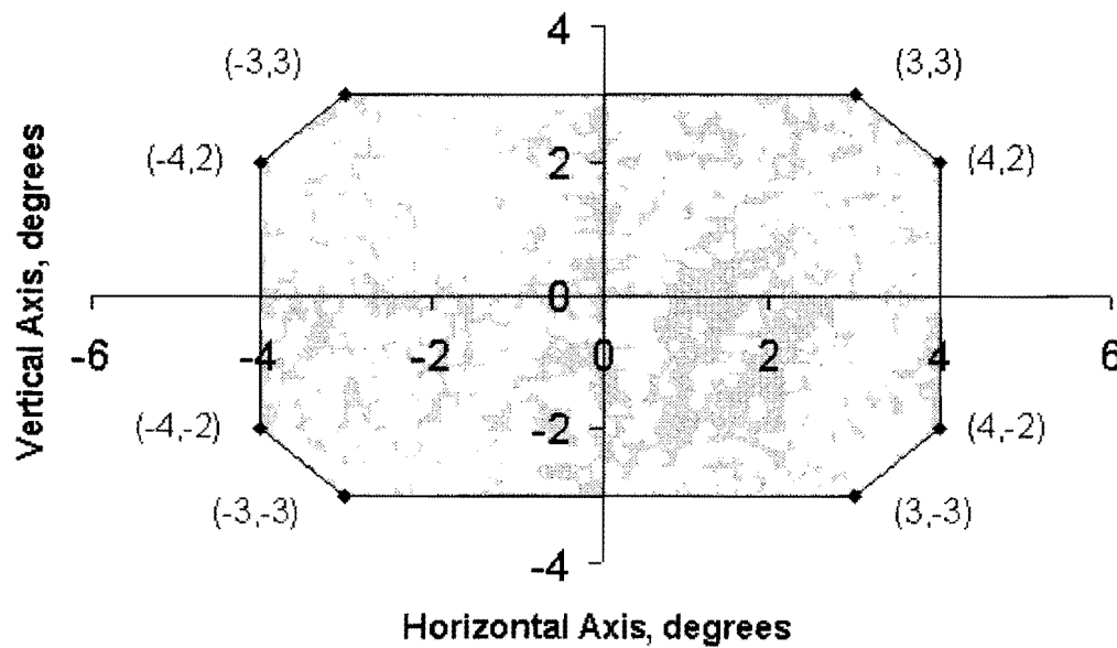
Figure 17. Minimum Angularity Requirements.
