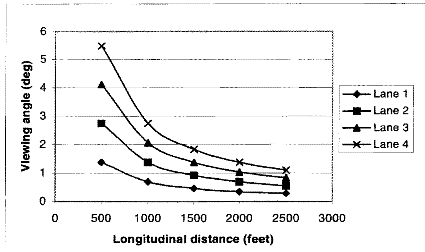
Figure 2. Change in Viewing Angle with Longitudinal Distance and Position of Car in Lane.
