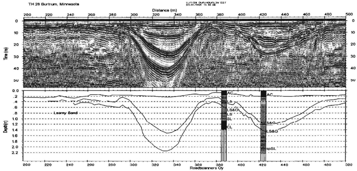
Figure 6. Using Road Doctor to Identify Varying Subgrade Conditions with Ground-Coupled GPR.
