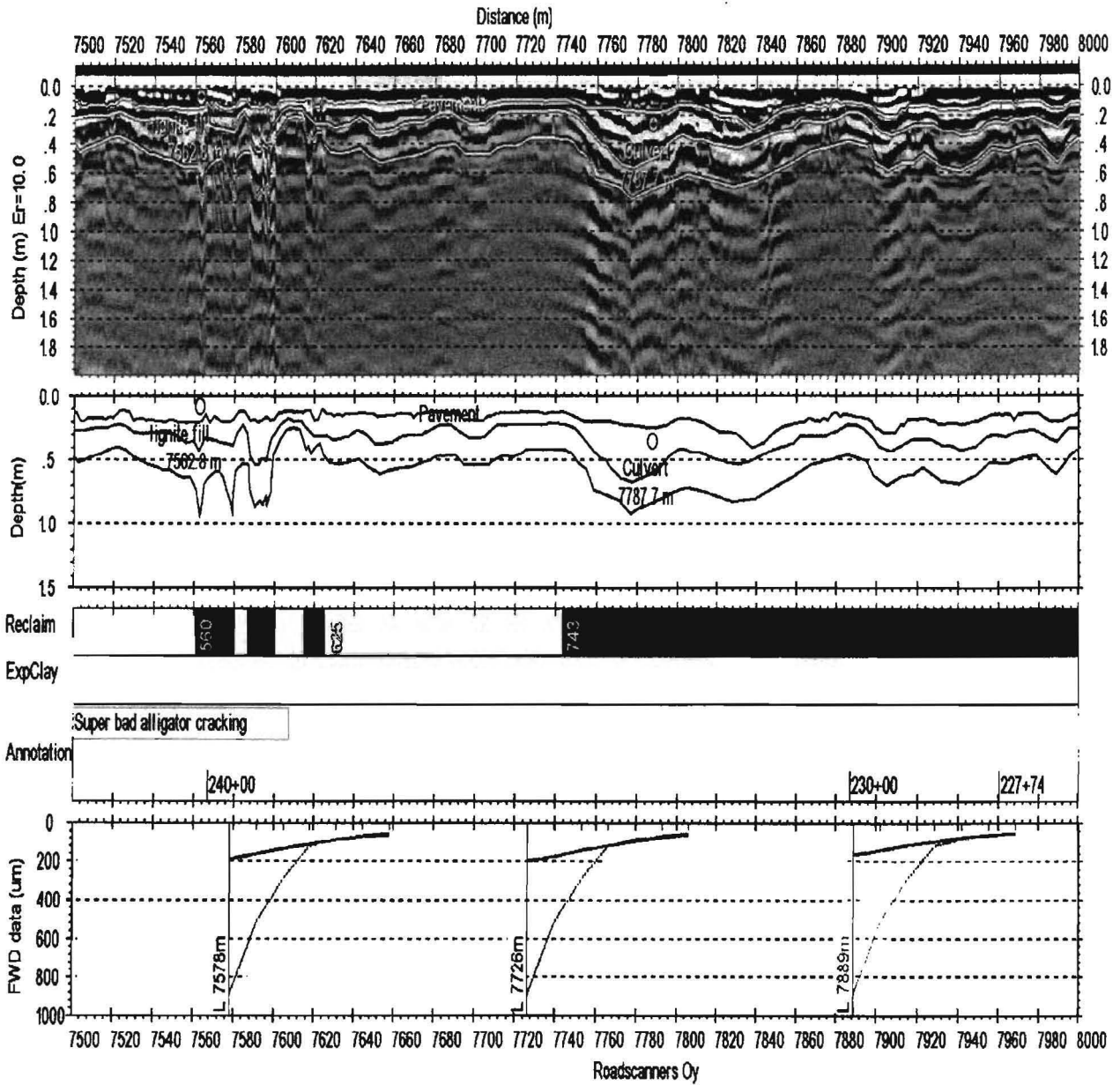
Figure 21. GPR Data from Badly Distressed Areas on FM 488. The Reclaimed Land Has a Distinctive Strong Repeating Reflections with Depth.
