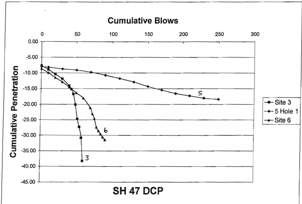
Figure 16. Validation Dynamic Cone (DCP) Data from SH 47 Showing Highly Variable Strengths for the Lime-Stabilized Layer. The DCP Results for Location 5 Are Judged To Be Ideal. However at Location 3 No Effective Lime Layer Was Present.
