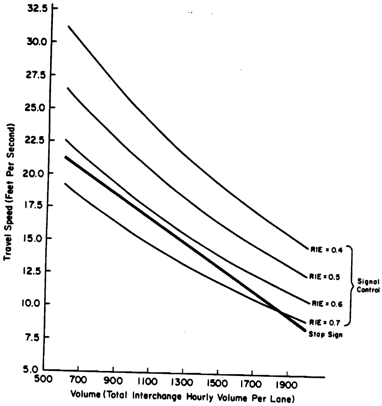
Figure 5. Travel Speed Versus Volume for Arterial Through Traffic by Stop Sign and Signal Control.
