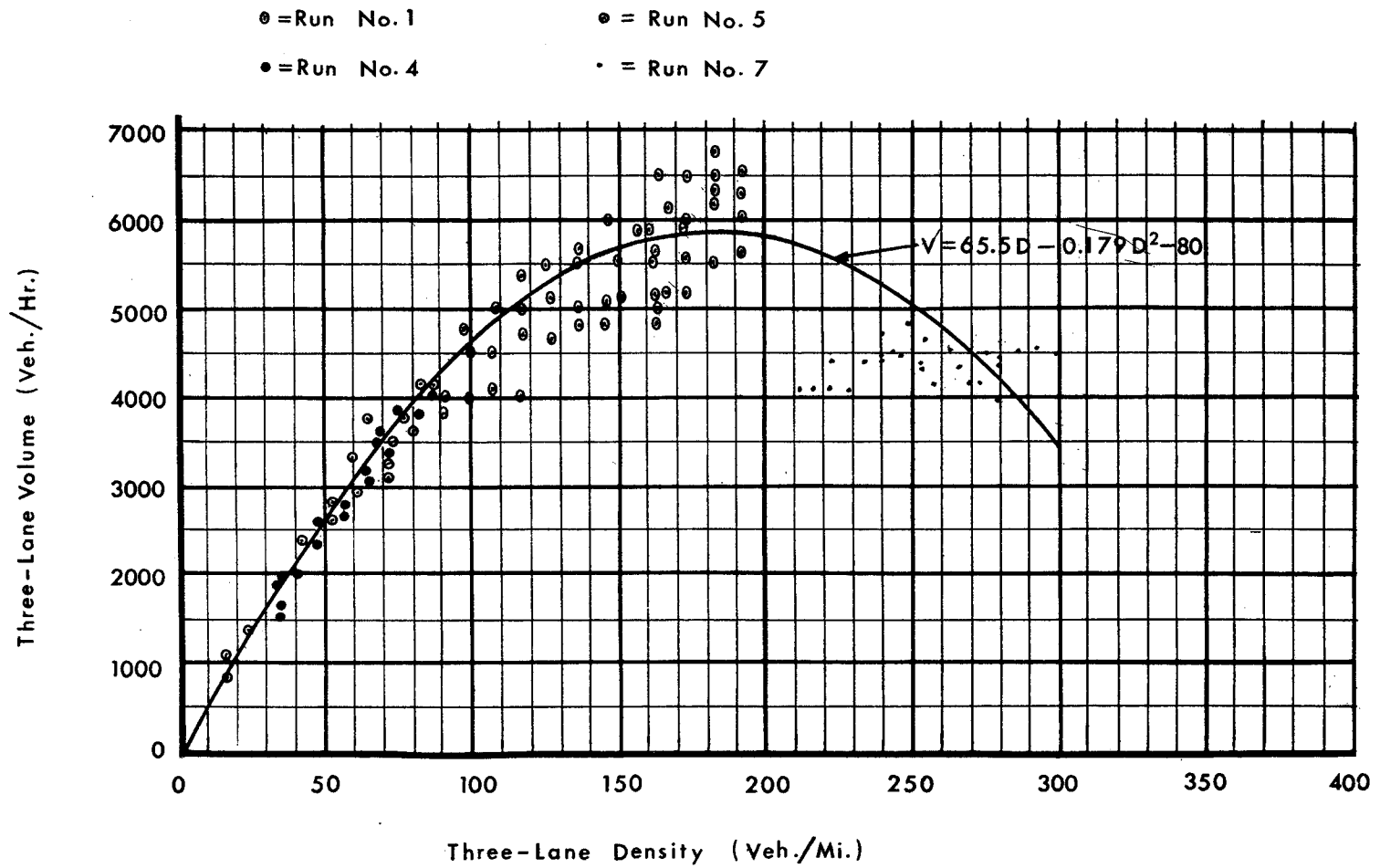
Figure 15. Volume-Density Relationship Obtained From Density Trap Studies
