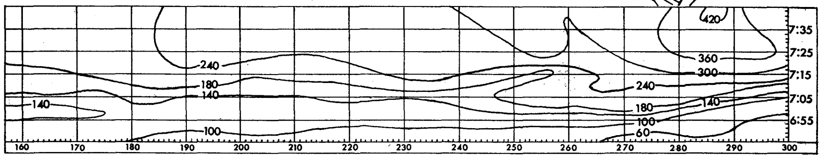
Figure 17. Density Contours (Three-Lane Total)
