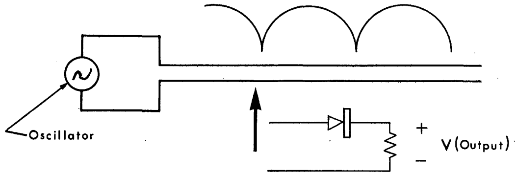
Figure 5. Transmission Line Circuitry Scheme
