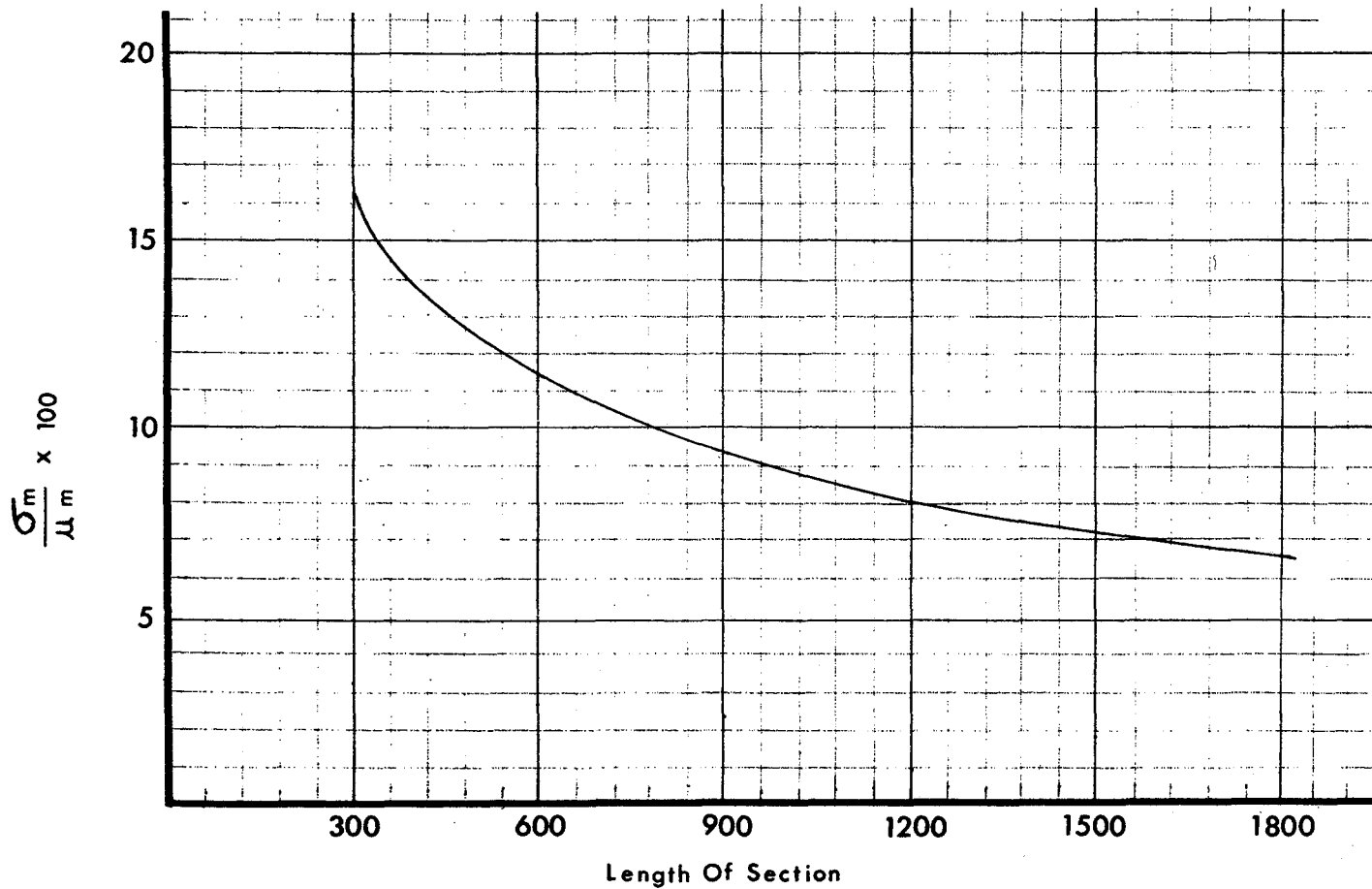
Figure 18. Relationship Between the Standard Deviation Percent of the Mean Concentration and the Length of Sensing Section at High Volumes
