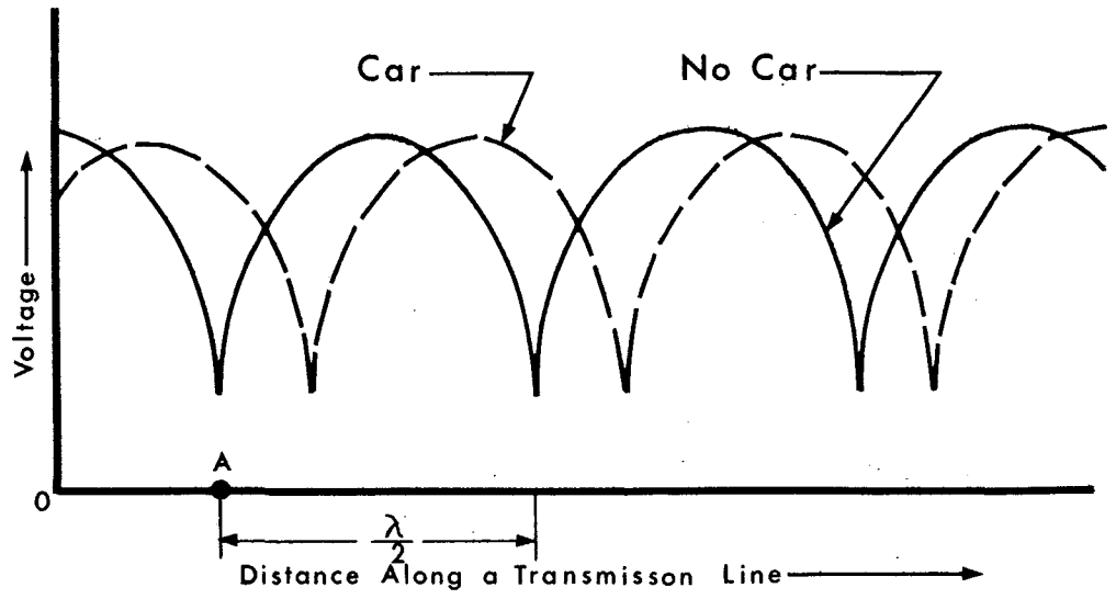
Figure 4. Standing Wave Variation Along a Transmission Line
