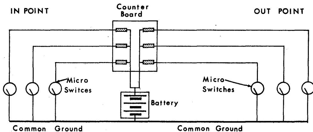
Figure 10. Wiring Scheme for Density Trap Apparatus
