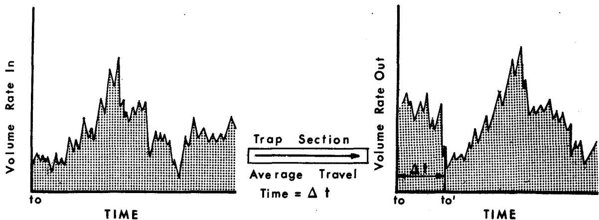
Figure 14. Volume Rates In and Out of a Density Trap
