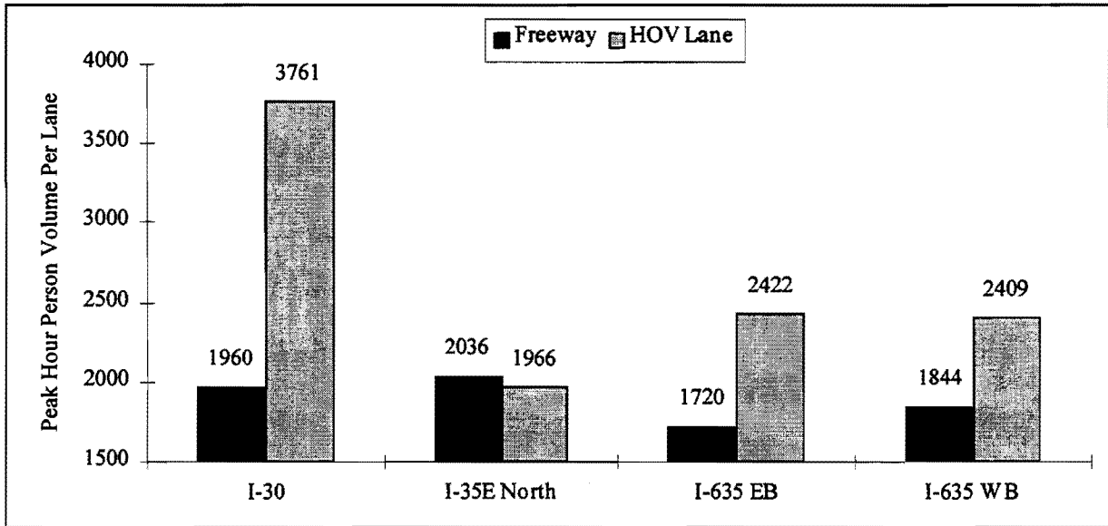
Figure 9. Peak Hour Person Volume per Lane
