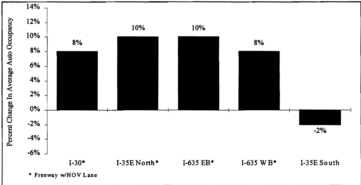
Figure 12. Percent Change in Average Automobile Occupancy
