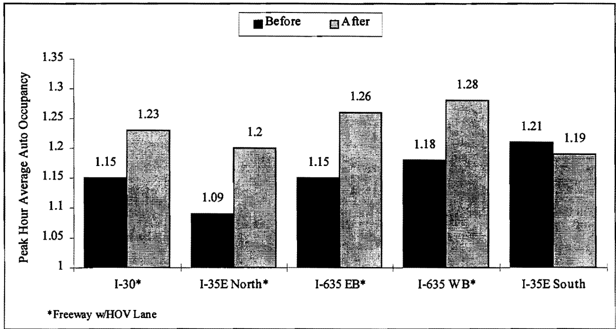
Figure 10. Changes in Average Automobile Occupancy
