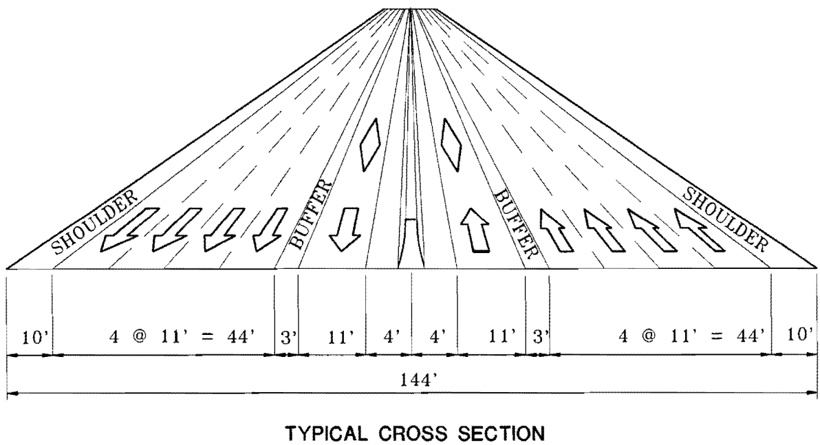
Figure 4. I-635 Lyndon B. Johnson Freeway HOV Lane
