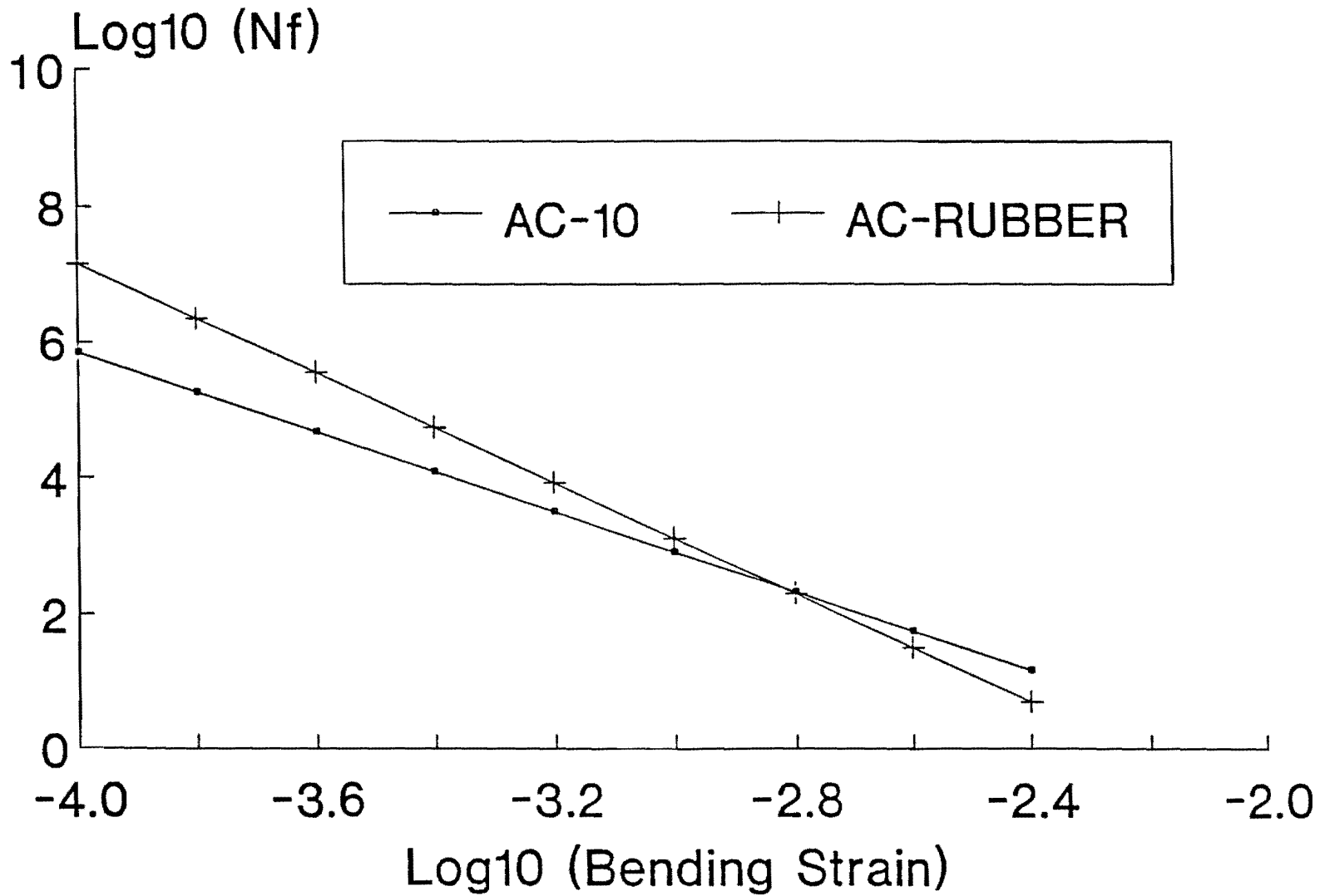
Figure C2. Fatigue Relationship at 34°F for AC-10 and Rubber-Modified Asphalt Mixtures.
