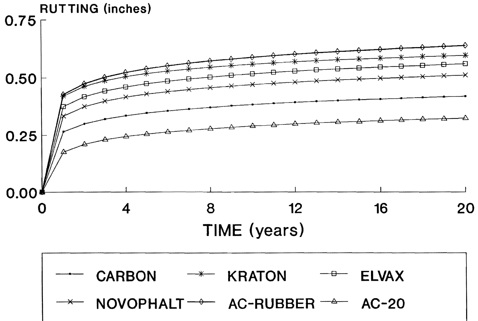
Figure 14. Rut-Depth Predictions for San Joaquin Valley and Rubber-Modified Asphalt Mixtures.
