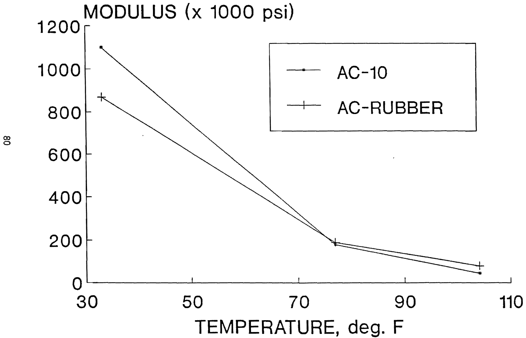
Figure C1. Variation of Diametral Resilient Modulus with Temperature for AC-10 and Rubber-Modified Asphalt Mixtures.
