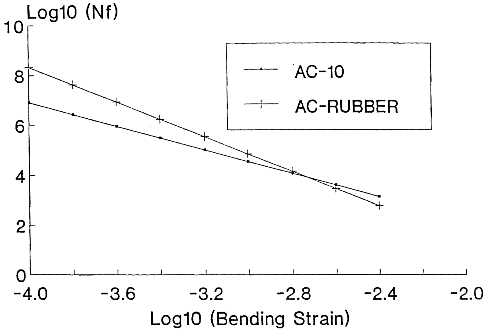
Figure C4. Fatigue Relationships at 104°F for AC-10 and Rubber-Modified Asphalt Mixtures.
