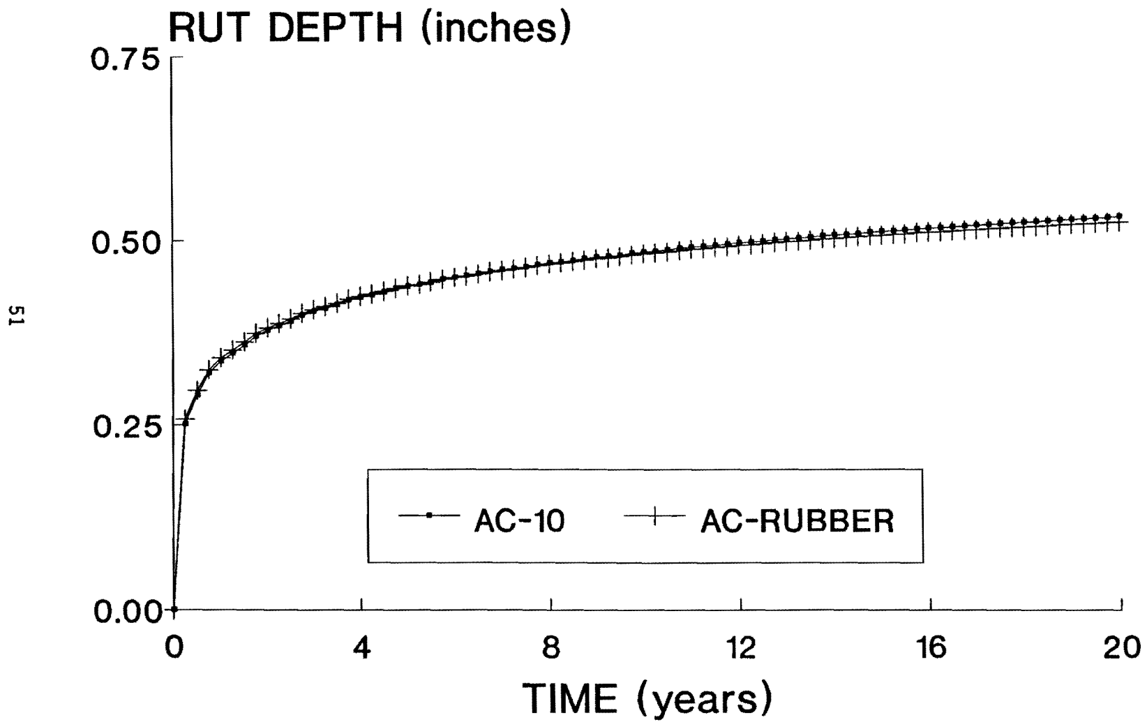
Figure 12. Comparison of Rut Depth Prediction for AC-10 and Asphalt-Rubber Concrete Mixtures.
