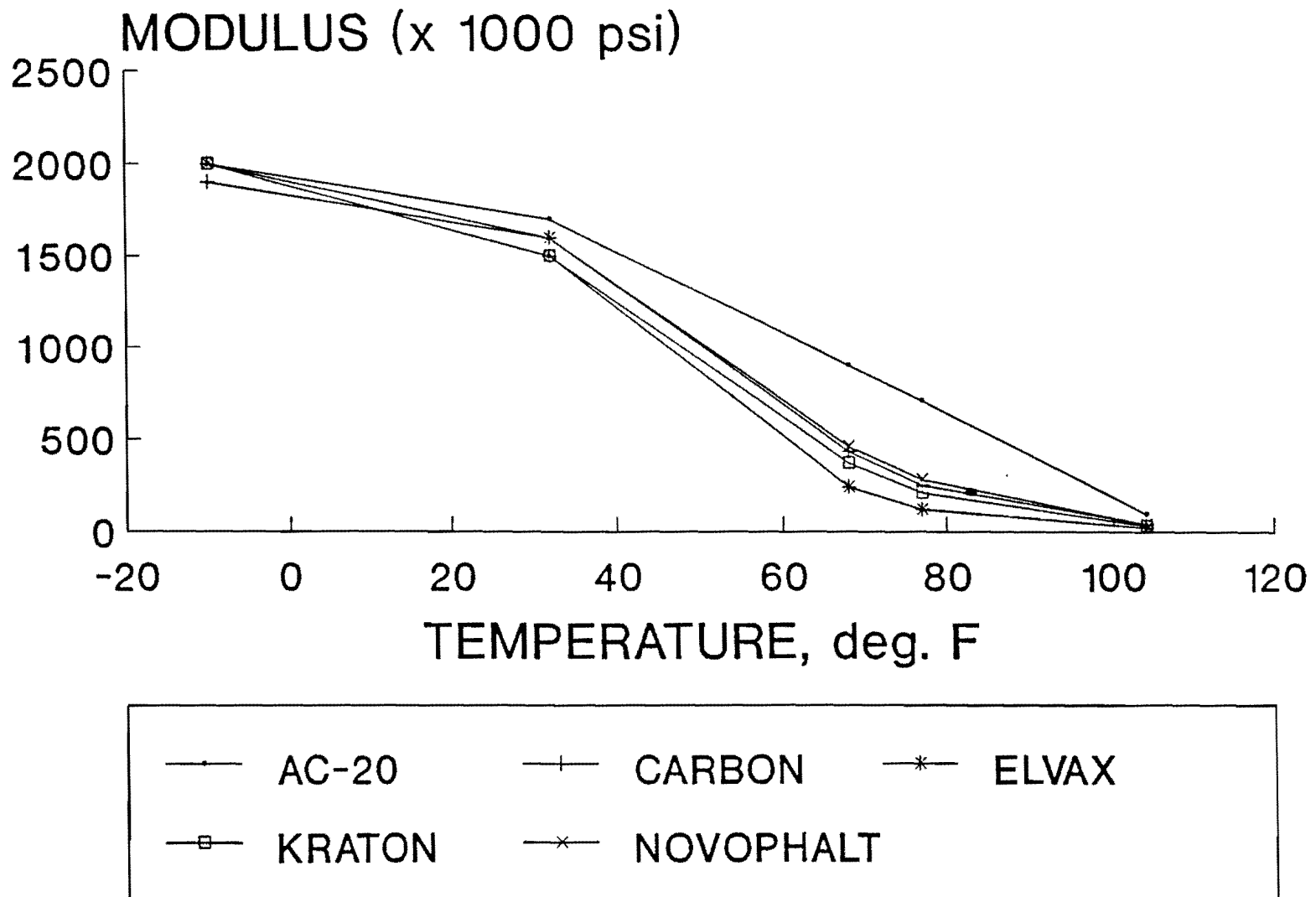
Figure C5. Variation of Diametral Resilient Modulus with Temperature for San Joaquin Valley Asphalt Mixtures.
