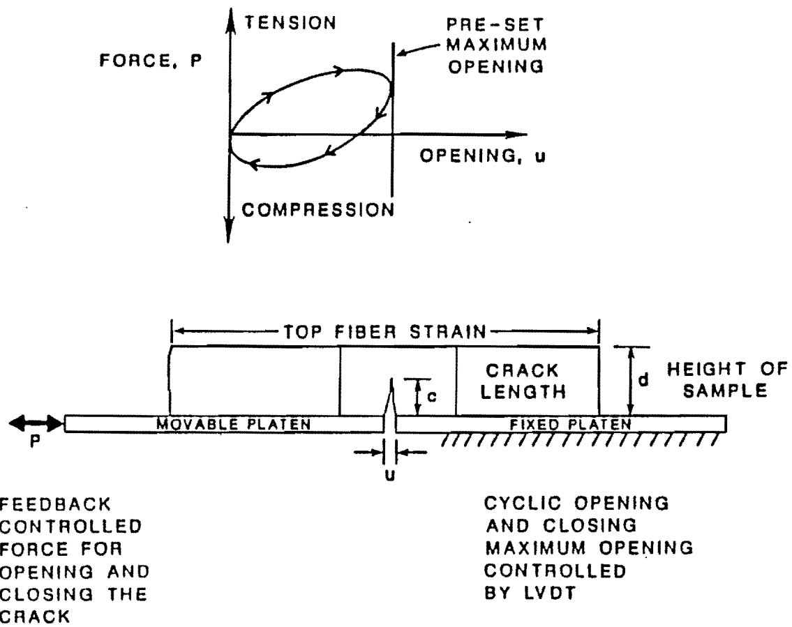
Figure C6. Schematic Diagram of Overlay Tester.
