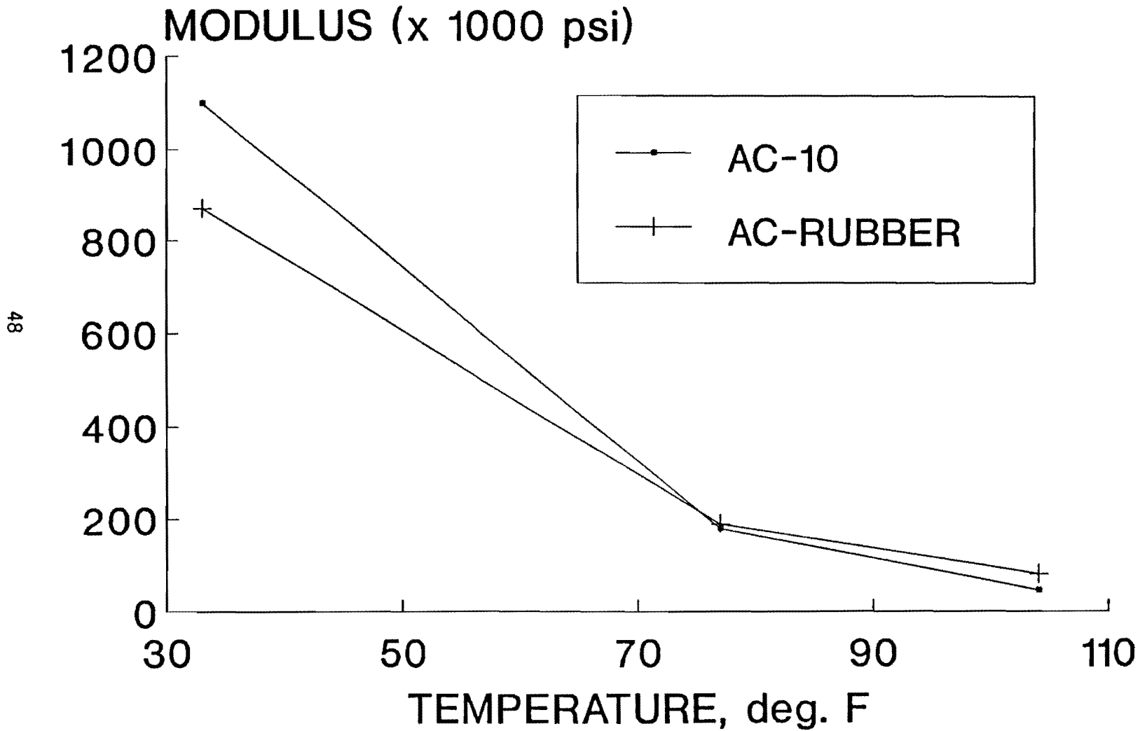
Figure 10. Variation of Diametral Resilient Modulus with Temperature for AC-10 and Asphalt-Rubber Concrete Mixtures.
