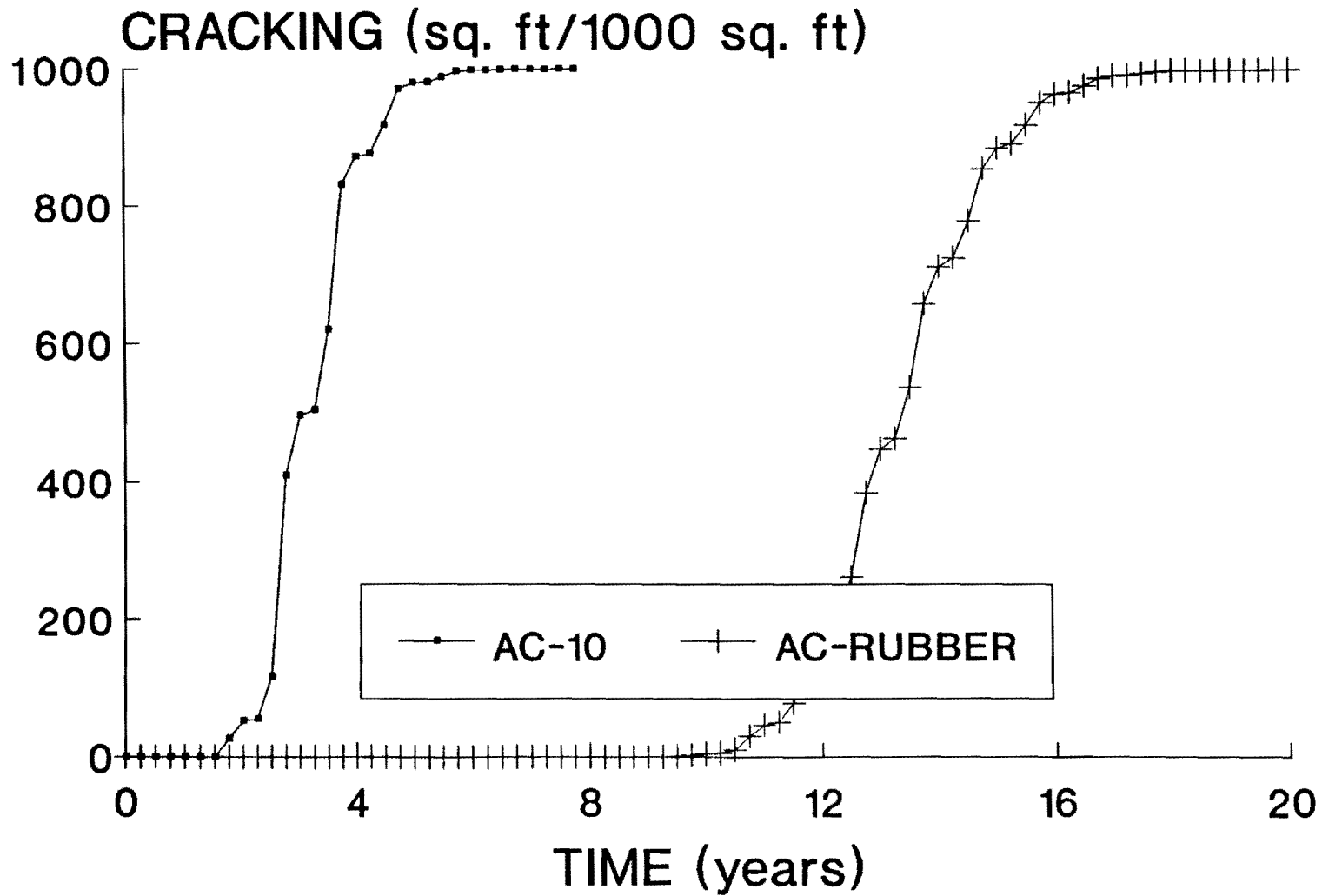
Figure 11. Comparison of Fatigue Performance of AC-10 and Asphalt-Rubber Concrete Mixtures.
