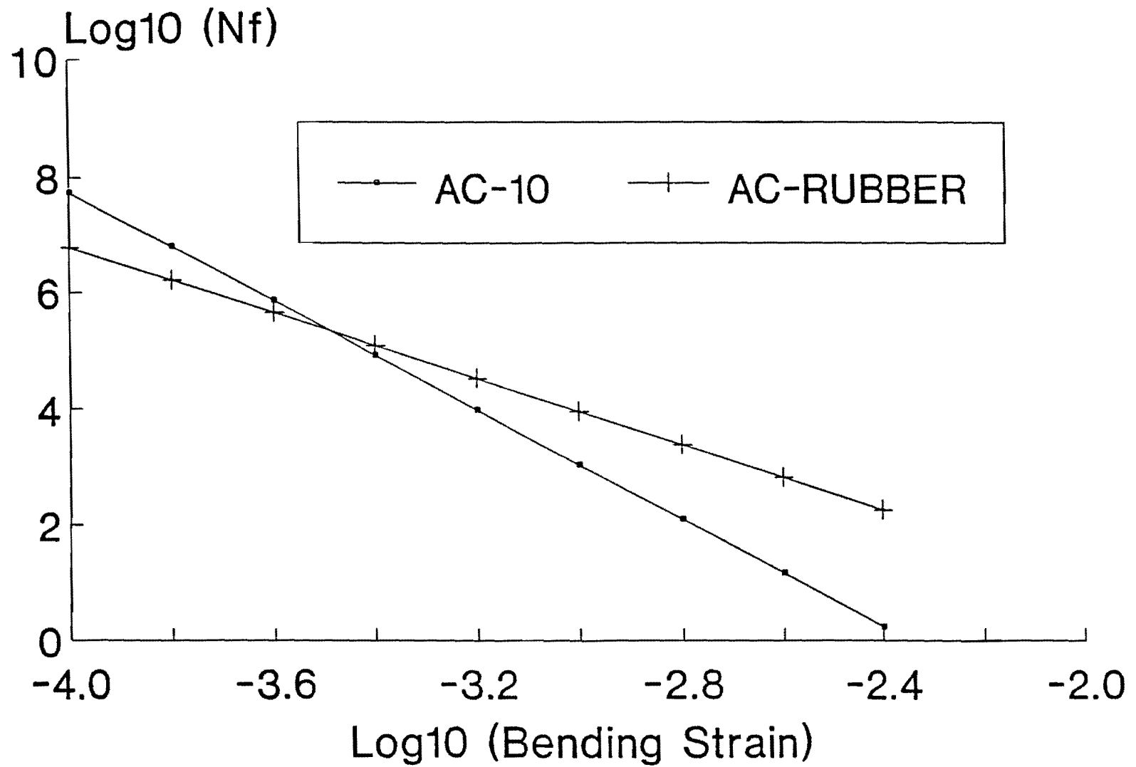
Figure C3. Fatigue Relationships at 68°F for AC-10 and Rubber-Modified Asphalt Mixtures.
