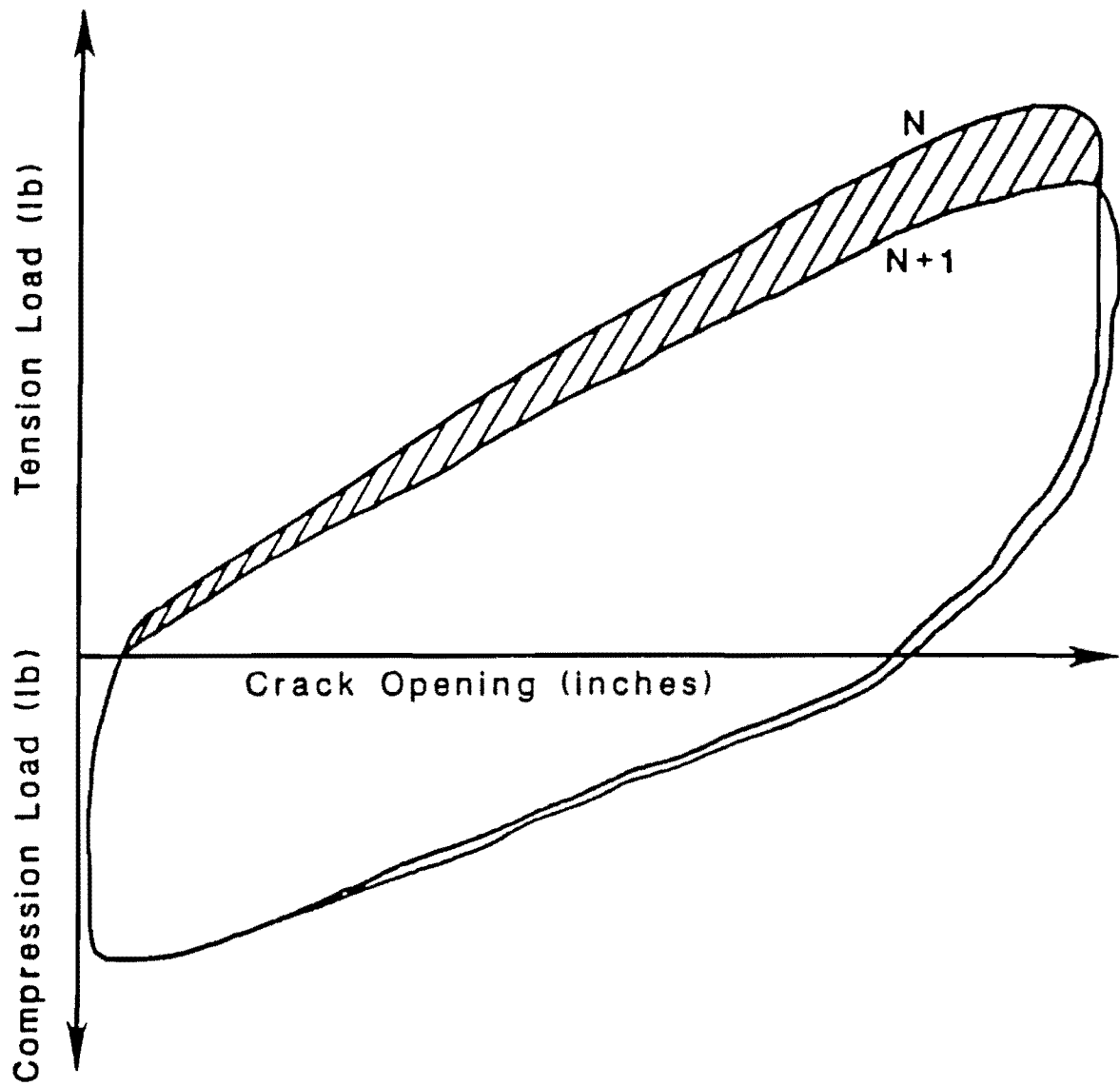
Figure C7. Typical Recording of Load Versus Crack Opening from Overlay Tester.
