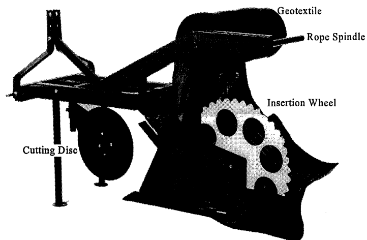
Figure 7. Tommy® Silt Fence Machine Source: Manufacturer's Brochure
