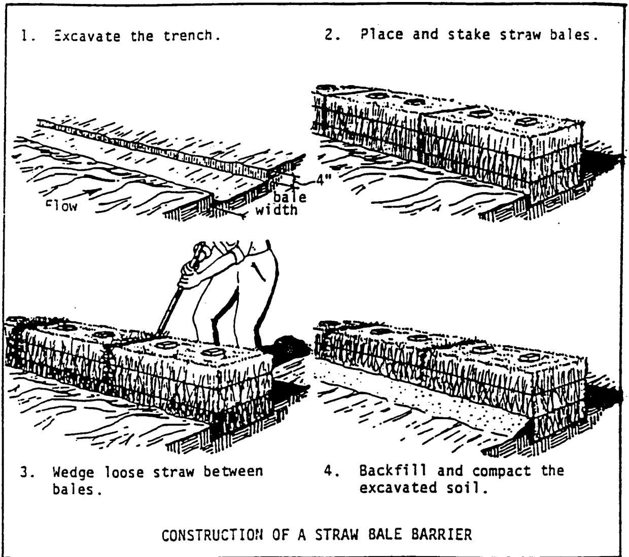
Figure II-5.20 Proper Installation of a Straw Bale Barrier
