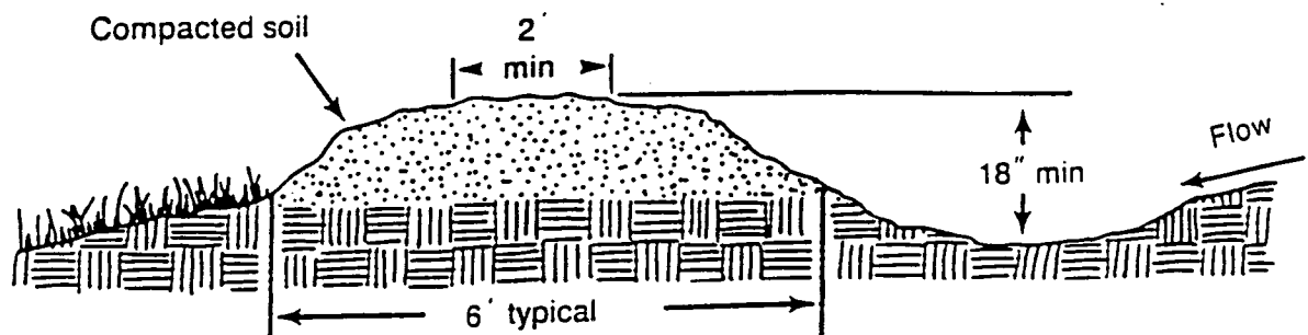
Figure 6.20a Temporary earthen diversion dike. Temporary Erosion Control Final Report
