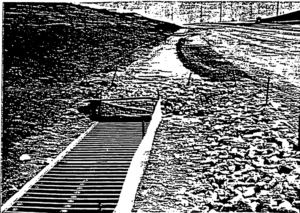
Figure 5.6 - A rock filter dam used in conjunction with a sediment control fence as inlet protection.
