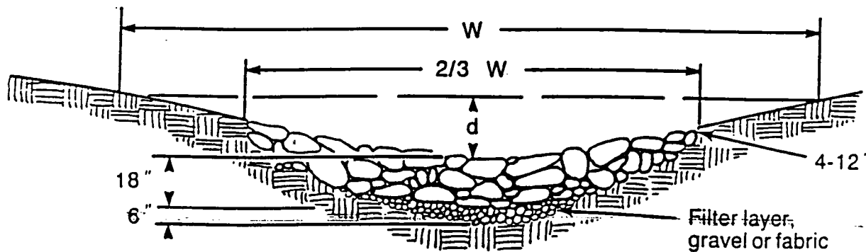
Figure 6.31a Construction detail of riprap channel cross sections.
