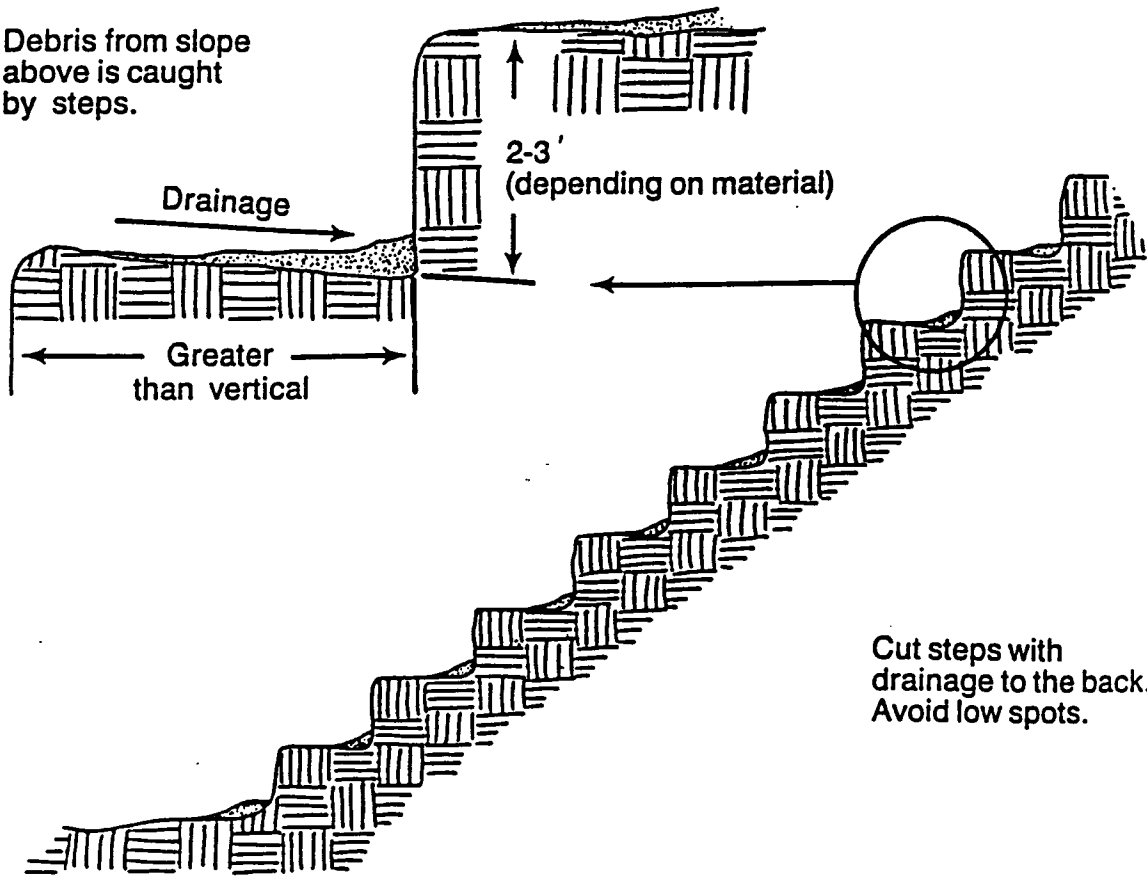
Figure 6.03b Stair stepping cut slopes (modified from Va SWCC).
