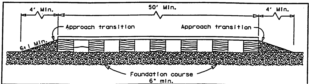
Figure 5.16 - Typical timber plank construction exit.
