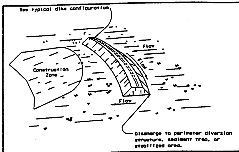
Figure 5.2 - Typical Interceptor Dike
