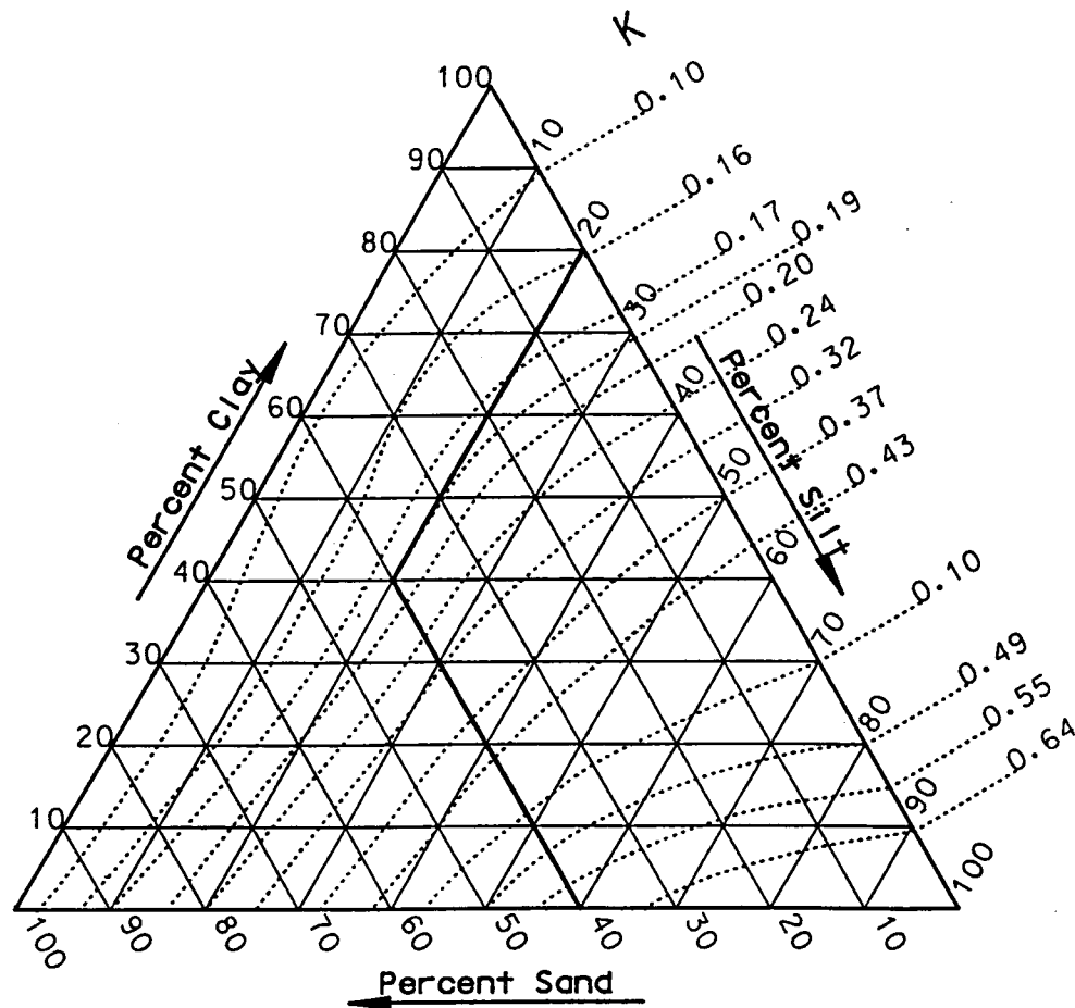
Figure 1. Nomograph for Estimating "K" Values
