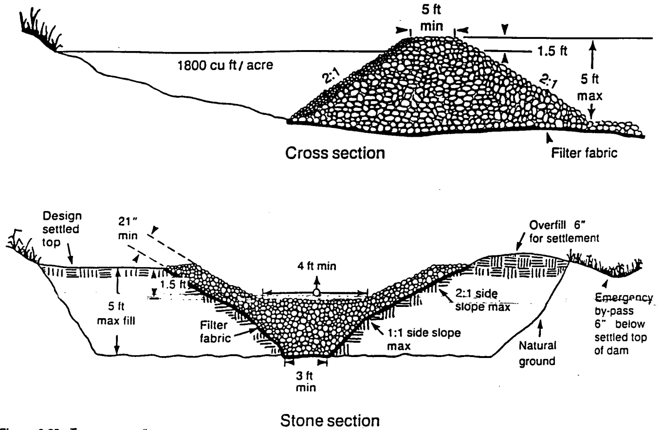
Figure 6.60a Temporary sediment trap.
