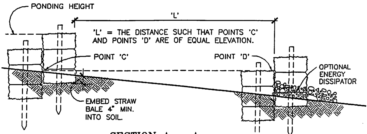
SECTION A - A SPACING BETWEEN CHECK DAMS
