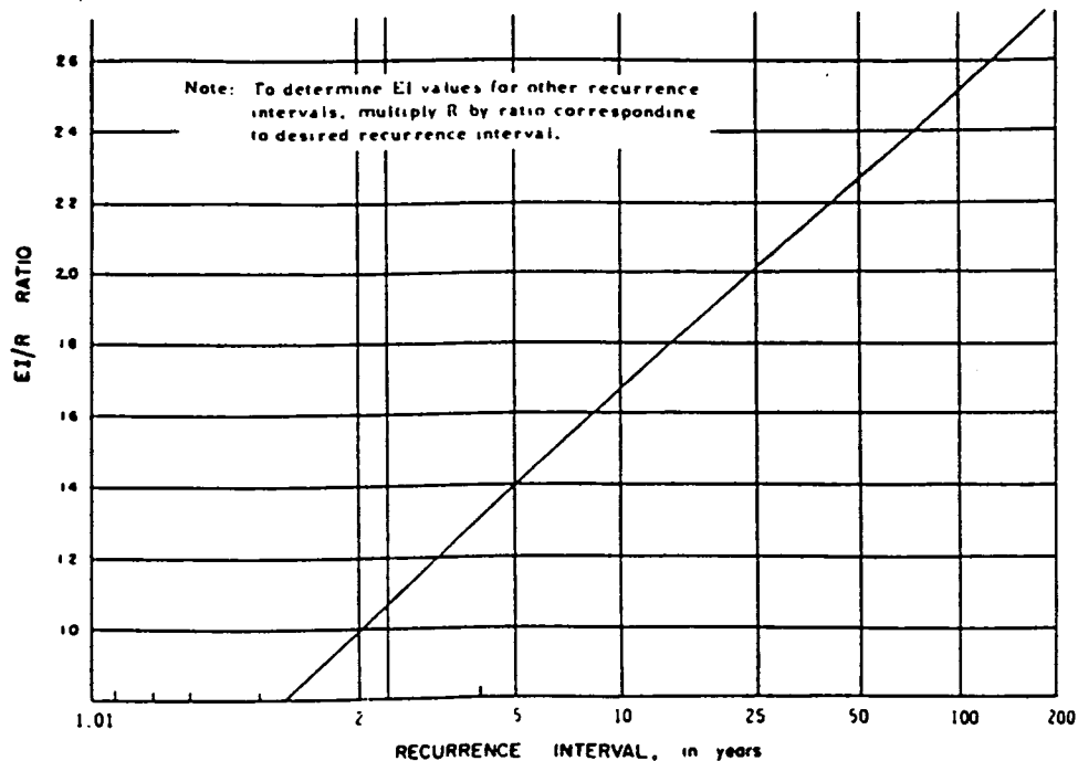
Figure 3.1 - Relationship between EI/R ratio and recurrence interval.
