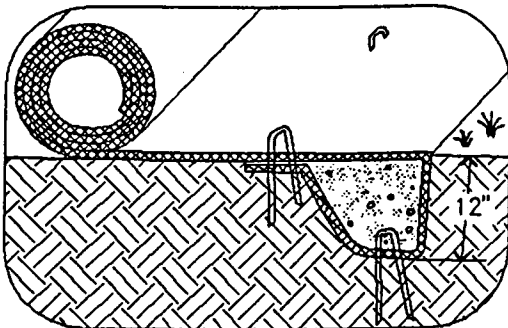
INITIAL CHANNEL ANCHOR TRENCH
