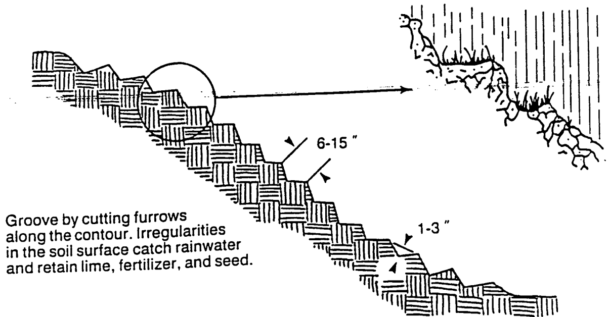
Figure 6.03c Grooving slopes (modified from Va SWCC).
