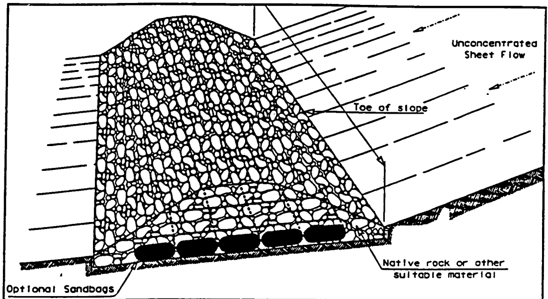
Figure 5.4 - Typical rock filter dam at toe of slope.
