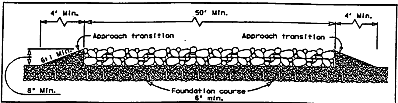
Figure 5.15 - Typical stone construction exit.
