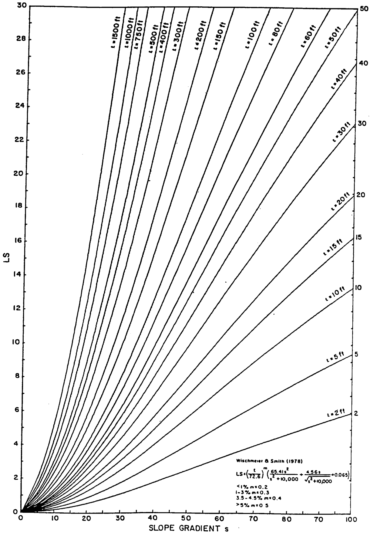
Figure 3.2 - Graphical Solution for Length Slope Factor
