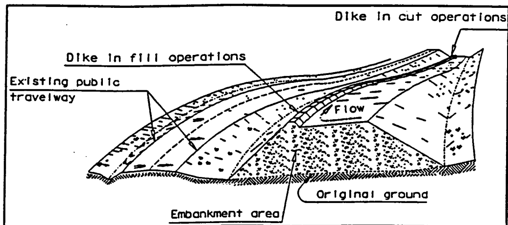
Figure 5.1 - Typical Diversion Dike installation
