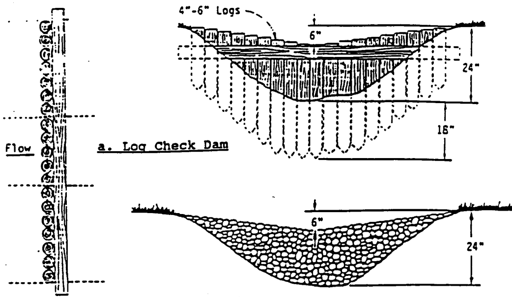
Figure II-5.14 Check Dams
