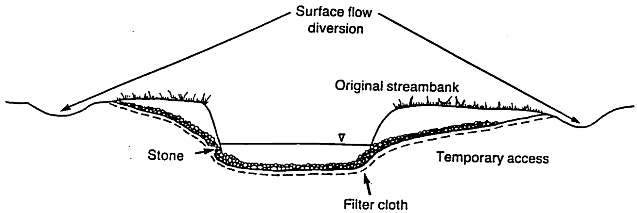
Figure 6.70a A well constructed ford offers little obstruction to flow while safely handling heavy loadings.
