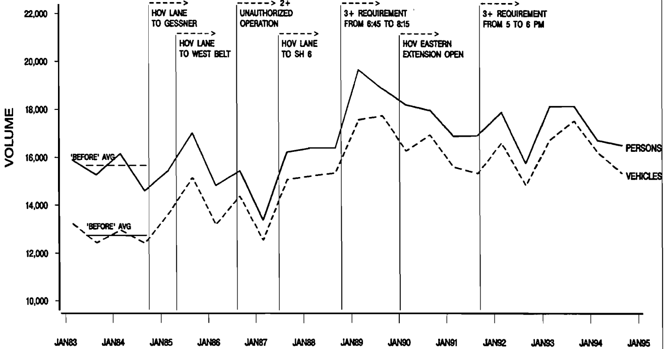
FIGURE A-10. KATY FREEWAY (IH 10W) MAINLANE AND HOV LANE A.M. PEAK HOUR AVERAGE OCCUPANCY
