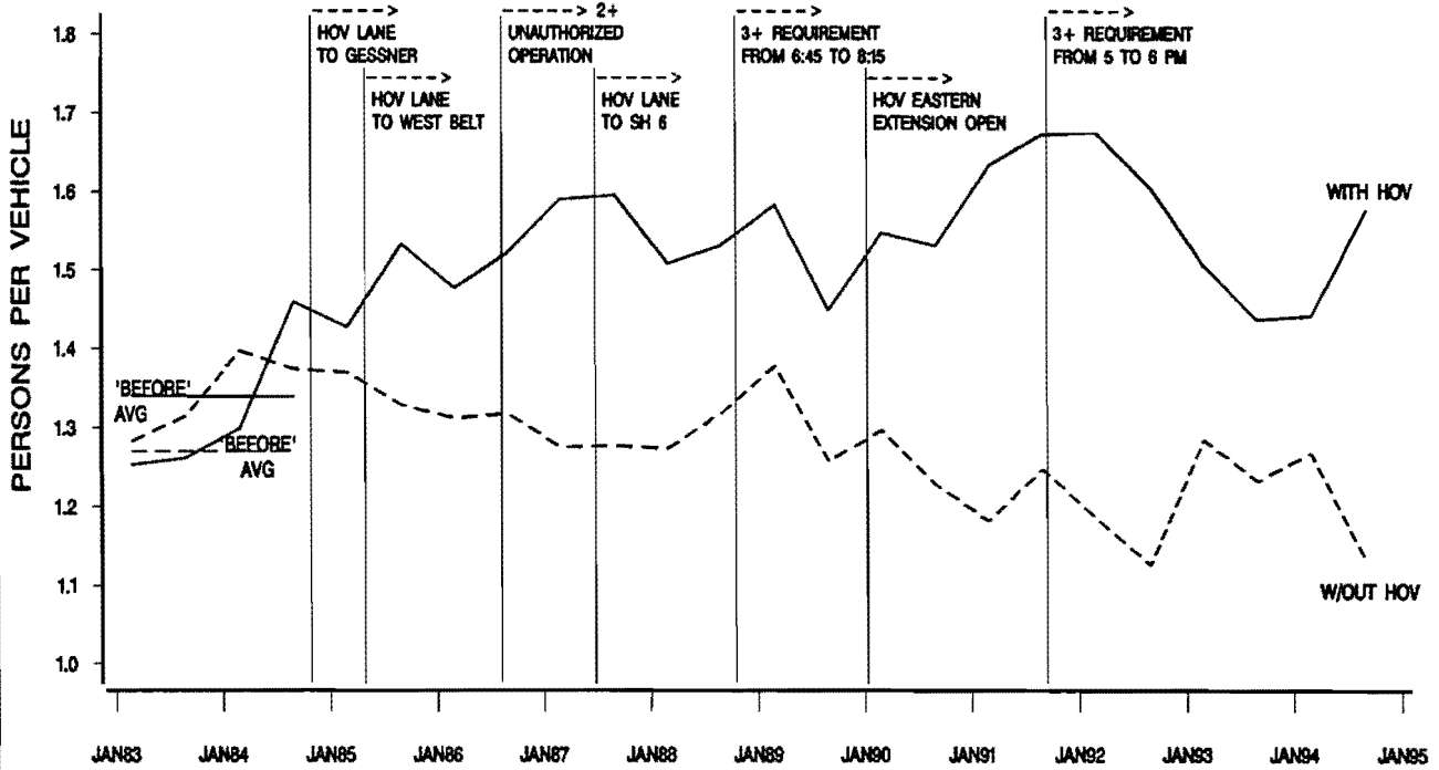
FIGURE A-14. KATY FREEWAY (IH 10W) MAINLANE AND HOV LANE A.M. PEAK HOUR 2+ CARPOOL UTILIZATION
