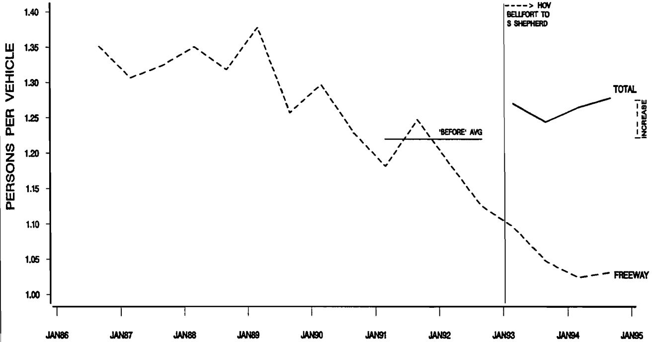
FIGURE E-12. SOUTHWEST FREEWAY (U.S. 59S) MAINLANE AND HOV LANE A.M. PEAK PERIOD AVERAGE OCCUPANCY
