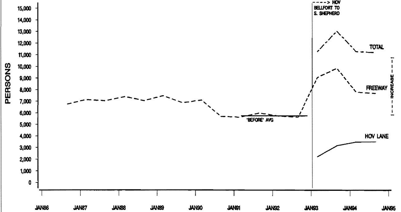
FIGURE E-10. SOUTHWEST FREEWAY (U.S. 59S) MAINLANE AND HOV LANE A.M. PEAK PERIOD PERSON TRIPS
