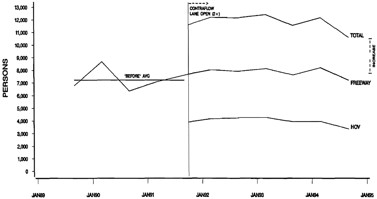
FIGURE F-10. EAST R.L. THORNTON FREEWAY (IH 30E) MAINLANE AND HOV LANE A.M. PEAK PERIOD PERSON TRIPS
