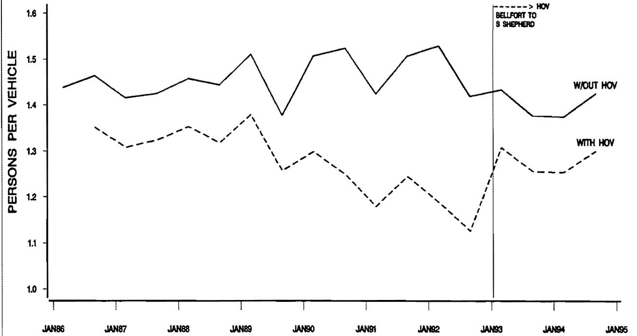
FIGURE E-14. SOUTHWEST FREEWAY (U.S. 59) MAINLANE AND HOV LANE A.M. PEAK HOUR 2+ CARPOOL UTILIZATION
