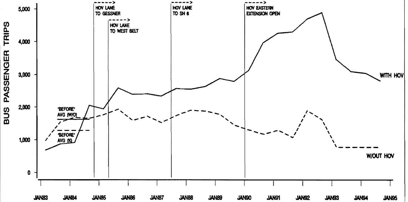
FIGURE A-20. KATY FREEWAY (IH 10W) CORRIDOR PARK-AND-RIDE DEMAND
