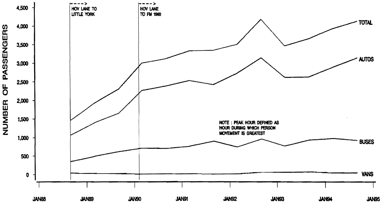
FIGURE D-2. NORTHWEST FREEWAY (US 290) HOV LANE A.M. PEAK PERIOD HOV LANE PERSON MOVEMENT
