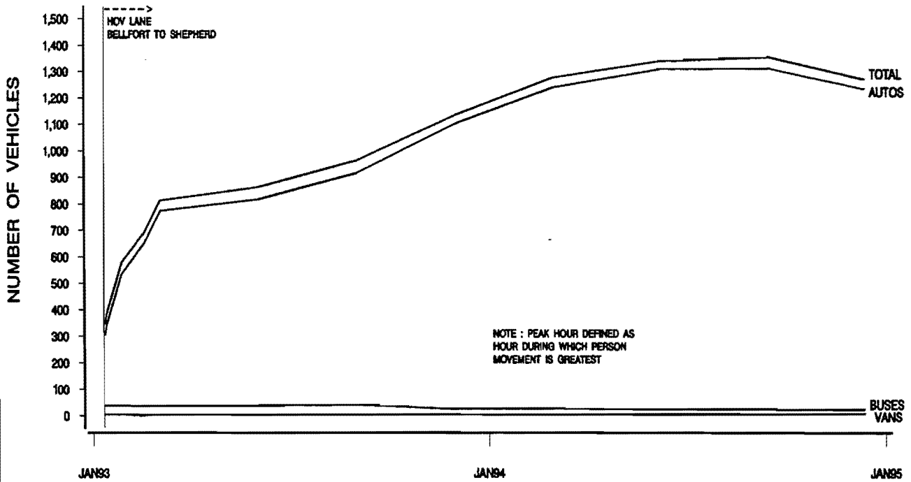
FIGURE E-4. SOUTHWEST FREEWAY (US 59S) HOV LANE A.M. PEAK PERIOD HOV LANE VEHICLE UTILIZATION
