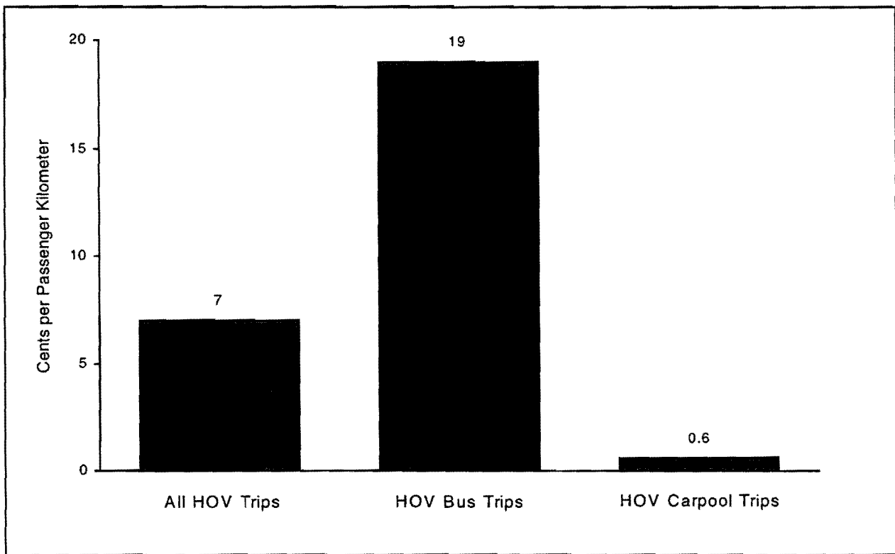
Figure 13. Operating Cost Per Passenger-Kilometer for the Operating Houston HOV Facilities, 1994
