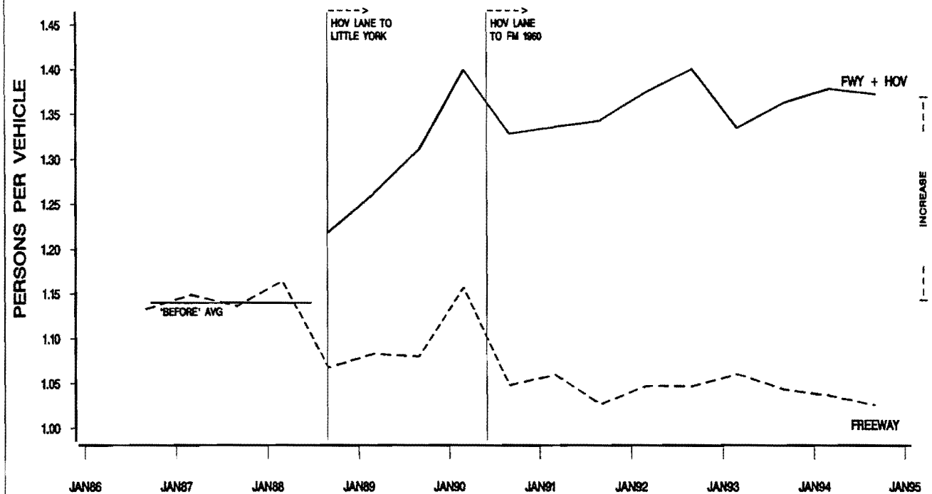
FIGURE D-12. NORTHWEST FREEWAY (U.S. 290) MAINLANE AND HOV LANE A.M. PEAK PERIOD AVERAGE OCCUPANCY
