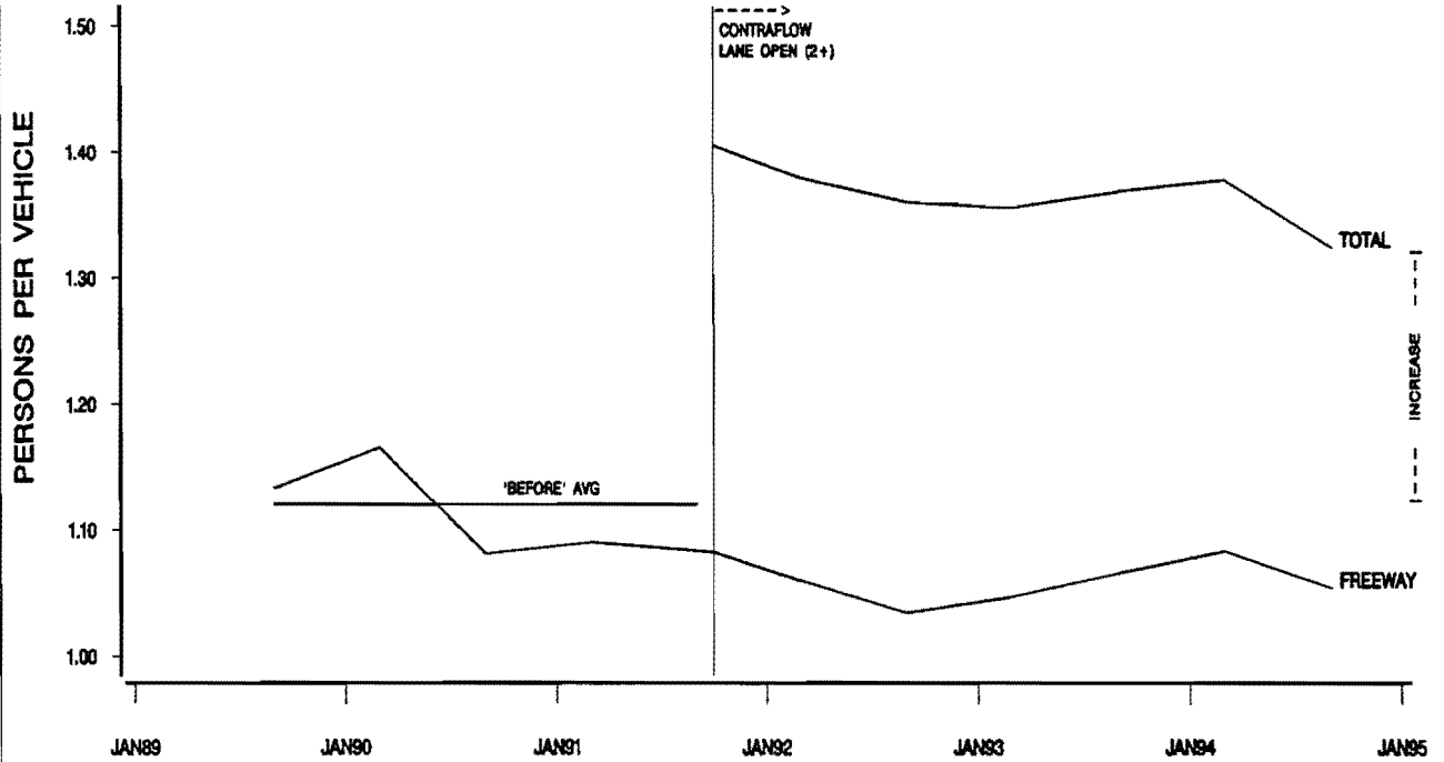
FIGURE F-12. EAST R.L. THORNTON FREEWAY (IH 30E) MAINLANE AND HOV LANE A.M. PEAK PERIOD AVERAGE OCCUPANCY
