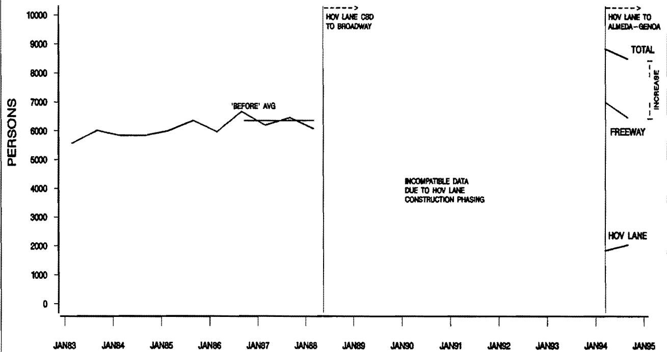
FIGURE C-10. GULF FREEWAY (IH 45S) MAINLANE AND HOV LANE A.M. PEAK PERIOD PERSON TRIPS
