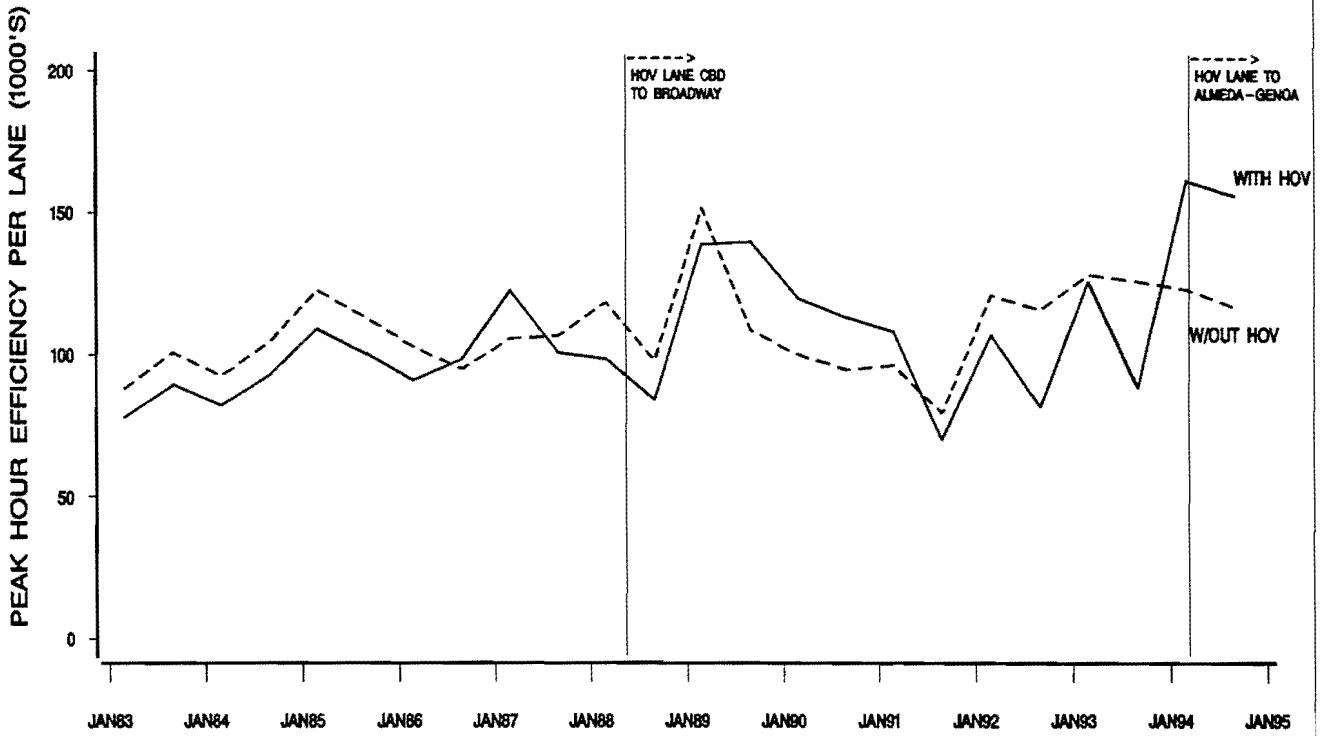
FIGURE C-16. GULF FREEWAY (IH 45S) MAINLANE AND HOV LANE A.M. PEAK HOUR BUS VEHICLE AND PASSENGER TRIPS
