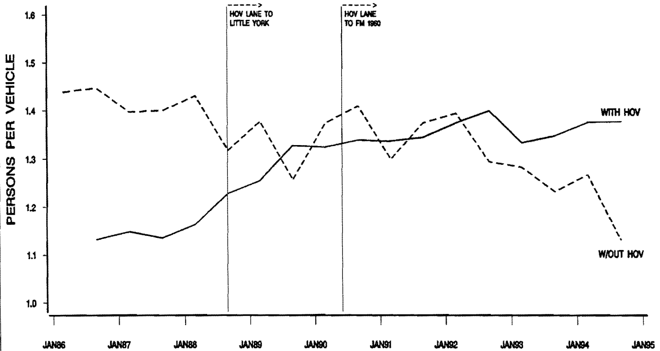
FIGURE D-14. NORTHWEST FREEWAY (U.S. 290) MAINLANE AND HOV LANE A.M. PEAK HOUR 2+ CARPOOL UTILIZATION
