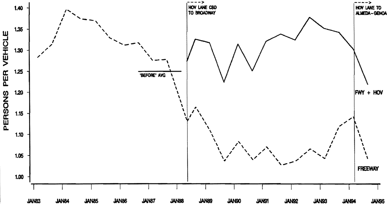
FIGURE C-12. GULF FREEWAY (IH 45S) MAINLANE AND HOV LANE A.M. PEAK PERIOD AVERAGE OCCUPANCY
