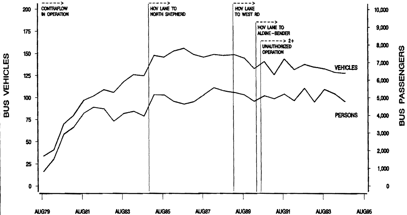
FIGURE B-18. A.M. PEAK PERIOD BUS PASSENGER TRIPS TOTAL, FREEWAY PLUS HOV LANE VOLUMES NORTH FREEWAY AND FREEWAY WITHOUT HOV LANE
