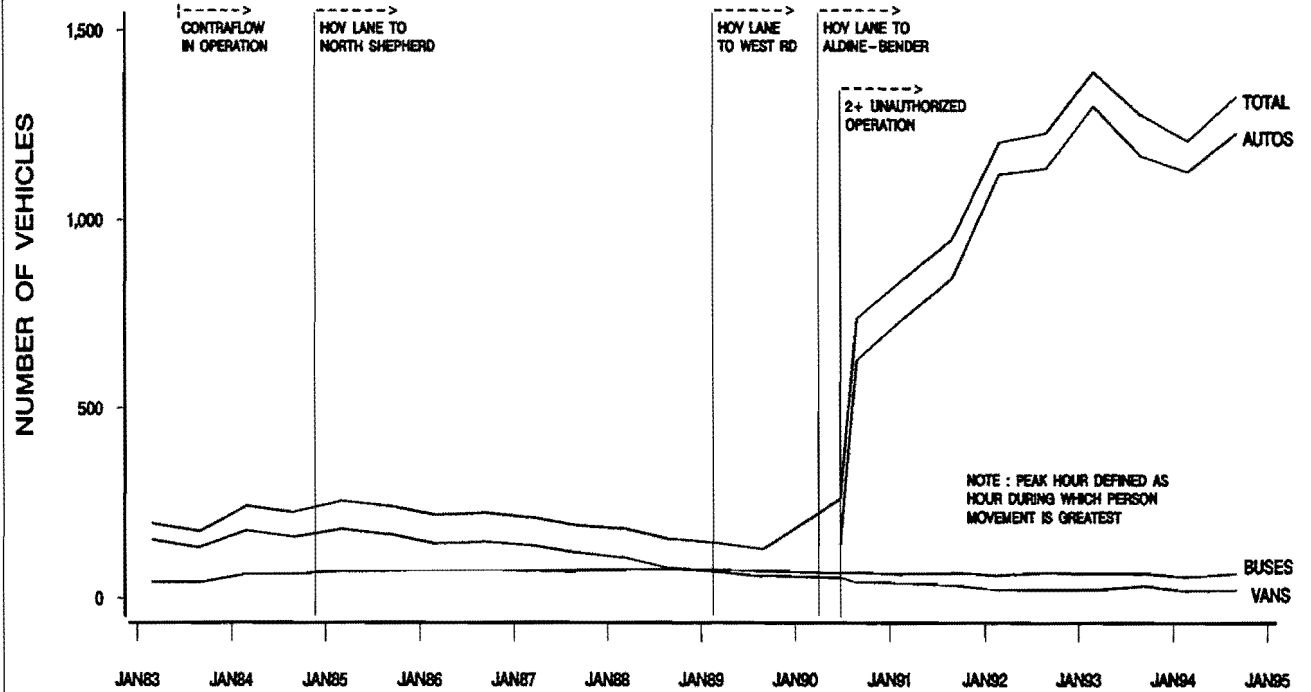
FIGURE B-4. NORTH FREEWAY (IH 45N) HOV LANE A.M. PEAK PERIOD HOV LANE VEHICLE UTILIZATION
