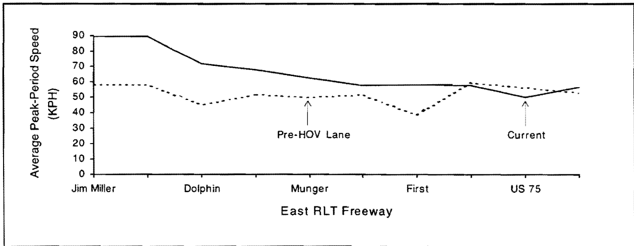
Figure 41. Freeway Peak-Period Speeds on Mainlanes, Pre-HOV and Current (Cont'd)
