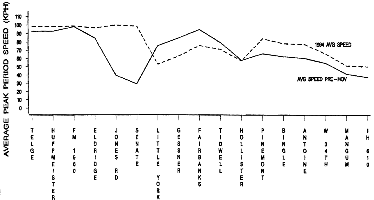
FIGURE D-8. NORTHWEST FREEWAY (U.S. 290) MAINLANE TRAVEL TIME AND SPEED SURVEY SOUTHBOUND, TELGE TO IH 610 A.M. PEAK PERIOD
