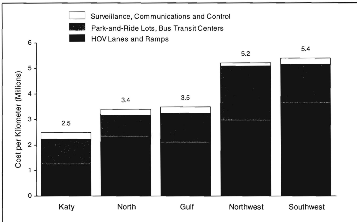
Figure 12. Capital Cost Per Kilometer (Year-of-Construction Dollars) of the Operating Houston HOV Facilities
