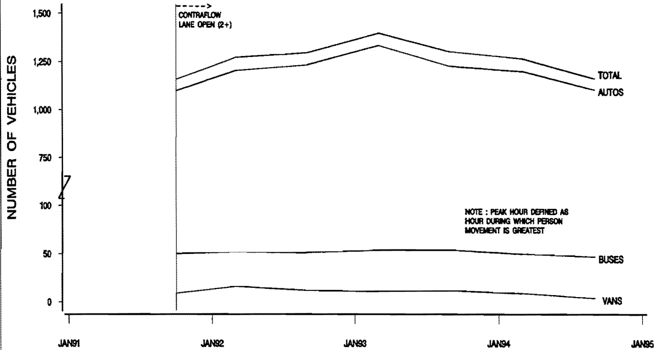
FIGURE F-4. EAST R.L. THORNTON FREEWAY (IH 30E) HOV LANE A.M. PEAK PERIOD HOV LANE VEHICLE UTILIZATION
