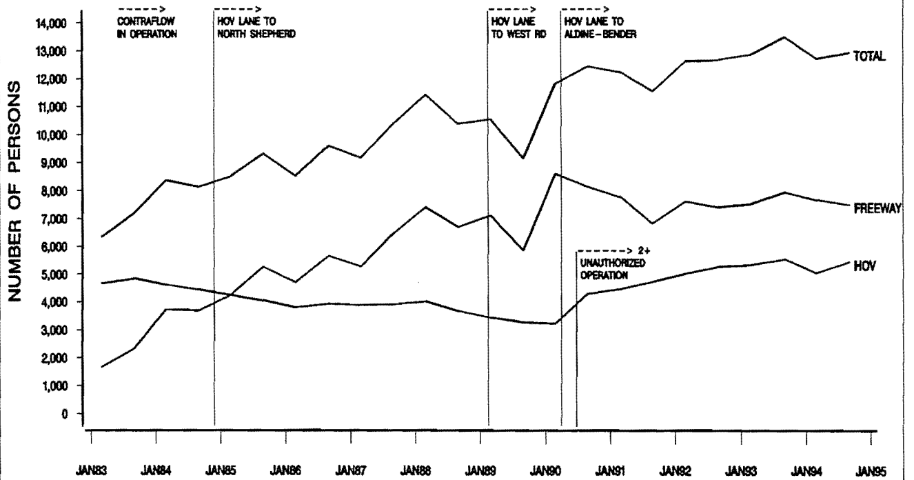
FIGURE B-12. NORTH FREEWAY (IH 45N) MAINLANE AND HOV LANE A.M. PEAK PERIOD PERSON TRIPS
