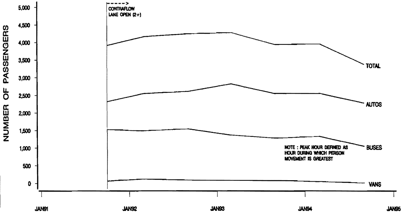
FIGURE F-2. EAST R.L. THORNTON FREEWAY (IH 30E) HOV LANE A.M. PEAK PERIOD HOV LANE PERSON MOVEMENT
