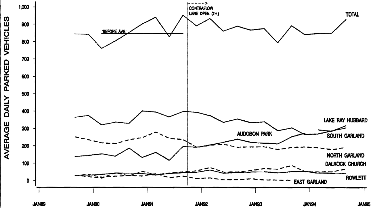
FIGURE F-20. AVERAGE DAILY VEHICLES AT PARK-AND-RIDE LOTS EAST R.L. THORNTON FREEWAY AND FREEWAY WITHOUT HOV LANE
