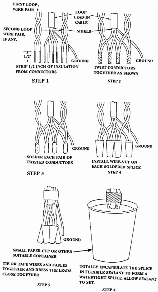
Figure 5.7 Paper Water Cup Watertight Seal Installation Procedure
