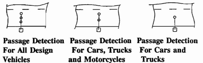
Figure 8.1 Suggested Microloop Installation Patterns
