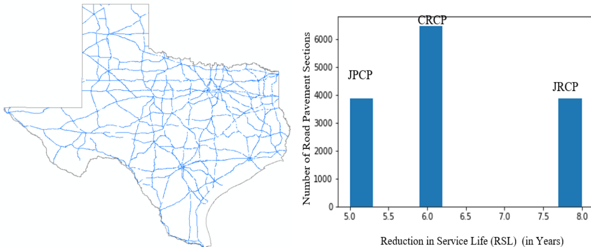
Figure 8.28. RSL Estimation for Rigid Pavements in Texas Highway Freight Network.
