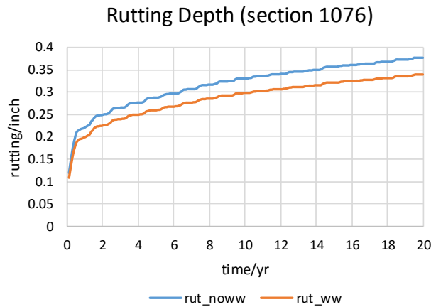
Figure 6.27. Rutting Evolution for Pavement Section 48-1076.
