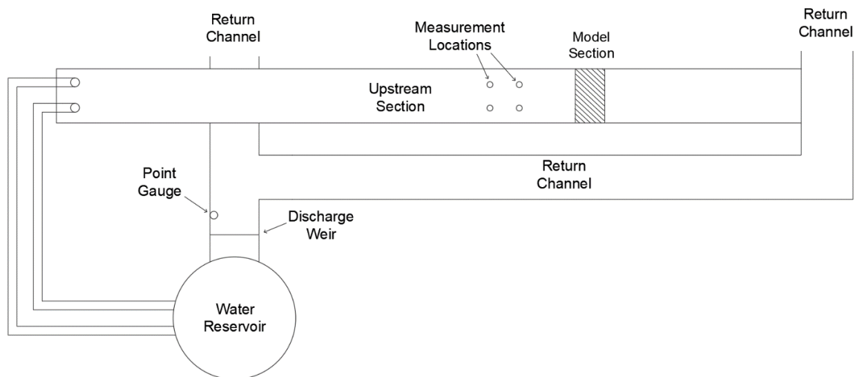
Figure 5.10. Flume Layout.
