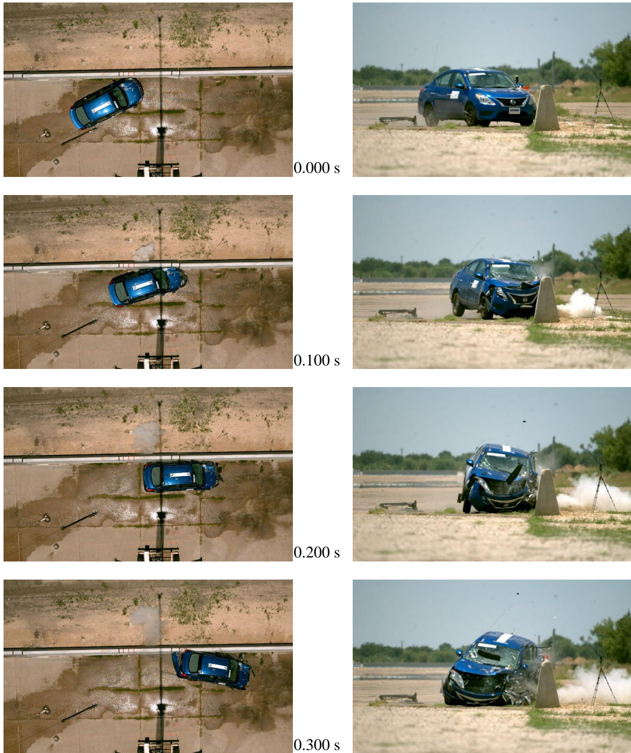
Figure C.1. Sequential Photographs for Test No. 469760-06-1 (Overhead and Frontal Views).
