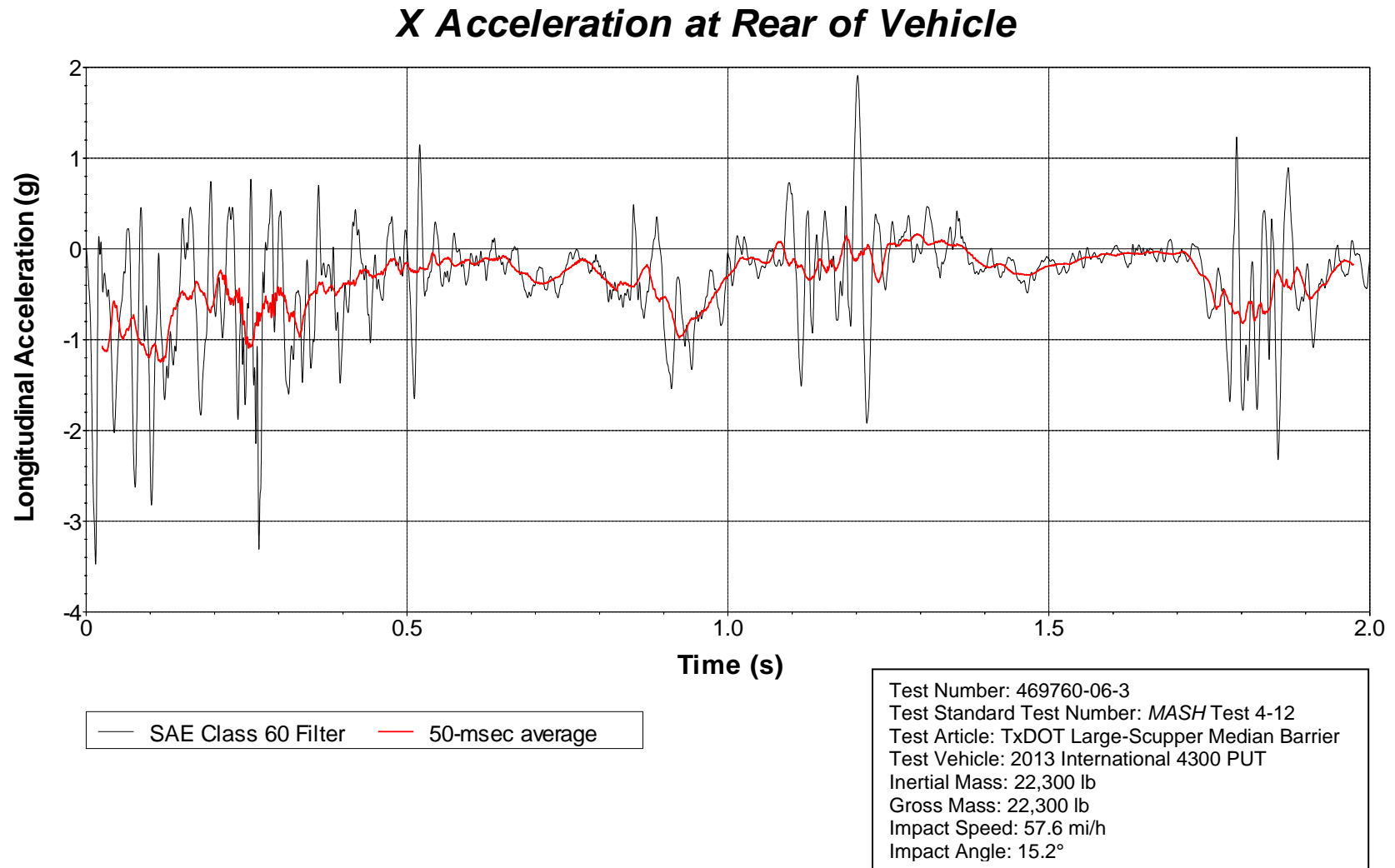
Figure E.7. Vehicle Longitudinal Accelerometer Trace for Test No. 469760-06-3 (Accelerometer Located at Rear of Vehicle).
