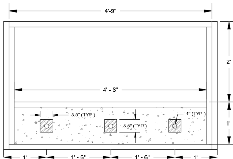
Figure 5.7. Initial Support Base Design.
