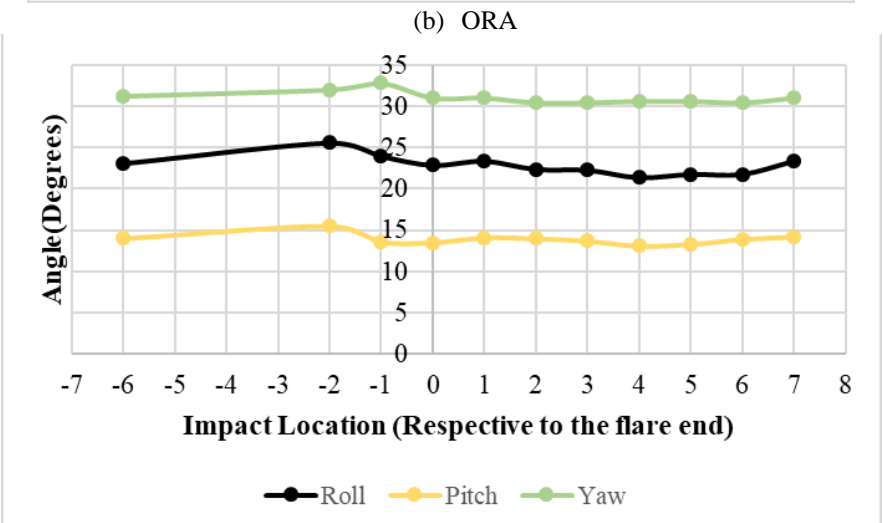
Figure 4.26. Parametric Analysis Results for Option A with Pickup Truck (without Tire Disengagement.)
