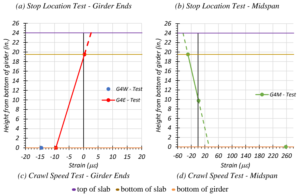
Figure 8.11. Static Strains for Interior Girder G4—Middle Path
