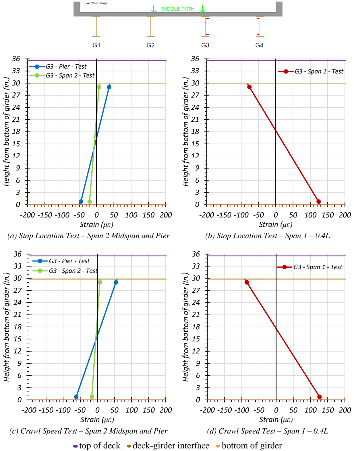
Figure 7.16. Static Strains for Interior Girder G3: Middle Path—Span 1
