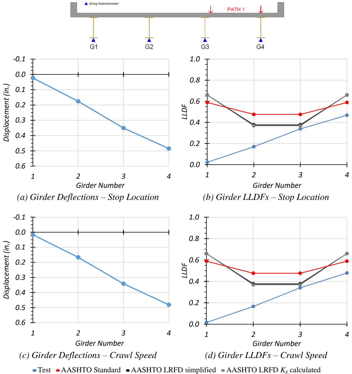
Figure 7.22. Static Deflection Results for Path 1—Span 1 Loading
