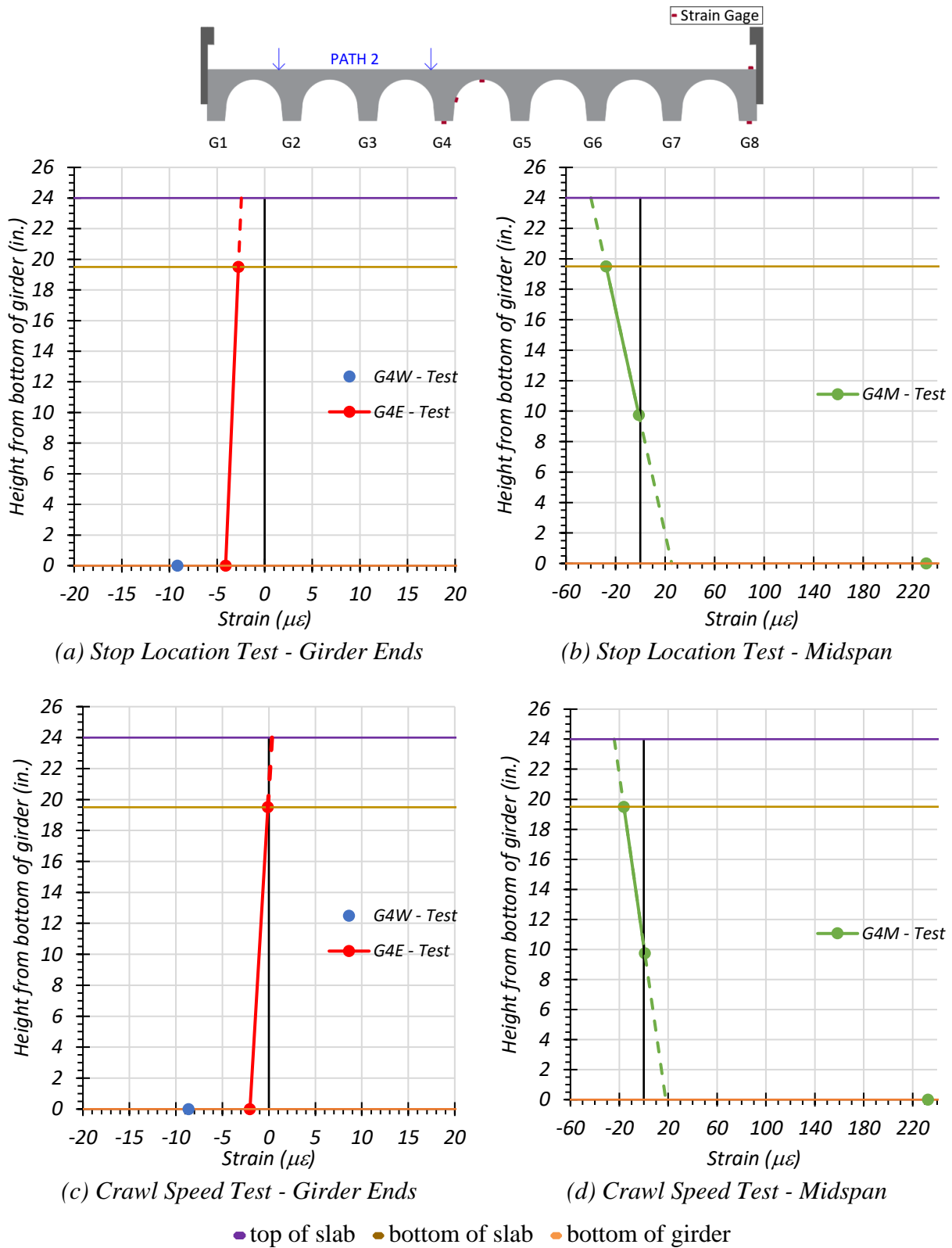
Figure 8.10. Static Strains for Interior Girder G4—Path 2
