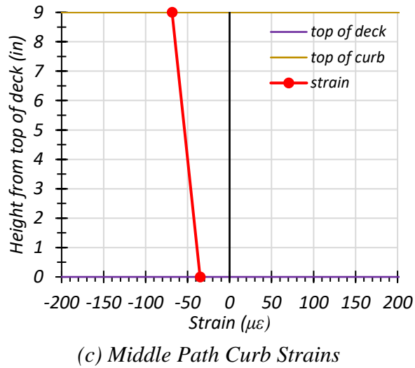
Figure 7.39. Curbs Strains for Loading of All Paths
