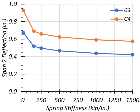
(c) Effect on Span 2 Deflection
