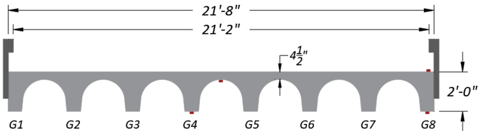
(c) End Section
