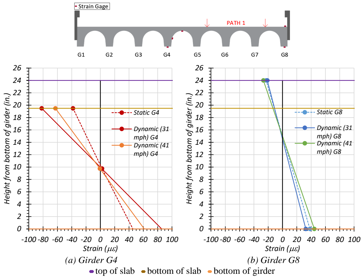
Figure 8.21. Maximum Strains for Static and Dynamic Tests for Path 1 Loading
