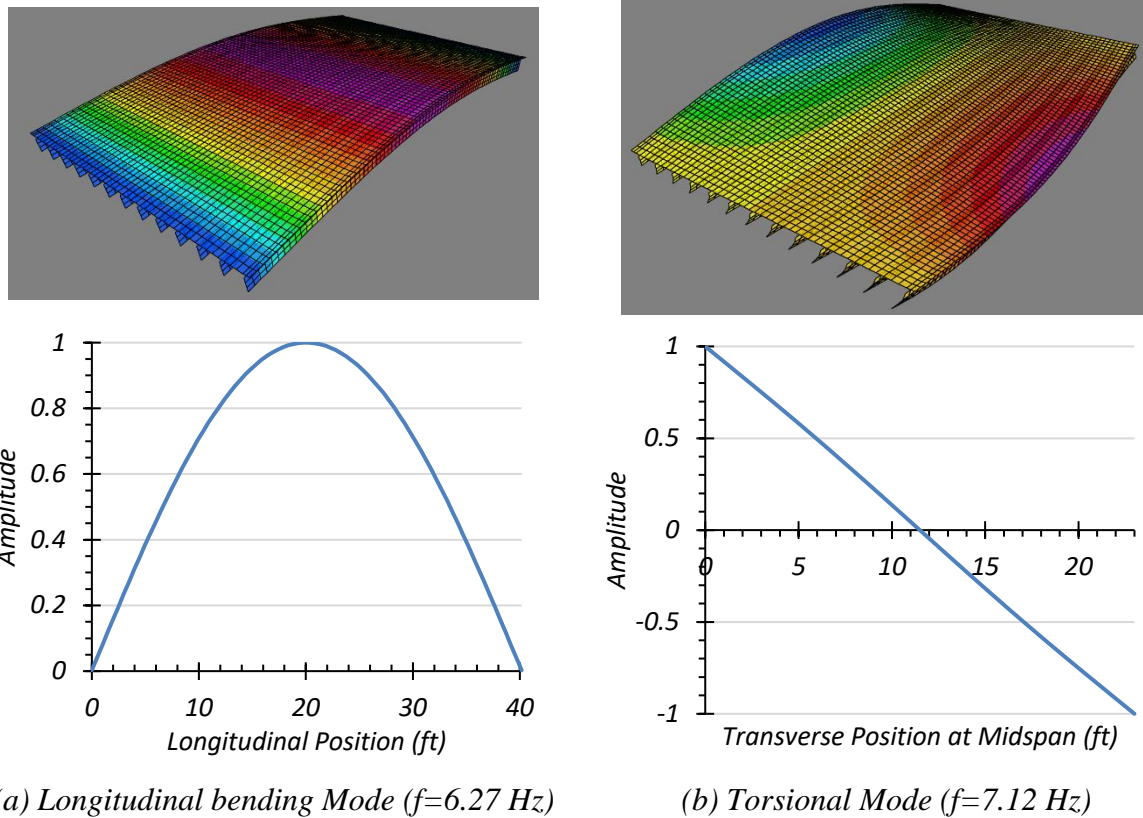
Figure 2.18. First Two Mode Shapes of Composite Bridge SM-5
