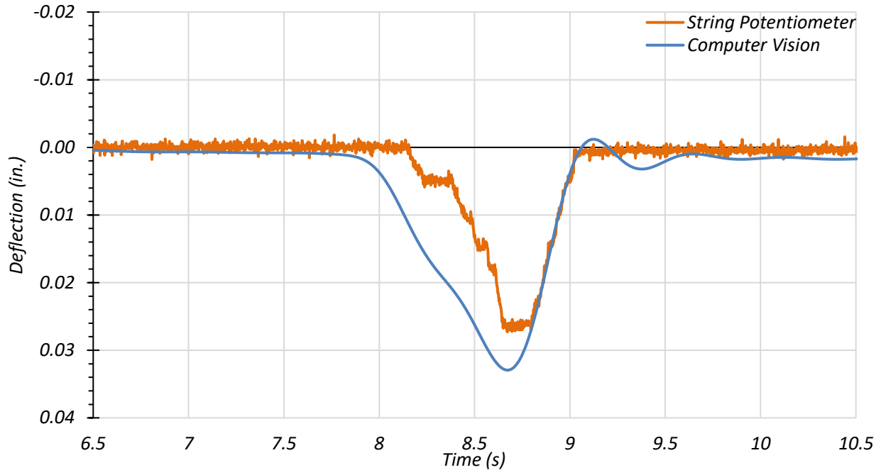
Figure 9.42. Section 9 Midspan Deflections for Path 1—Dynamic Test at 31 mph
