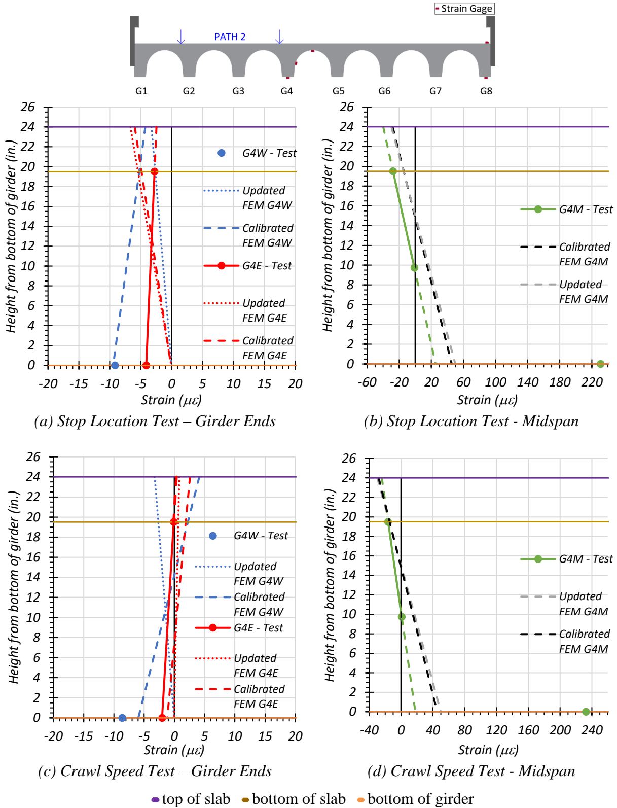
Figure 8.38. Comparison of Static Strains for G4 with FEM Results—Path 2
