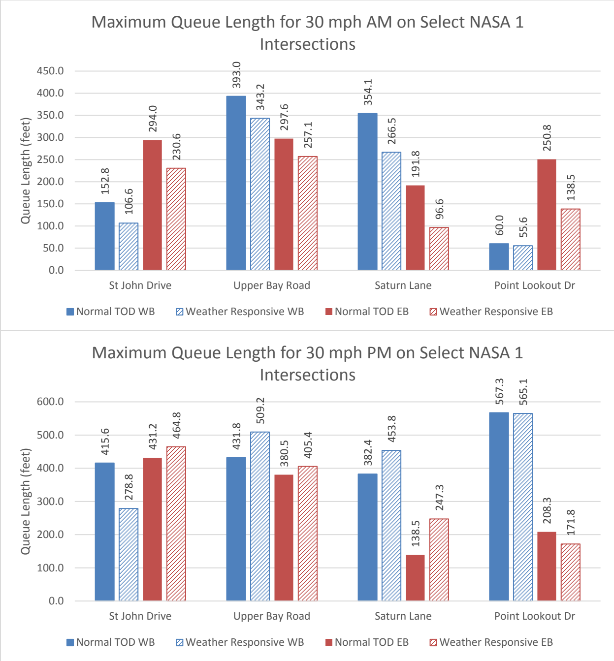
Figure 42. Maximum Queue Lengths – NASA Road 1 in Nassau Bay, TX.
