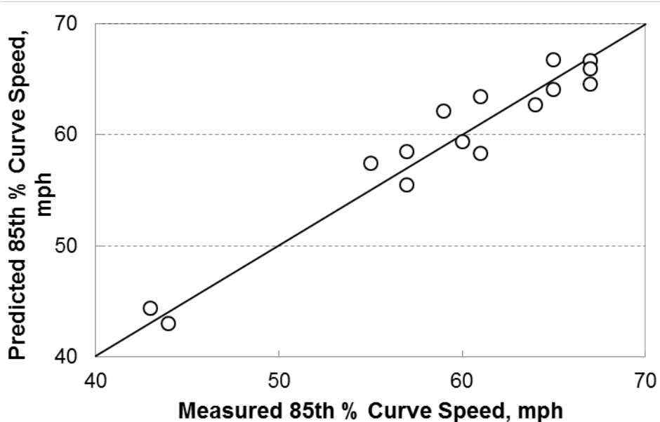
Figure 40. Comparison of Measured and Predicted Curve Speeds.
