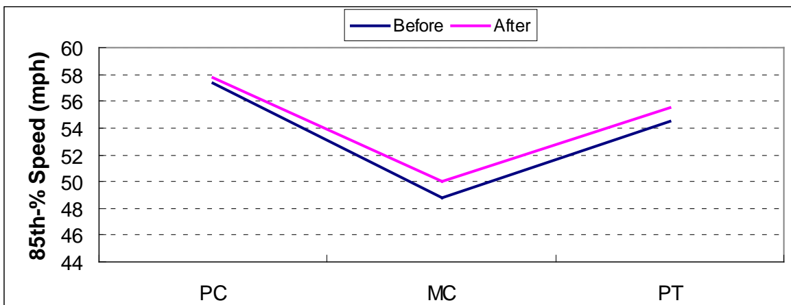
Figure 56. Speed Profile.
