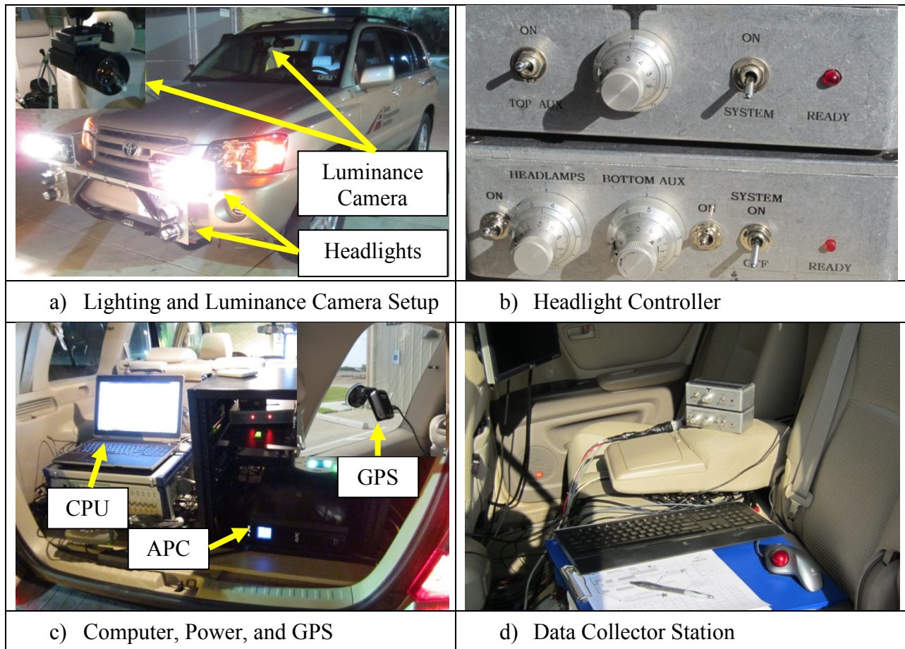
Figure 8. Human Factors Data Collection Setup.
