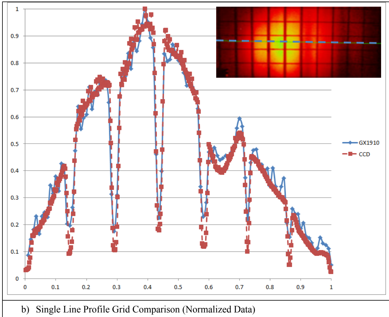
Figure 3. Camera Comparison Grid Method (Continued).
