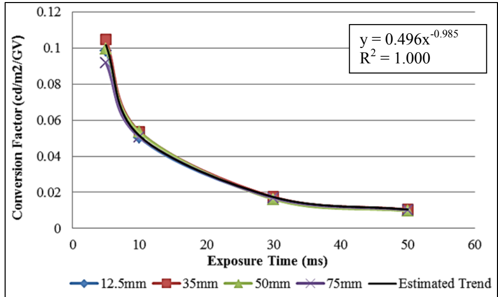
Figure 7. Focal Length Comparison.
