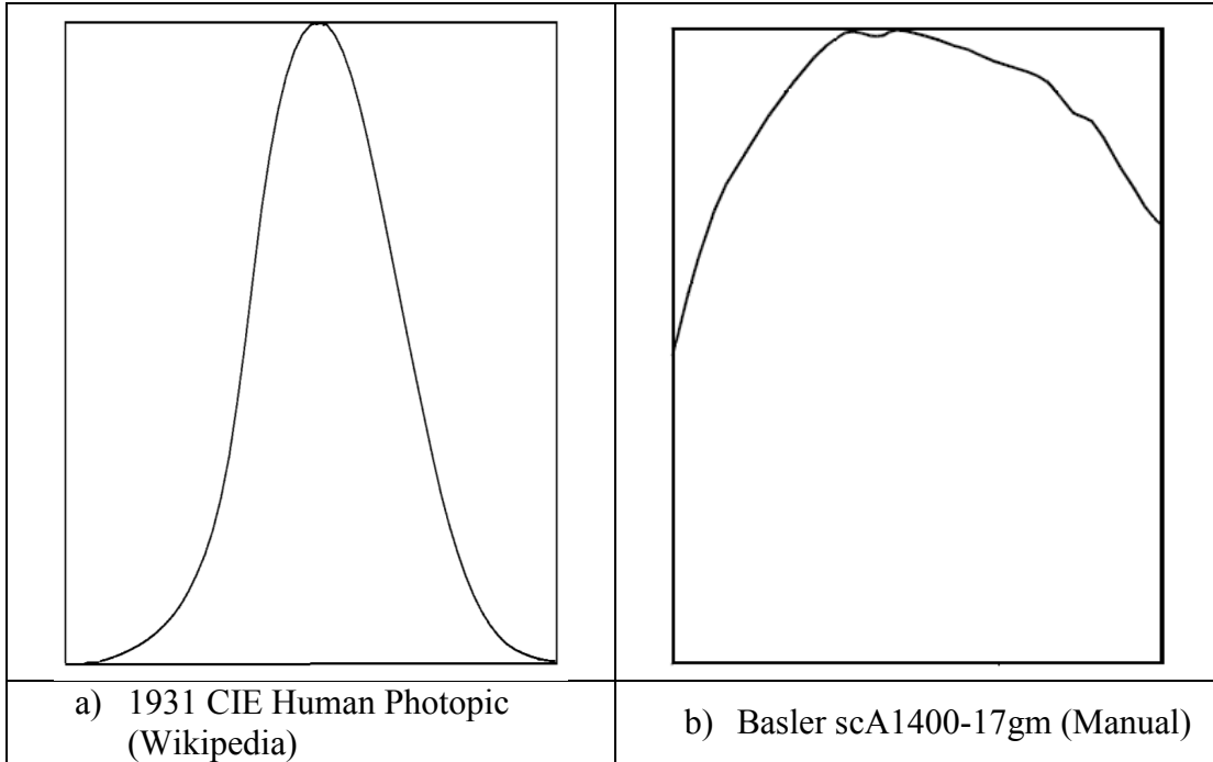
Figure 4. 400–700 nm Luminous Efficiency Function Comparison.
