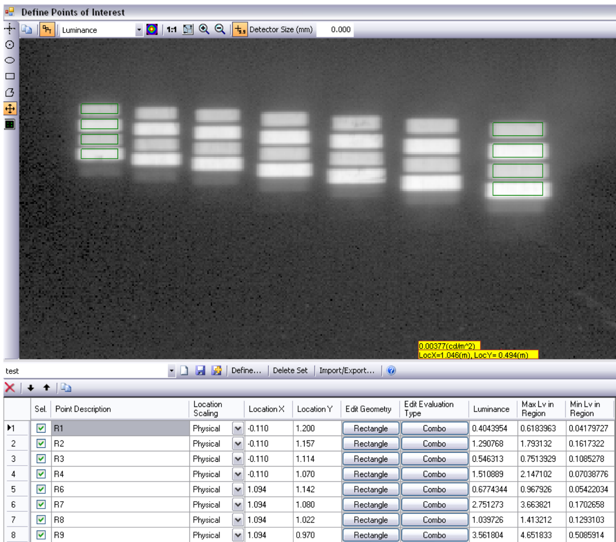
Figure 2. CCD Photometer Luminance Measurements.
