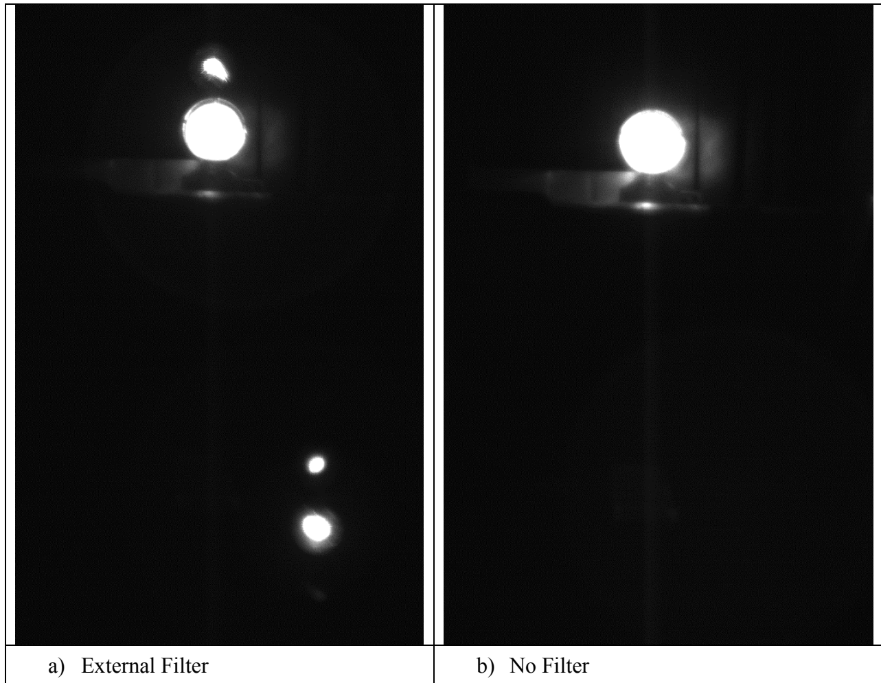
Figure 5. Internal Reflection Problem with External Filter Installation.
