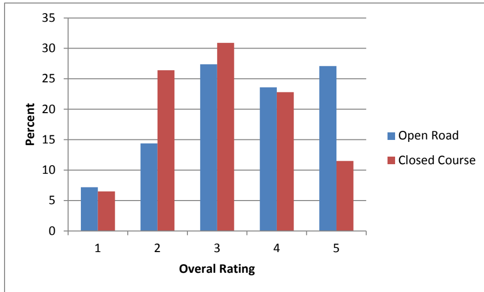
Figure 12. Open Road versus Closed Course Overall Rating for Tangent Treatments.
