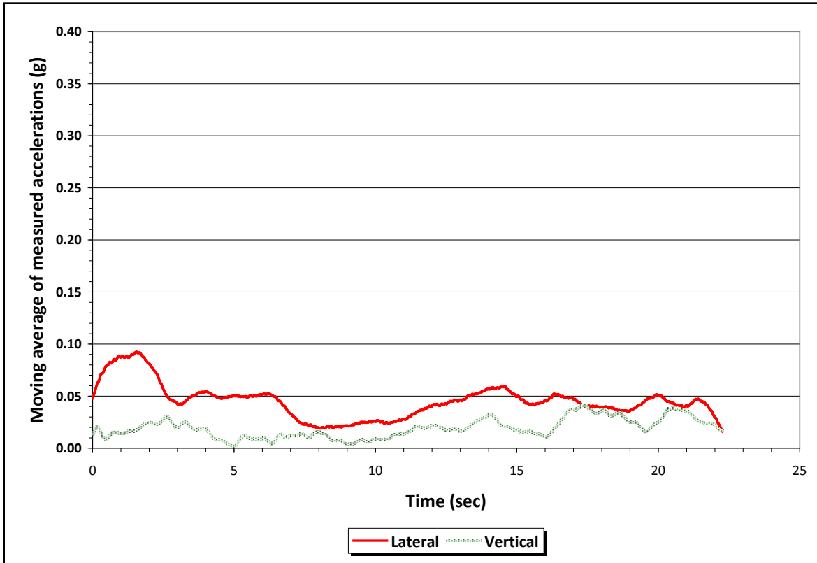
Figure 15. Average Accelerations on SH6 Curve Section (C19) Computed over a 1-second Moving Time Window.
