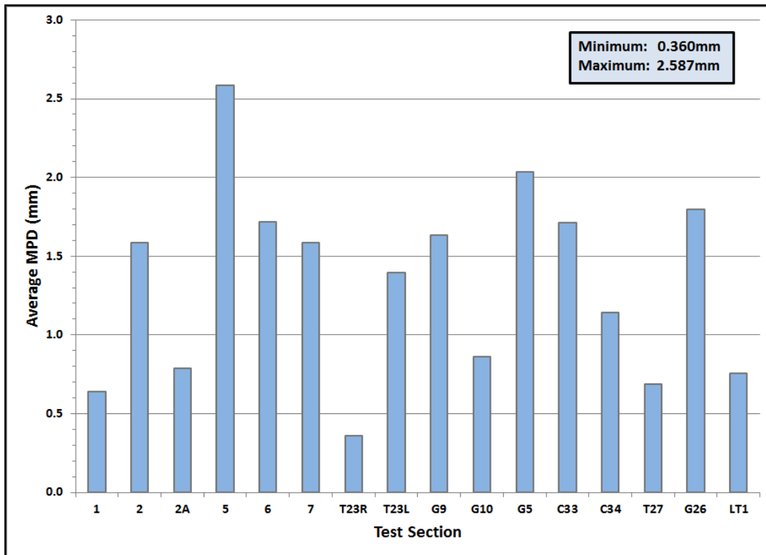
Figure 38. Average MPDs Determined from CTM Measurements on Each Section.
