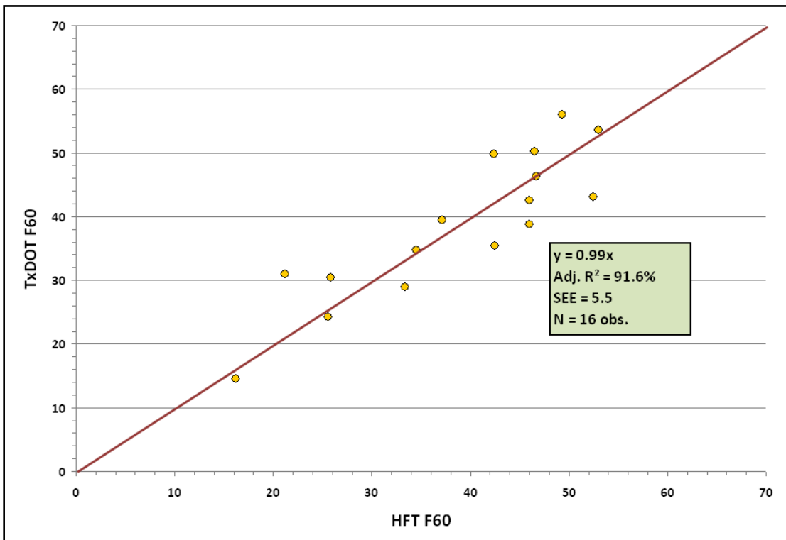
Figure 41. Comparison of Calibrated F60 Values (TxDOT Locked-Wheel vs. HFT).
