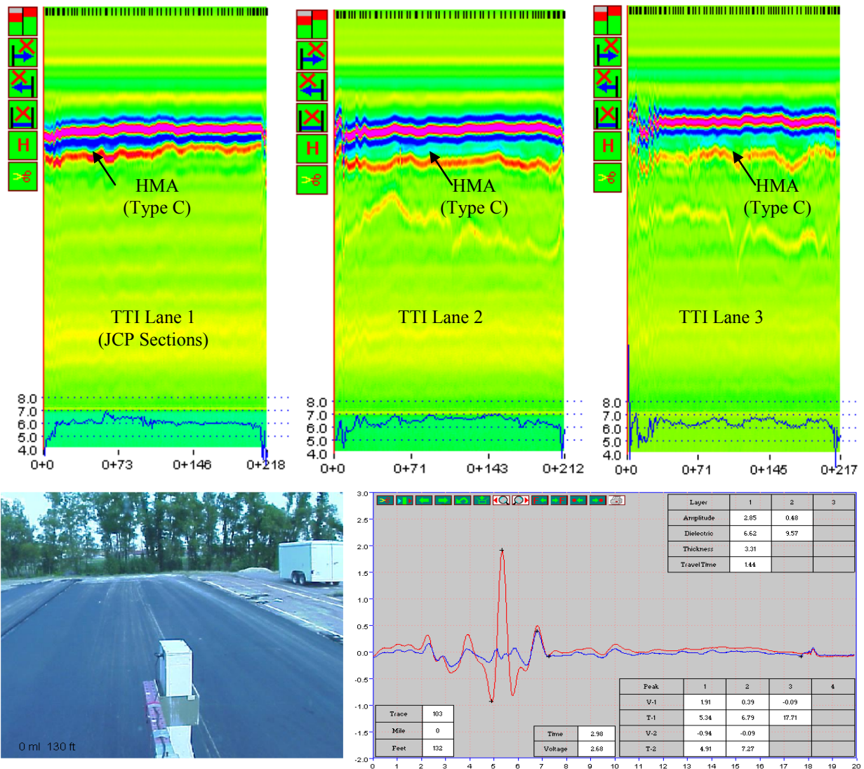
Figure 3-8. GPR Measurements.
