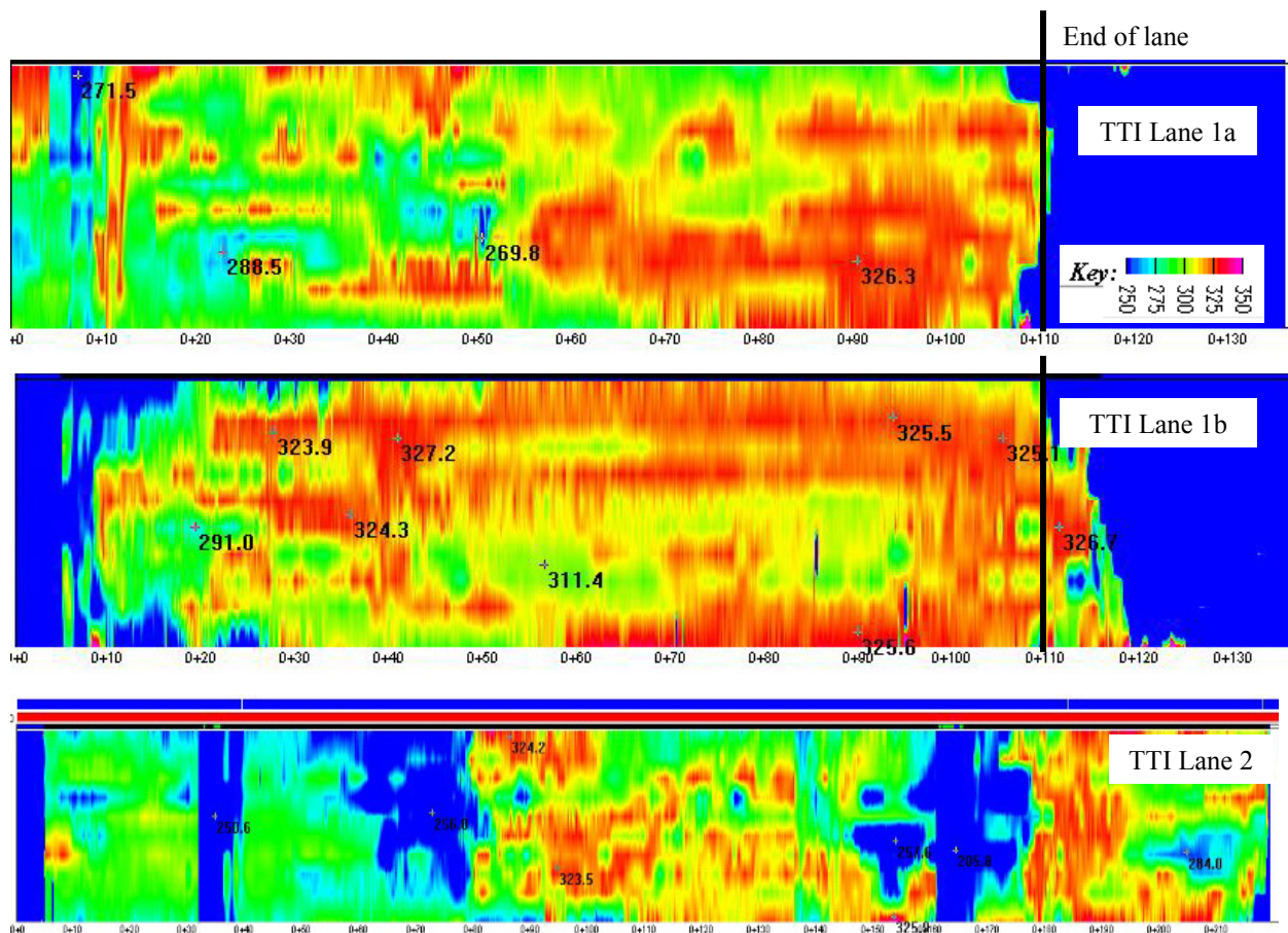
Figure 3-7. IR Thermal Imaging of the HMA (Type C) Mat.
