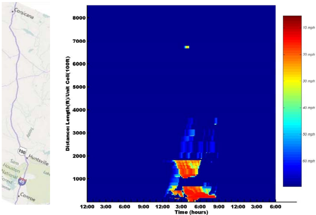
Figure 42. Speed Contour Example on I-45.
