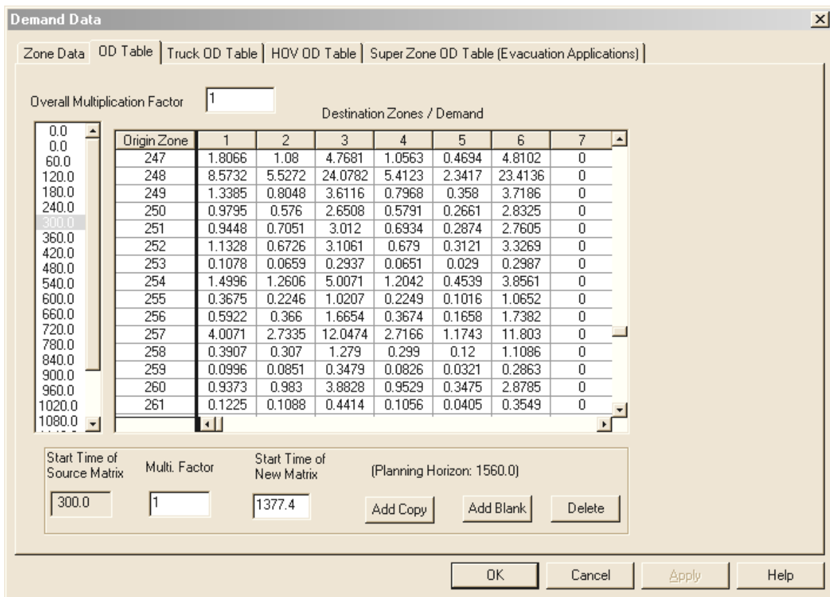
Figure 9. DynusT Origin-Destination Demand Data.
