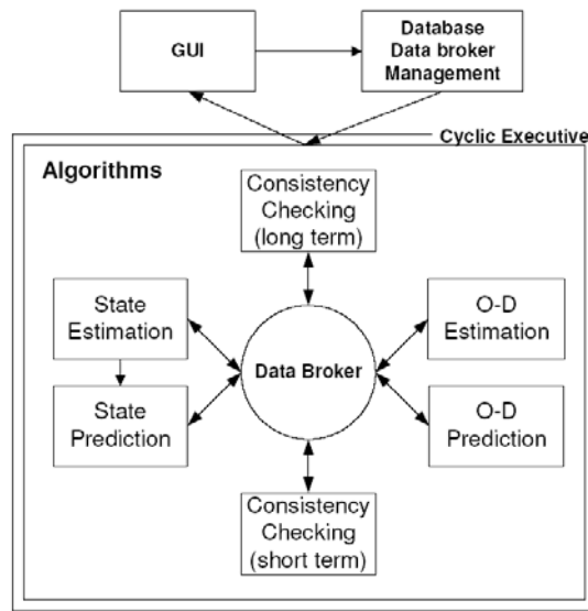
Figure 3. DynaSmart-X Schematic View (33).
