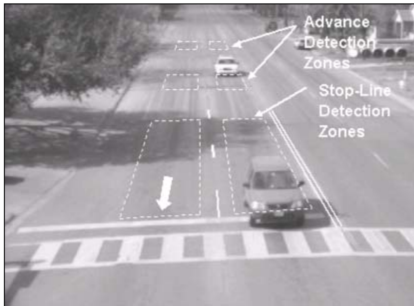
Figure 6. Illustrative Optimal Detection Zone Layout.
