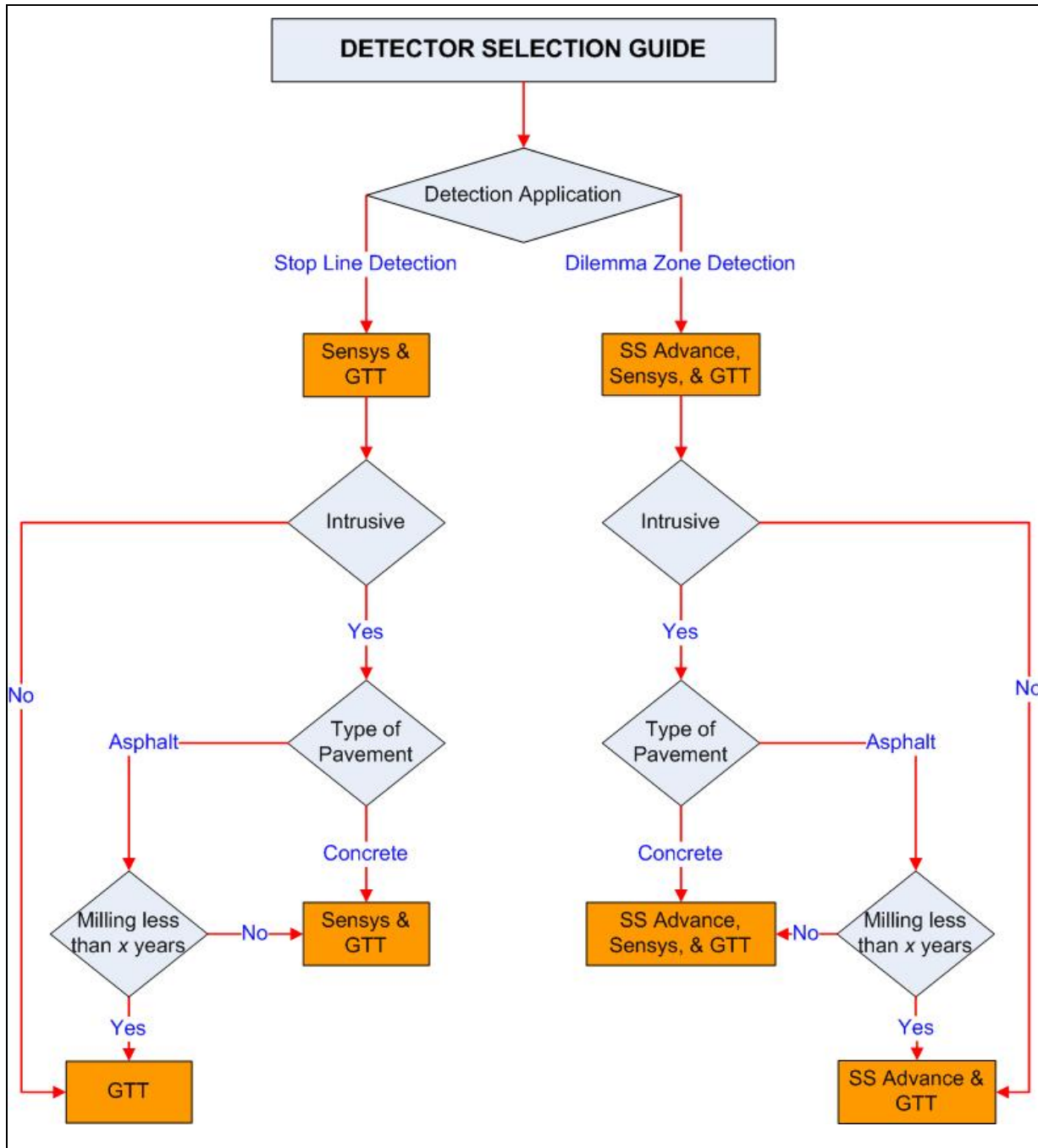
Figure 24. Flowchart for Detector Selection Process.
