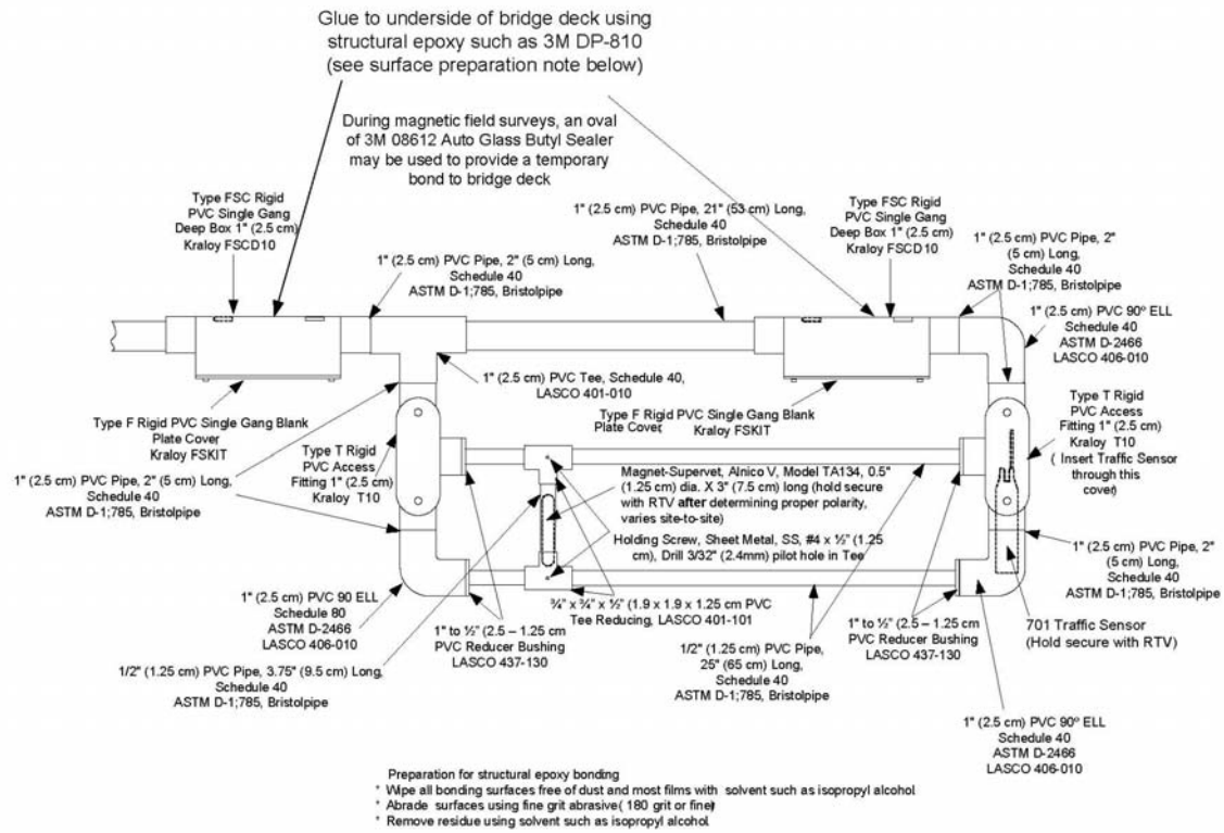
Figure 7. Ambient Magnetic Field Adjustment Device 2
