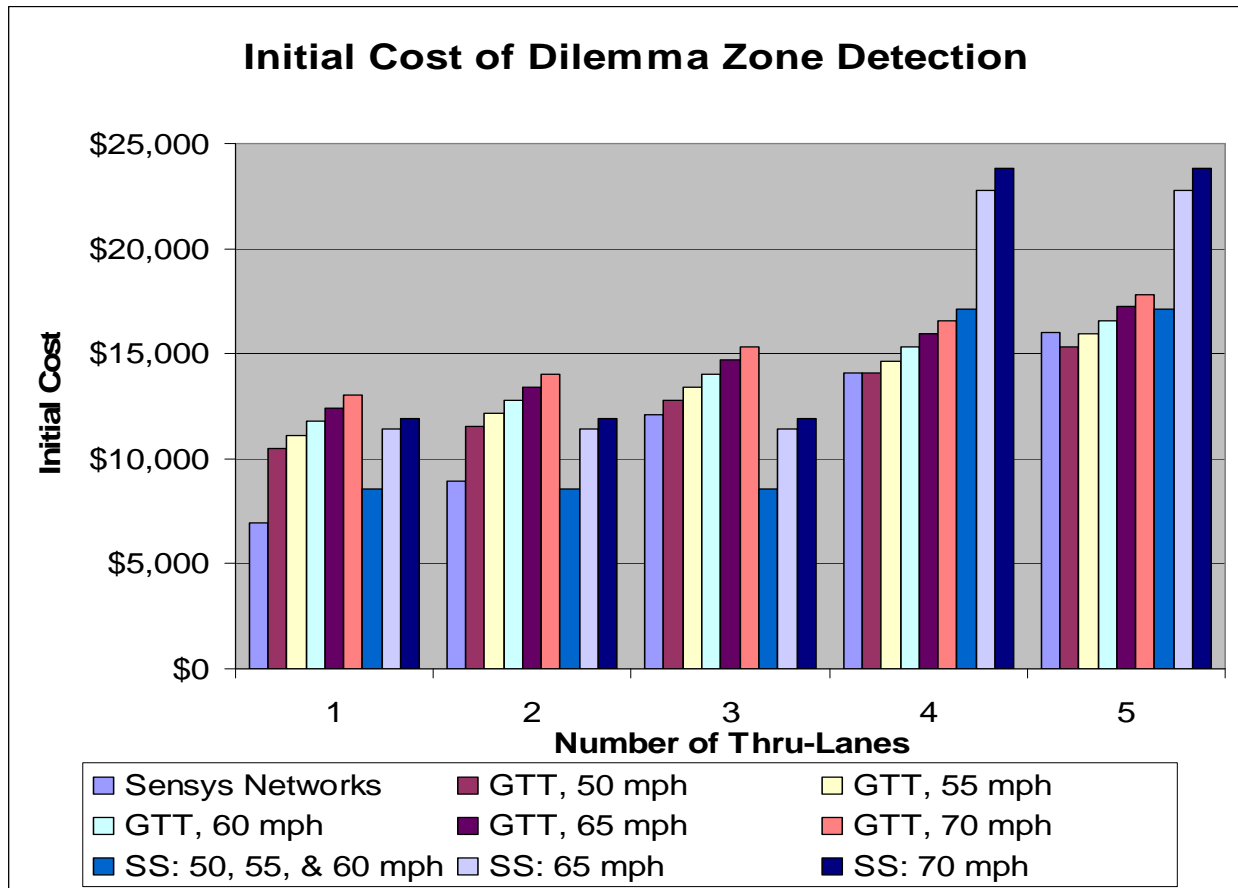
Figure 13. Initial Cost of Dilemma Zone Detection per Approach (No Stop Line Detection).
