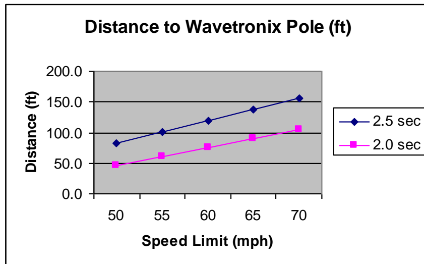
Figure 85. Maximum Distance of Advance Detector from Stop Line.
