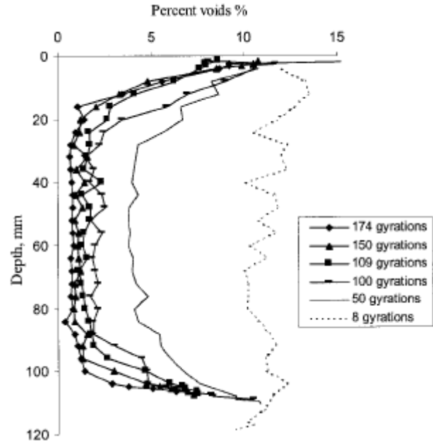
Figure 2-13. Distribution of Voids in Gyratory Specimens (Masad et al., 1999b).
