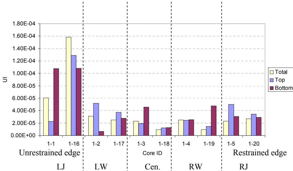
Figure 4-27. UI for the US 259 Test Section (Pattern 1).
