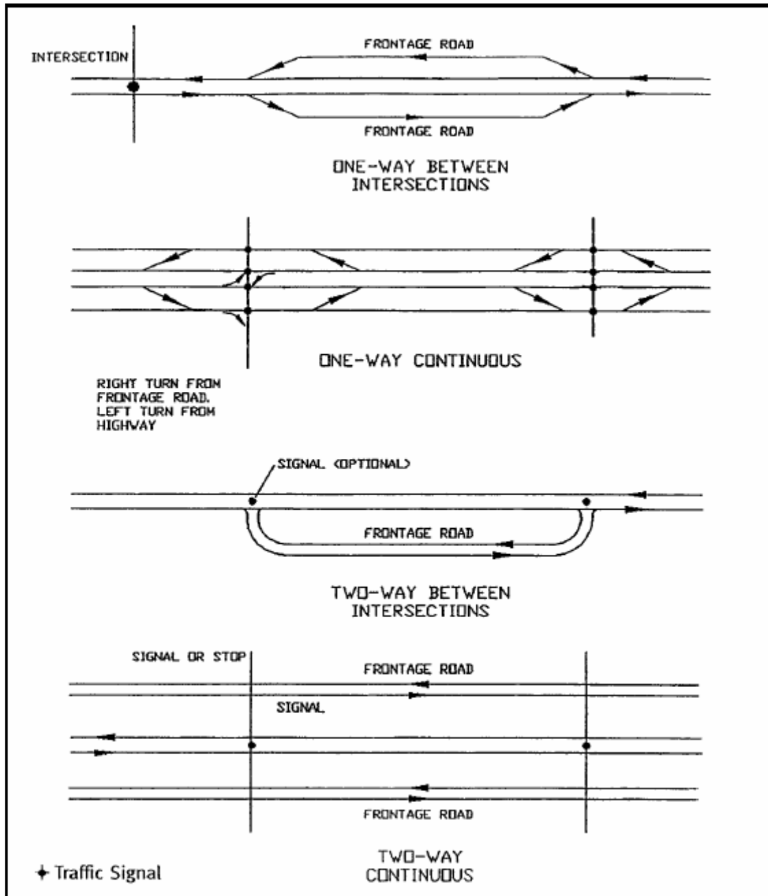
Figure 2-30. Types of Frontage Roads (II).
