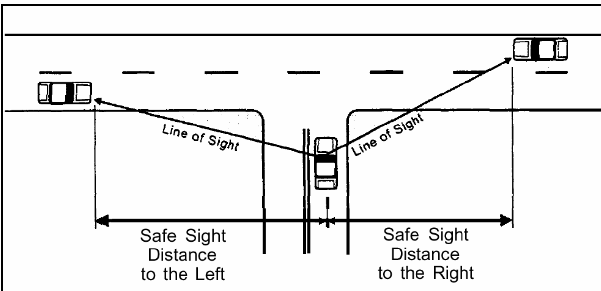
Figure 2-11. Entering Sight Distance Criteria (13).
