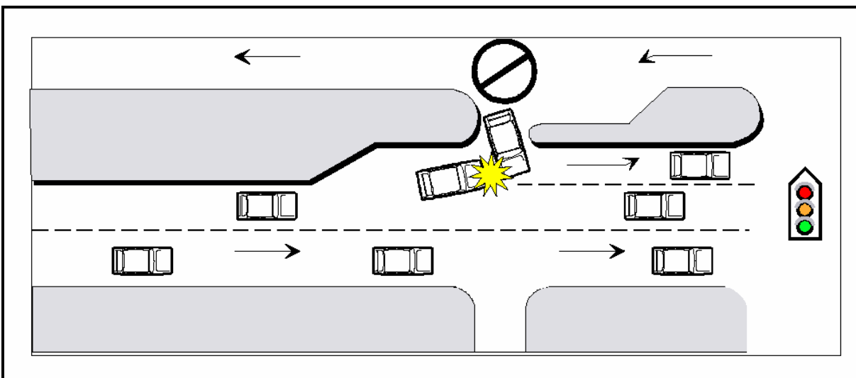
Figure 2-17. Left-Turn Median Opening Prohibition (16).
