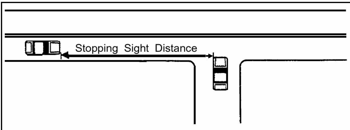
Figure 2-10. Stopping Sight Distance Criteria (13) .
