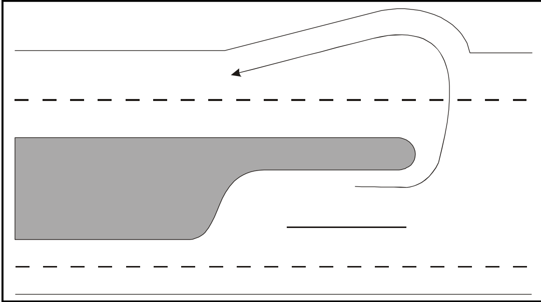
Figure 2-26. Flare-Out Jughandle Design (15).
