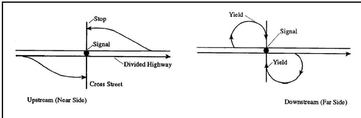
Figure 2-25. Basic Jughandle Design (11).
