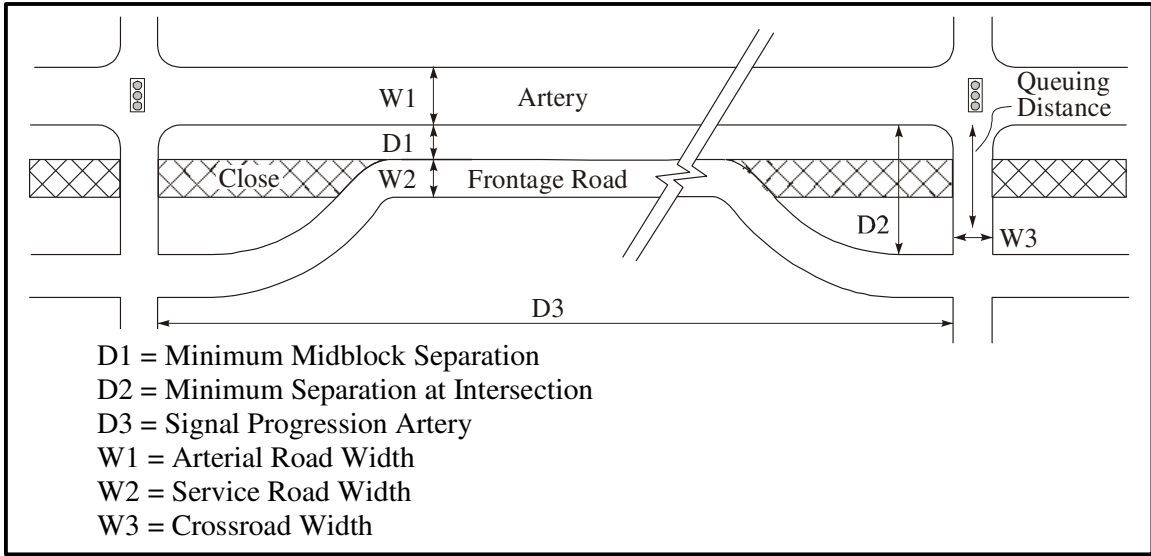
Figure 2-33. Arterial Frontage Road Design (II).
