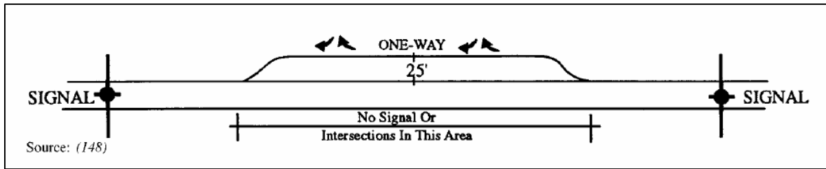
Figure 2-32. Arterial Frontage Road Concept for Retrofit Conditions (3).
