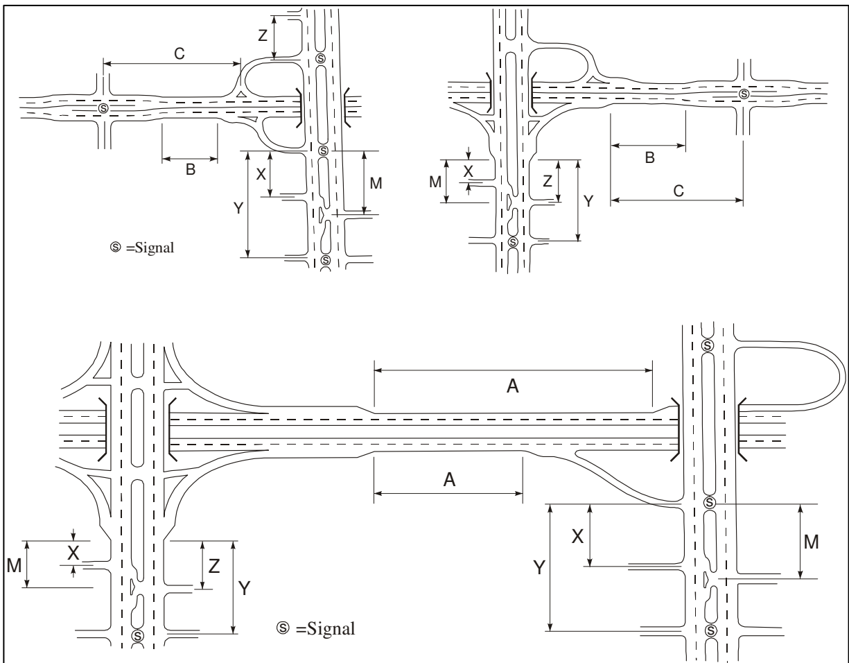
Figure 2-29. Interchange Spacing.
