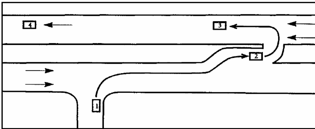
Figure 2-19. U-Turn Alternative for Left-Turn Egress (II).
