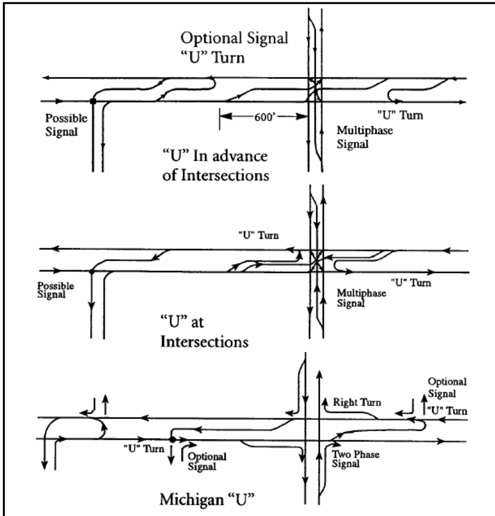
Figure 2-20. U-Turn Alternative Approaches (II).
