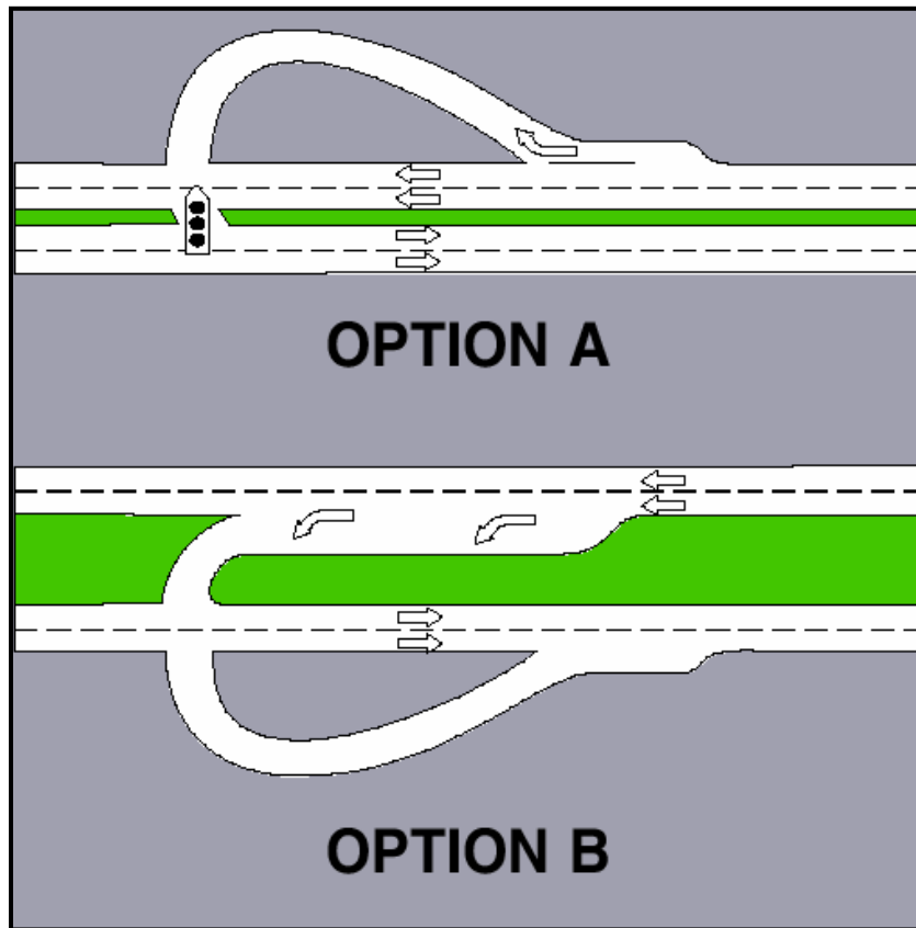
Figure 2-27. Jughandle U-Turn Design for Large Vehicles or Limited Pavement Width (15)
