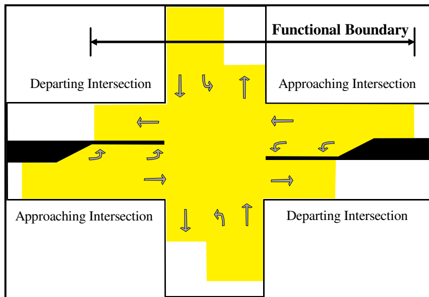
Figure 2-13. Functional Boundary of an Intersection (14).
