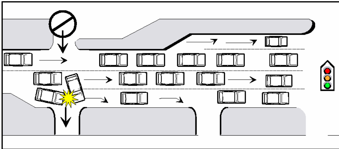
Figure 2-18. Right-Turn Median Opening Avoidance (16).
