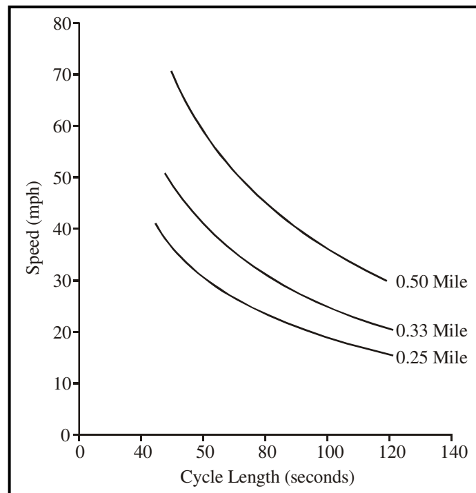
Figure 2-8. Signal Spacing as a Function of Speed and Cycle Length (II).
