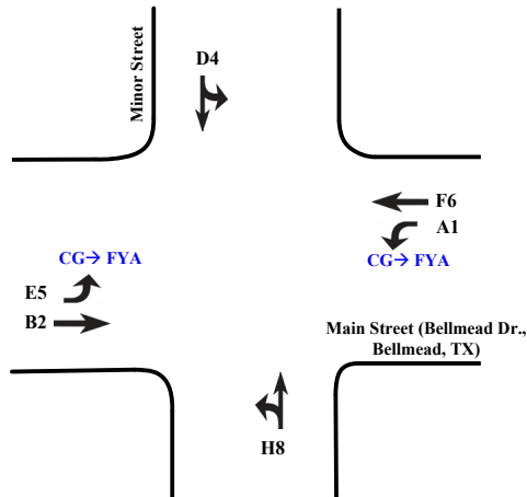
Figure 4-13: Signal Phase Assignment
