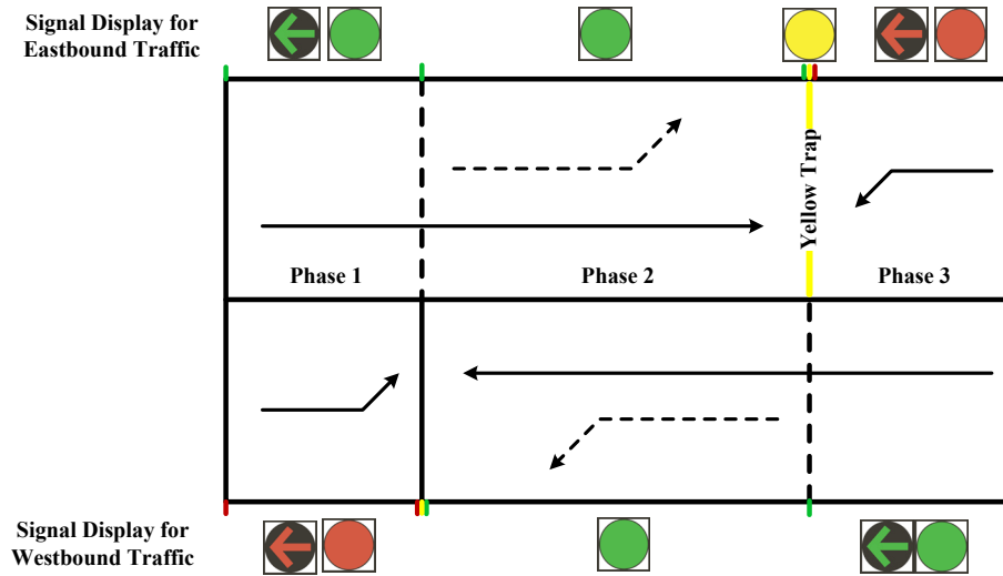
Figure 1-1: Yellow Trap Illustration in Phasing Graph
