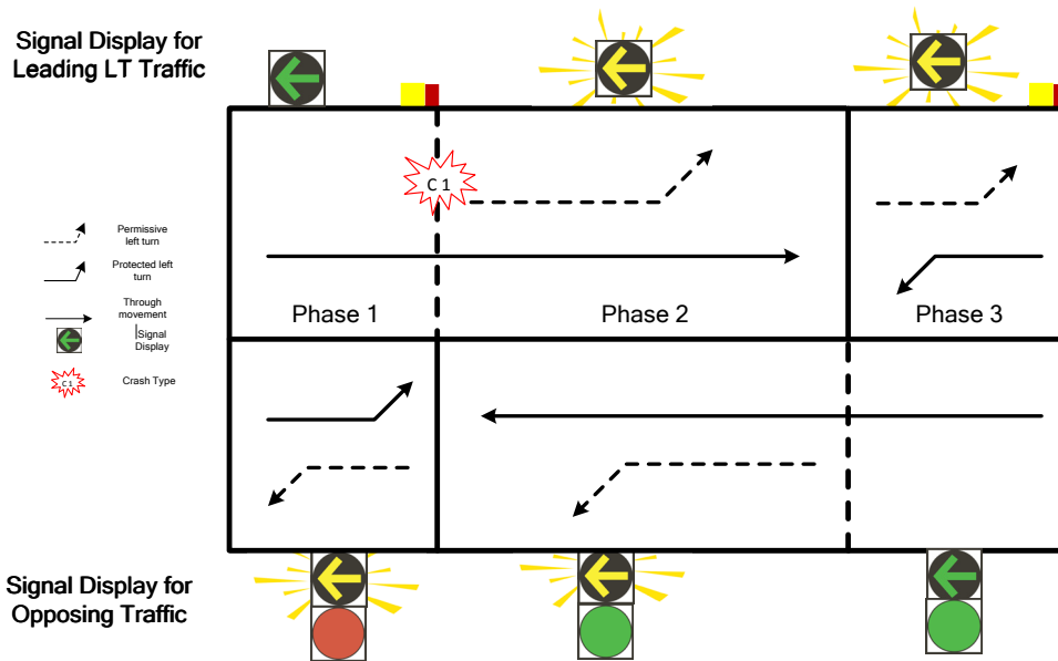
Figure 5-2: Signal Phase of Lead-Lag PPLT Operation
