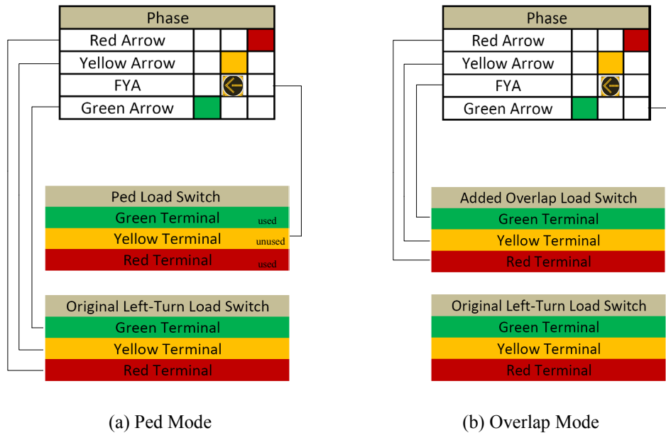
Figure 6-7: Typical Overlap Programming Methods for FYA PPLT
