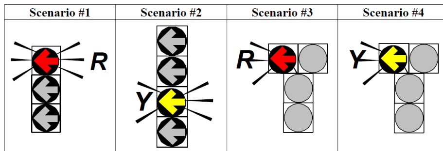
Figure 2-6: Permissive Displays Evaluated at Wide-Median Applications
