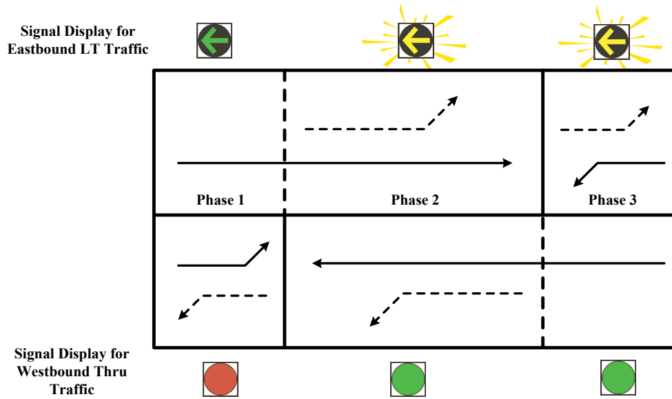
Figure 1-5: Fixed the “Yellow Trap” with FYA
