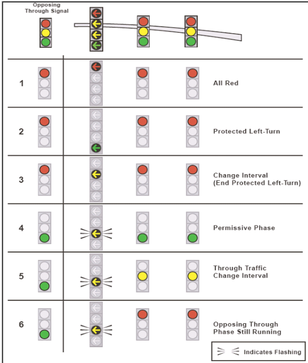
Figure 1-3: FYA Logic Link
