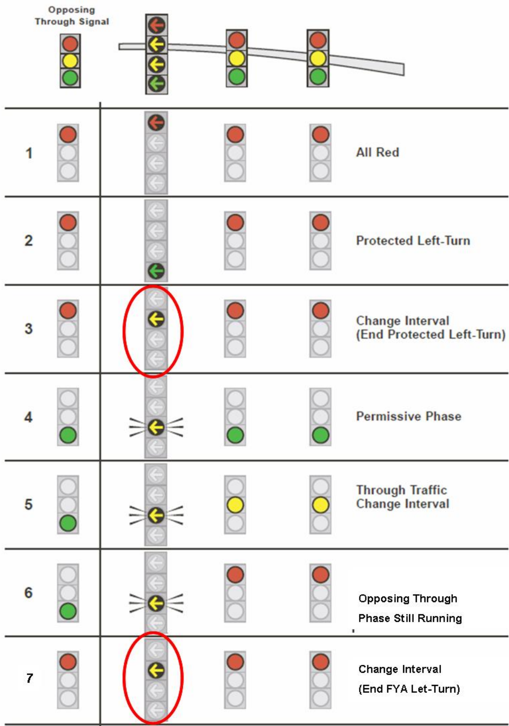
Figure 2-9: Two Meanings of Steady Yellow Arrows
