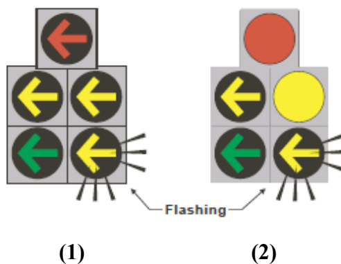
Figure 2-8: Potential FYA Retrofit to Five-Section Cluster Displays (Exclusive Left-Turn Displays)
