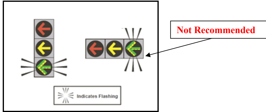
Figure 6-2: Three-Section Signal Face
