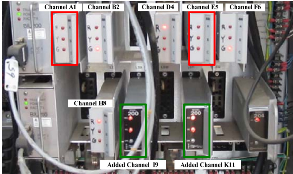
Figure 4-11: Cabinet and Load Switches for Implementation of FYA
