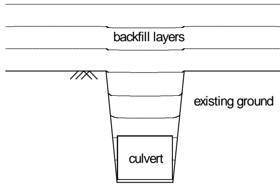
FIGURE 2.2. TRENCH CULVERT
