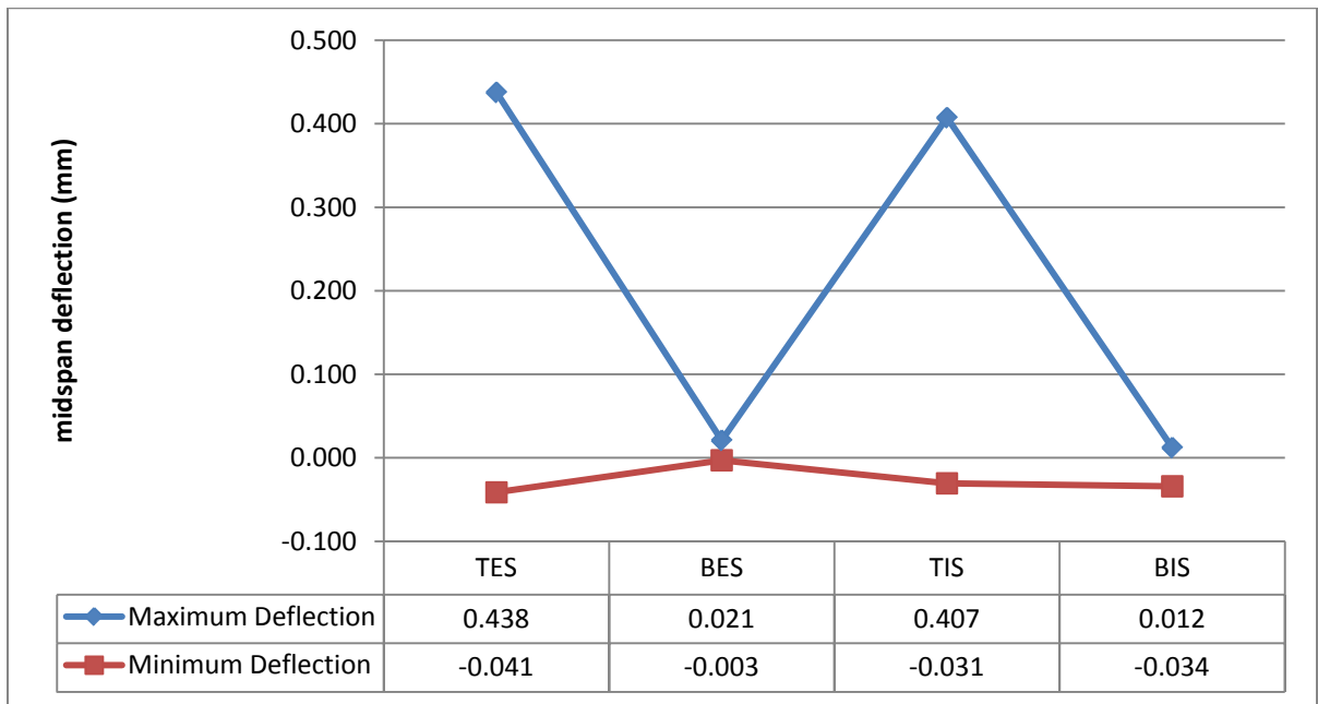
FIGURE 6.20. MEASURED DEFLECTIONS IN MILLIMETERS FOR THE SHALLOWATER CULVERT: 4' OF FILL
