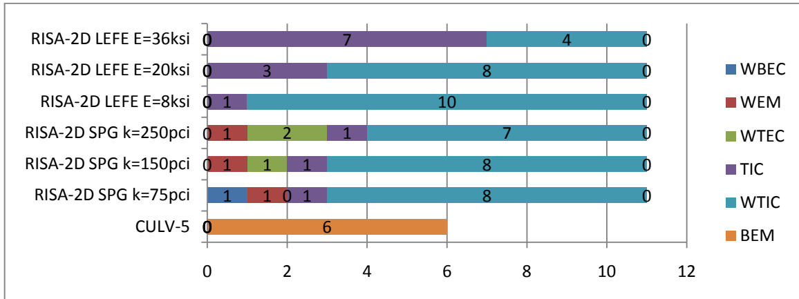
FIGURE 4.41. 1958 ERA 60KSI STEEL CONTROLLING CRITICAL SECTIONS: 2' OF FILL
