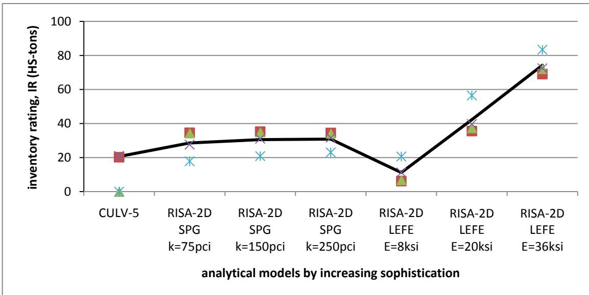
FIGURE 4.21. 1946 ERA INVENTORY RATINGS: FM-MBC-3-26
