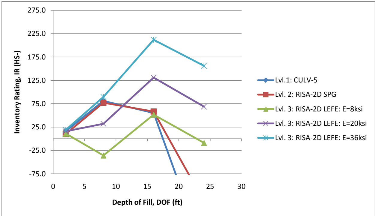
FIGURE 5.7. INVENTORY RATING VS. DEPTH OF FILL FOR MC-7-16 4 7X4W16.
