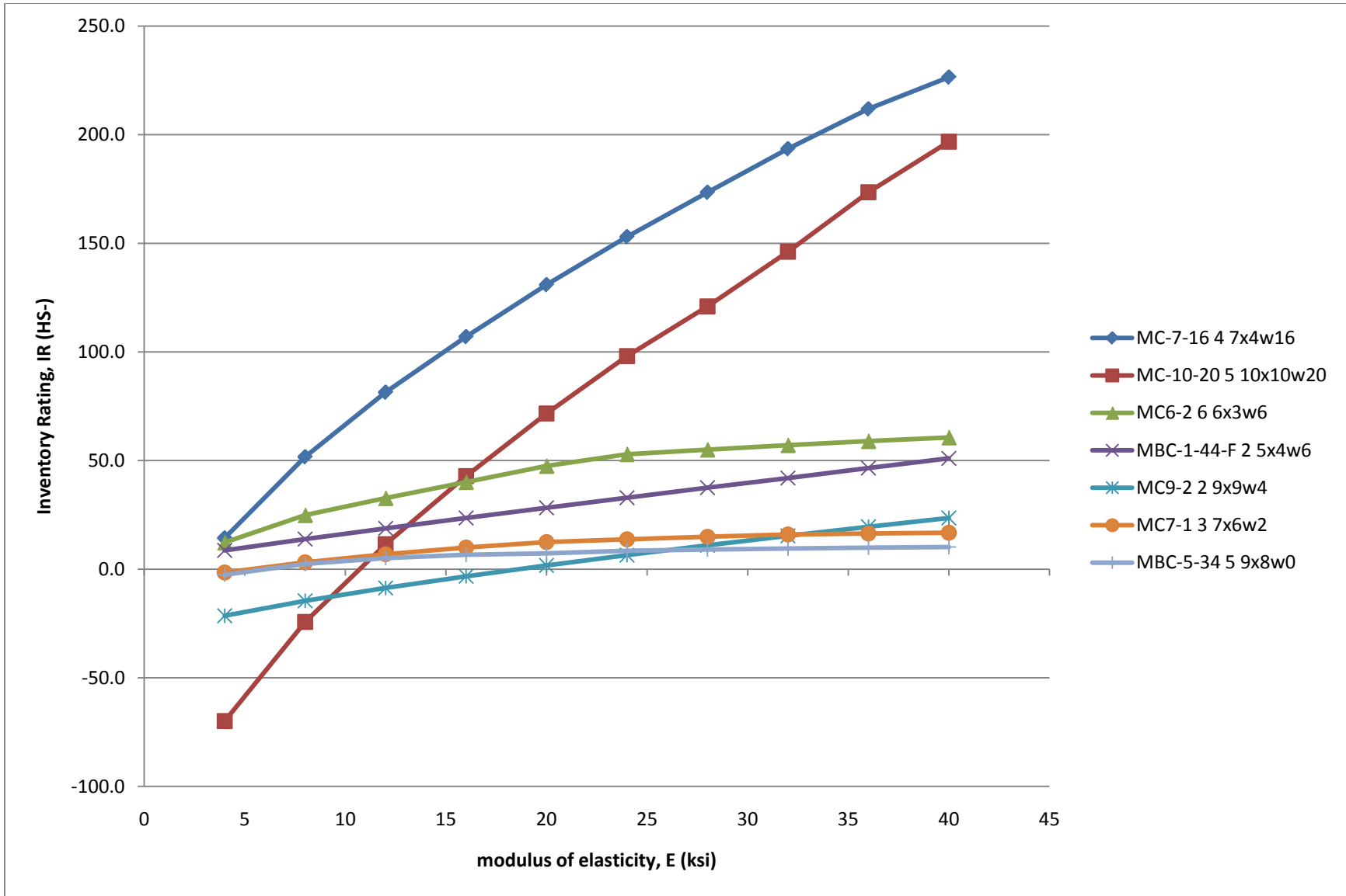
FIGURE 5.6. MODULUS OF ELASTICITY VS. THE INVENTORY RATING FOR SEVEN REPRESENTATIVE CULVERT DESIGNS.
