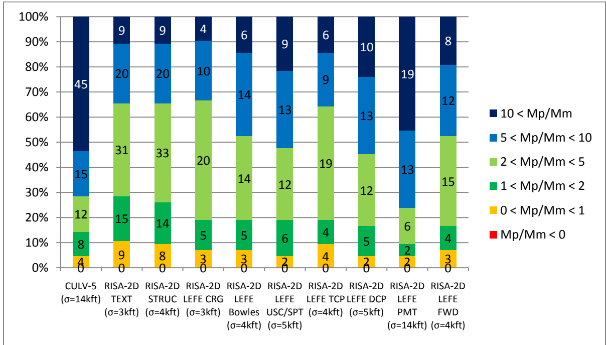
FIGURE 6.26. LIVE LOAD GOODNESS PLOT FOR PLAINVIEW CULVERT: 3.5' OF FILL
