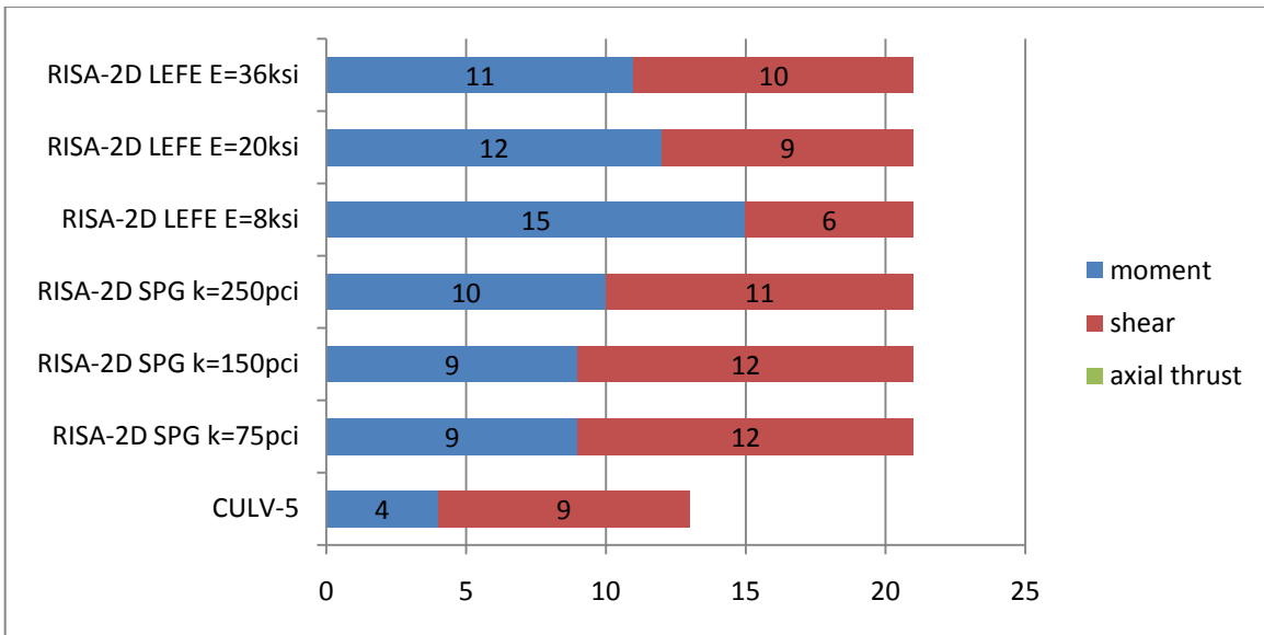
FIGURE 4.49. 2003 ERA CONTROLLING FAILURE MODE
