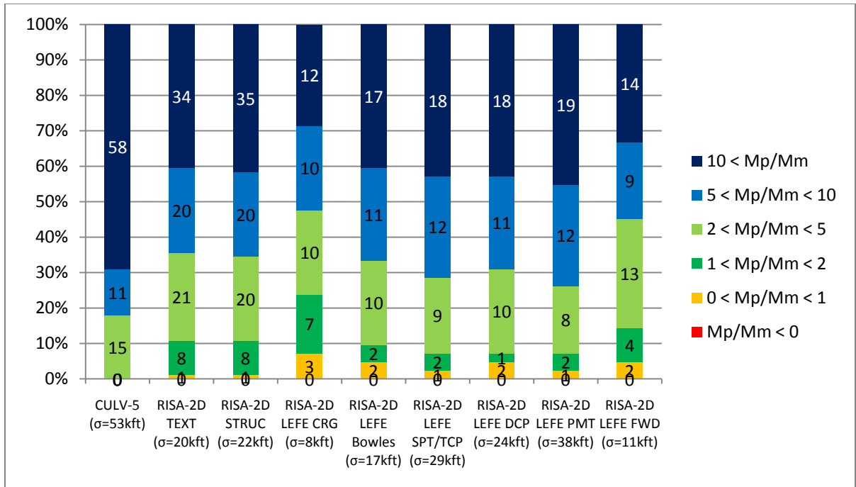
FIGURE 6.12. LIVE LOAD GOODNESS PLOT FOR SHALLOWATER CULVERT: 2' OF FILL
