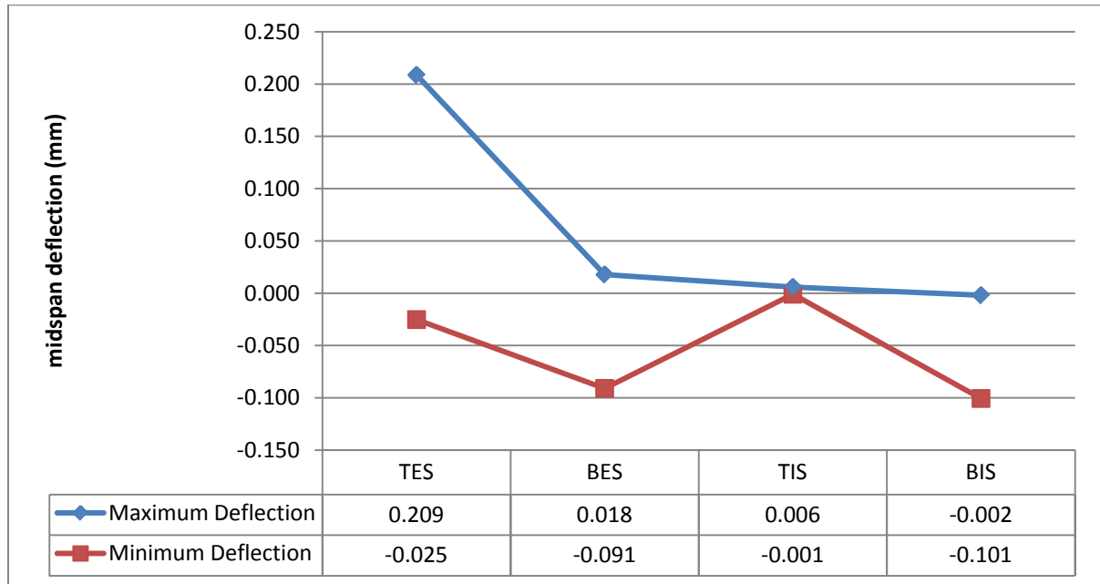
FIGURE 6.36. MEASURED DEFLECTIONS IN MILLIMETERS FOR THE TULIA CULVERT: 1.5' OF FILL
