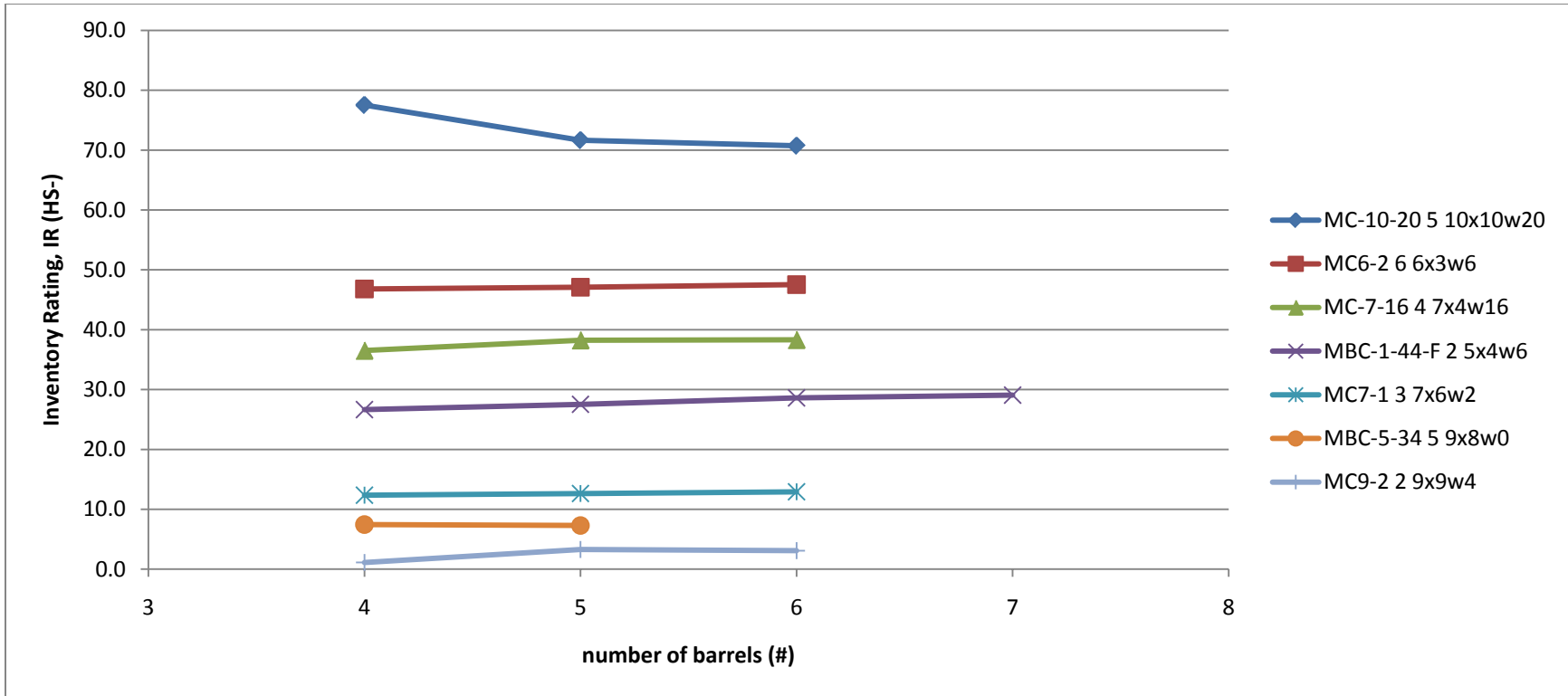
FIGURE 5.3. NUMBER OF BARRELS VS. THE INVENTORY RATING FOR SEVEN REPRESENTATIVE CULVERT DESIGNS.
