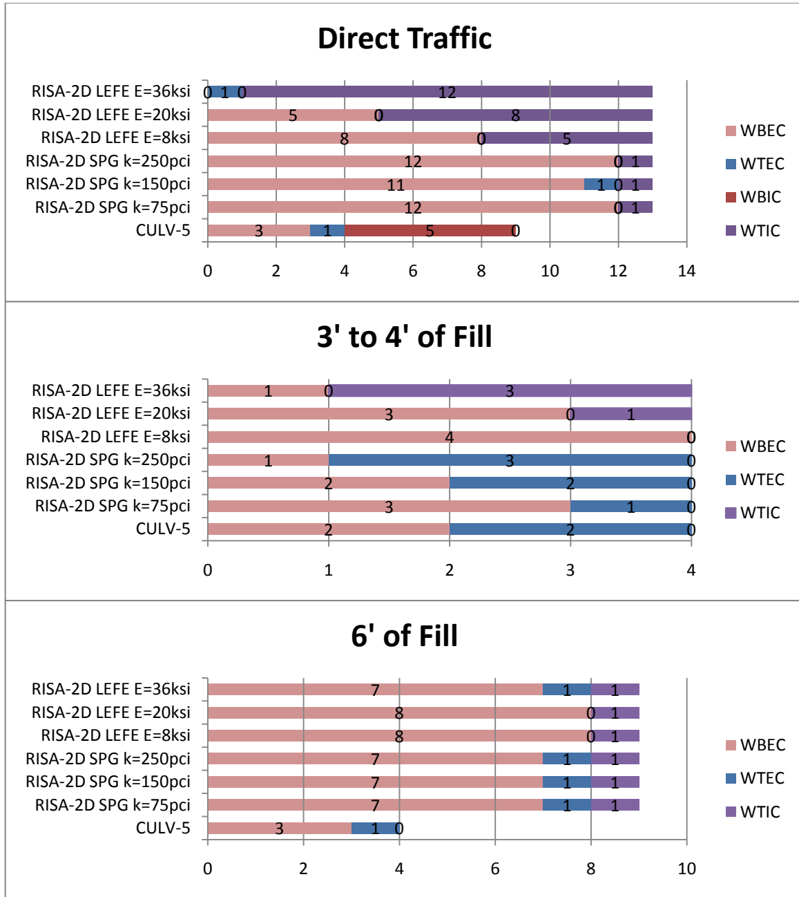
FIGURE 4.15. 1938 ERA CONTROLLING CRITICAL SECTIONS: 0 TO 6' OF FILL
