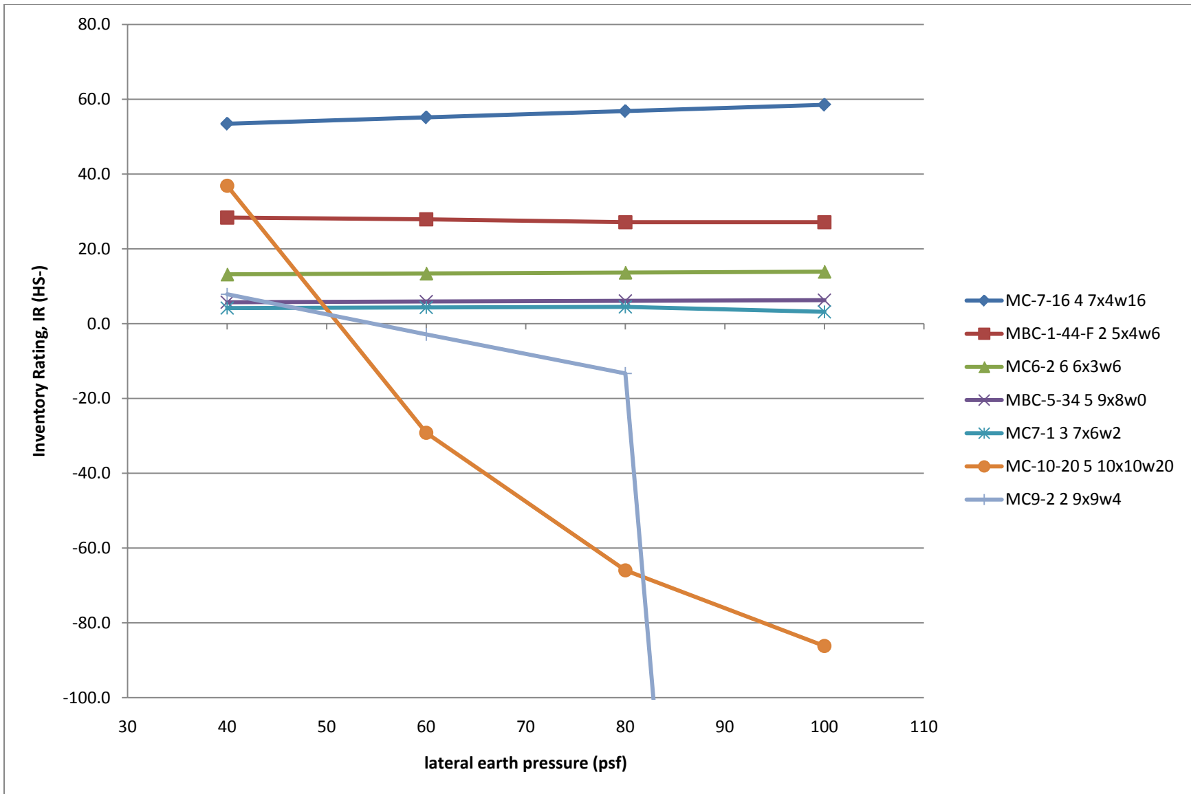
FIGURE 5.4. LATERAL EARTH PRESSURE VS. THE INVENTORY RATING FOR SEVEN REPRESENTATIVE CULVERT DESIGNS USING CULV-5.
