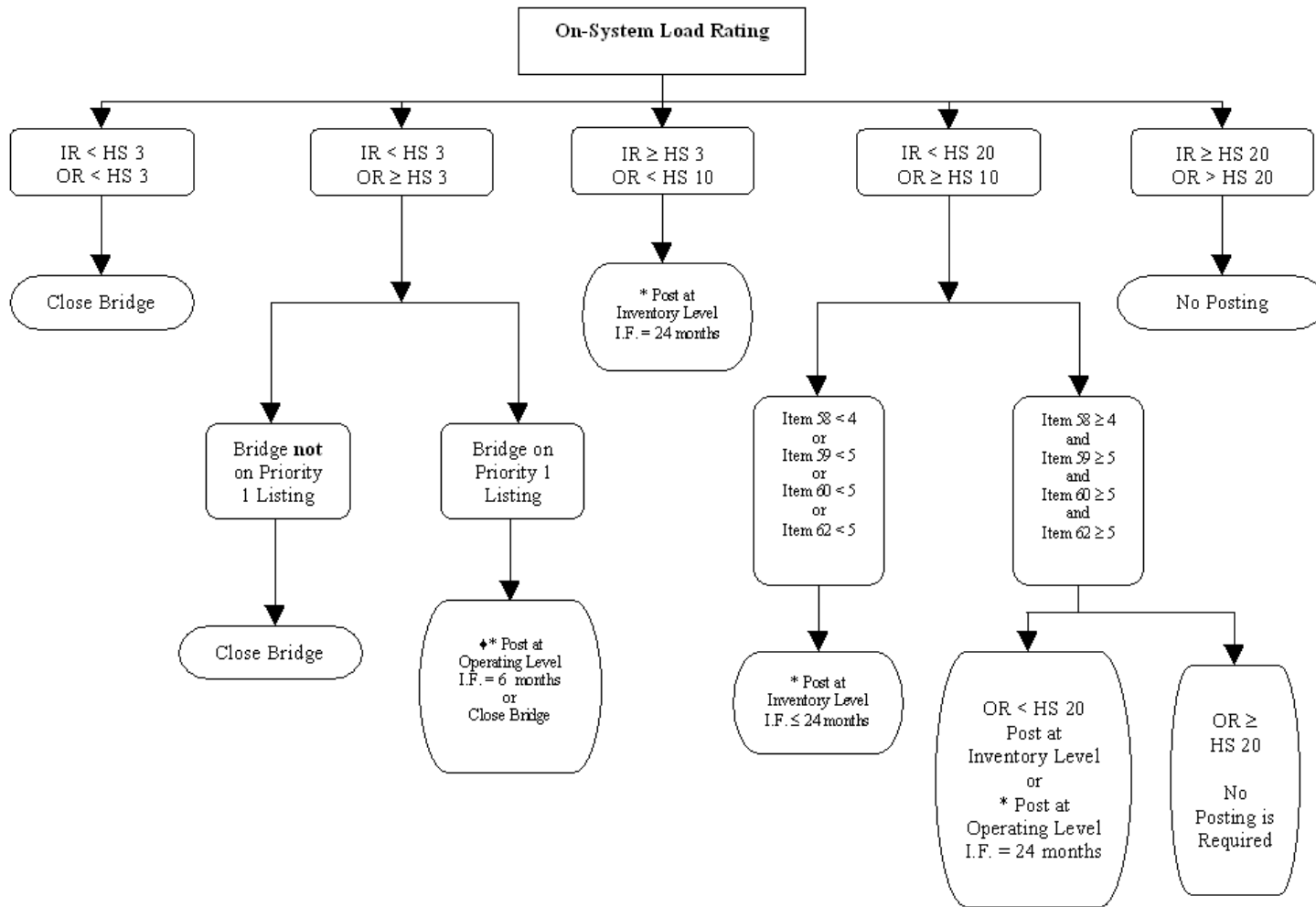
FIGURE 3.1. LOAD POSTING GUIDELINES (TXDOT BRIDGE INSPECTION MANUAL FIG.5-3).
