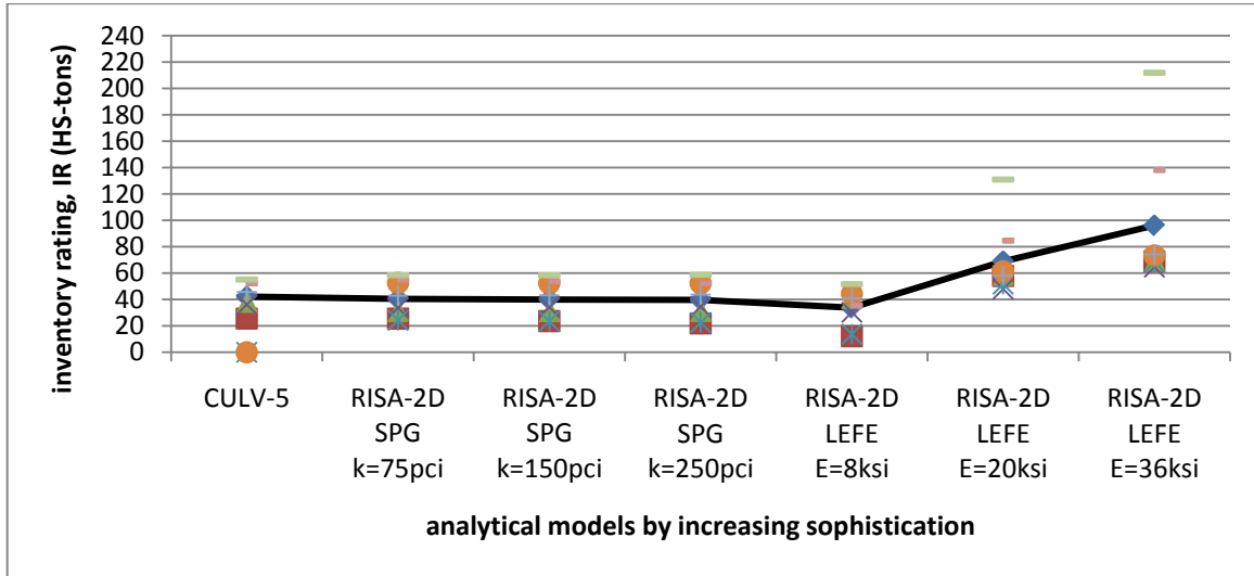
FIGURE 4.46. 2003 ERA INVENTORY RATINGS: 7' TO 16' OF FILL
