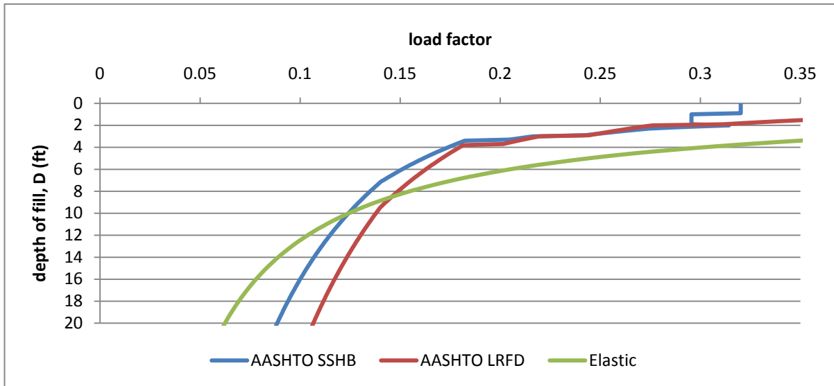
FIGURE 3.9. TWO-DIMENSIONAL FEA COMPARISONS OF LIVE LOADS
