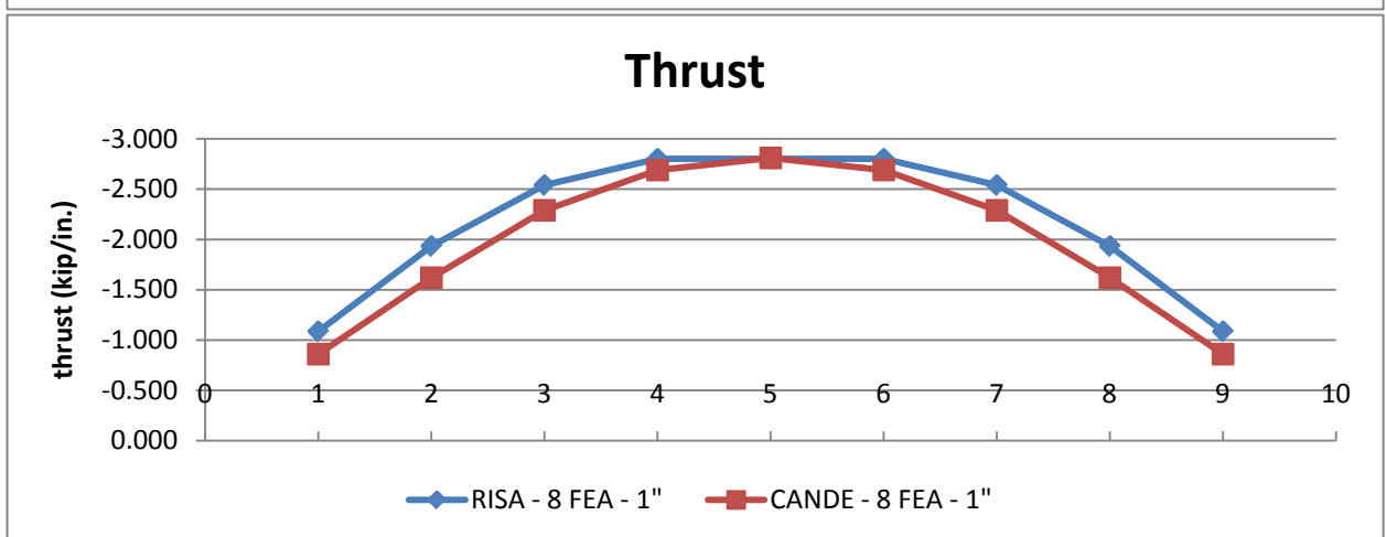
FIGURE 3.10. DEMANDS FROM SIMPLE BEAM MODEL COMPARISON.
