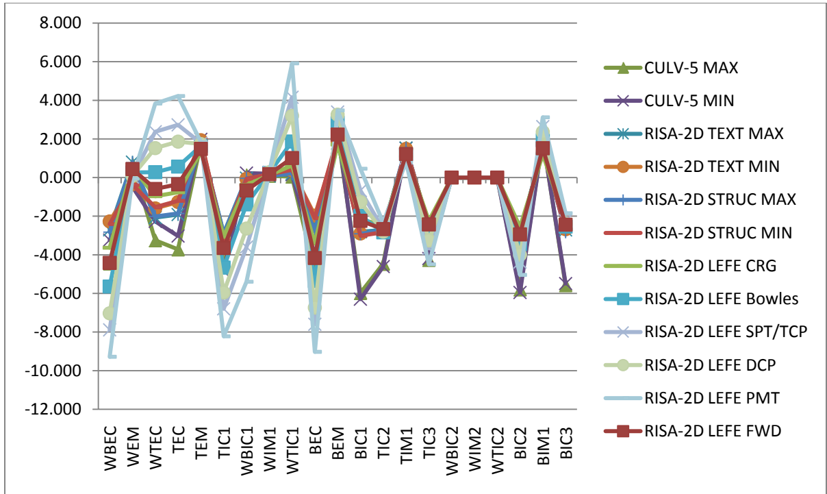
FIGURE 6.11. DEAD LOAD PREDICTED FOR SHALLOWATER CULVERT: 2' OF FILL.
