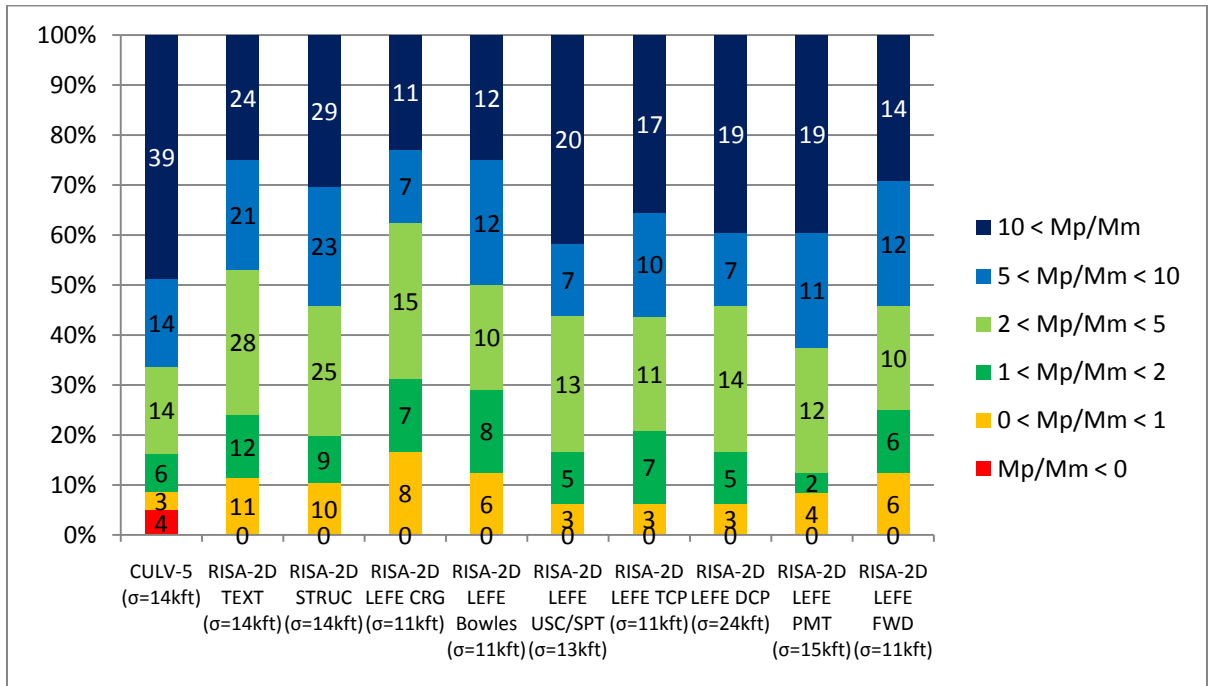
FIGURE 6.34. LIVE LOAD GOODNESS PLOT FOR TULIA CULVERT: 1.5' OF FILL
