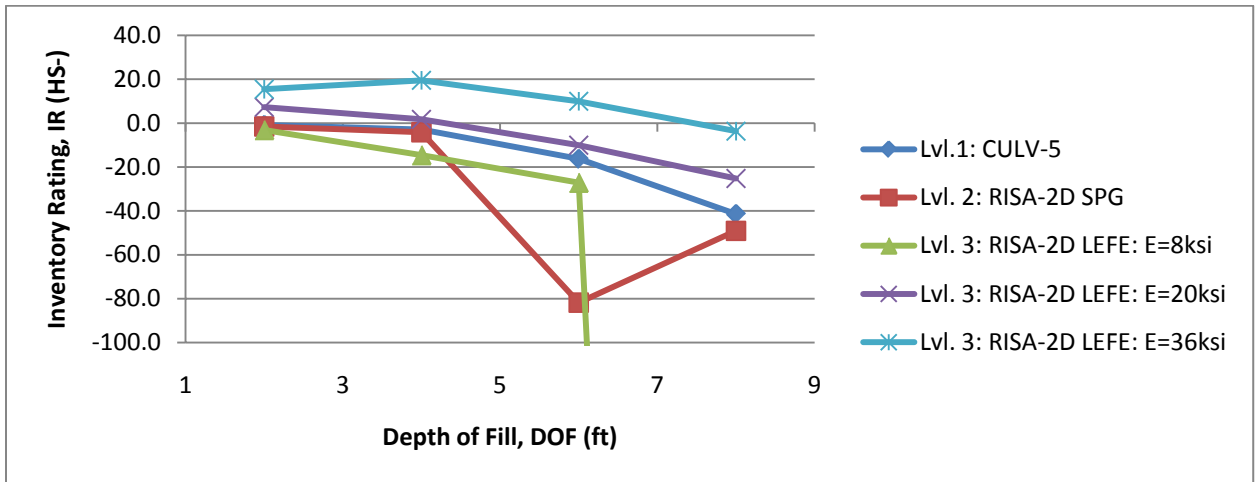
FIGURE 5.10. INVENTORY RATING VS. DEPTH OF FILL FOR MC9-2 2 9X9W4.
