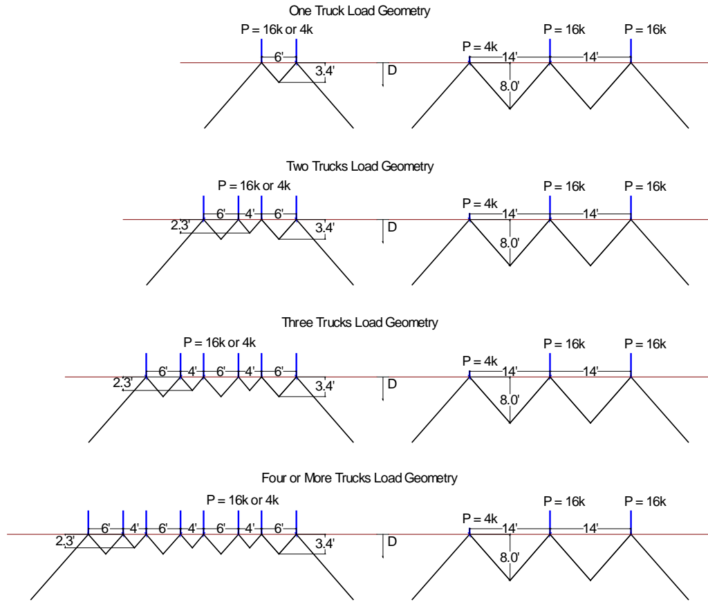
FIGURE 3.6. TWO DIMENSIONAL FRAME LOAD GEOMETRY
