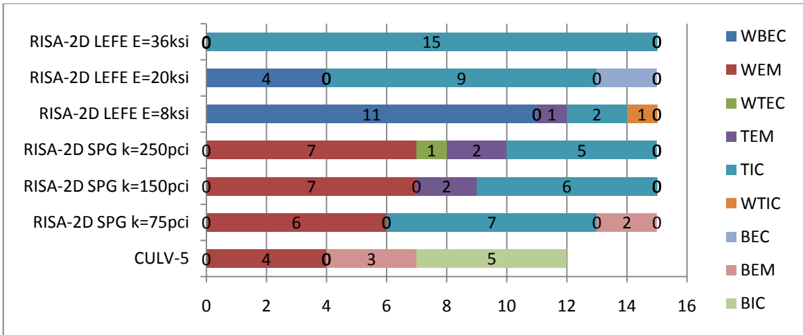
FIGURE 4.43. 1958 ERA 60KSI STEEL CONTROLLING CRITICAL SECTIONS: 6' OF FILL
