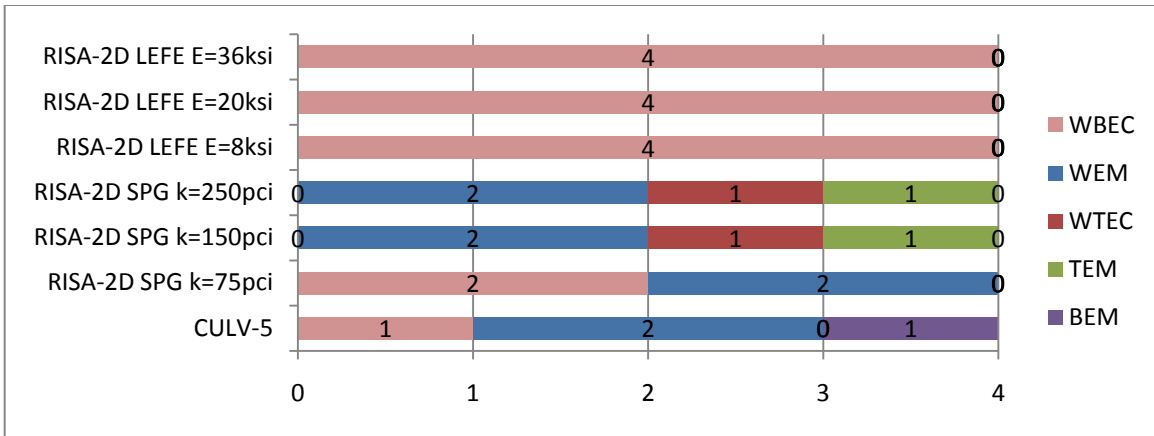
FIGURE 4.24. 1946 ERA CONTROLLING CRITICAL SECTIONS: MC-10-3-45
