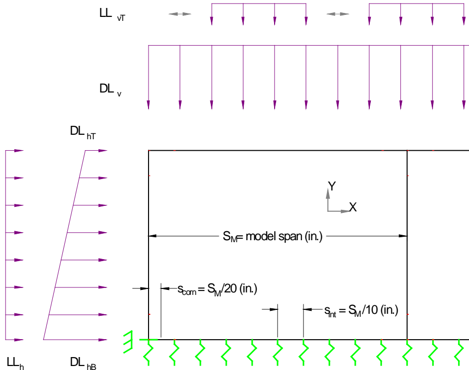
FIGURE 3.4. GENERAL, TWO-DIMENSIONAL, LINEAR-ELASTIC STRUCTURAL FRAME MODELS LOADING DIAGRAM.(TXDOT, 2009)
