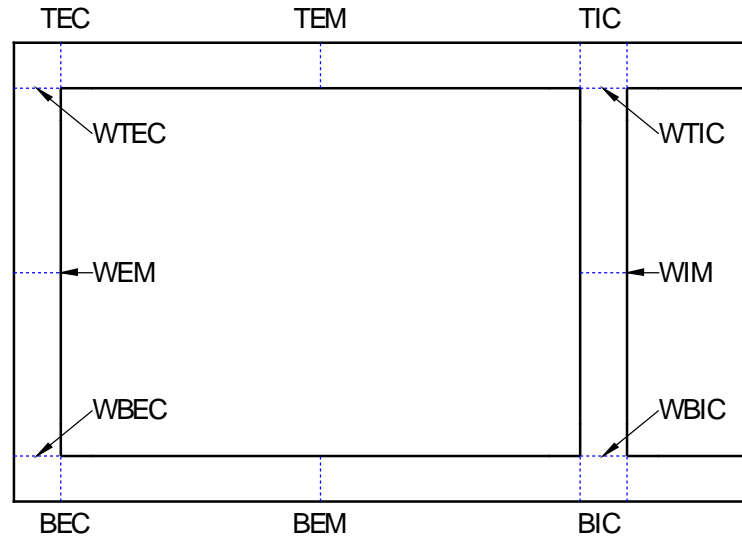
FIGURE 4.7. MOMENT CRITICAL SECTIONS FOR CULVERTS WITHOUT HAUNCHES.
