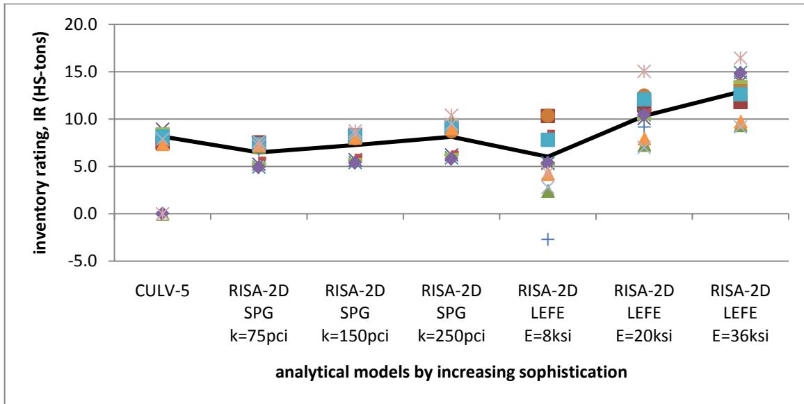
FIGURE 4.10. 1938 ERA INVENTORY RATINGS: DIRECT TRAFFIC
