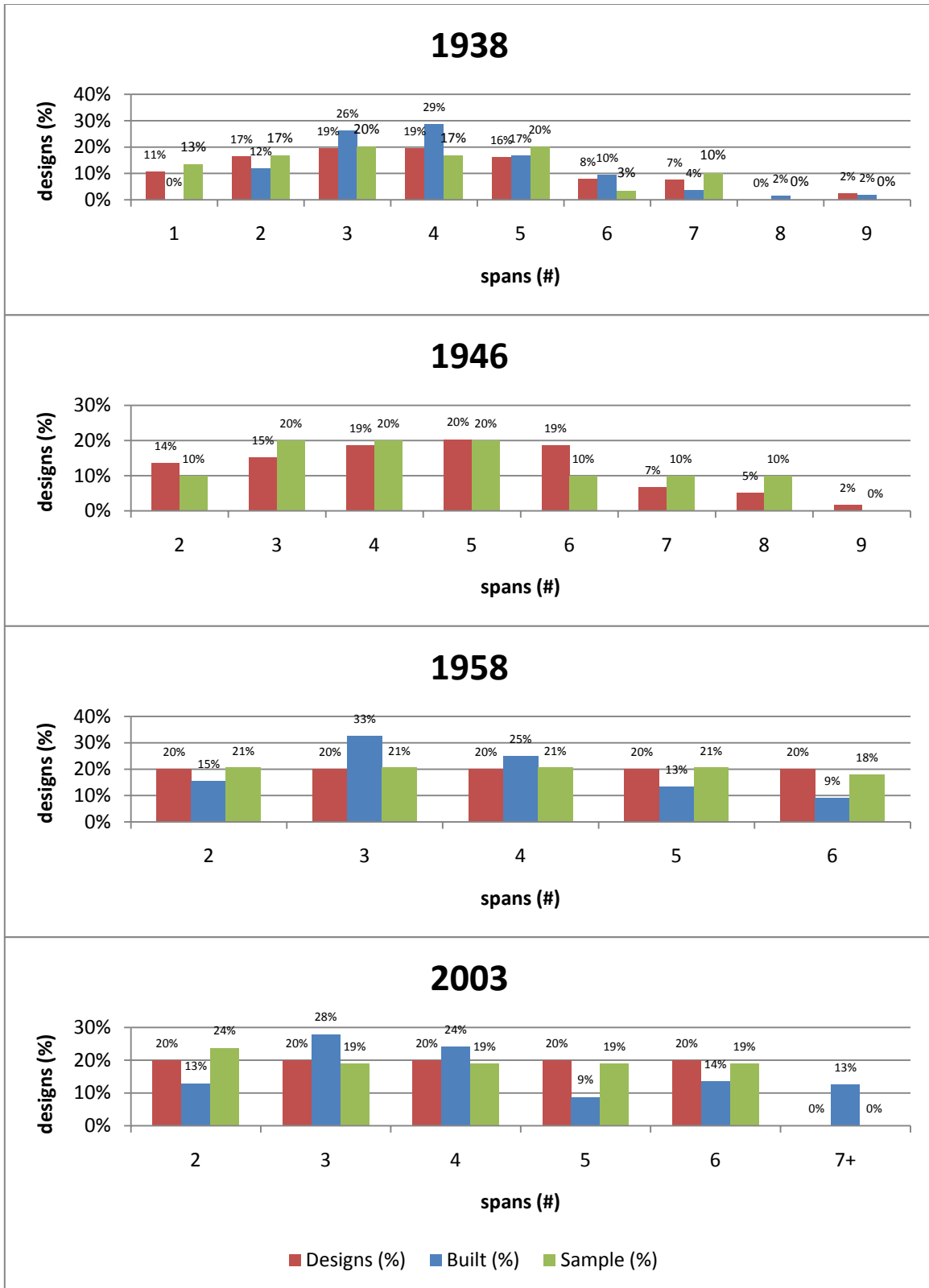
FIGURE 4.3. DISTRIBUTION OF THE NUMBER OF SPANS FOR DESIGNS, BUILT AND SAMPLE POPULATIONS
