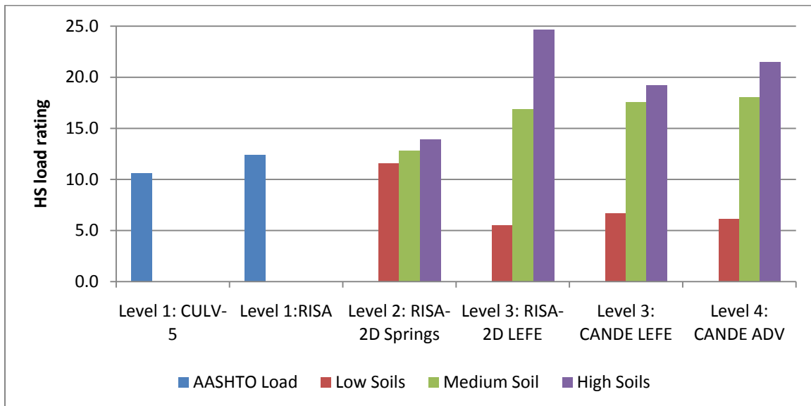
FIGURE 3.11. LOAD RATING COMPARISON OF FULL SCALE CULVERT
