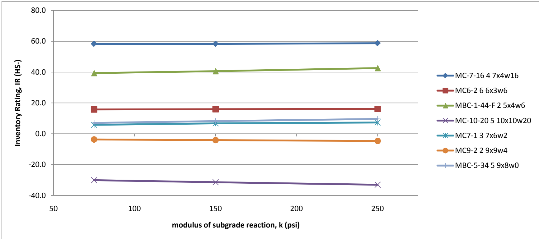
FIGURE 5.1. MODULUS OF SUBGRADE REACTION VS. THE INVENTORY RATING FOR SEVEN REPRESENTATIVE CULVERT DESIGNS.
