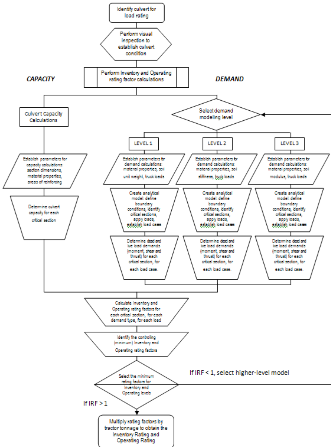
FIGURE 3.2. FLOW CHART DEPICTING THE TXDOT CULVERT LOAD RATING PROCESS.
