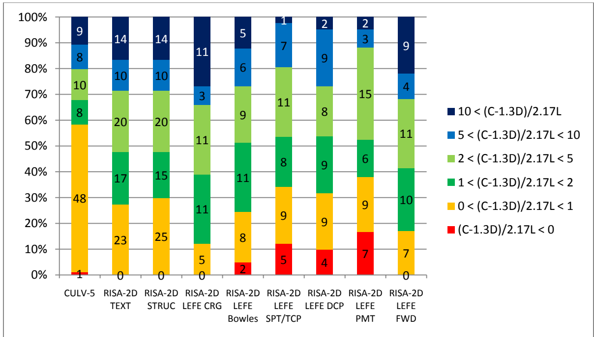
FIGURE 6.13. LOAD RATING GOODNESS PLOT FOR SHALLOWATER CULVERT: 2' OF FILL
