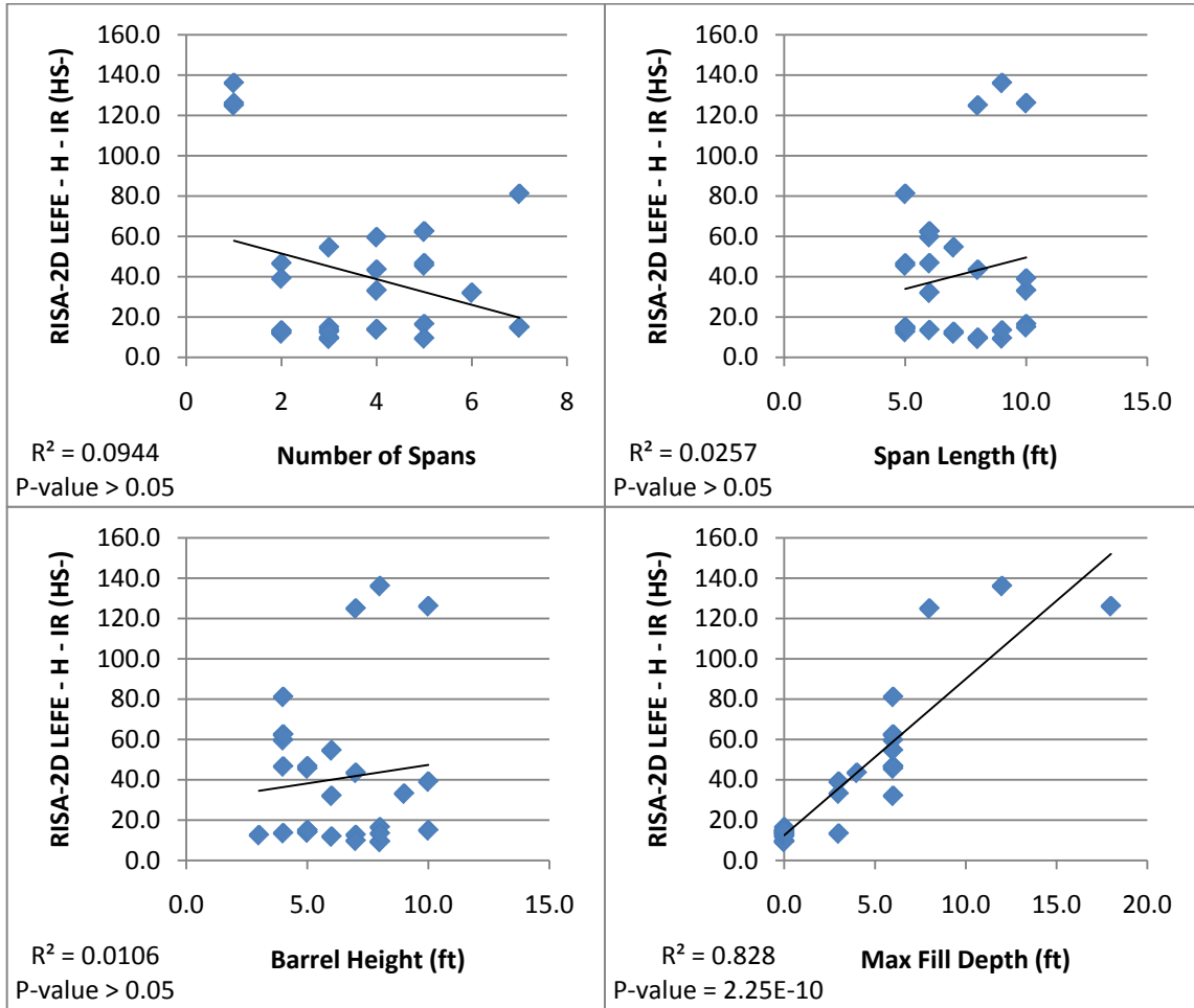
FIGURE 4.9. 1938 ERA STATISTICAL ANALYSIS FOR SIGNIFICANT INDEPENDENT VARIABLES
