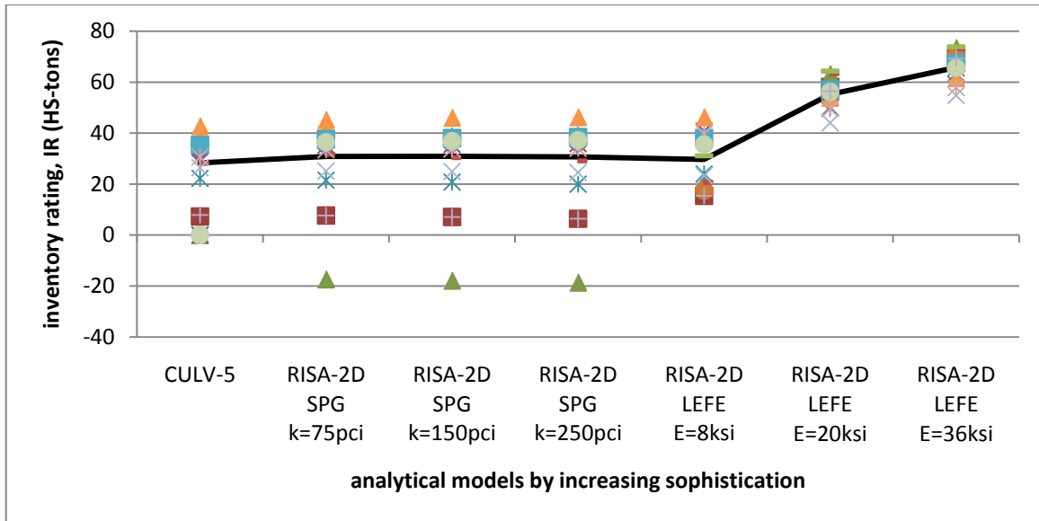
FIGURE 4.39. 1958 ERA 60KSI STEEL INVENTORY RATINGS: 6' OF FILL
