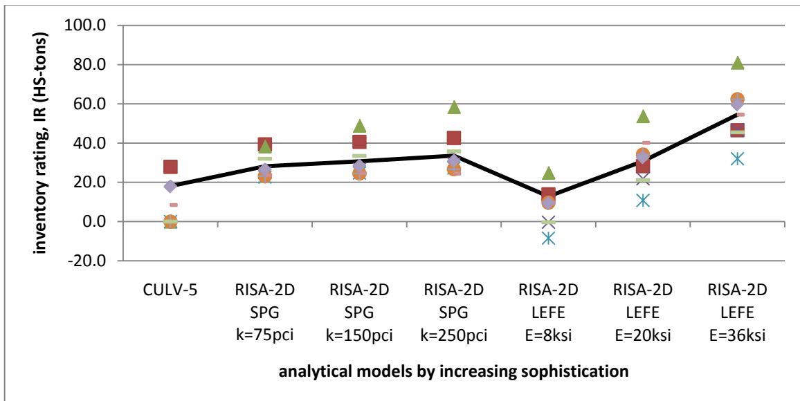
FIGURE 4.12. 1938 ERA INVENTORY RATINGS: 6' OF FILL
