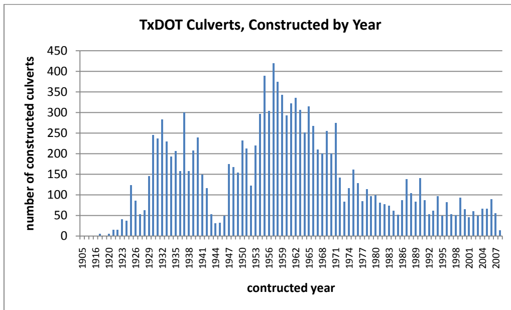
FIGURE 4.1. TXDOT'S AS-BUILT CULVERT POPULATION
