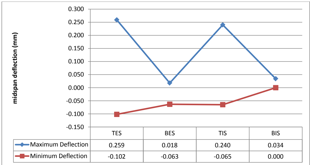
FIGURE 6.28. MEASURED DEFLECTIONS IN MILLIMETERS FOR THE PLAINVIEW CULVERT: 3.5' OF FILL
