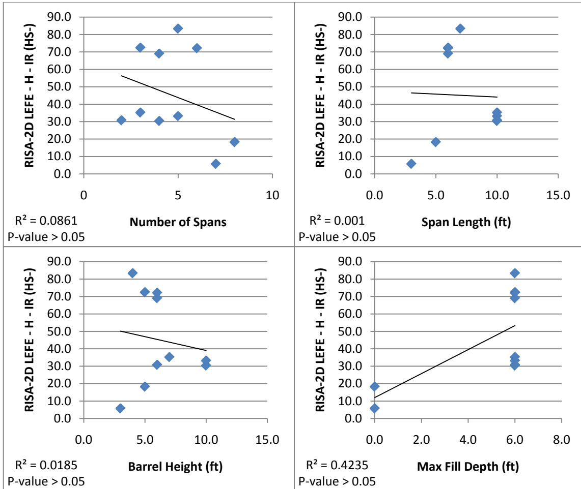
FIGURE 4.18. 1946 ERA STATISTICAL ANALYSIS FOR SIGNIFICANT INDEPENDENT VARIABLES
