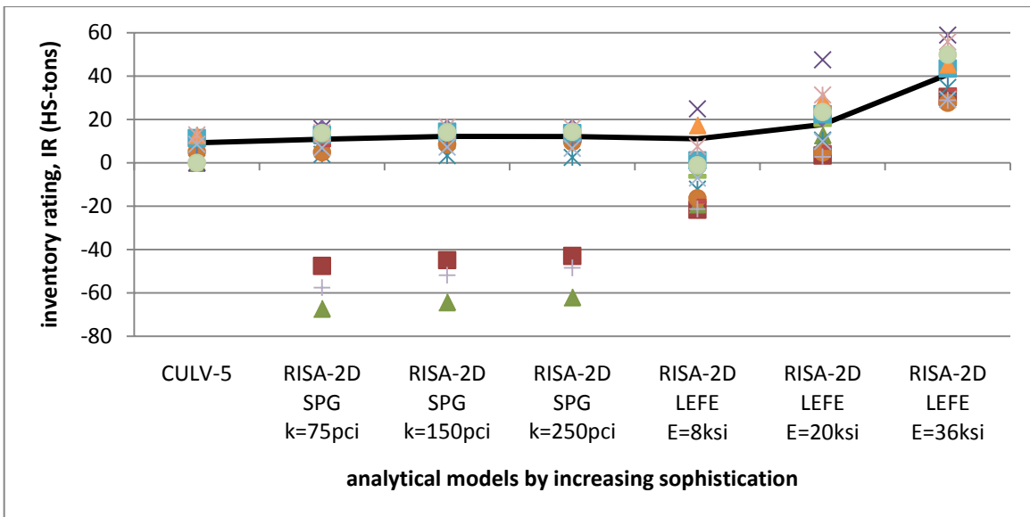
FIGURE 4.30. 1958 ERA 36KSI STEEL INVENTORY RATING: 6' OF FILL
