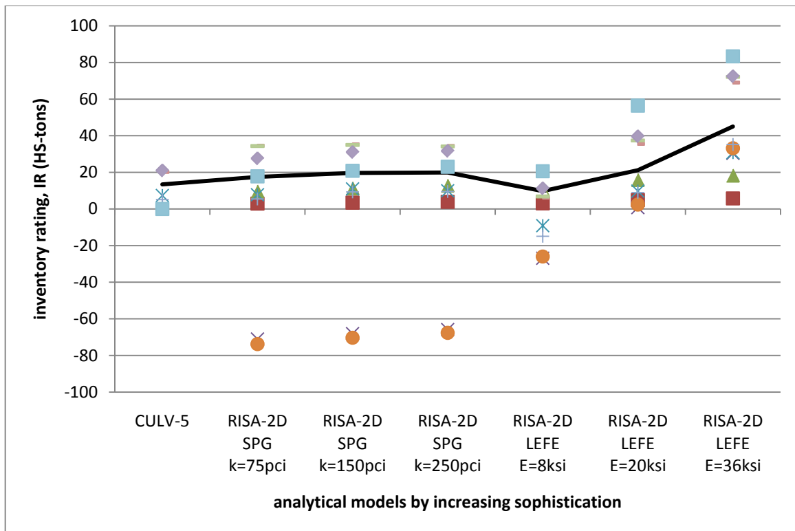
FIGURE 4.17. 1946 ERA INVENTORY RATINGS: UNDIFFERENTIATED
