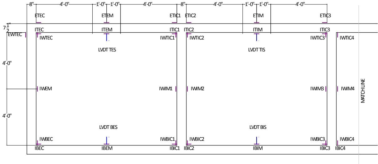
FIGURE 6.8. SHALLOWATER INSTRUMENTATION PLAN.
