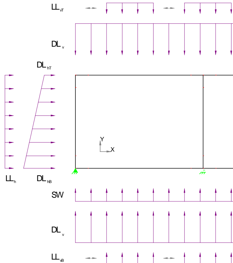
FIGURE 3.3. PREPACKAGED, TWO-DIMENSIONAL CULVERT MODELS LOADING DIAGRAM. (TXDOT, 2009).
