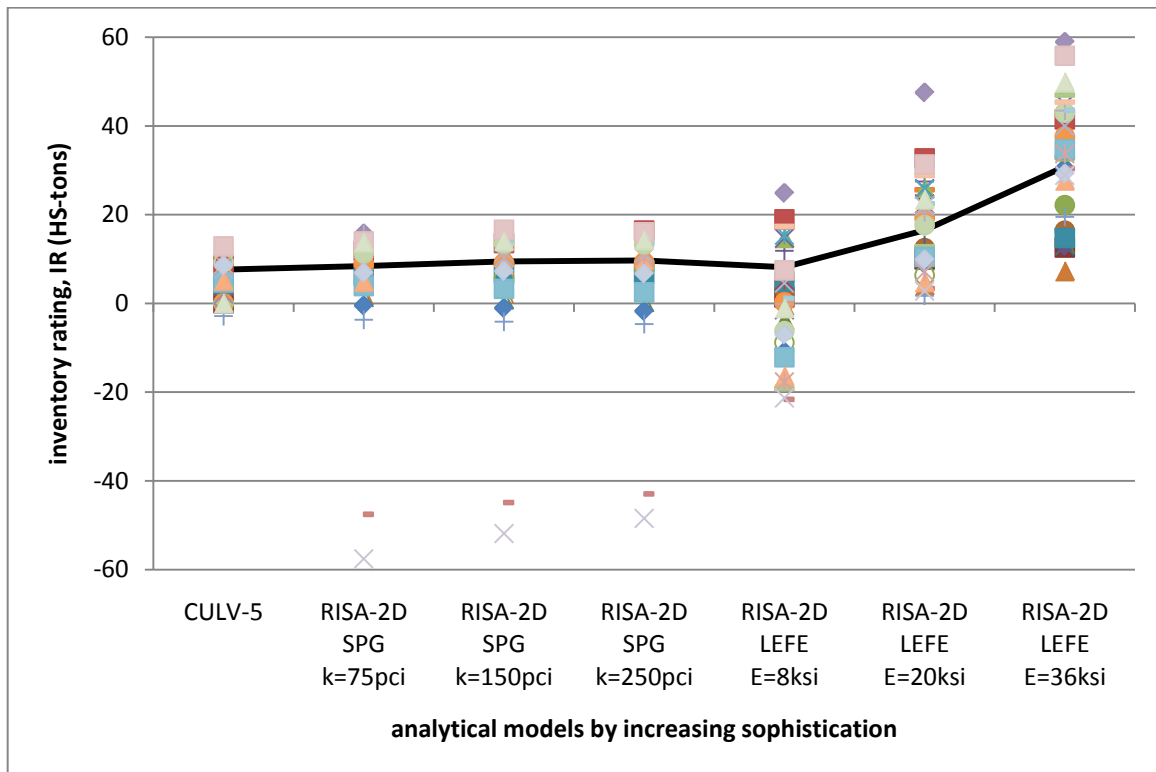
FIGURE 4.26. 1958 ERA 36KSI STEEL INVENTORY RATINGS: UNDIFFERENTIATED
