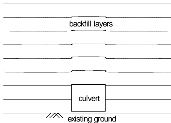
FIGURE 2.1. EMBANKMENT CULVERT
