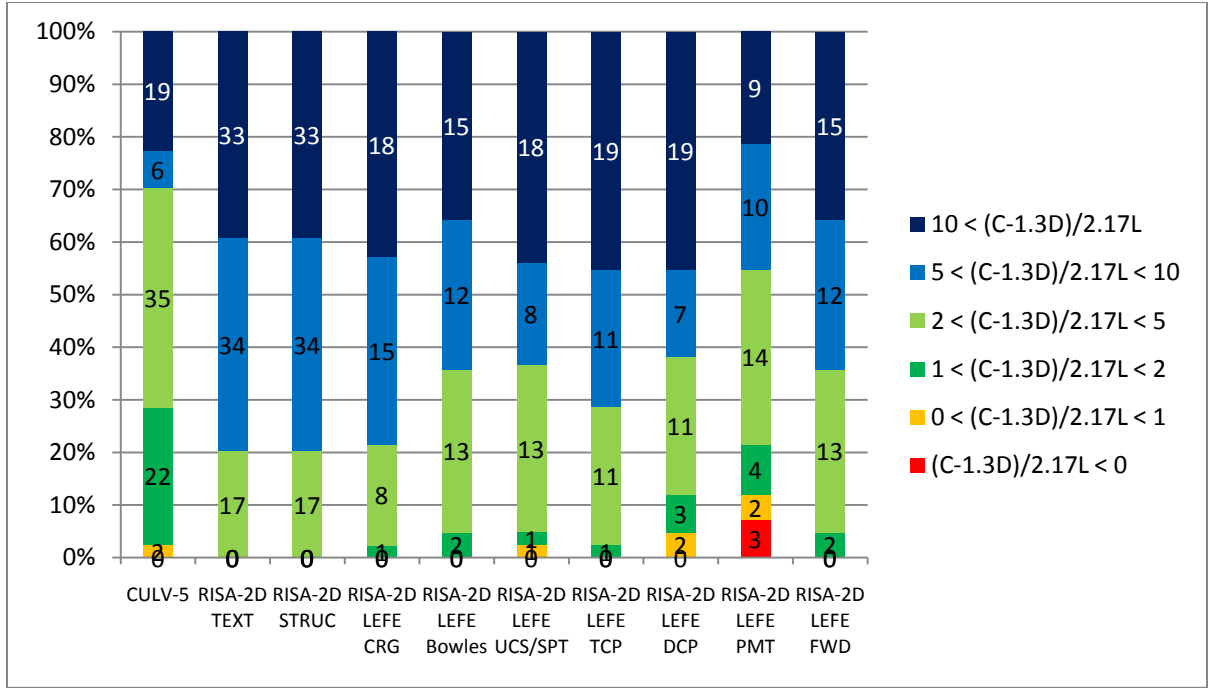
FIGURE 6.27. LOAD RATING GOODNESS PLOT FOR PLAINVIEW CULVERT: 3.5' OF FILL
