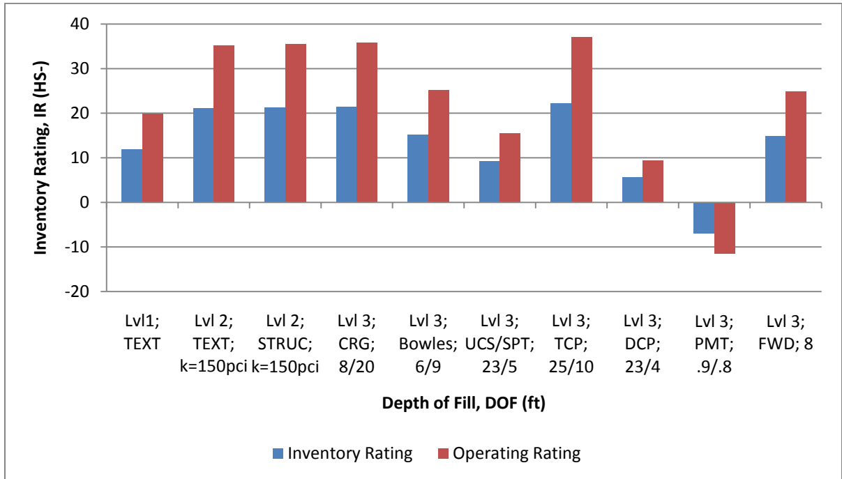
FIGURE 6.23. LOAD RATING FOR PLAINVIEW CULVERT: 3.5' OF FILL
