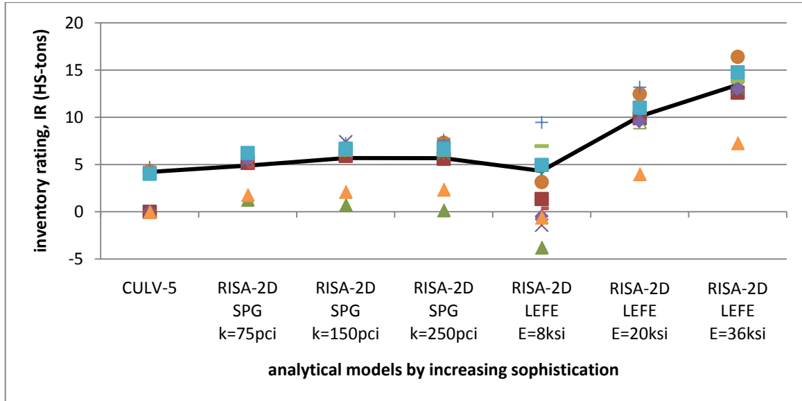
FIGURE 4.28. 1958 ERA 36KSI STEEL INVENTORY RATINGS: 2' OF FILL
