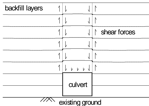
FIGURE 2.4. NEGATIVE SOIL ARCHING
