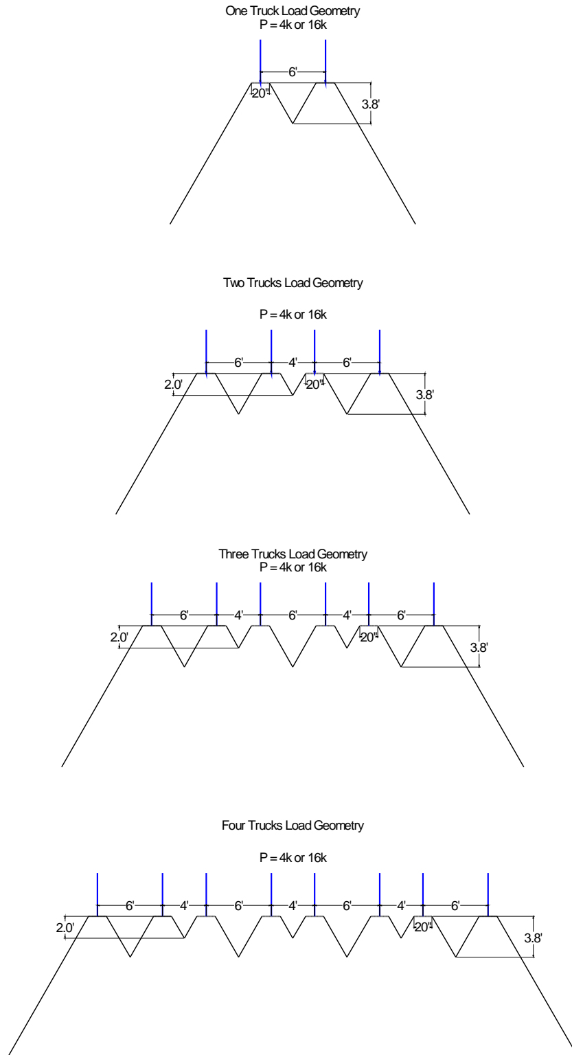
FIGURE 3.8. TWO DIMENSIONAL FINITE ELEMENT AASHTO LRFD LIVE LOAD GEOMETRY
