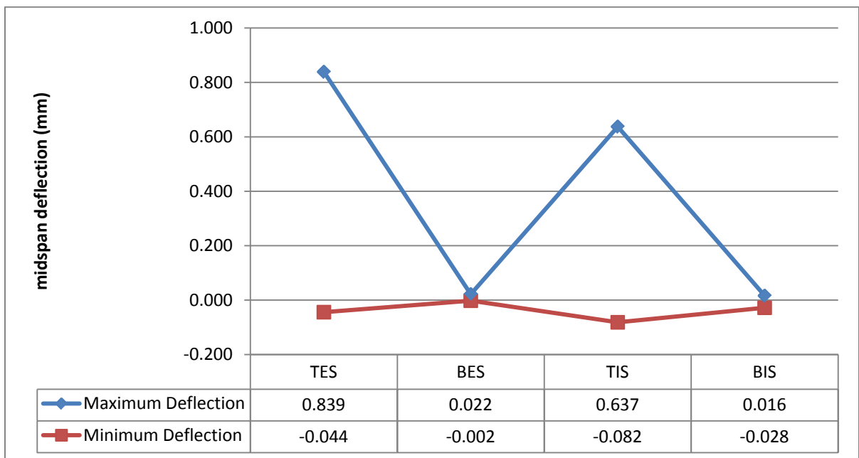
FIGURE 6.14. MEASURED DEFLECTIONS IN MILLIMETERS FOR THE SHALLOWATER CULVERT: 2' OF FILL
