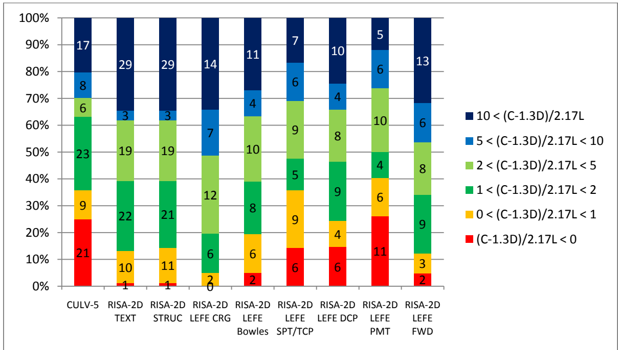
FIGURE 6.19. LOAD RATING GOODNESS PLOT FOR SHALLOWATER CULVERT: 4' OF FILL
