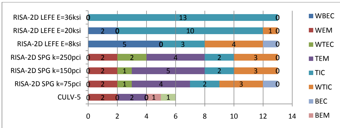
FIGURE 4.42. 1958 ERA 60KSI STEEL CONTROLLING CRITICAL SECTIONS: 4' OF FILL
