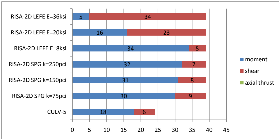
FIGURE 4.40. 1958 ERA 60KSI STEEL CONTROLLING FAILURE MODES
