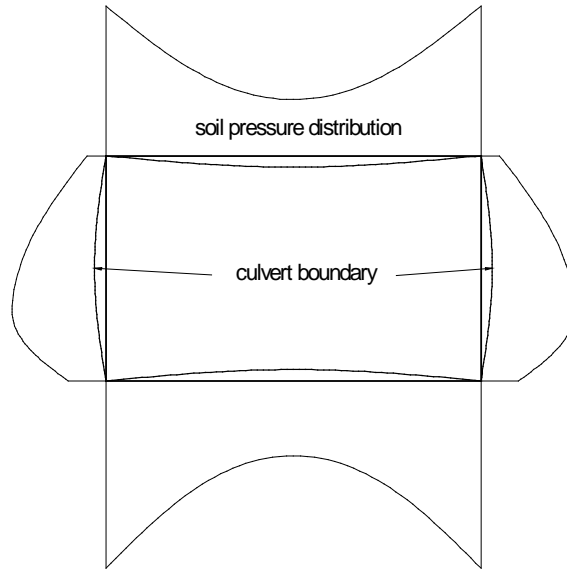
FIGURE 2.6. SOIL PRESSURE DISTRIBUTIONS DUE TO CULVERT DEFORMATION(DASGUPTA & SENGUPTA, 1991)
