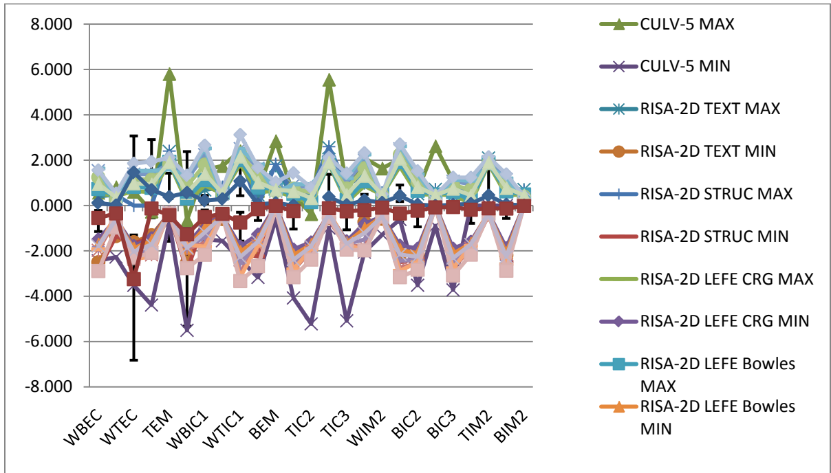
FIGURE 6.32. LIVE LOAD MOMENTS PREDICTED AND MEASURED FOR TULIA CULVERT: 1.5' OF FILL.
