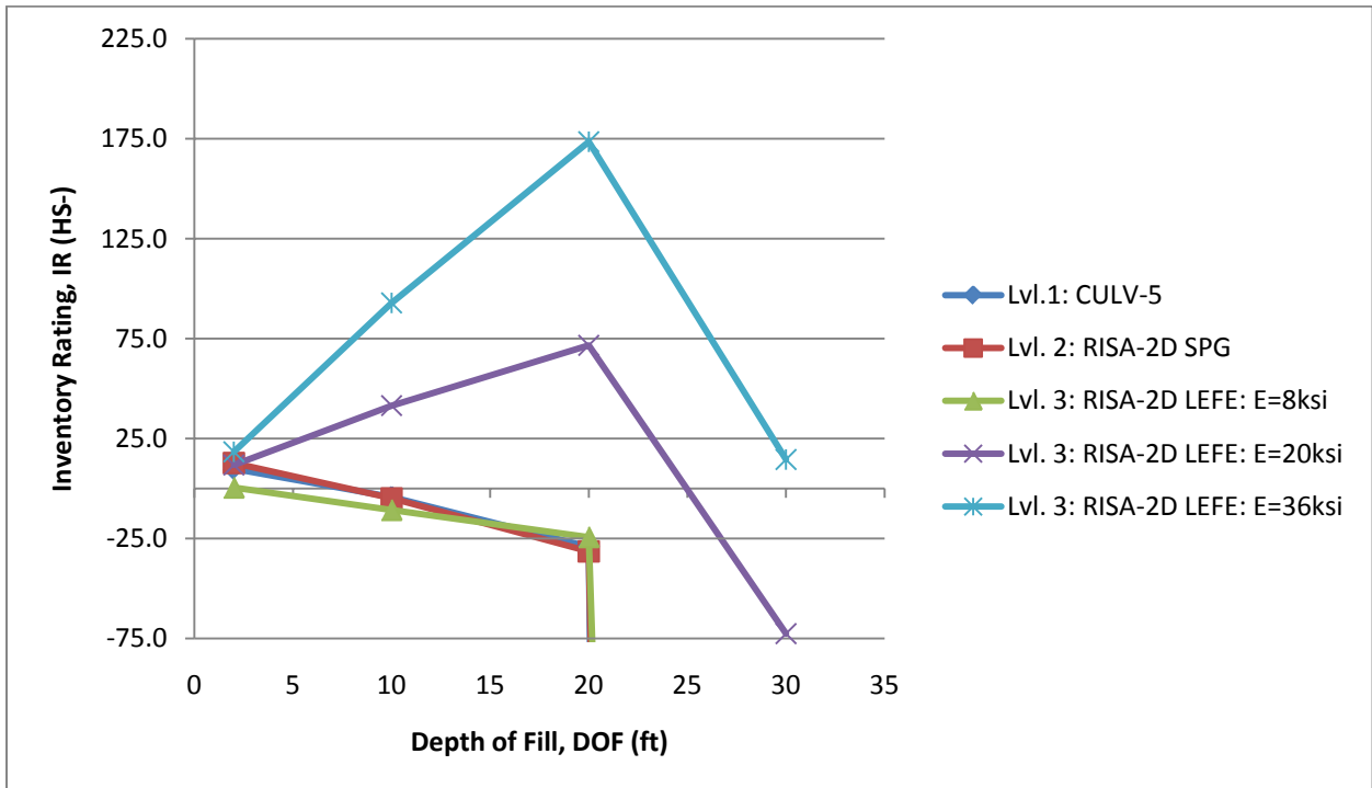
FIGURE 5.8. INVENTORY RATING VS. DEPTH OF FILL FOR MC-10-20 5 10X10W20.
