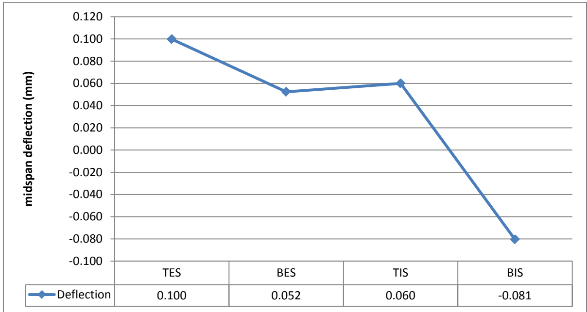
FIGURE 6.39. MEASURED DEFLECTIONS IN MILLIMETERS FOR THE SHALLOW WATER CULVERT FROM 2' TO 4' OF FILL
