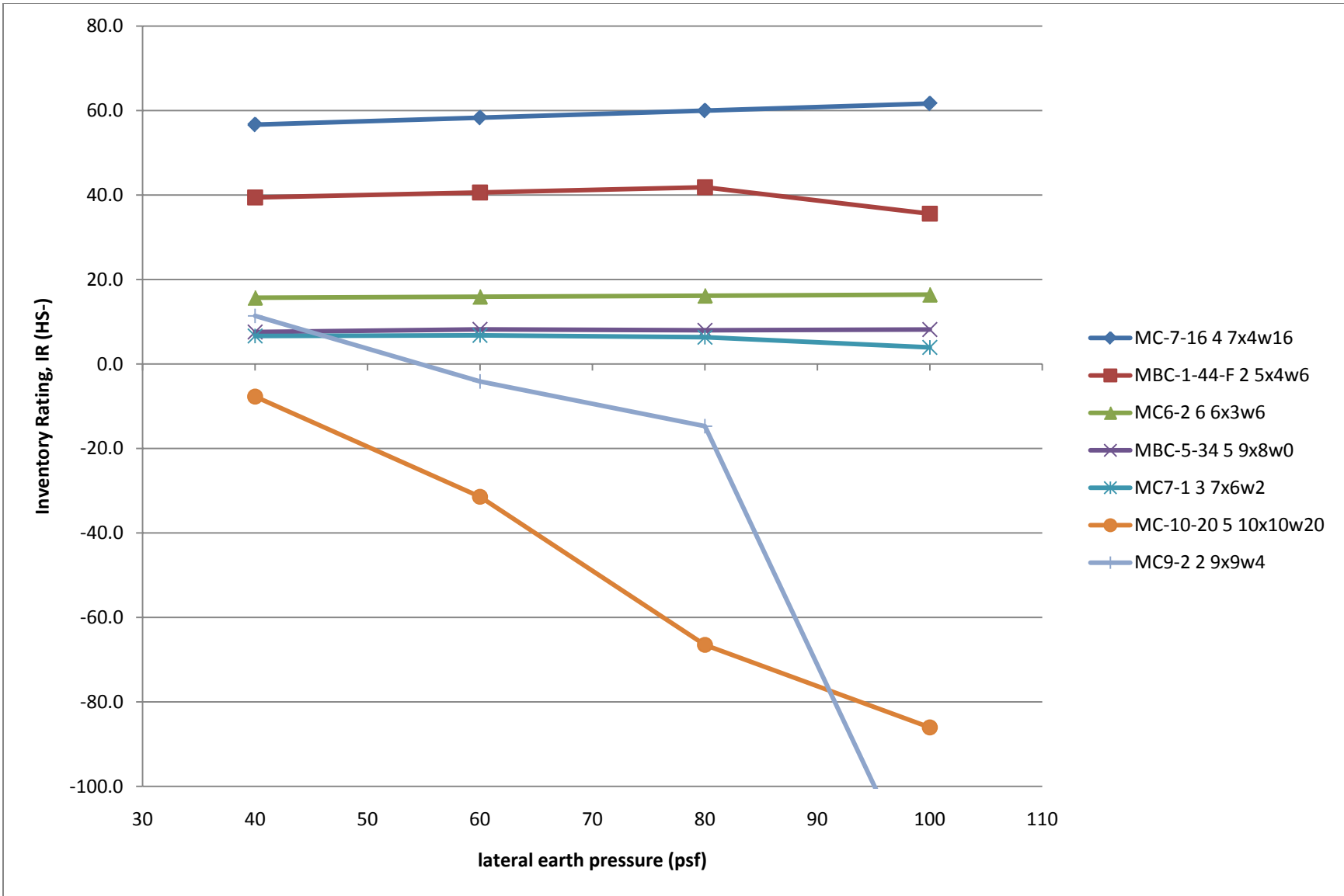
FIGURE 5.5. LATERAL EARTH PRESSURE VS. INVENTORY RATING FOR SEVEN REPRESENTATIVE CULVERT DESIGNS USING RISA-2D.MODULUS OF ELASTICITY, E
