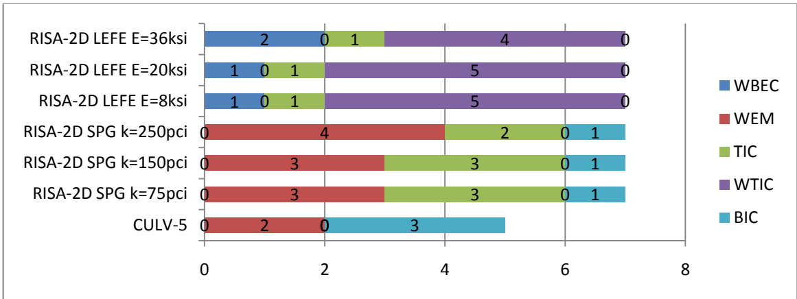
FIGURE 4.52. 2003 ERA CONTROLLING CRITICAL SECTIONS: 23' OF FILL
