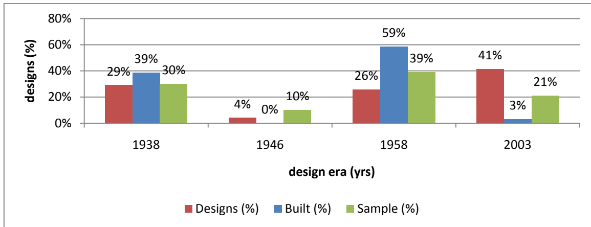
FIGURE 4.2. CULVERT DESIGNS VS BUILT VS SAMPLE BY DESIGN ERA
