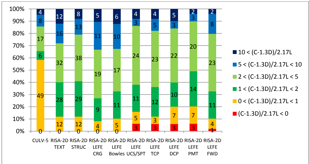
FIGURE 6.35. LOAD RATING GOODNESS PLOT FOR TULIA CULVERT: 1.5' OF FILL
