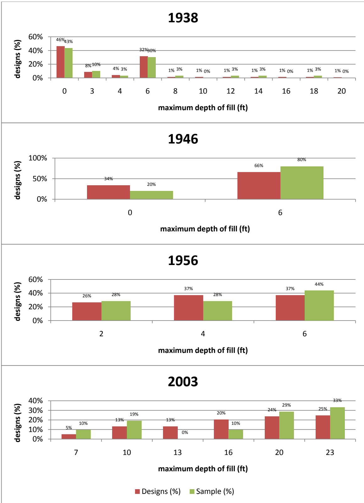
FIGURE 4.6. DISTRIBUTION OF MAXIMUM DEPTH OF FILL FOR DESIGNS AND SAMPLE POPULATIONS
