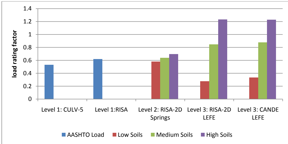
FIGURE 3.12. MOMENT RATING OF FULL SCALE CULVERT
