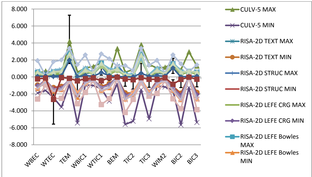
FIGURE 6.24. LIVE LOAD MOMENTS PREDICTED AND MEASURED FOR PLAINVIEW CULVERT: 3.5' OF FILL.
