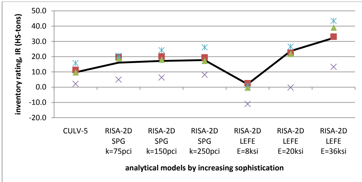
FIGURE 4.11. 1938 ERA INVENTORY RATINGS: 3' AND 4' OF FILL
