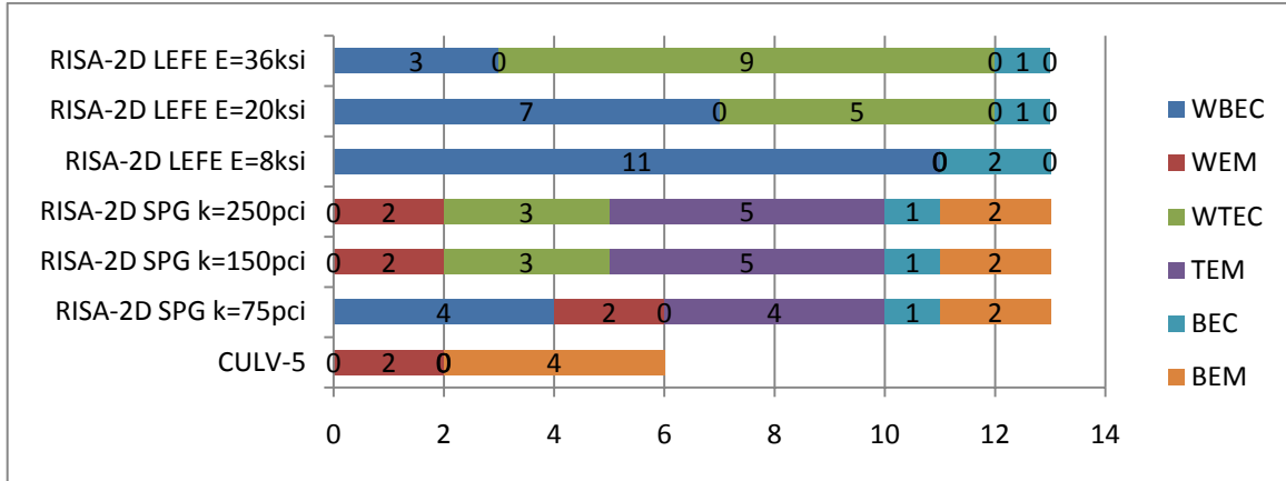
FIGURE 4.33. 1958 ERA 36KSI STEEL CONTROLLING CRITICAL SECTIONS: 4' OF FILL
