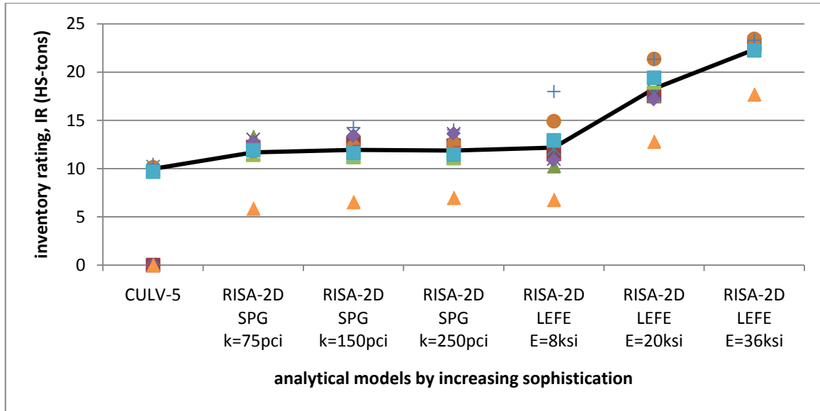
FIGURE 4.37. 1958 ERA 60KSI STEEL INVENTORY RATINGS: 2' OF FILL
