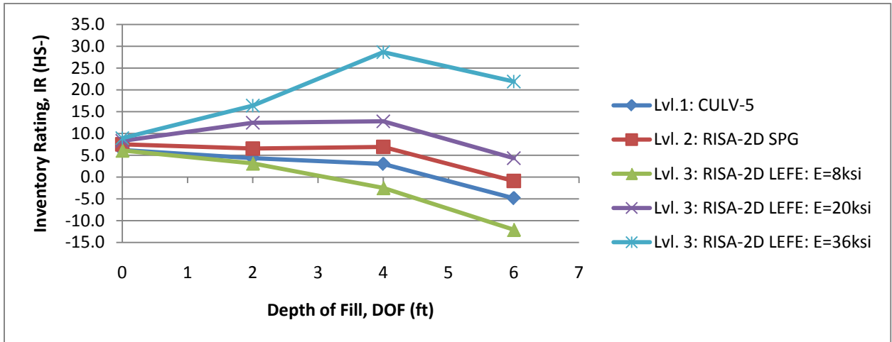
FIGURE 5.9. INVENTORY RATING VS. DEPTH OF FILL FOR MC7-1 3 7X6W2.
