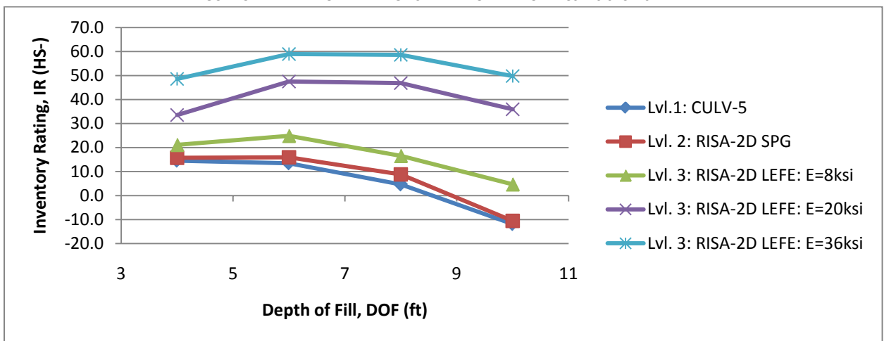
FIGURE 5.11. INVENTORY RATING VS. DEPTH OF FILL FOR MC6-2 6 6X3W6.
