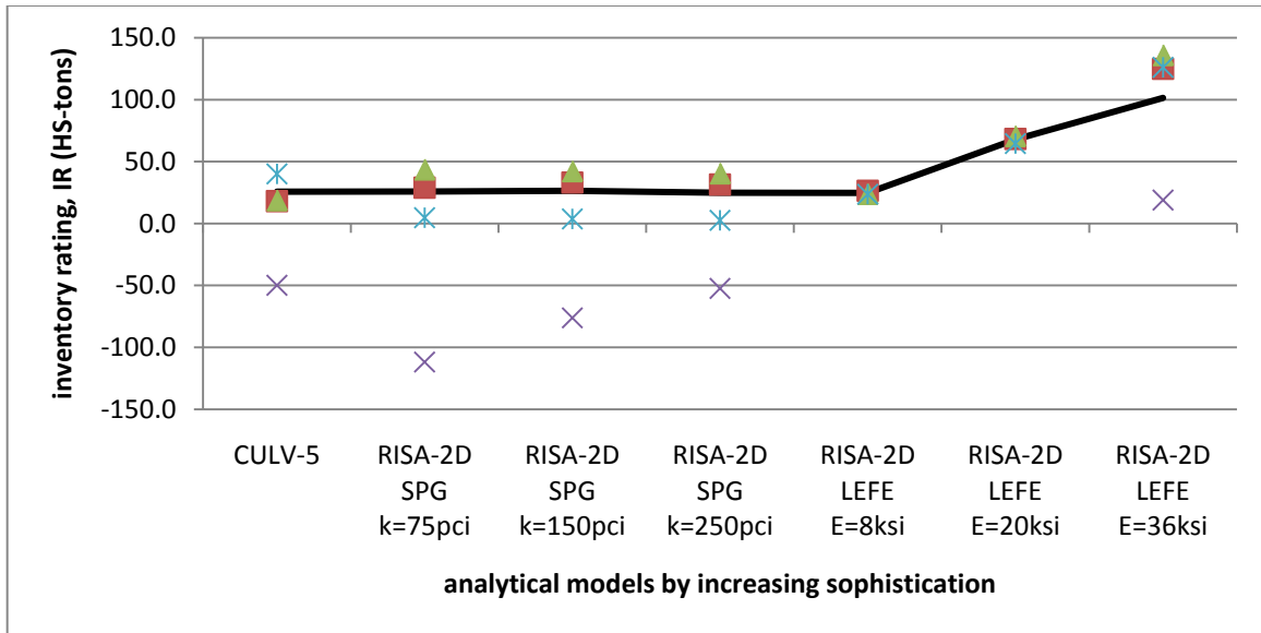
FIGURE 4.13. 1938 ERA INVENTORY RATINGS: 8' TO 18' OF FILL
