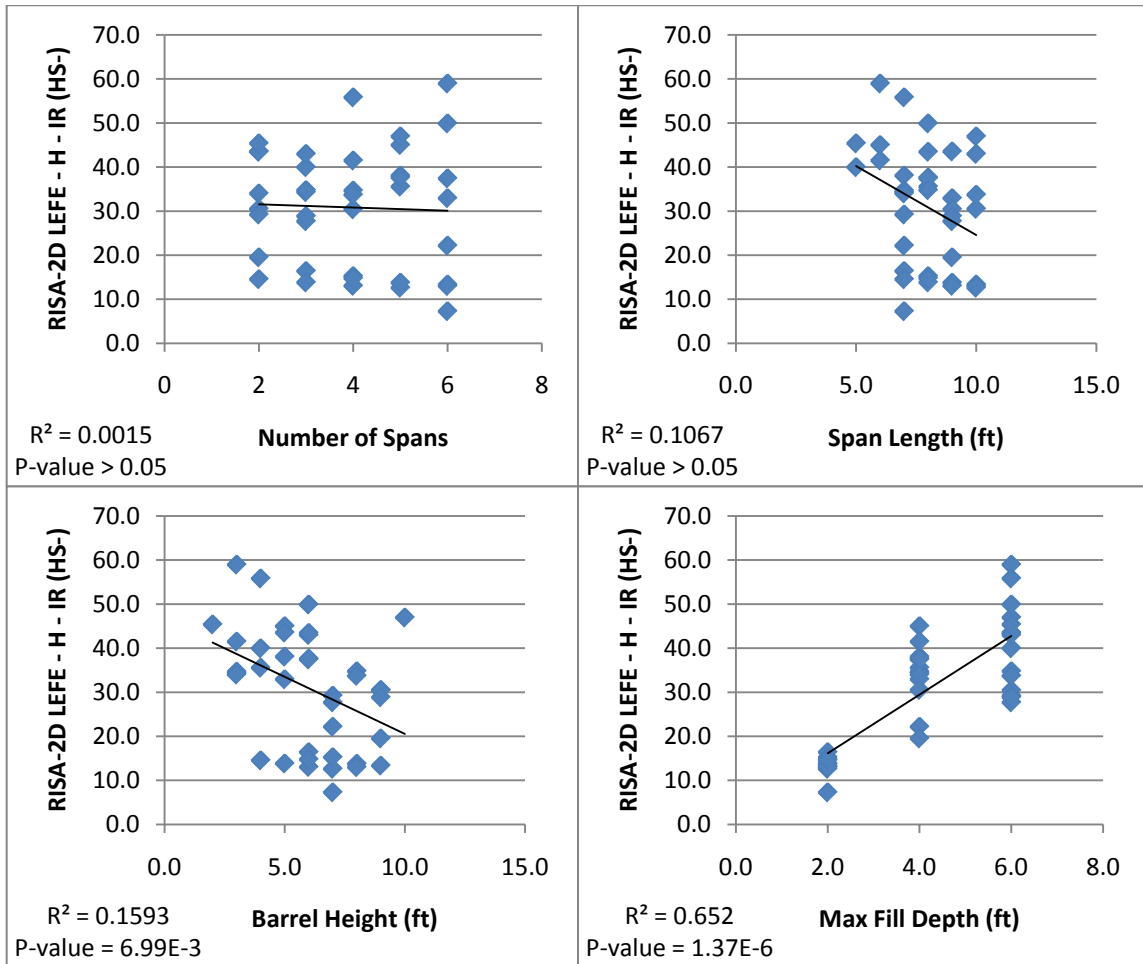
FIGURE 4.27. 1958 ERA 36KSI STEEL STATISTICAL ANALYSIS FOR SIGNIFICANT INDEPENDENT VARIABLES
