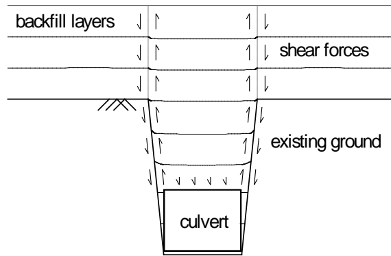
FIGURE 2.5. POSTIVE SOIL ARCHING
