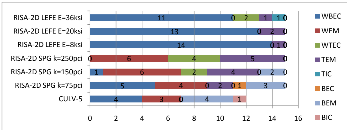
FIGURE 4.34. 1958 ERA 36KSI STEEL CONTROLLING CRITICAL SECTIONS: 6' OF FILL
