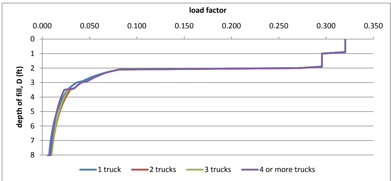
FIGURE 3.7. TWO DIMENSIONAL FRAME ANALYSIS COMPARISONS OF LIVE LOADS
