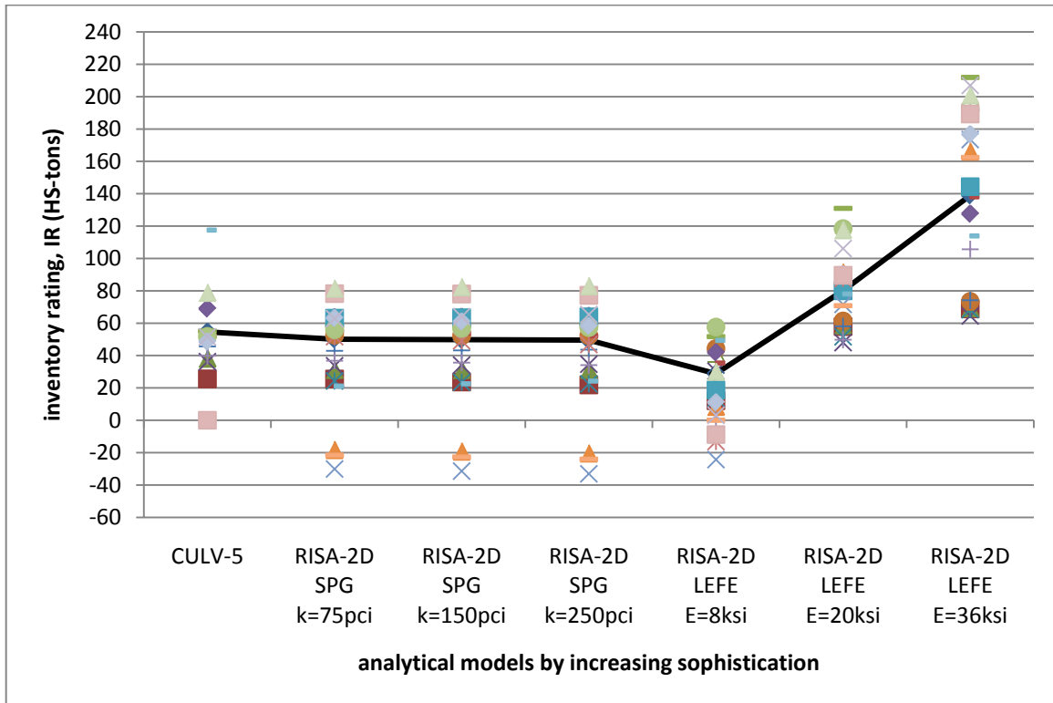
FIGURE 4.44. 2003 ERA INVENTORY RATINGS: UNDIFFERENTIATED
