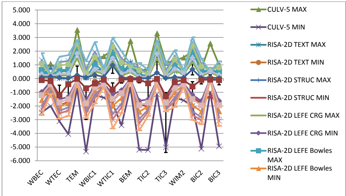
FIGURE 6.16. LIVE LOAD MOMENTS PREDICTED AND MEASURED FOR SHALLOWATER CULVERT: 4' OF FILL.
