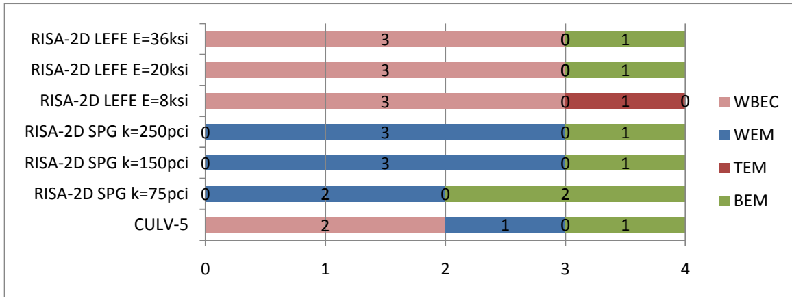
FIGURE 4.16. 1938 ERA CONTROLLING CRITICAL SECTIONS: 8' TO 18' OF FILL
