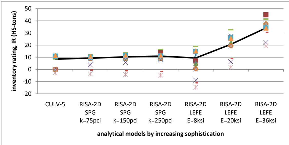
FIGURE 4.29. 1958 ERA 36KSI STEEL INVENTORY RATINGS: 4' OF FILL
