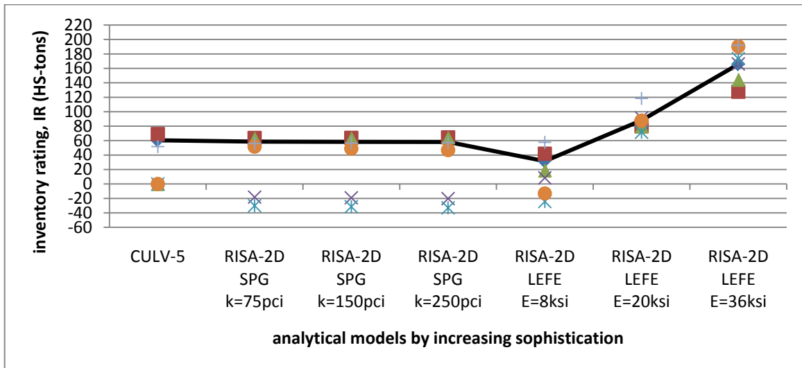
FIGURE 4.47. 2003 ERA INVENTORY RATINGS: 20' OF FILL
