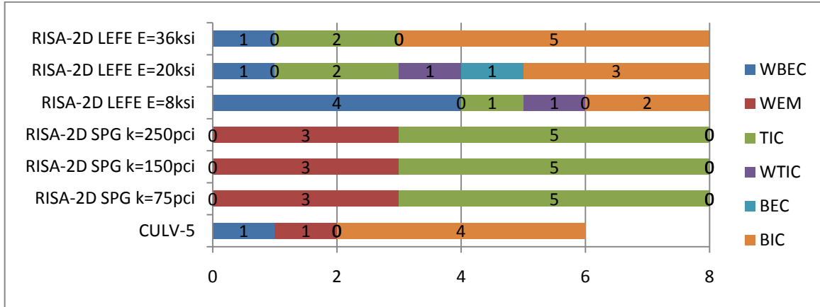
FIGURE 4.50. 2003 ERA CONTROLLING CRITICAL SECTIONS: 7' TO 16' OF FILL
