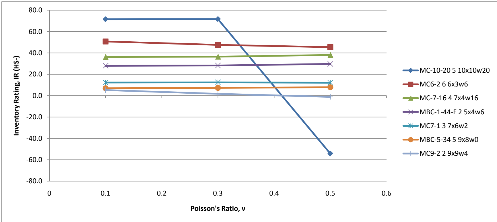
Figure 5.2. Poisson's Ratio vs. the Inventory Rating for Seven Representative Culvert Designs.
