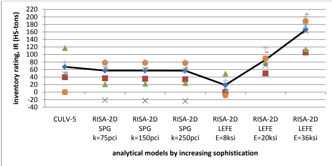
FIGURE 4.48. 2003 ERA INVENTORY RATINGS: 23' OF FILL
