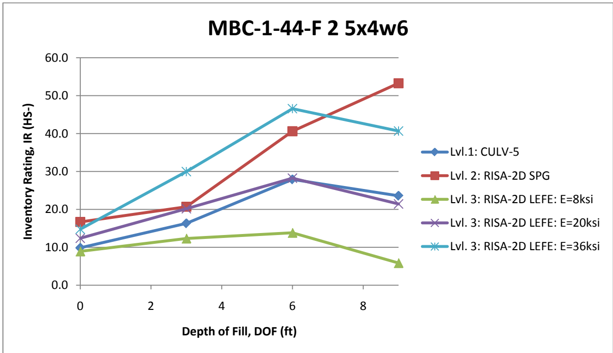
FIGURE 5.13. INVENTORY RATING VS. DEPTH OF FILL FOR MBC1-44-F 2 5X4W6.
