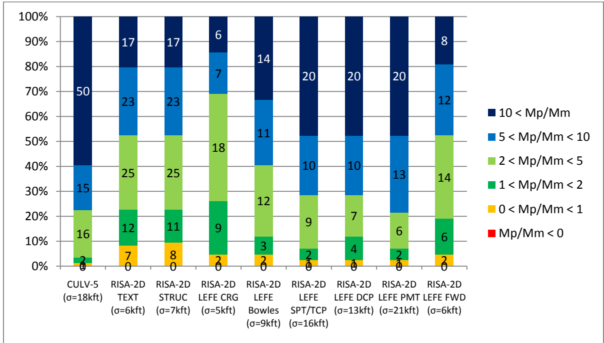
FIGURE 6.18. LIVE LOAD GOODNESS PLOT FOR SHALLOWATER CULVERT: 4' OF FILL
