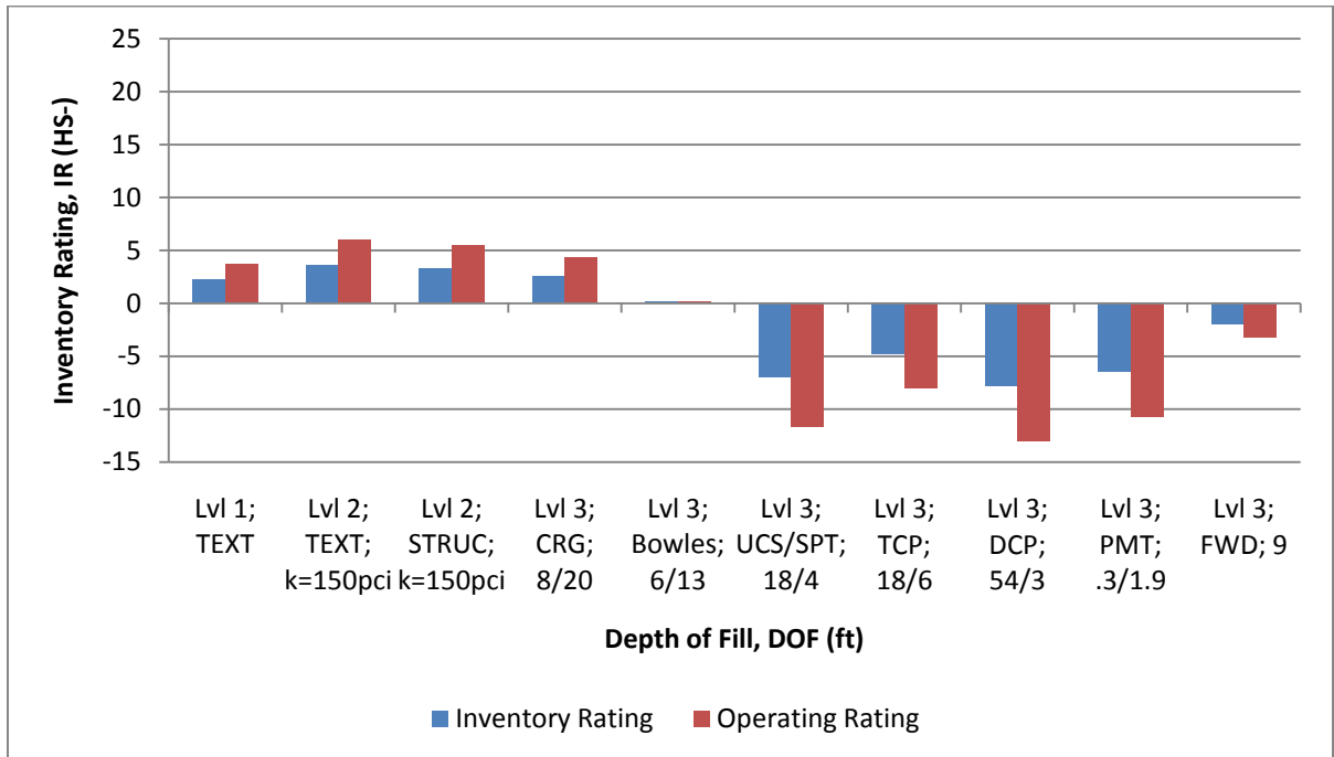
FIGURE 6.31. LOAD RATING FOR TULIA CULVERT: 1.5' OF FILL
