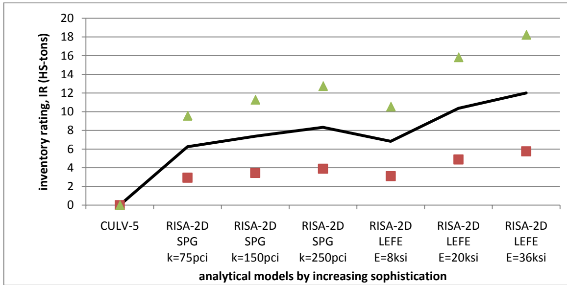
FIGURE 4.19. 1946 ERA INVENTORY RATINGS: MBC-3
