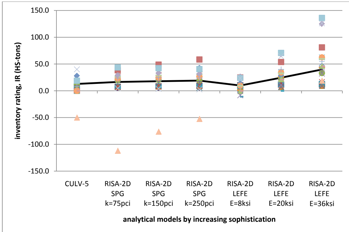
FIGURE 4.8. 1938 ERA INVENTORY RATINGS: UNDIFFERENTIATED
