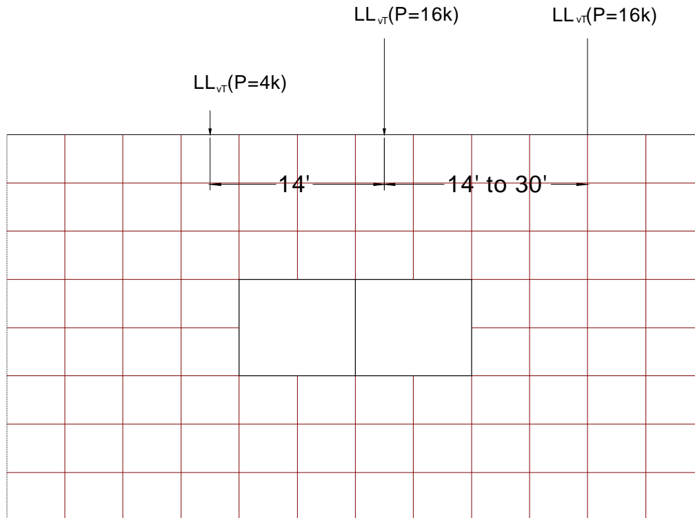
FIGURE 3.5. GENERAL, TWO-DIMENSIONAL, LINEAR-ELASTIC SOIL-STRUCTURE INTERACTION MODELS LOADING DIAGRAM.(TXDOT, 2009)
