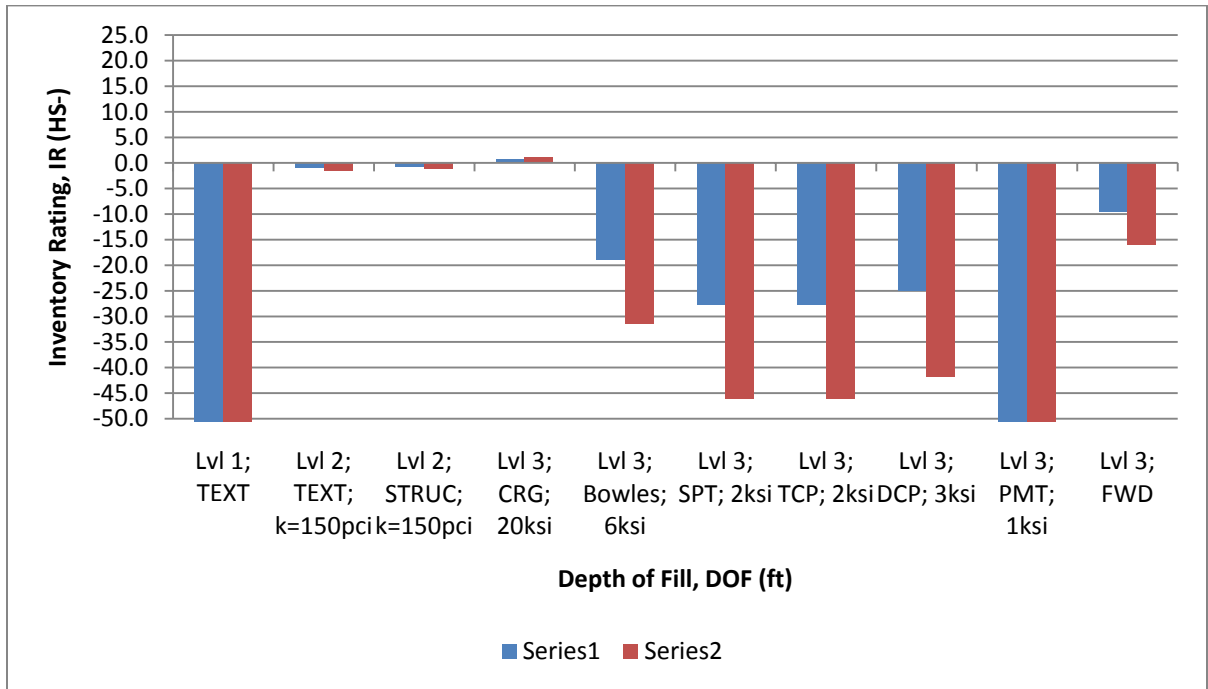
FIGURE 6.15. LOAD RATING FOR SHALLOWATER CULVERT: 4' OF FILL
