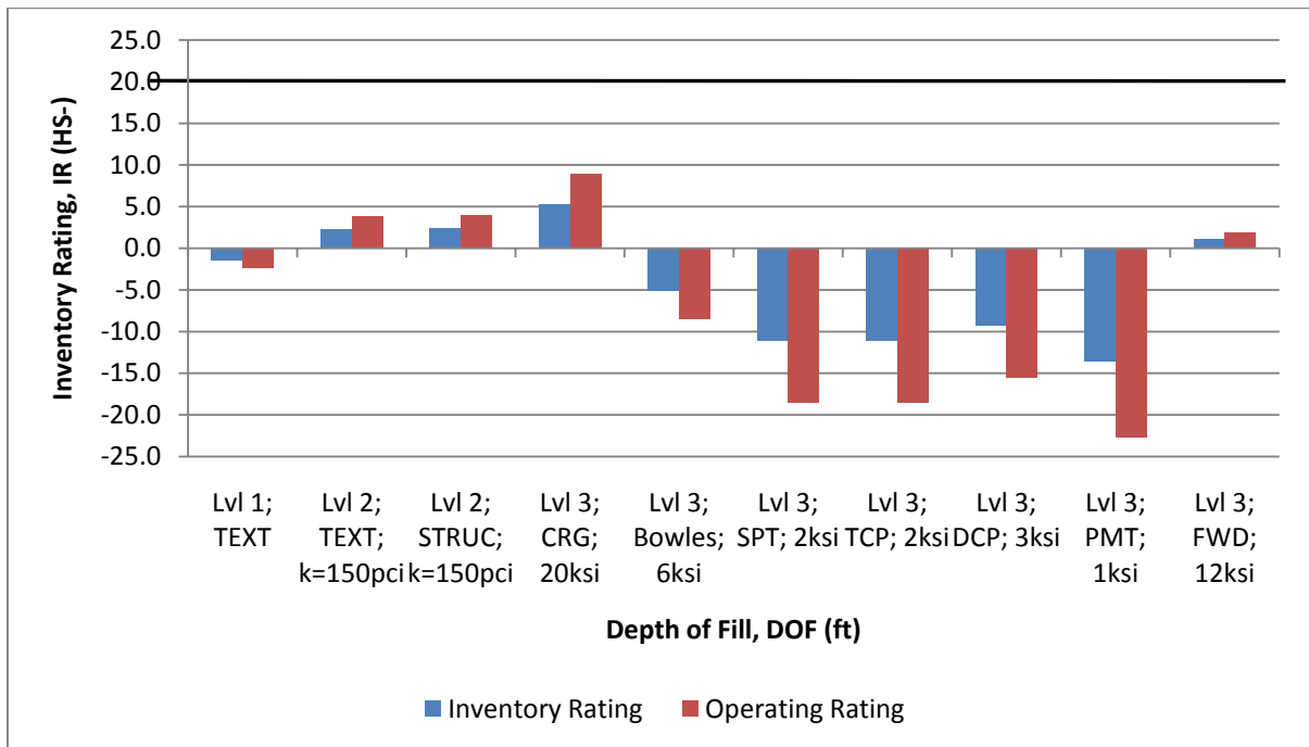
FIGURE 6.9. LOAD RATING FOR SHALLOWATER CULVERT: 2' OF FILL
