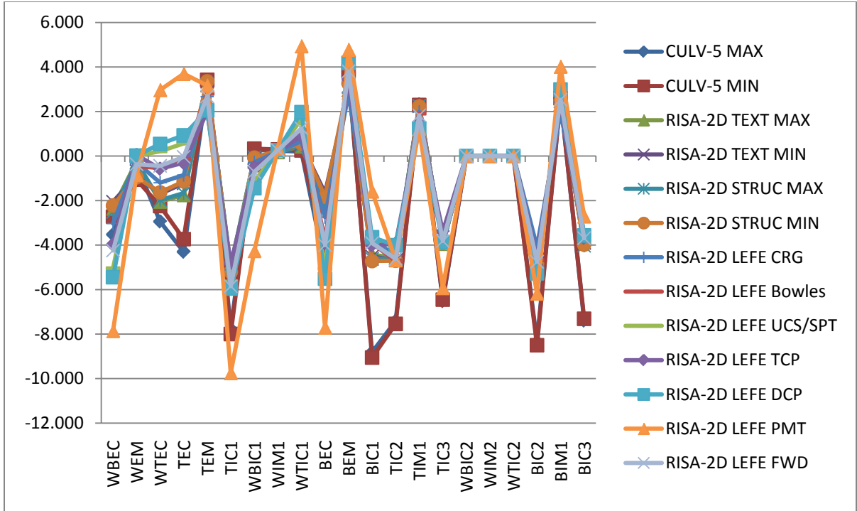
FIGURE 6.25. DEAD LOAD PREDICTED FOR PLAINVIEW CULVERT: 3.5' OF FILL.
