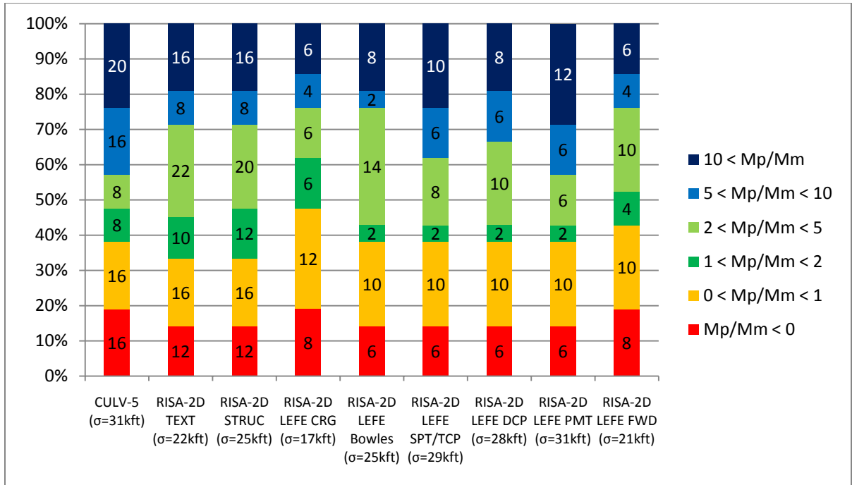
FIGURE 6.38. CHANGE IN DEAD LOAD GOODNESS FOR THE SHALLOWATER CULVERT FROM 2' TO 4' OF FILL.
