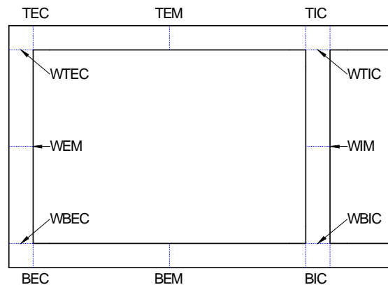
FIGURE 6.1. CRITICAL SECTIONS
