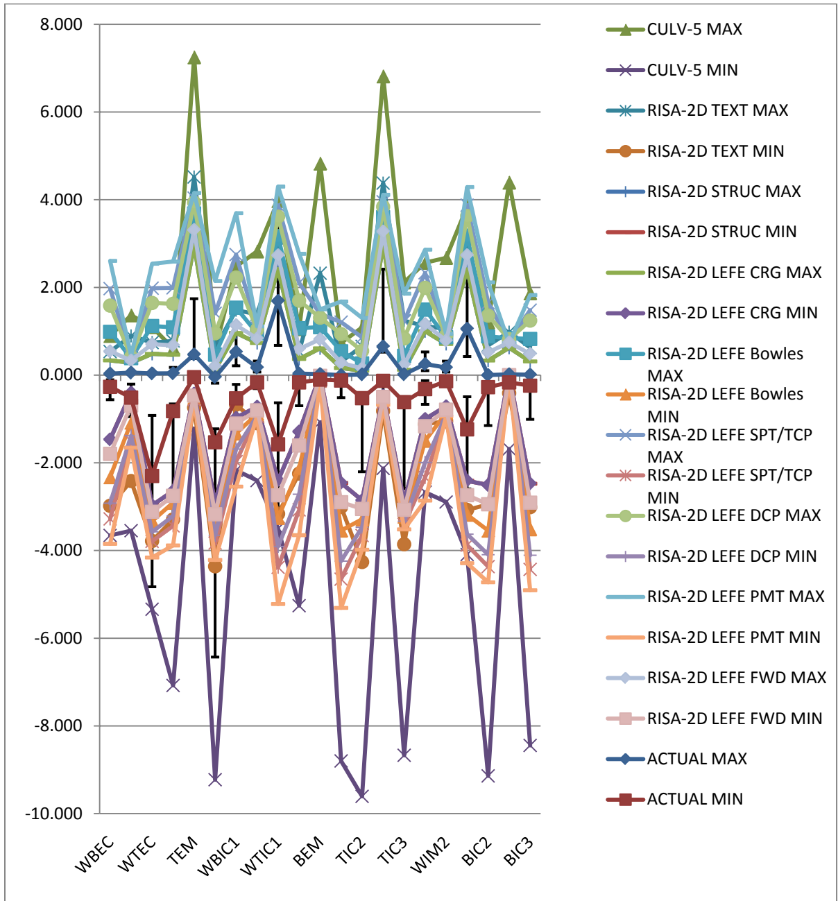
FIGURE 6.10. LIVE LOAD MOMENTS PREDICTED AND MEASURED FOR SHALLOWATER CULVERT: 2' OF FILL.
