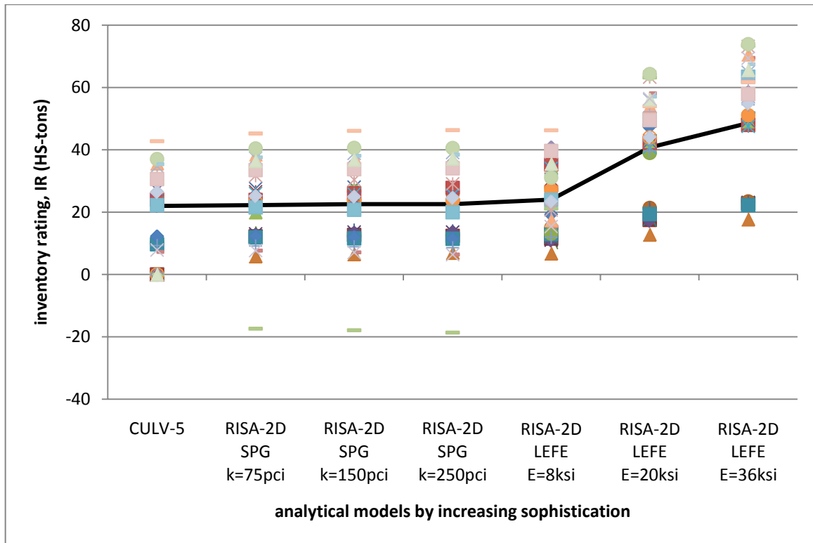
FIGURE 4.35. 1958 ERA 60KSI STEEL INVENTORY RATINGS: UNDIFFERENTIATED
