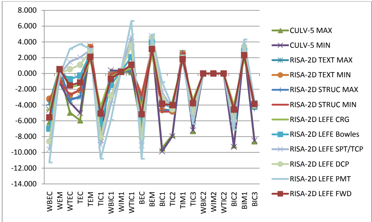
FIGURE 6.17. DEAD LOAD PREDICTED FOR SHALLOWATER CULVERT: 4' OF FILL.
