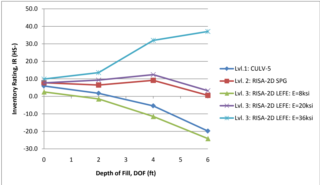
FIGURE 5.12. INVENTORY RATING VS. DEPTH OF FILL FOR MBC-5-34 5 9X8W0.
