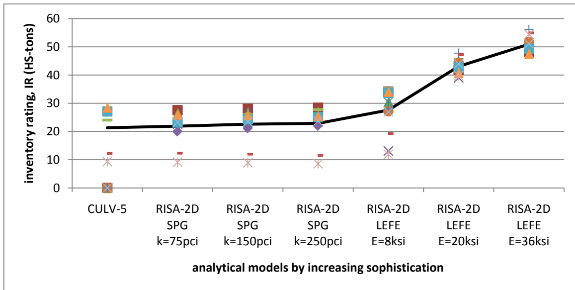
FIGURE 4.38. 1958 ERA 60KSI STEEL INVENTORY RATING: 4' OF FILL
