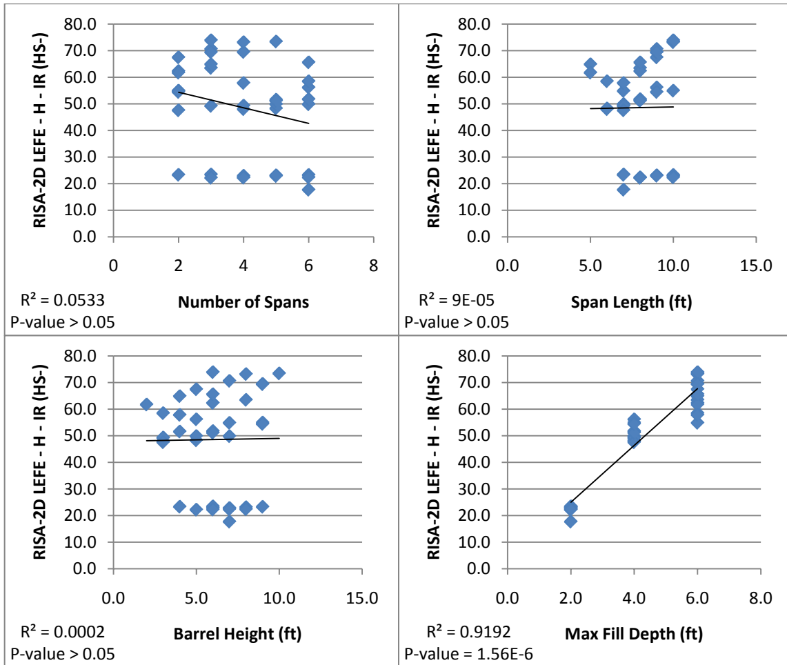
FIGURE 4.36. 1958 ERA 60KSI STEEL STATISTICAL ANALYSIS FOR SIGNIFICANT INDEPENDENT VARIABLES
