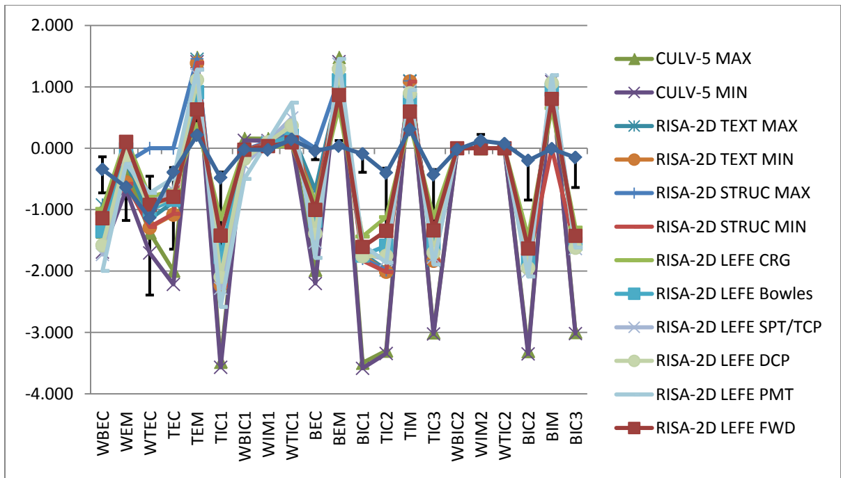
FIGURE 6.37. THE CHANGE IN DEAD LOAD MOMENT, PREDICTED AND MEASURED, FOR THE SHALLOWATER CULVERT FROM 2' TO 4' OF FILL.
