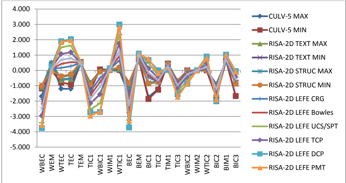
FIGURE 6.33. DEAD LOAD PREDICTED FOR TULIA CULVERT: 1.5' OF FILL.
