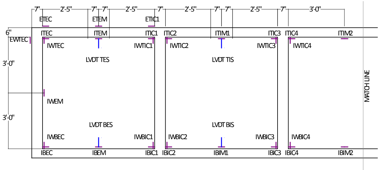
FIGURE 6.30. TULIA INSTRUMENTATION PLAN.
