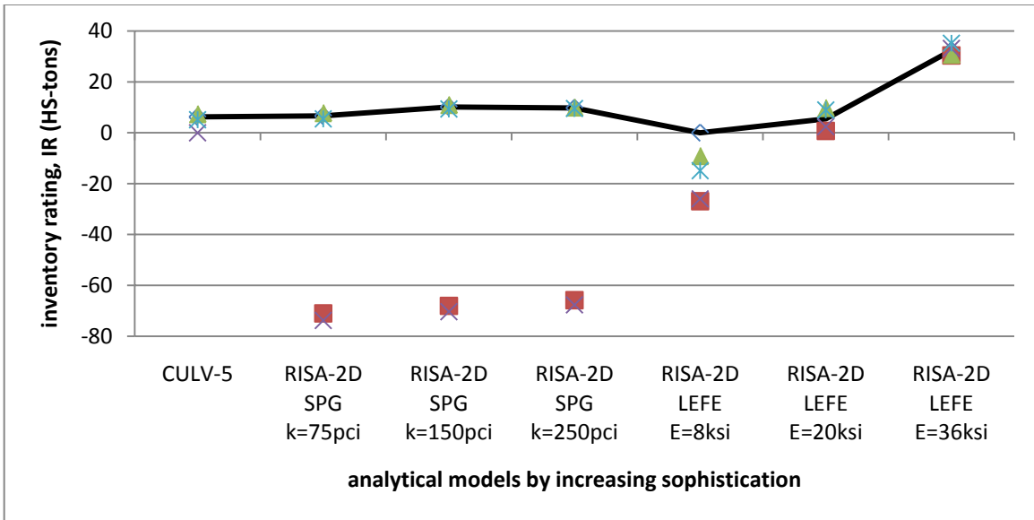
FIGURE 4.20. 1946 ERA INVENTORY RATINGS: MC10-3-45
