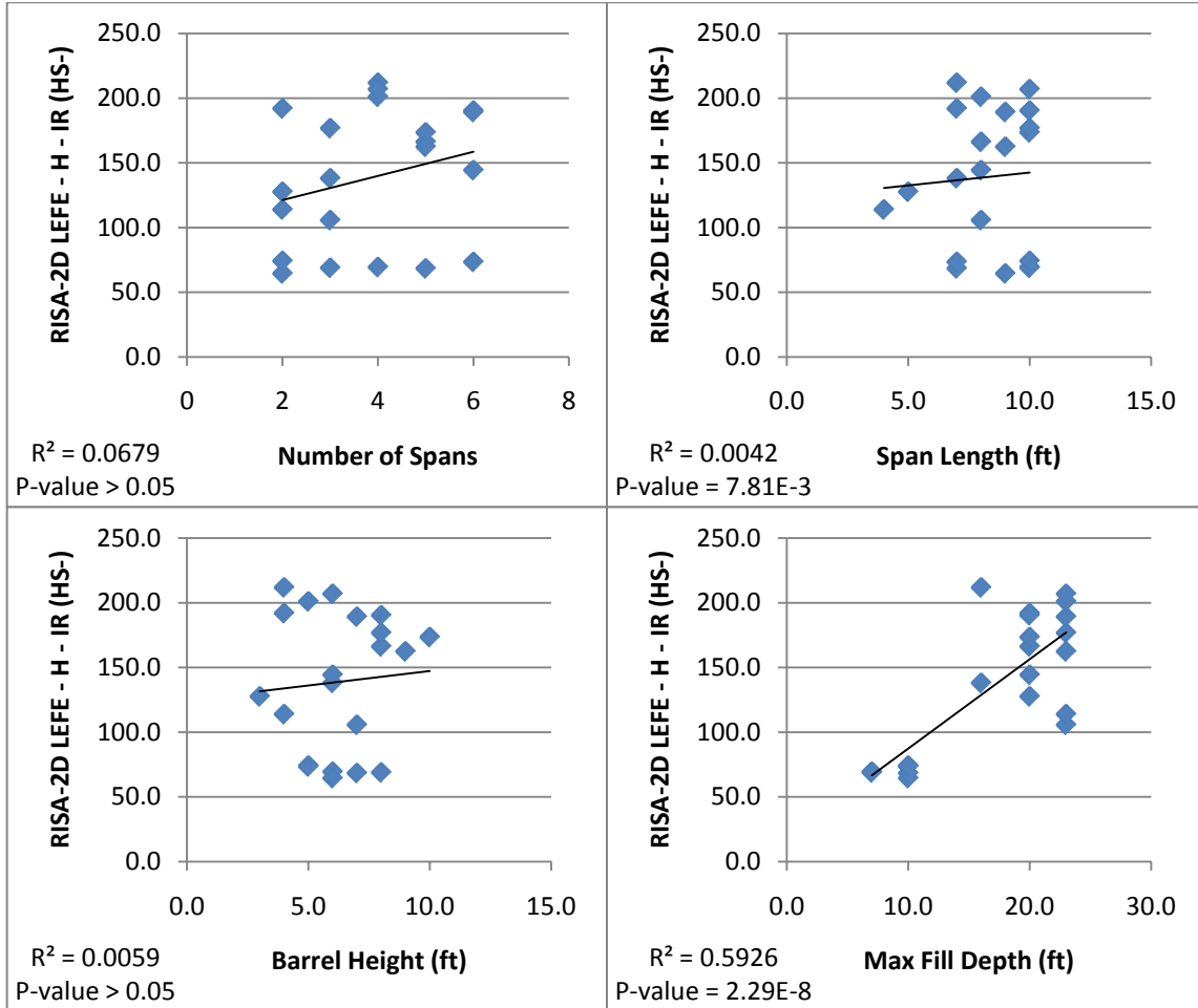
FIGURE 4.45. 2003 ERA STATISTICAL ANALYSIS FOR SIGNIFICANT INDEPEDNET VARIABLES
