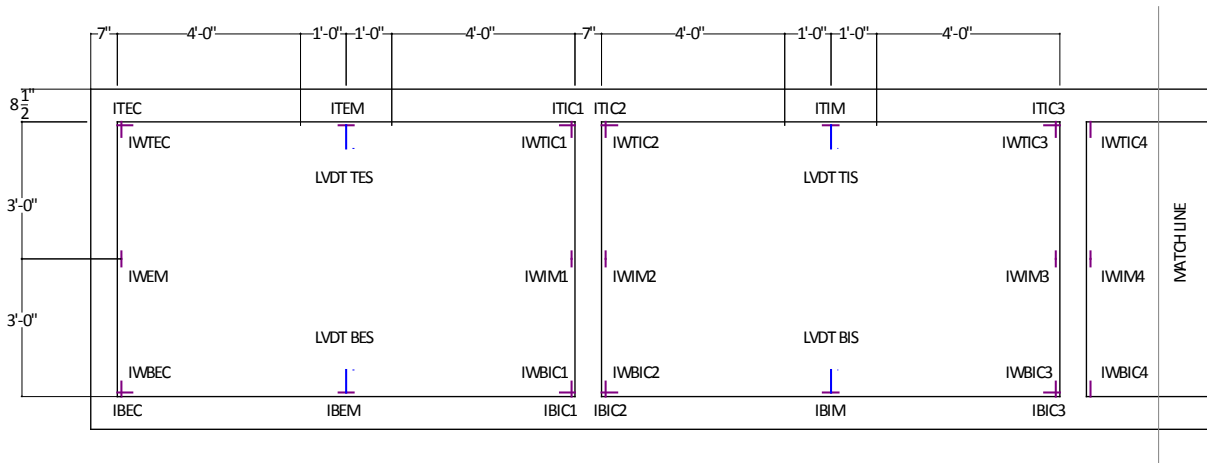
FIGURE 6.22. PLAINVIEW INSTRUMENTATION PLAN.
