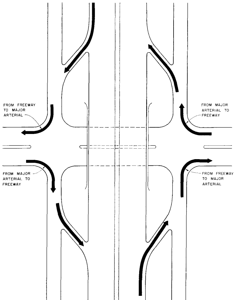
Figure 21. Interchange movements.
