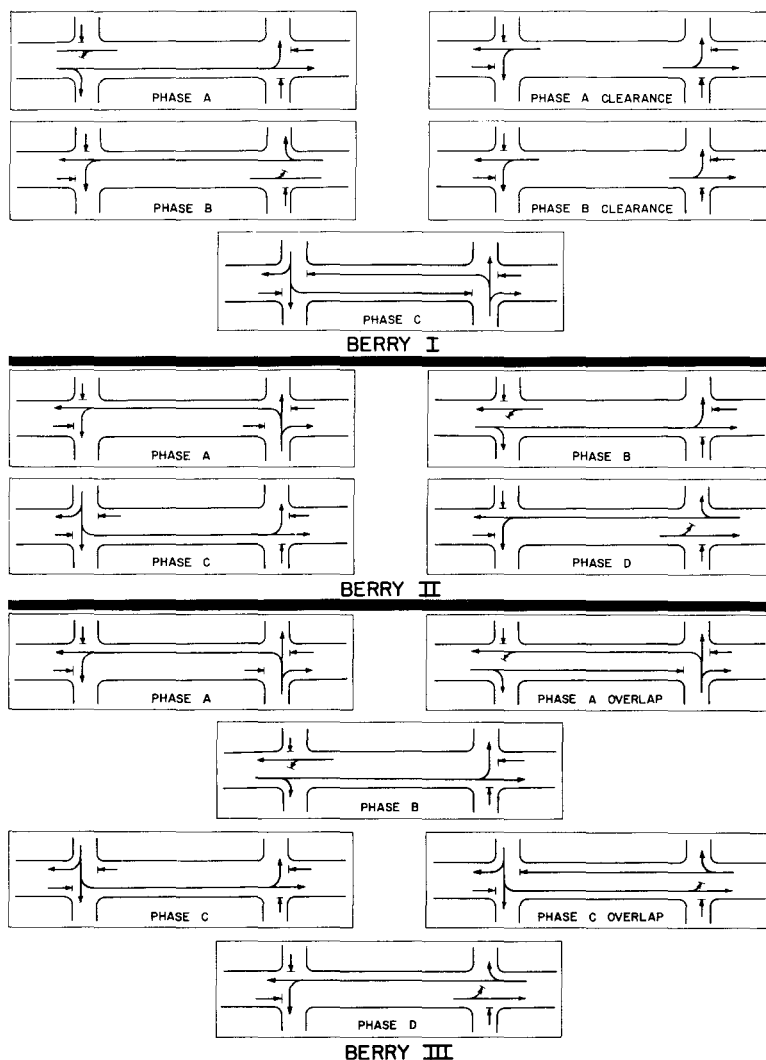
Figure 11. Phasing sequences.
