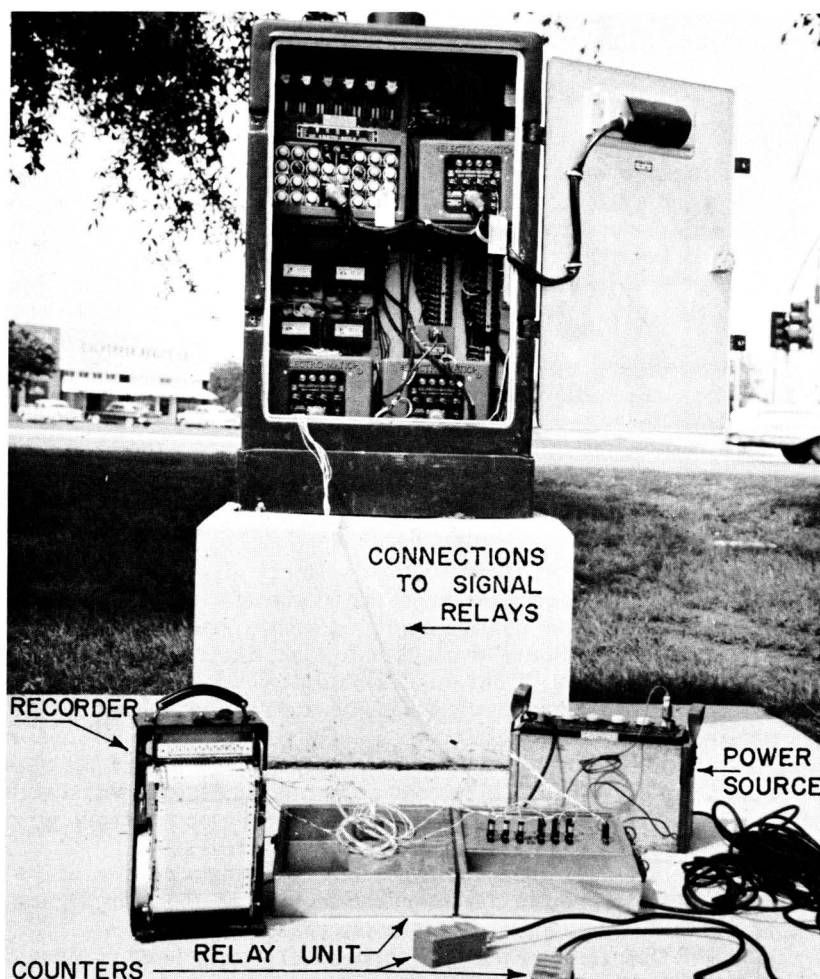
Figure 9. Recording equipment.
