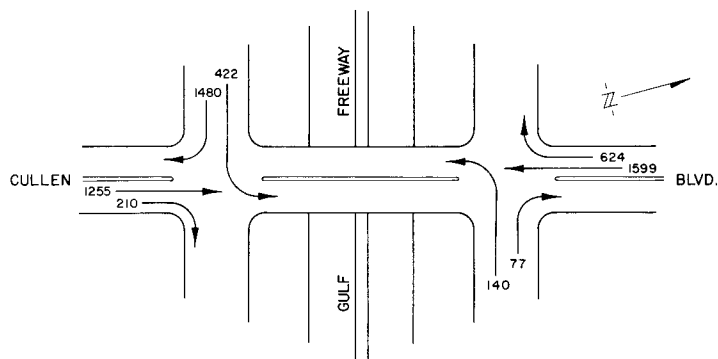
Figure 27. Estimated hourly volumes (1,980), p. m. peak.
