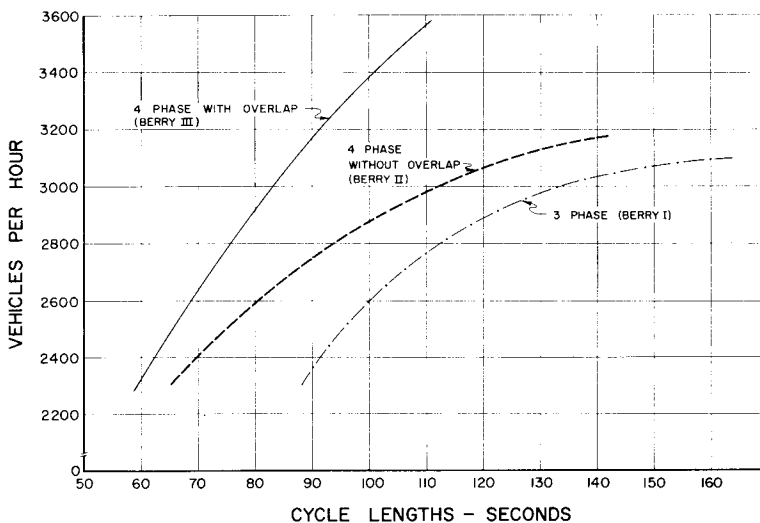
Figure 17. Plot of cycle lengths vs number of vehicles moved per hour.
