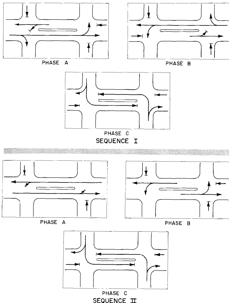
Figure 3. Signal phasings.
