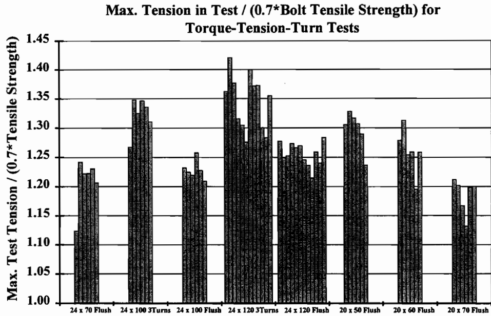
Figure 4. 28 Maximum tension in Test/(0.7*bolt tension strength) for torque-tension-turn tests
