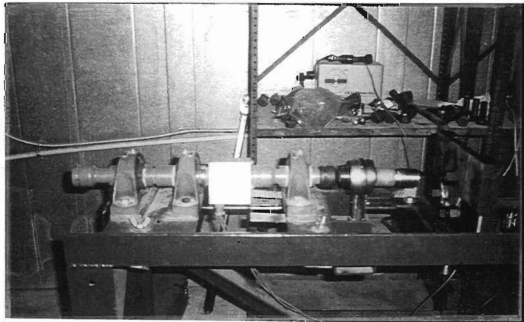
Figure 3. 14 Solid plate test setup
