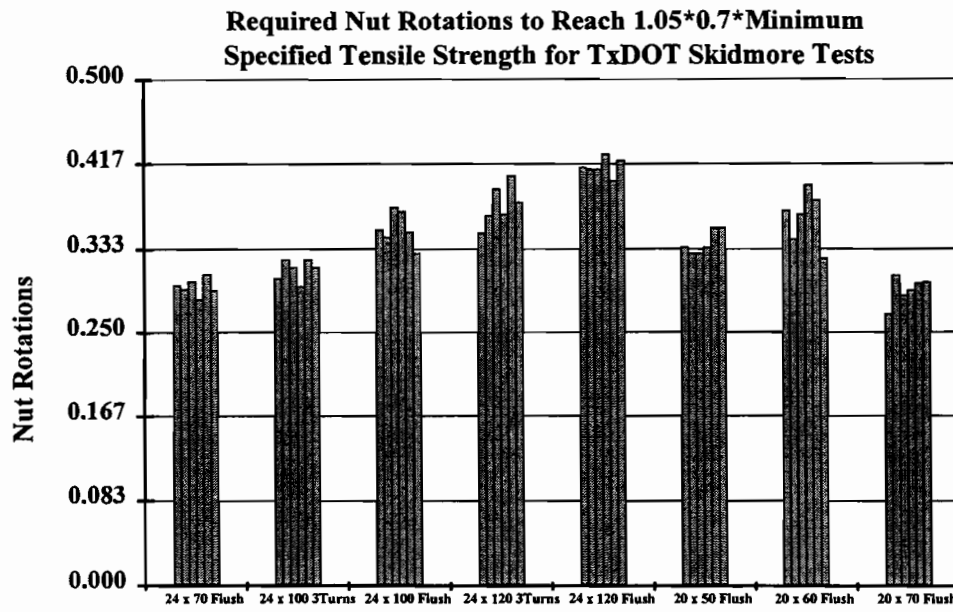
Figure 4. 31 Required nut rotations to reach 1.05*0.70*minimum specified tensile strength in TxDOT tests
