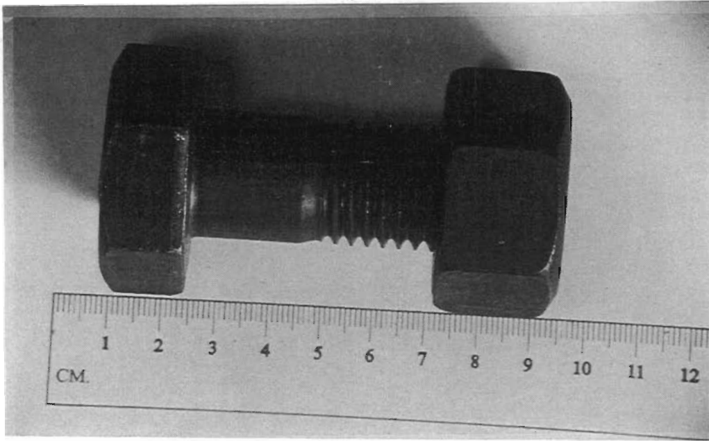
Figure 3.3 Example of flush grip for a 24 mm x 70 mm bolt
