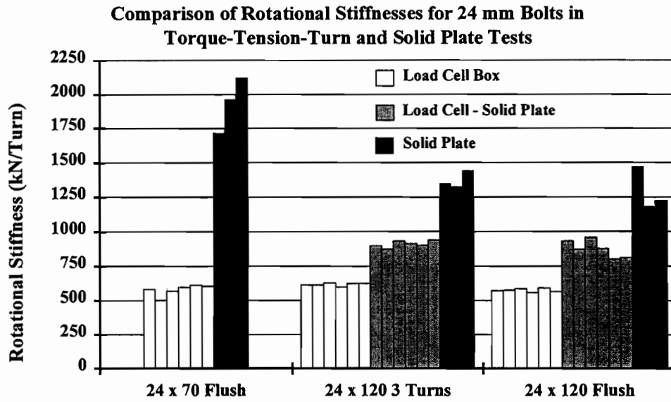
Figure 4. 12 Comparison of rotational stiffnesses for 24 mm bolts in torque-tension-turn and solid plate tests
