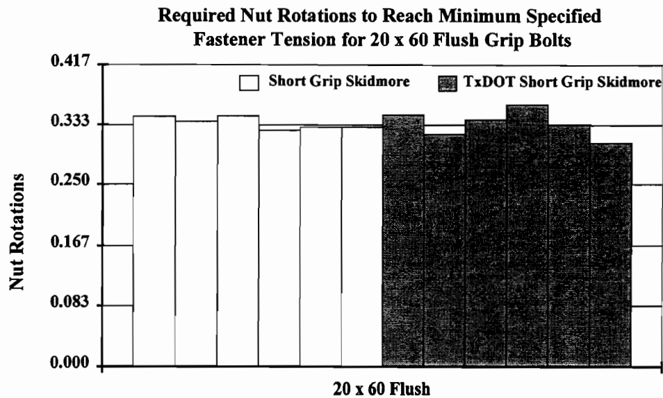
Figure 4. 20 Required nut rotations to reach minimum specified fastener tension for 20 x 60 flush grip bolts
