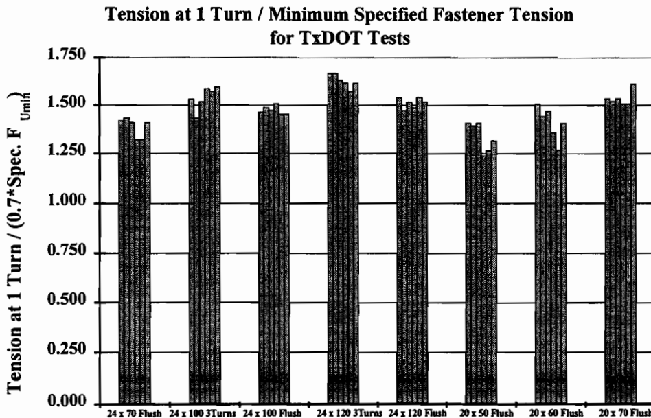
Figure 4. 29 Tension at one turn / minimum specified fastener tension for TxDOT tests
