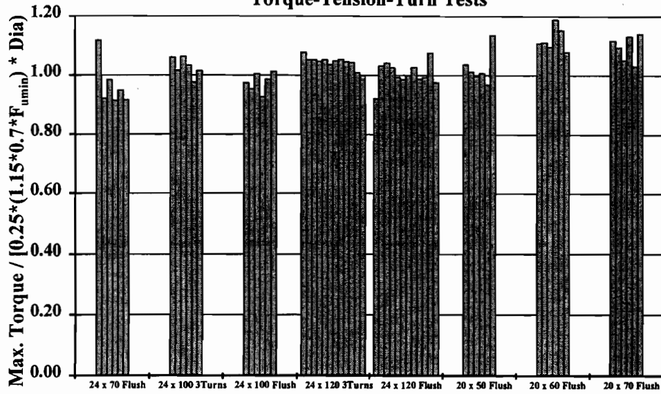
Figure 4. 26 Maximum torque in test/AASHTO maximum allowable torque
