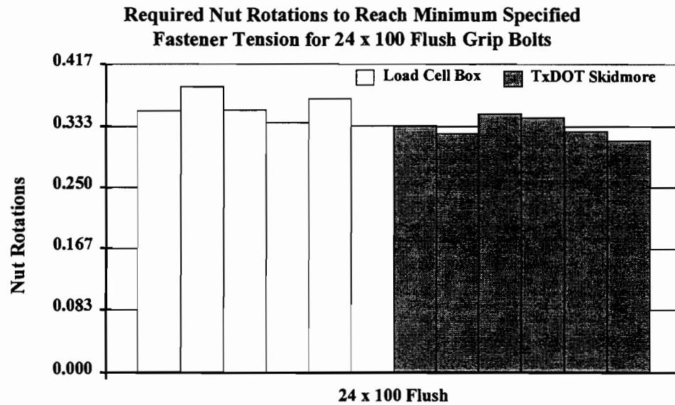
Figure 4. 16 Required nut rotations to reach minimum specified fastener tension for 24 x 100 flush grip bolts
