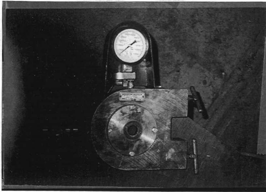
Figure 3. 2 Skidmore-Wilhelm bolt calibrator used for direct tension tests
