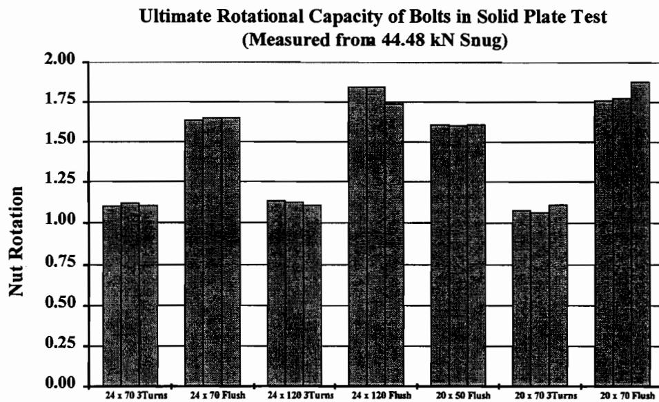
Figure 4. 22 Ultimate rotational capacity of bolts in solid plate tests
