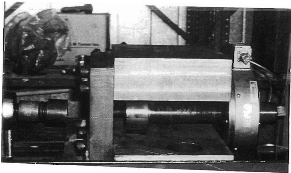
Figure 3. 9 Grip length adjustment apparatus for load cell box system
