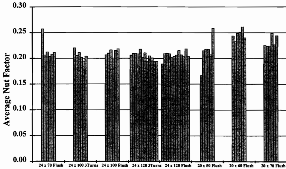
Figure 4. 25 Average nut factors in torque-tension-turn tests
