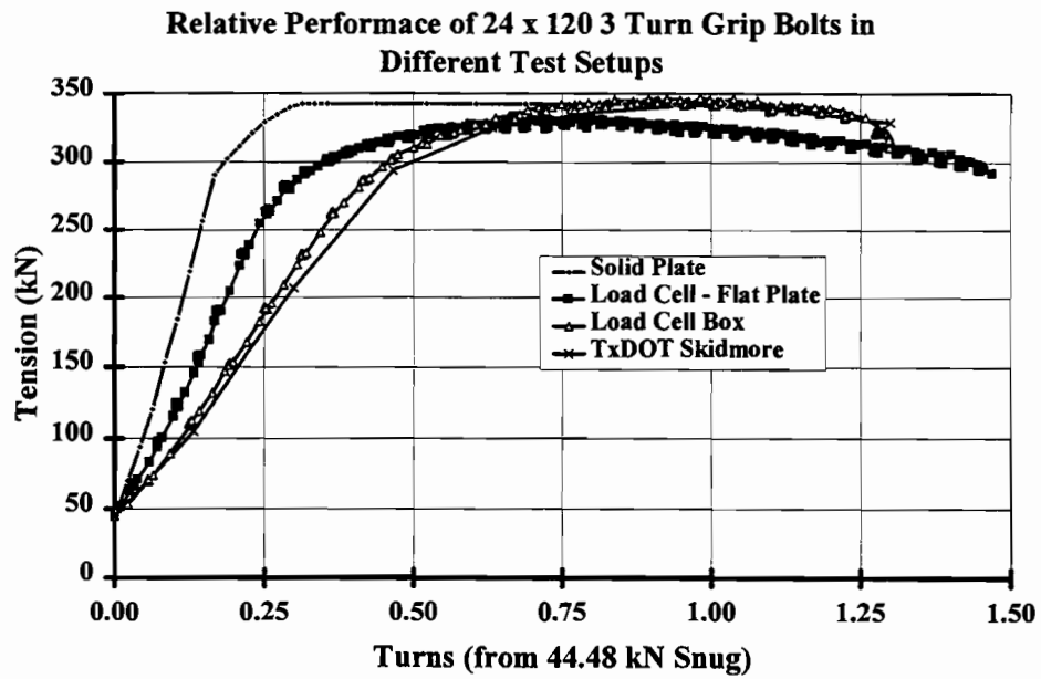
Figure 4.6 Relative performance of 24 x 120 three turn grip bolts in different test setups
