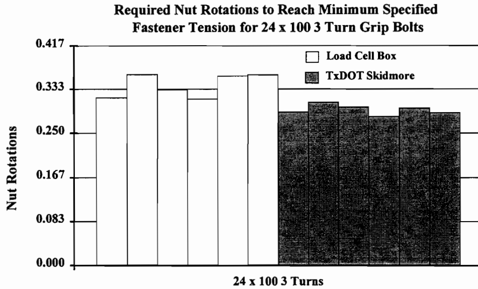
Figure 4. 17 Required nut rotations to reach minimum specified fastener tension for 24 x 100 three turn grip bolts
