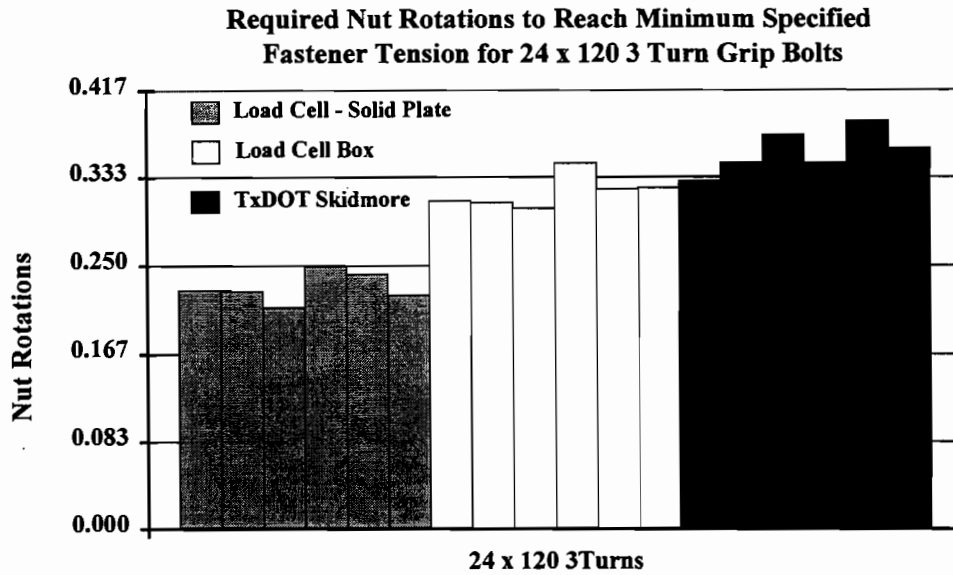
Figure 4. 19 Required nut rotations to reach minimum specified fastener tension for 24 x 120 three turn grip bolts
