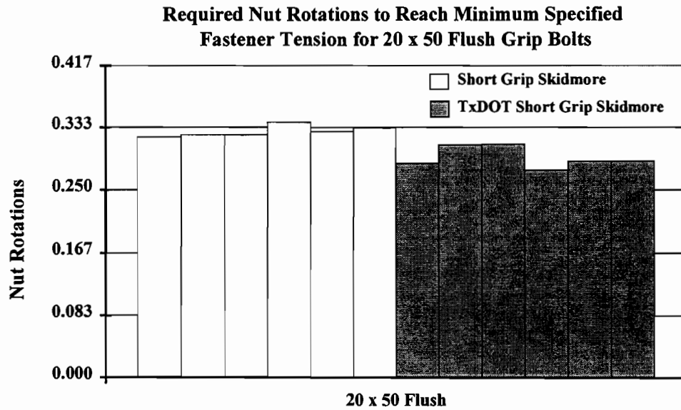
Figure 4. 21 Required nut rotations to reach minimum specified fastener tension for 20 x 50 flush grip bolts
