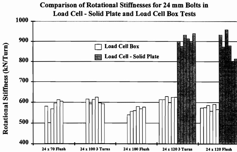
Figure 4. 11 Comparison of rotational stiffnesses for 24 mm bolts in load cell solid plate and load cell box tests
