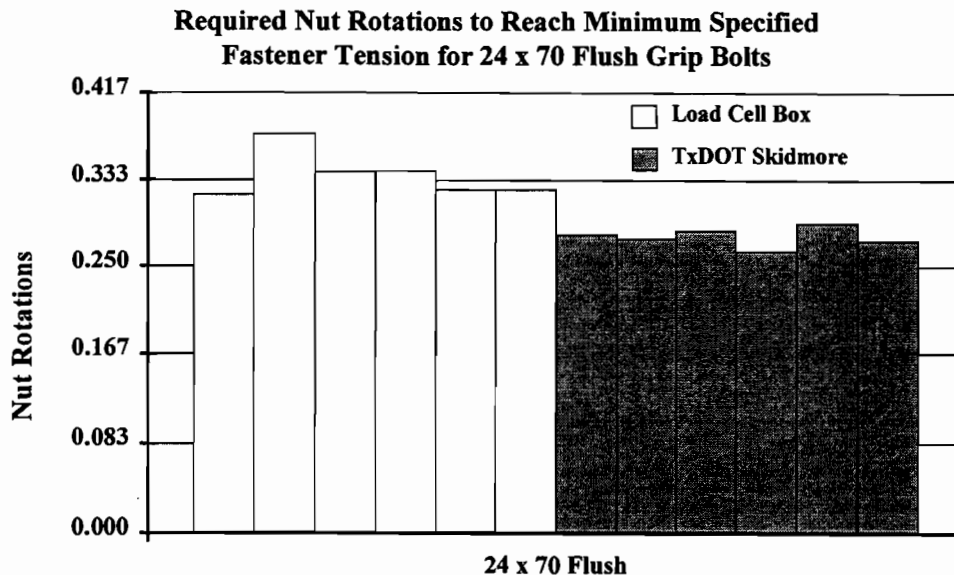
Figure 4.15 Repaired nut rotations to reach minimum specified fastener tension for 24 x 70 flush grip bolts
