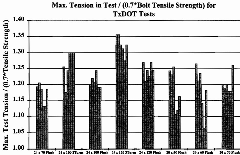
Figure 4. 27 Maximum tension in Test/(0.7*bolt tensile strength) for TxDOT tests
