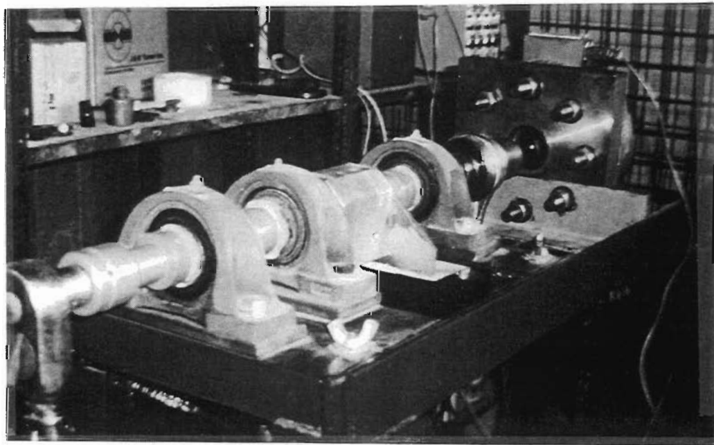
Figure 3.6 Front view of load cell - flat plate system
