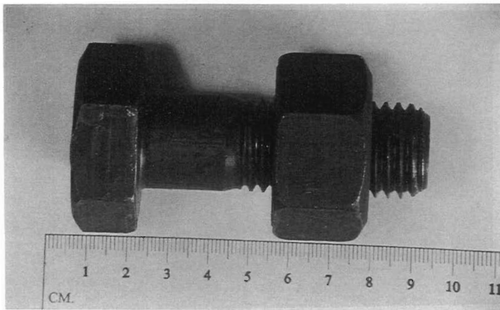
Figure 3.4 Example of three turns grip for a 24 mm x 70 mm bolt
