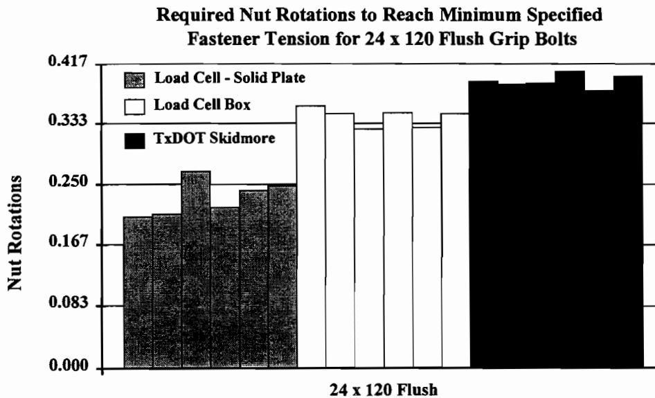
Figure 4. 18 Required nut rotations to reach minimum specified fastener tension for 24 x 120 flush grip bolts
