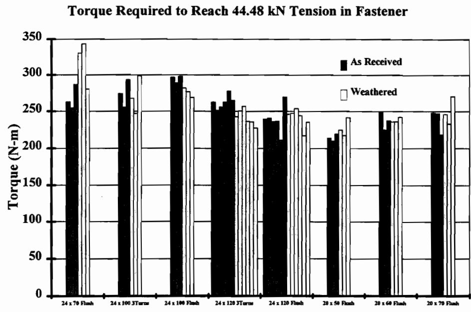
Figure 4.2 Torque required to reach 44.48 kN tension in fastener
