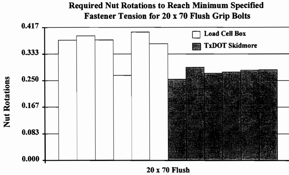
Figure 4. 23 Required nut rotations to reach minimum specified fastener tension for 20 x 70 flush grip bolts
