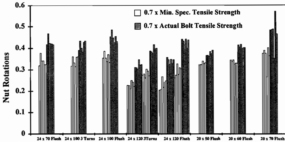
Figure 5.2 Comparison of turns required to reach 0.7 x min. spec. tensile strength with turns required to reach 0.7 x actual bolt tensile strength
