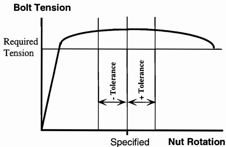
Figure 2.1 Sample tension-turn relationship for A325 bolt
