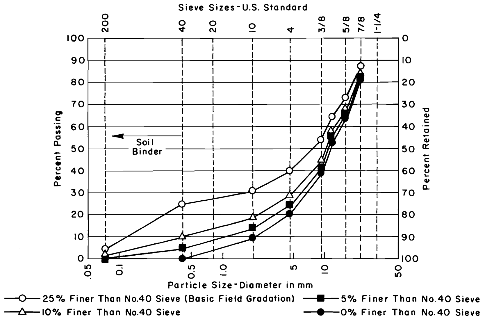
Fig 2. Gradations of Lubbock limestone mixtures.
