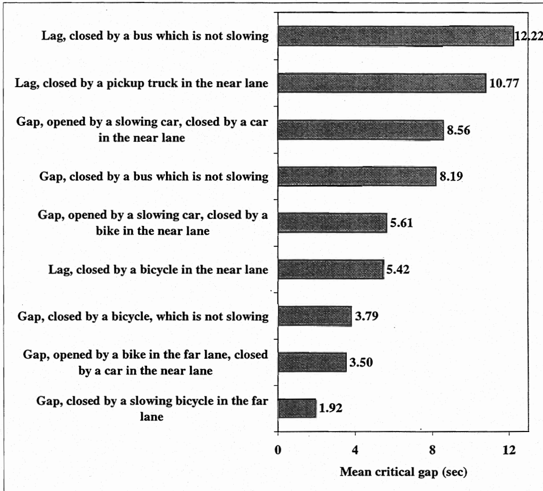
Figure 2.14. Comparison of a variety of possible lateral left-turning automobile gap acceptance situations.
