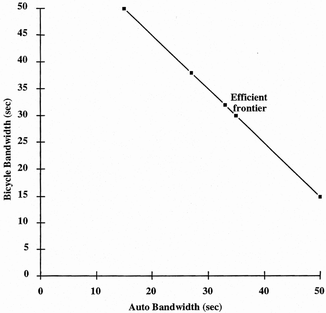
Figure 4.11. Plot of nondominated solutions to biobjective example formulation
