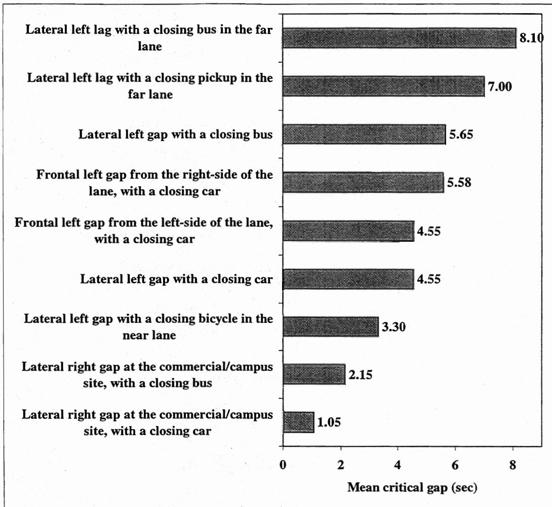
Figure 2.15. Comparison of a variety of possible gap acceptance situations for bicycles.
