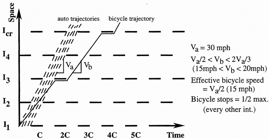
Figure 4.3. Effect of increasing bicycle progression speed.
