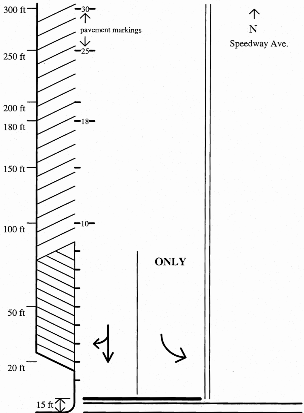
Figure 3.9. Diagram of the data collection site: the approach to the intersection of 26 th and Speedway in Austin, Texas.
