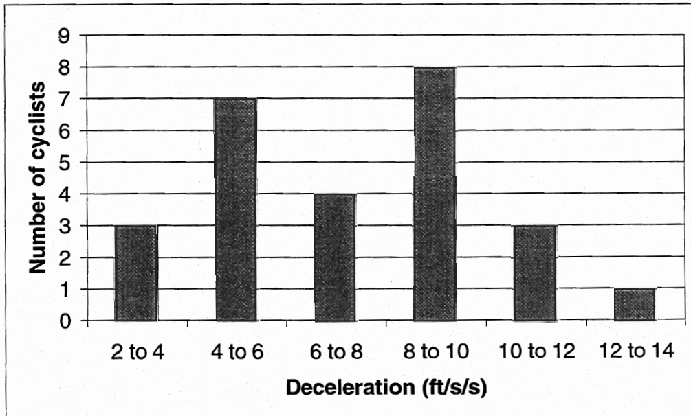
Figure 3.3. Frequency distribution of comfortable deceleration measurements.
