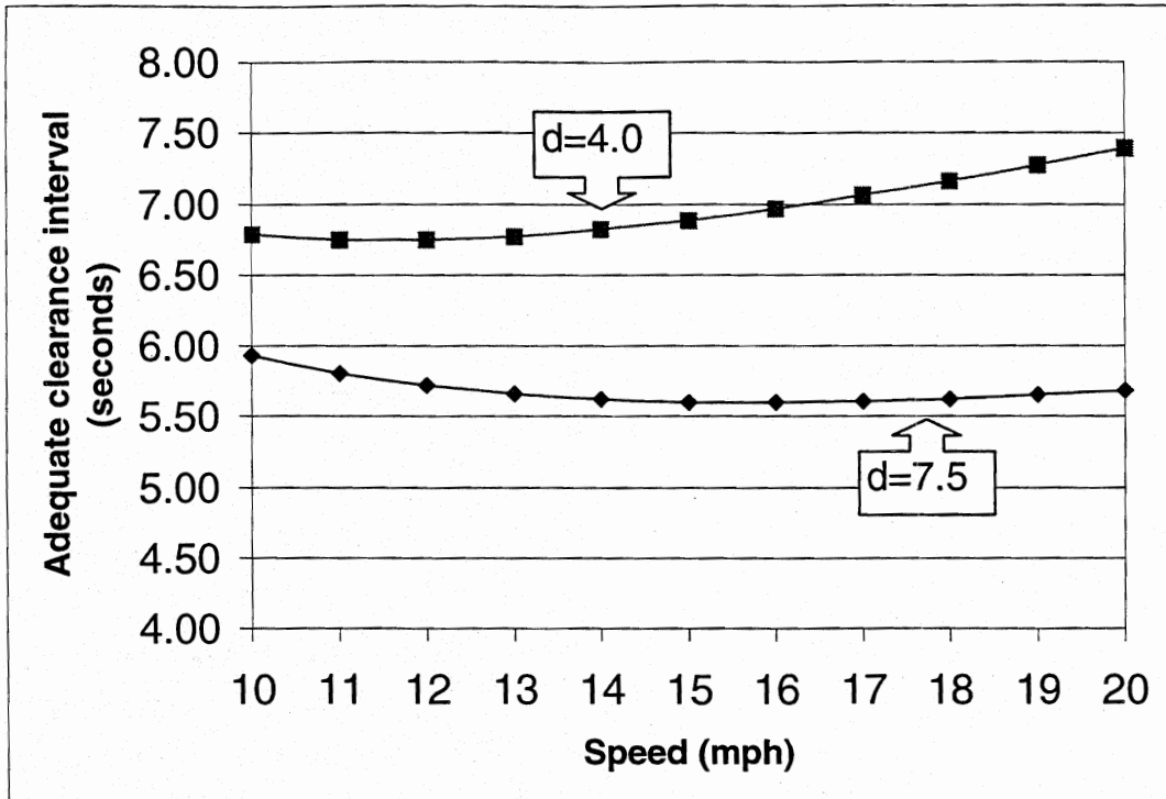
Figure 3.8. Sensitivity of adequate clearance intervals for bicycles, traveling at speeds between 10 and 20 mph, to a deceleration of 7.5 ft/s 2 (relative to 4.0 ft/s 2 ), assuming no acceleration, a design clearance point at a distance 30 ft from the stopbar, and a perception-reaction time of 2.5 seconds.
