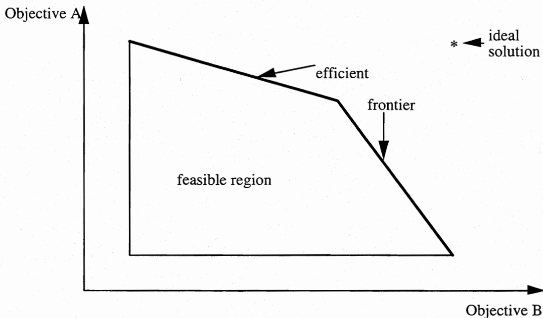
Figure 4.9. Illustration of an efficient frontier in biobjective space
