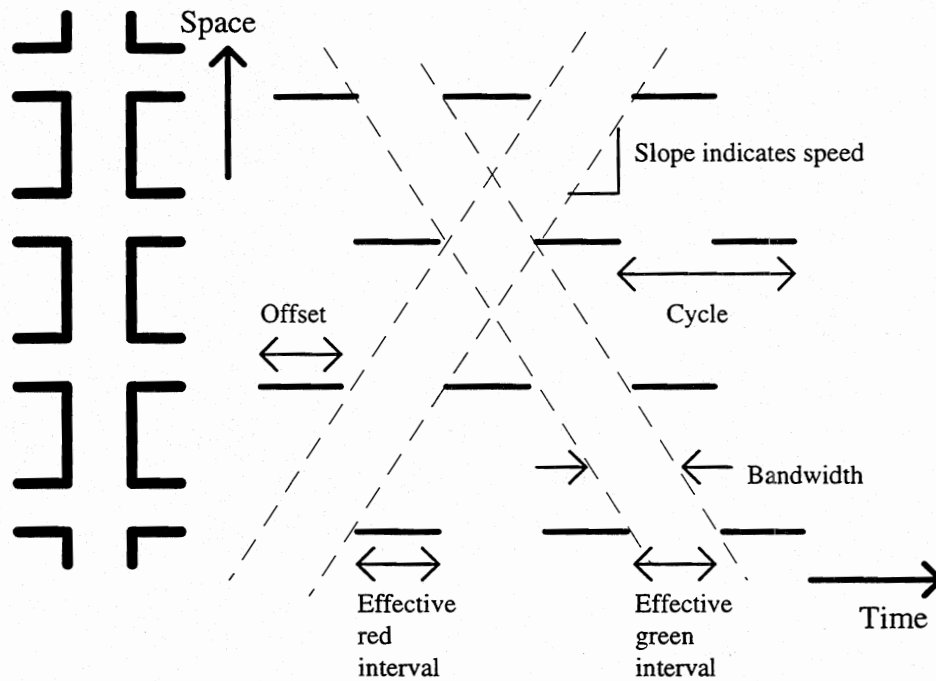
Figure 4.1. Example time-space diagram.
