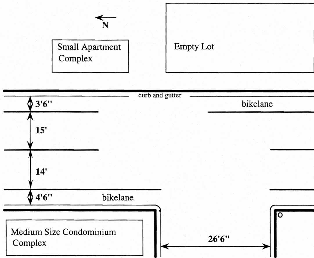
Figure 2.6. Residential site used to collect gap data at the intersection of Speedway and 34 th in Austin, TX.
