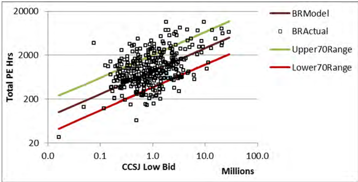
Figure 3.40: PE Hours Model for BR Projects with Upper and Lower 70% Range: Log-Log Plot
