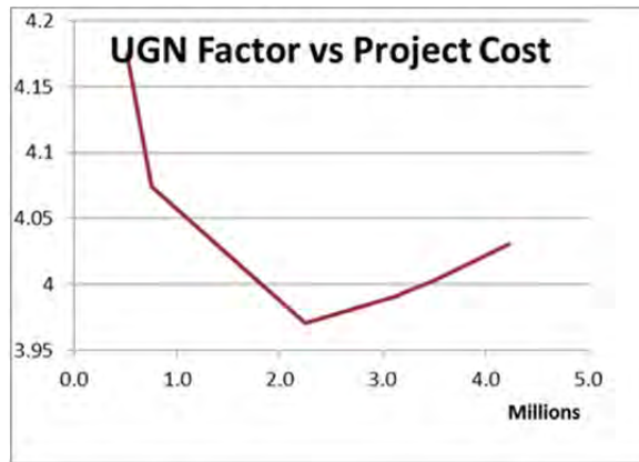
Figure 3.65: Change in Widening Factor for UGN Projects across Cost Range
