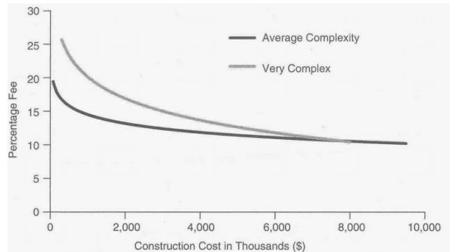
GRAPH 3. Total Fee vs. Construction Cost for New Construction.
