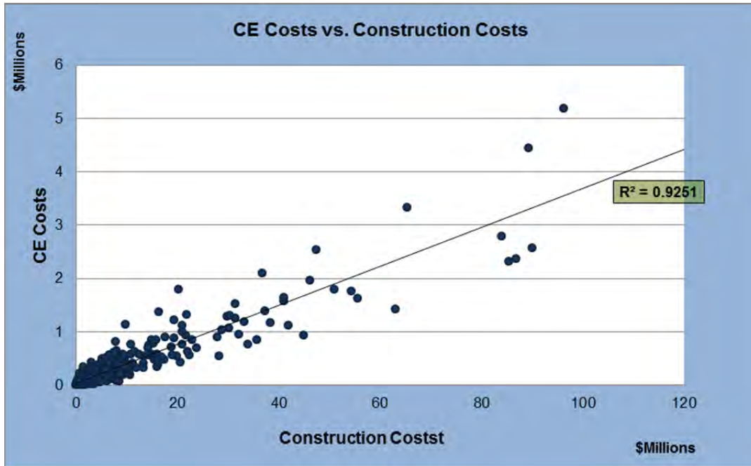
Figure 4.7: Scatter Plots of CE Costs vs. Construction Costs (Before Transformation)
