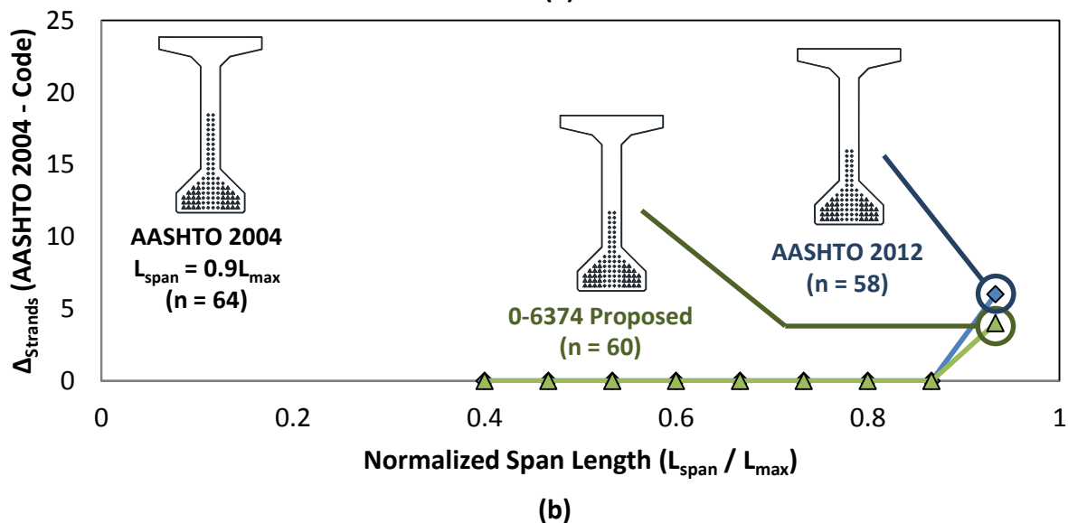
Figure D.11 - Type VI: (a) total prestress loss, (b) Difference in total strands required by AASHTO LRFD 2012 and 0-6374 Proposed versus AASHTO LRFD 2004
