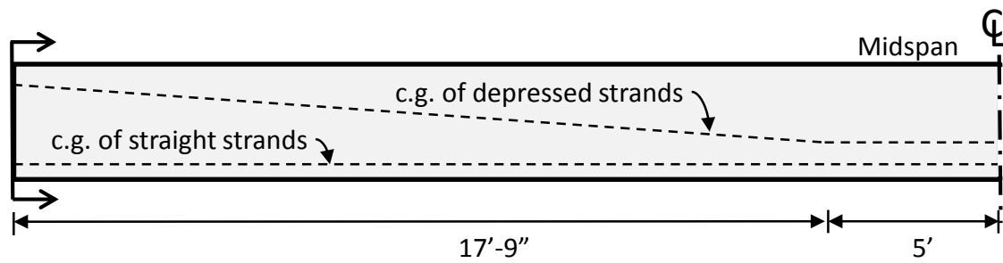
Figure 3.2 – Longitudinal elevation of specimens
