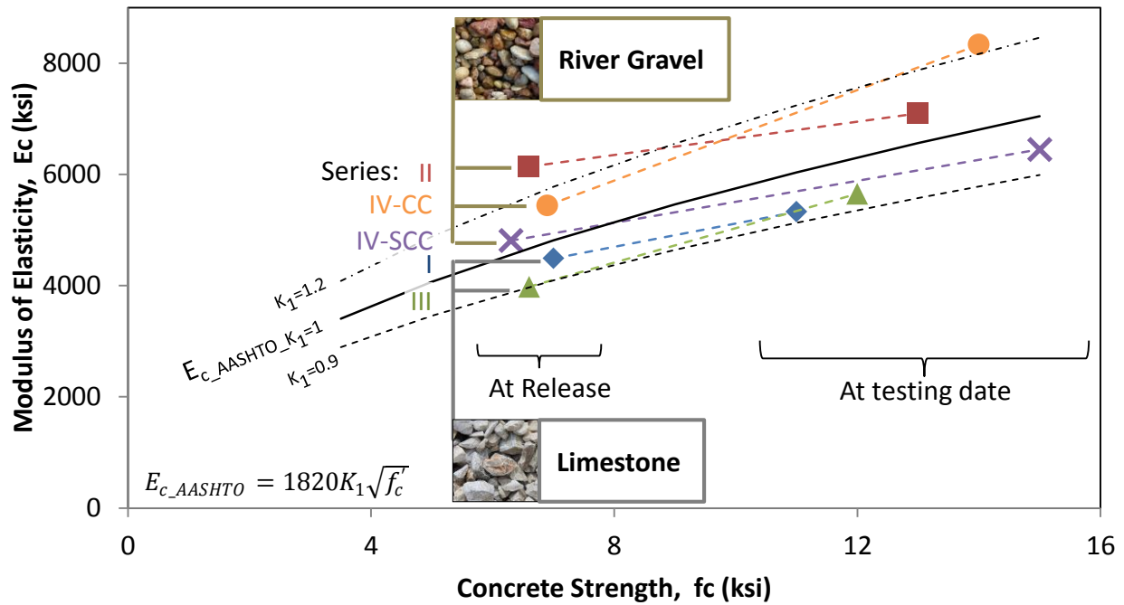
Figure 4.1 – Concrete modulus of elasticity
