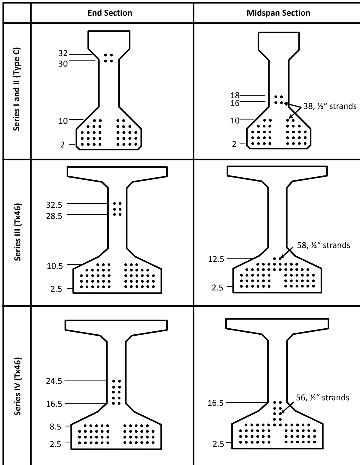
Figure 3.3 – Prestressing strand layout for all series (all dimensions are offsets from bottom of girder assuming a 2-inch grid)
